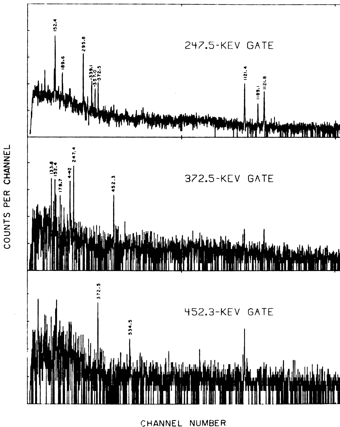
Figure 6. Coincidence gates associated with the K^\pi = 2^- octupole band.
