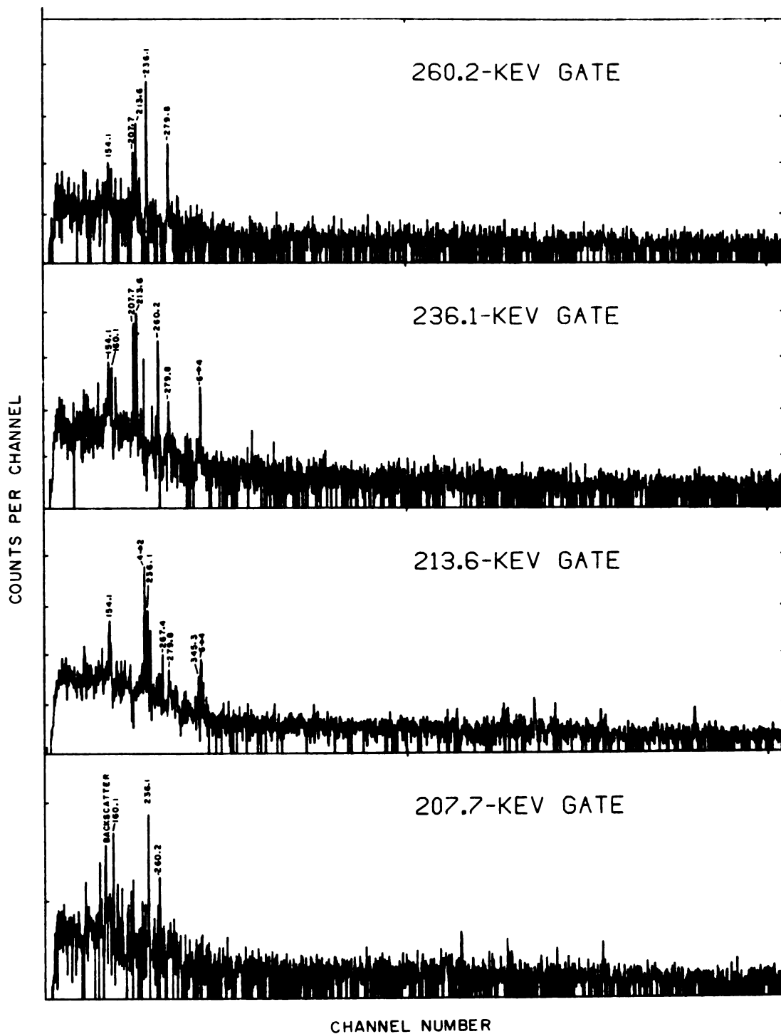
Figure 10. Coincidence gates associated with the K^\pi = 8^- band.
