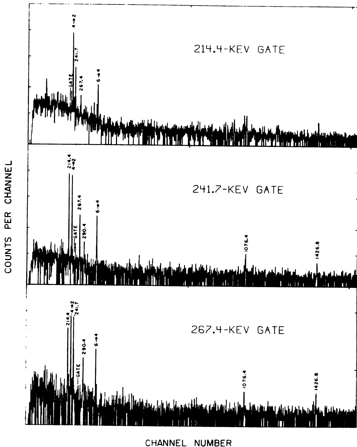
Figure 8. Coincidence gates associated with the K^\pi = 6^+ bands.
