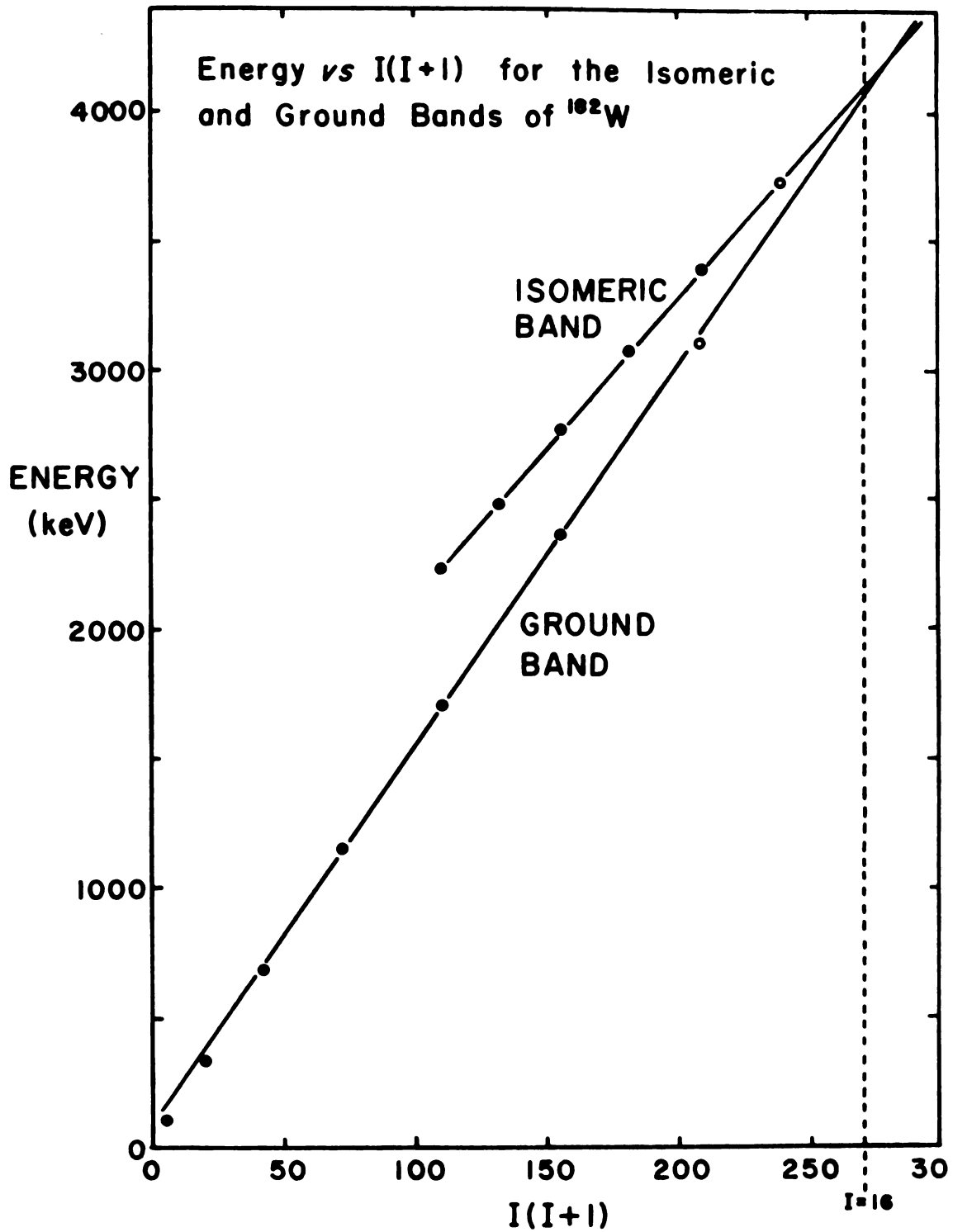
Figure 19. A plot of energy vs. I(I+1) for the ground and K^\pi = 10^+ bands in ^{182}\text{W} .
