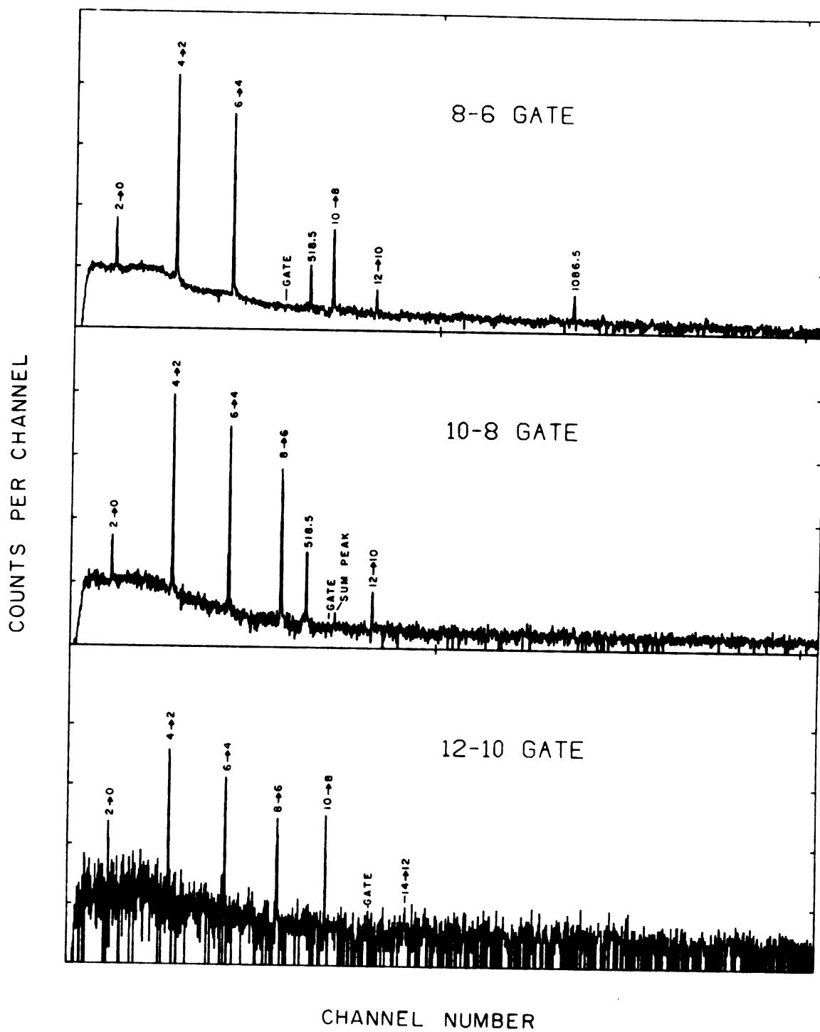
Figure 16. Coincidence spectra associated with the ground state band.
