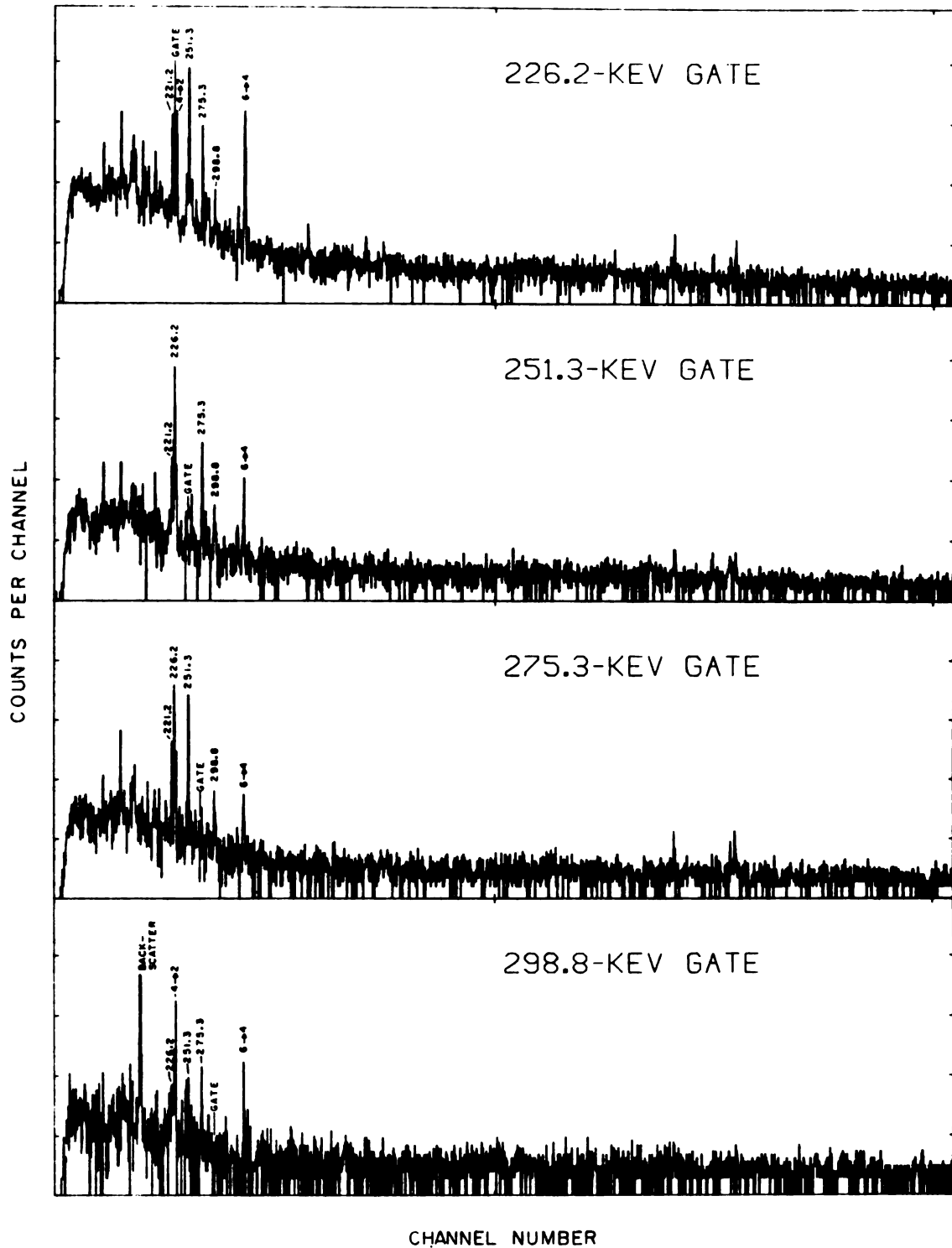
Figure 9. Coincidence gates associated with the K^\pi = 7^- band.
