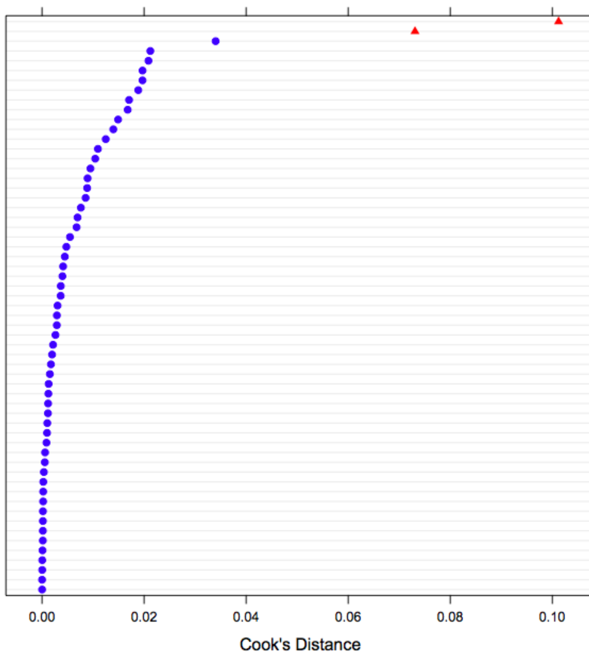
Figure C.1: Influence Country Robust Check for Model 4
