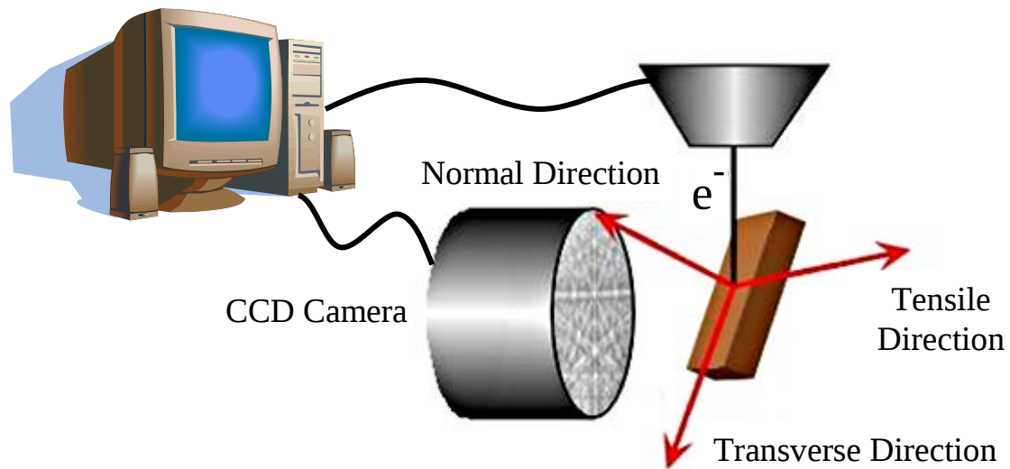
Figure II-15. The schematic shows an EBSD configuration. The electron beam interacts with a sample that is tilted 70^\circ . Backscattered electrons form diffraction patterns on the phosphor screen that are imaged by CCD camera. A computer controls the electron beam, indexes the imaged diffraction pattern, and saves the orientation of each data point. Axes are defined directions on the sample: the transverse direction, tensile direction, and normal direction.
