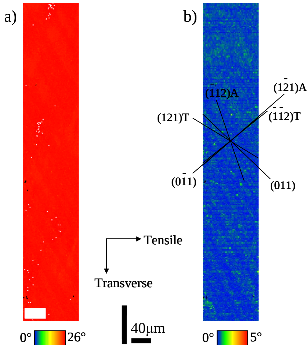
Figure IV-25. Two different representations of the same orientation data obtained after deformation of sample T3 from an 112x327μm area with 1μm step size. The scale bars are common to both images. a) A map of relative difference between the deformed and initial orientations with a range from 0°(blue) to 26°(red). b) A local average misorientation map based on first neighbors with a range of average misorientation from 0°(blue) to 5°(red).
