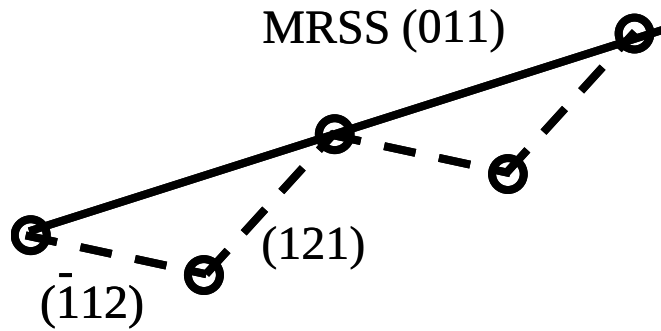
Figure V-6. Schematic of a slip trace along the MRSS plane, which appears to be a (011) slip trace (solid line), though is actually being imitated by the slip traces of a \{112\} slip relaxation screw dislocation (dashed lines) due to frequent cross slip (at the open circles). Imitation seems most plausible if the (121) and (\bar{1}12) planes both possess reasonably high resolved shear stresses. If (\bar{1}12) had a very low resolved glide shear stress or negative non-glide shear stresses, activity on (\bar{1}12) would be less likely, and thus imitation less likely.
