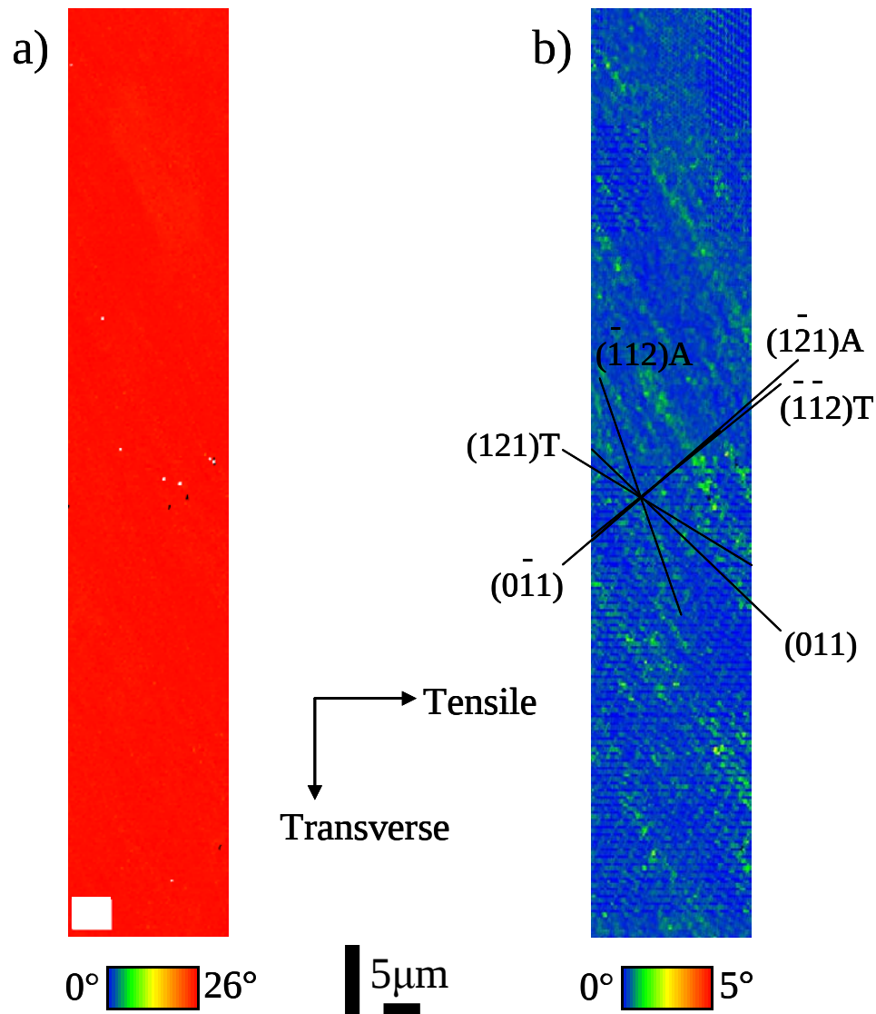
Figure IV-26. Two different representations of the same orientation data obtained after deformation of sample T3 from a 22x65μm area with 0.2 μm step size. The scale bars are common to both images. a) A map of relative difference between the deformed and initial orientations with a range from 0°(blue) to 26°(red). b) A local average misorientation map based on first neighbors with a range of average misorientation from 0°(blue) to 5°(red).
