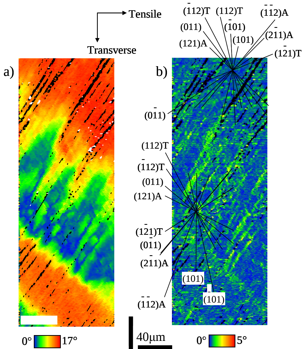
Figure IV-30. Two different representations of the same orientation data obtained after deformation of Sample P3 from an 112x327μm area with 1μm step size. The scale bar is common to both images. a) A map of relative difference between the deformed and initial orientations with a range from 0° (blue) to 17° (red). b) A local average misorientation map based on first neighbors with a range of average misorientation from 0° (blue) to 5° (red).
