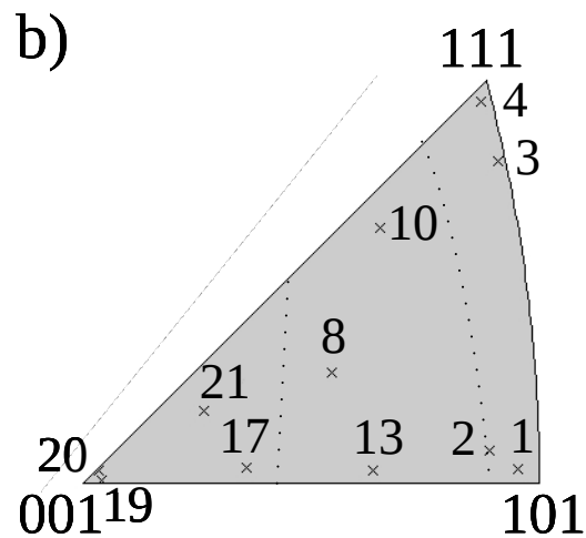
Figure II-6. a) The shear stress-shear strain curves for orientations away from symmetry boundaries. b) The reference triangle plots the tensile axis of D&F specimens to show the variation of shear stress-shear strain behavior with crystal orientation. The dashed lines are the boundaries between different observed primary slip planes from Figure II-4b (reproduced and adapted from [24]).
