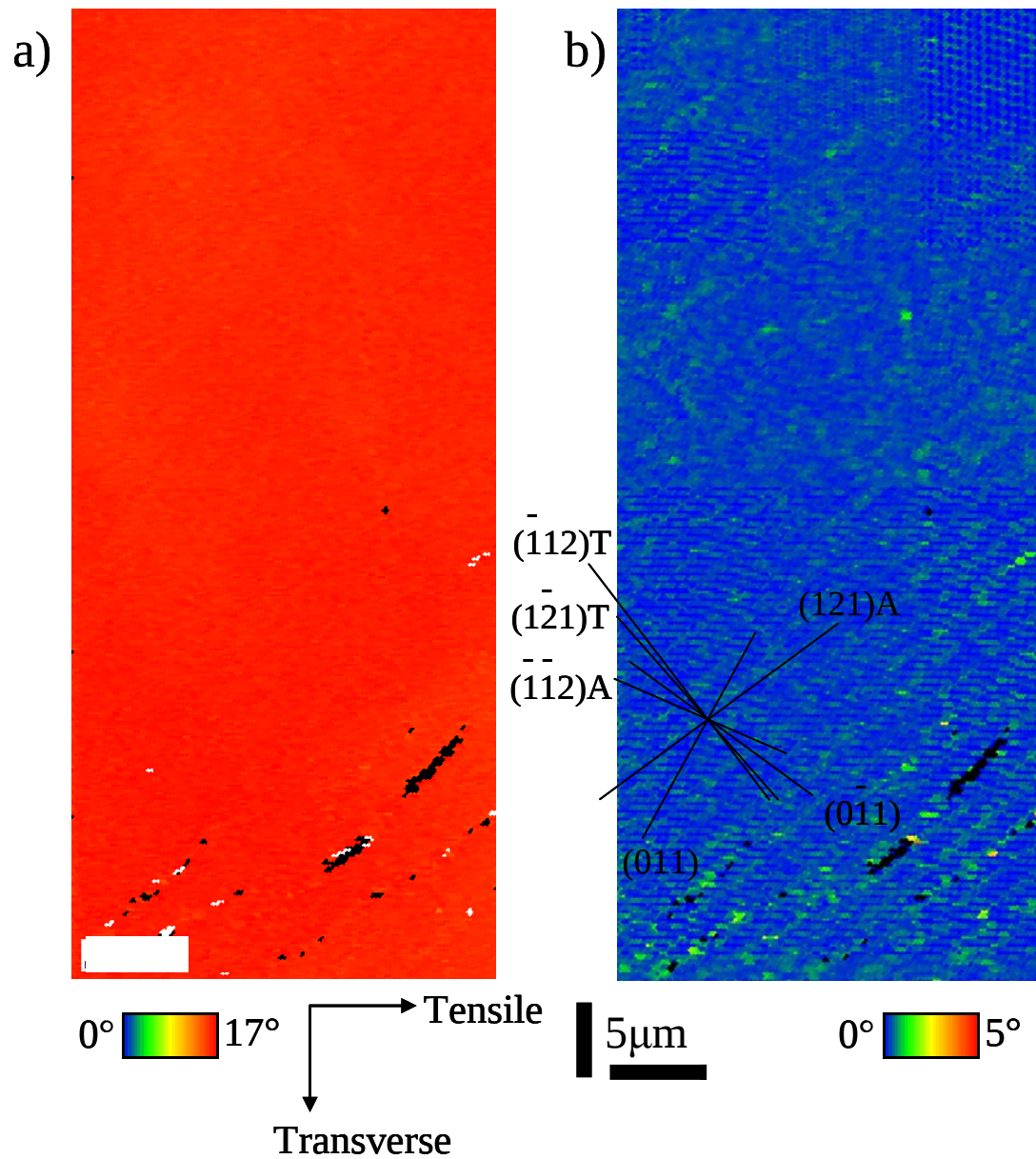
Figure IV-21. Two different representations of the same orientation data obtained after deformation of sample X3 from a 22x65μm area with 0.2 μm step size. The scale bar is common to both images. a) A map of relative difference between the deformed and initial orientations with a range from 0°(blue) to 17°(red). b) A local average misorientation map based on first neighbors with a range of average misorientation from 0°(blue) to 5°(red).
