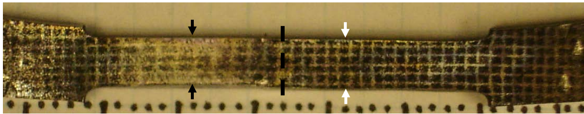
Figure IV-14. a) Side view of Sample A after deformation. The sample was cut in half (dashed line). The left side became welded sample AF side A, and had thinned from \sim 3\text{mm} to \sim 2\text{mm} (black arrows). The right side became welded sample CA side A, and remained \sim 3\text{mm} thick (white arrows). b) Back of Sample A after deformation with fiducial spots. Areas of the left side had upwards of 60% local strain (black arrows) along the long axis, while the right side had around 7% (white arrows).
