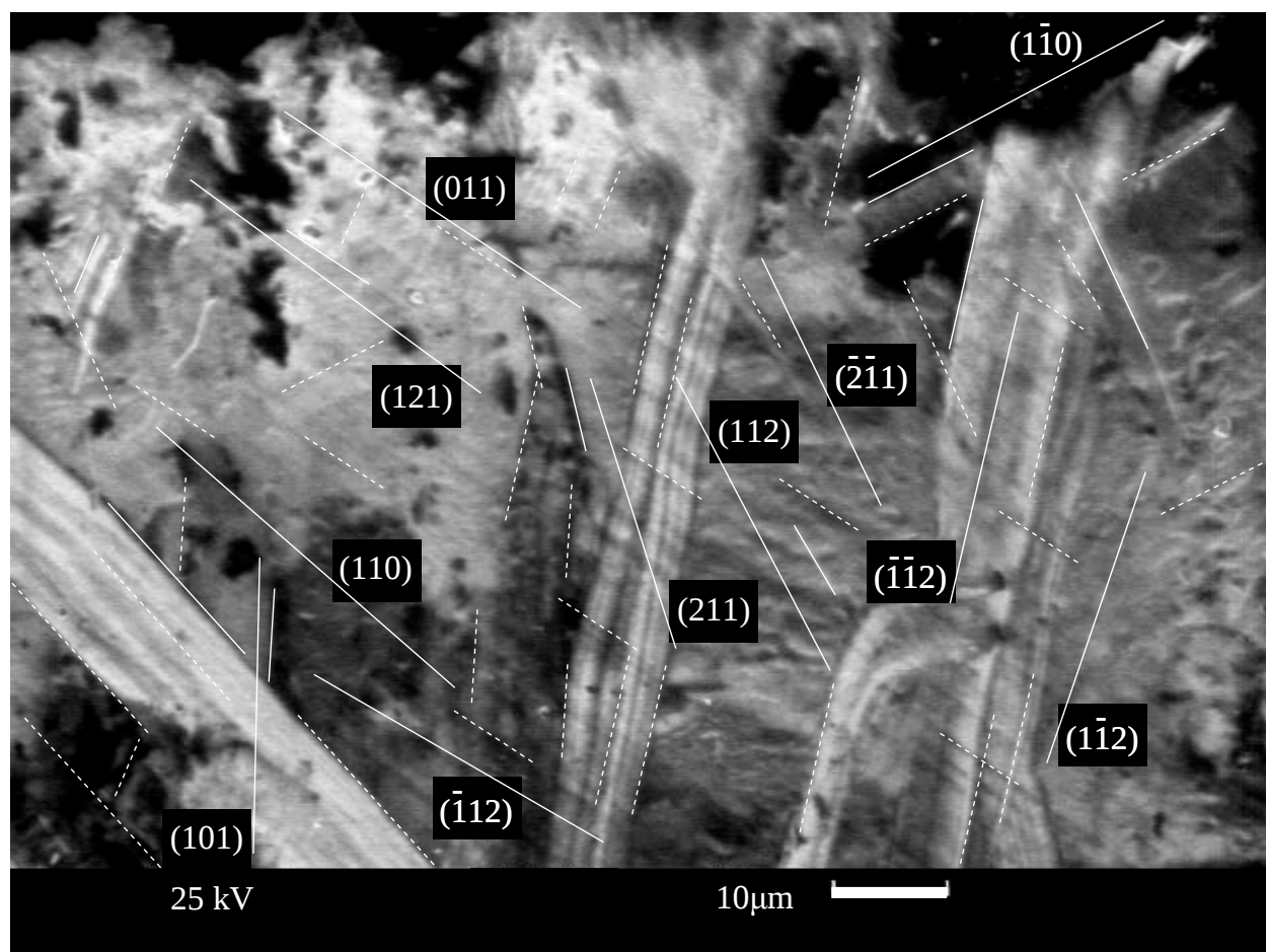
Figure A-17. Slip traces on the transverse surface of sample R2 after deformation (SEI). Calculated slip traces are the long labeled lines to which the visible traces (short white solid and short white dashed lines) were matched.
