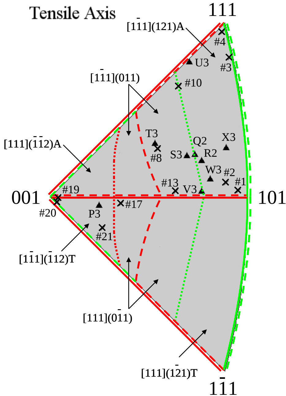
Figure V-9. This stereographic projection section shows the initial tensile axes for the D&F and Ningxia sample sets. The slip system whose Schmid factors are greatest in the area between boundaries are labeled. The boundaries mark where the Schmid factors of all the different slip systems are equal between two different: \{110\} slip systems (solid lines), \{112\} slip systems (dashed lines), \{110\} and \{112\} slip systems (dotted lines). The boundary between the slip systems is colored: same slip directions (green), intersecting slip directions (red).
