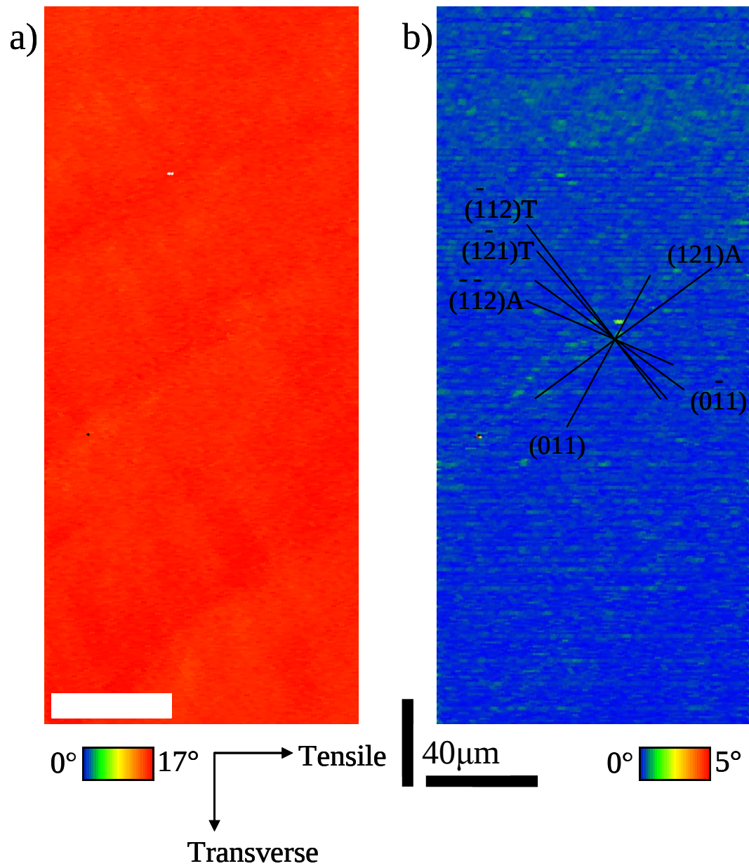
Figure IV-20. Two different representations of the same orientation data obtained after deformation of sample X3 from an 112x327μm area with 1μm step size. The scale bars are common to both images. a) A map of relative difference between the deformed and initial orientations with a range from 0°(blue) to 17°(red). b) A local average misorientation map based on first neighbors with a range of average misorientation from 0°(blue) to 5°(red).
