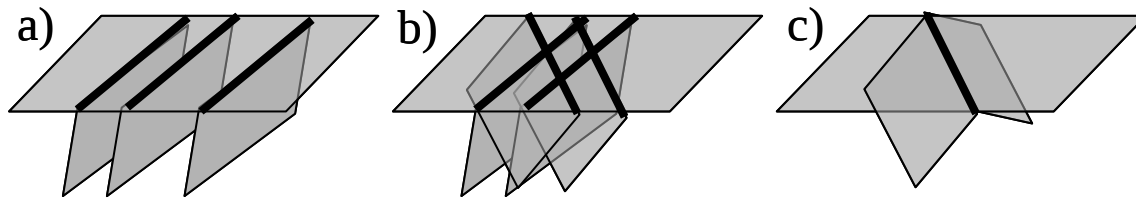
Figure III-5. Examples of slip traces. a) Slip traces of the same slip system are parallel, b) Intersecting slip traces of two different slip systems, c) Two different slip systems that produce a very similar slip trace.
