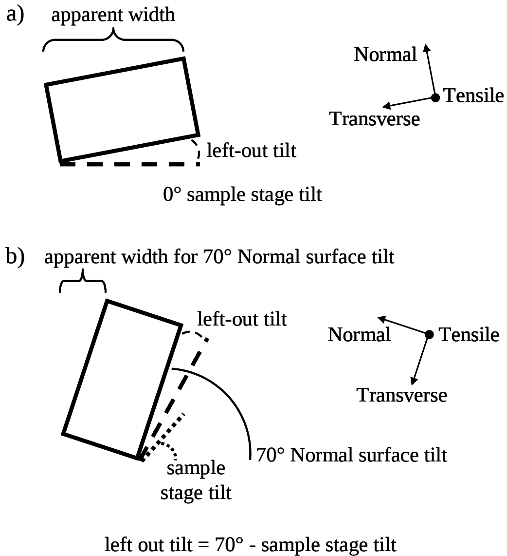
Figure III-4. A schematic of the cross-section of the deformed gage length used to determine the left-out tilt. a) the sample at 0° stage tilt, and b) the sample tilted such that the deformed surface was properly tilted to 70° to enable OIM.
