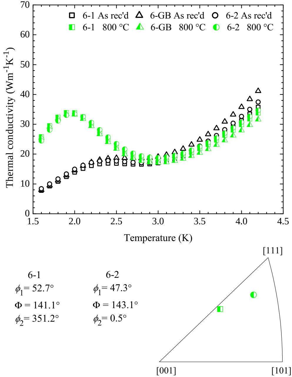
Figure 4.6: The thermal conductivities of the grains 1 (squares) and 2 (circles), and across the grain boundary (triangles) of specimen 6 in their as-received condition (open symbols) and after 800 °C for 2 h heat treatment (half-filled symbols). The Euler angles \phi_1 , \Phi , and \phi_2 representing the crystal orientation along the heat flow direction for the two grains after the 800 °C heating, as well as the inverse pole figure illustrating the orientations, are shown below the thermal conductivity plot.
