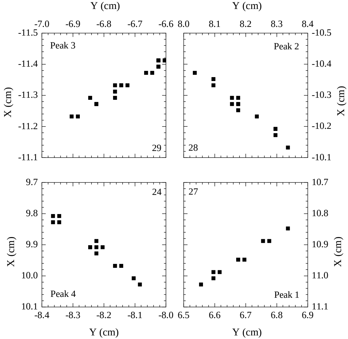
Figure 4.22: Detected peak maximum locations for peaks from \{222\} planes for specimen 9 after the 600 °C for 2 h heat treatment. The x- and y-distances are with respect to the location of the beam on the detector. The four peak clusters are the locations of the X-rays diffracted by the two \{111\} planes identified in Figure 4.18. Each individual cluster is a group of \{222\} peaks from several of the 1620 frames recorded per specimen. The number listed in each cluster, towards the center of the figure, is the actual number of frames from which \{222\} peaks are detected. The spread of the peaks within each cluster represents imperfection density in the crystal.
