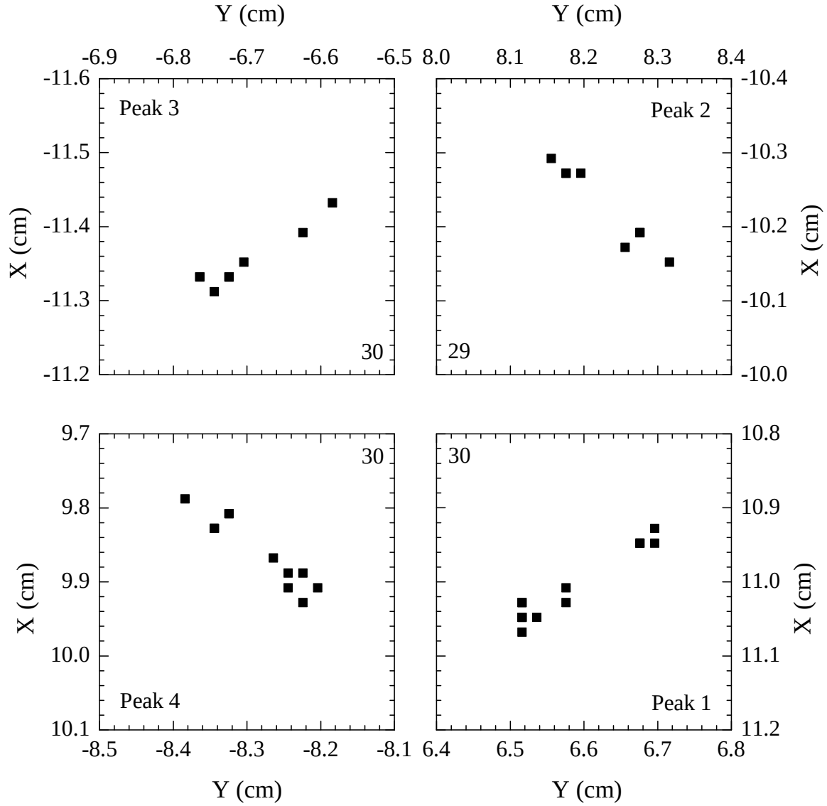
Figure 4.24: Detected peak maximum locations for peaks from \{222\} planes for specimen 11 after the 1000 °C for 2 h heat treatment. The x- and y-distances are with respect to the location of the beam on the detector. The four peak clusters are the locations of the X-rays diffracted by the two \{111\} planes identified in Figure 4.20. Each individual cluster is a group of \{222\} peaks from several of the 1620 frames recorded per specimen. The number listed in each cluster, towards the center of the figure, is the actual number of frames from which \{222\} peaks are detected. The spread of the peaks within each cluster represents imperfection density in the crystal.
