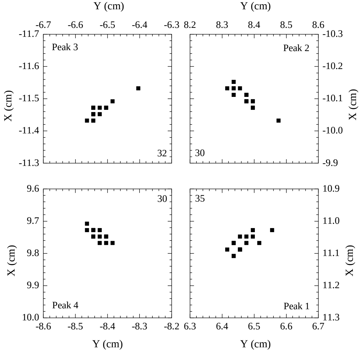
Figure 4.25: Detected peak maximum locations for peaks from \{222\} planes for specimen 12 after the 1200 °C for 2 h heat treatment. The x- and y-distances are with respect to the location of the beam on the detector. The four peak clusters are the locations of the X-rays diffracted by the two \{111\} planes identified in Figure 4.21. Each individual cluster is a group of \{222\} peaks from several of the 1620 frames recorded per specimen. The number listed in each cluster, towards the center of the figure, is the actual number of frames from which \{222\} peaks are detected. The spread of the peaks within each cluster represents imperfection density in the crystal.
