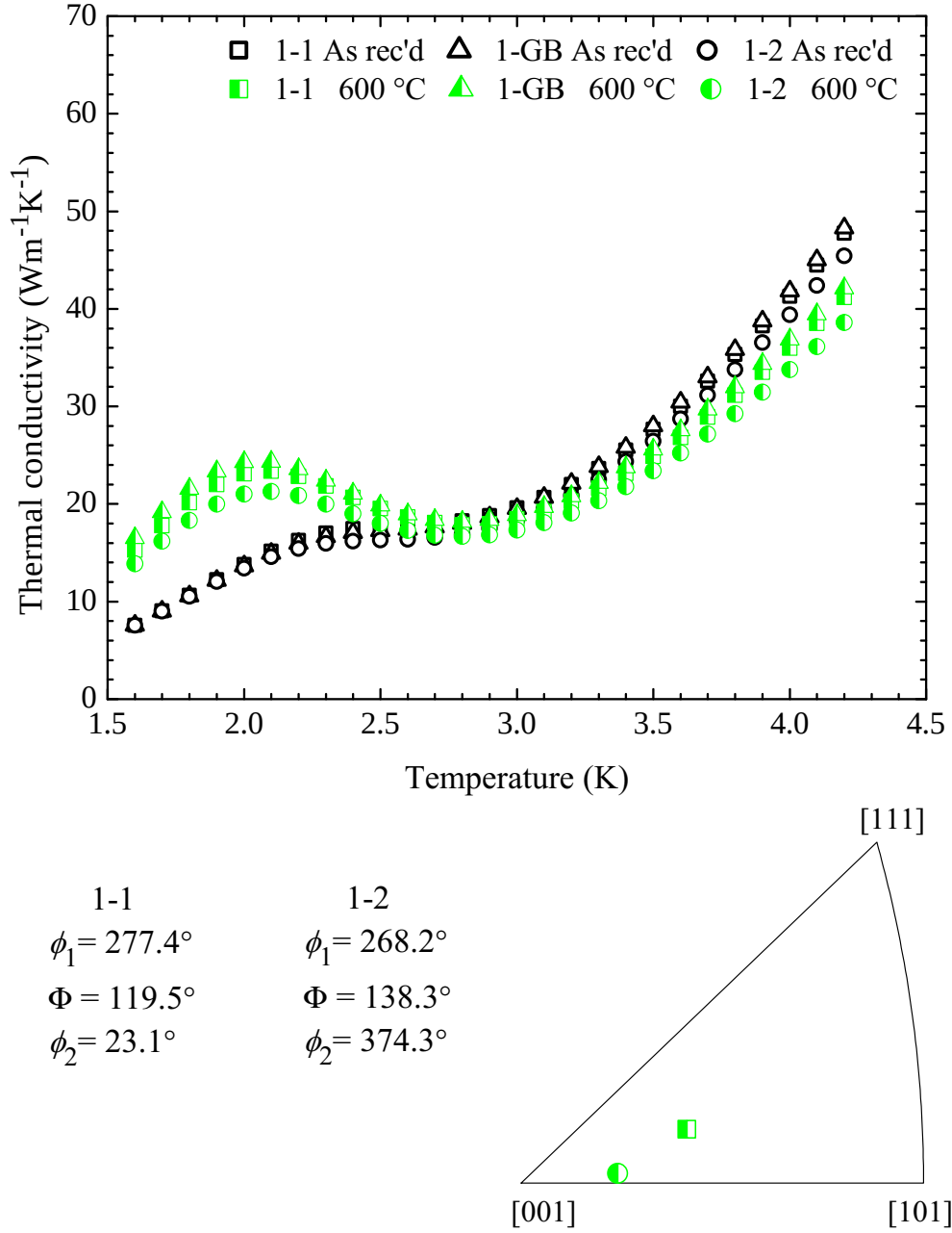
Figure 4.1: The thermal conductivities of grains 1 (squares) and 2 (circles), and across the grain boundary (triangles) of specimen 1 in their as-received condition (open symbols) and after 600 °C for 6 h heat treatment (half-filled symbols). The Euler angles \phi_1 , \Phi , and \phi_2 representing the crystal orientation along the heat flow direction for the two grains after the 600 °C heating, as well as the inverse pole figure illustrating the orientations, are shown below the thermal conductivity plot.
