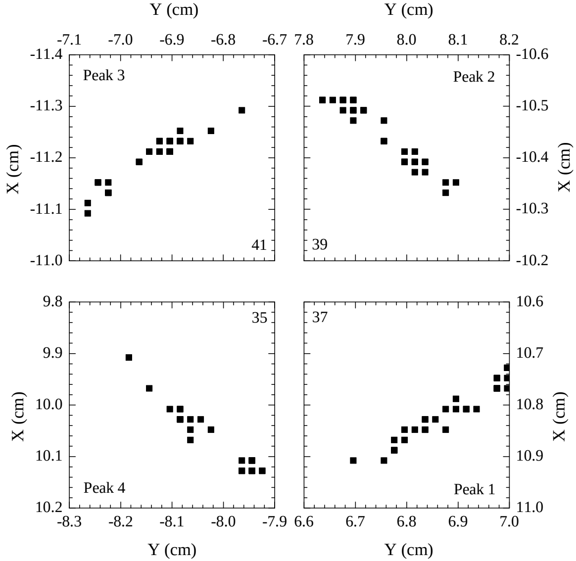
Figure 4.23: Detected peak maximum locations for peaks from \{222\} planes for specimen 10 after the 800 °C for 2 h heat treatment. The x- and y-distances are with respect to the location of the beam on the detector. The four peak clusters are the locations of the X-rays diffracted by the two \{111\} planes identified in Figure 4.19. Each individual cluster is a group of \{222\} peaks from several of the 1620 frames recorded per specimen. The number listed in each cluster, towards the center of the figure, is the actual number of frames from which \{222\} peaks are detected. The spread of the peaks within each cluster represents imperfection density in the crystal.
