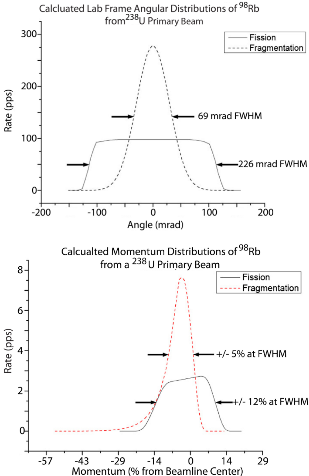
Figure 28: Comparison of the lab frame fragment momentum and angular distributions in fission and fragmentation calculated with LISE++. Typical acceptances for the best fragment separators (such as the A1900 at the NSCL) are \pm 50 mr in angle and \pm 2.5\% in momentum. One can see from the figure that it is impossible to accept the full fission yield with such a device.
