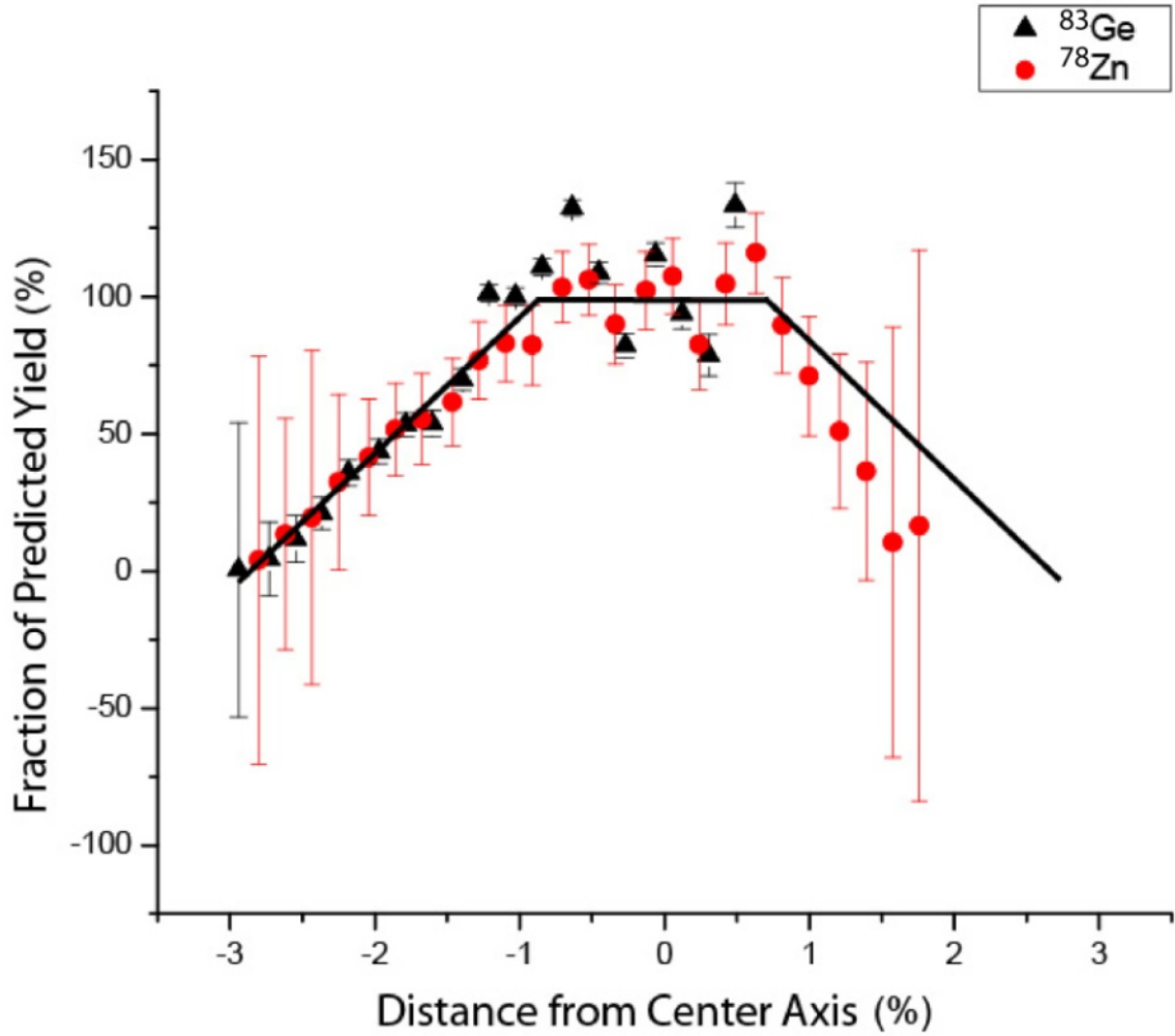
Figure 30: Experimentally determined transmission through the A1900 relative to LISE++ first order predictions as described in the text. The solid line is the predicted fraction taken from a 5 th order LISE Monte Carlo Simulation. This demonstrates the loss of transmission as the fragments are transmitted further from the central axis which is accounted for in higher order LISE++ calculations. Notably only the region of +/- 1% has essentially the predicted first order transmission.
