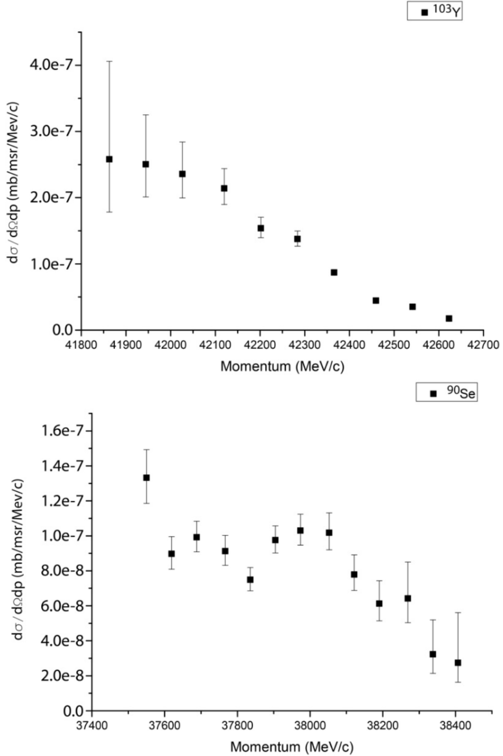
Figure 32: Double Differential Cross Sections determined from recorded momentum distributions. The angular acceptance was taken from the experimentally determined transmission given table 5, for the appropriate momentum deviation from the central trajectory. The distributions, assuming a momentum independent angular transmission, are predicted to show a linear slope similar to the first order predictions in Figure 29.
