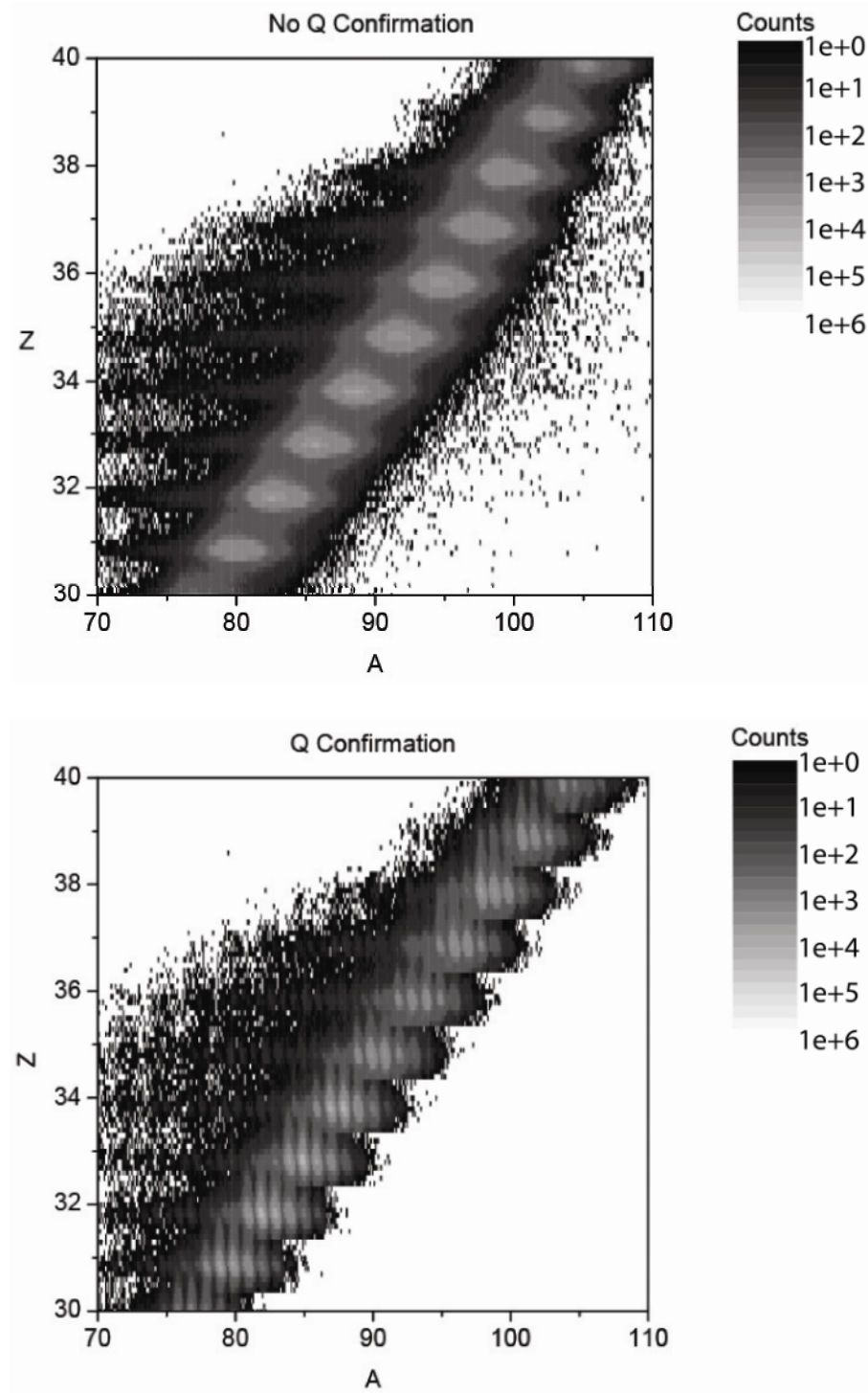
Figure 21: (Top) A typical data set using the charge state calculation based upon the TKE and A/Q . (Bottom) The same data set using an integer value of Q determined with the confirmation method. In this case a number of invalid data points were discarded, cleaning the distribution.
