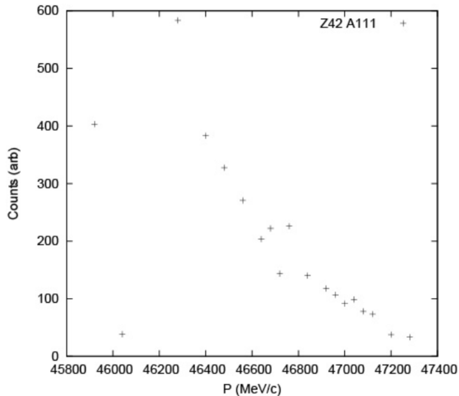
Figure 33: A sample of the momentum distributions generated in this work. The entire set of several hundred partial distributions is available at ( http://www.nscl.msu.edu/~sherrill/nettleton/plots.pdf ).
