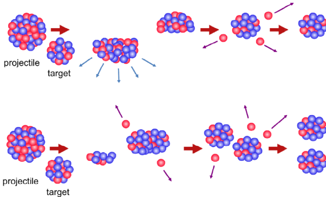
Figure 3 (Top) Pictorial representation of a projectile fragmentation reaction. Note that part of the initial isotope is removed by collision with the target and the remainder continues on essentially unimpeded. Afterwards it deexcites by emission particles or gamma-rays.
