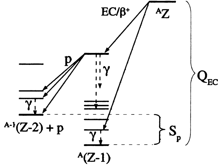
Figure 1.1: Schematic decay scheme illustrating the \beta p -emission process. \beta -decays into daughter excited states above S_p can result in a subsequent proton decay. Competing \gamma -decays are labeled with dashed arrows.
