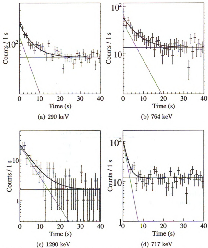
Figure 5.12: Decay curves recorded for the \beta -activity correlated to implantations of ^{97}\text{Cd} in coincidence with selected \gamma rays from the depopulation of levels in the daughter nucleus ^{97}\text{Ag}^*
