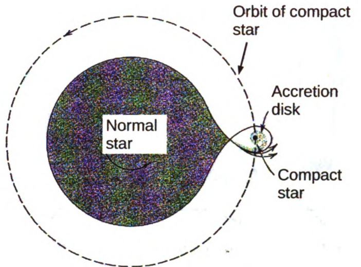
(a) accretion by Roche overflow
