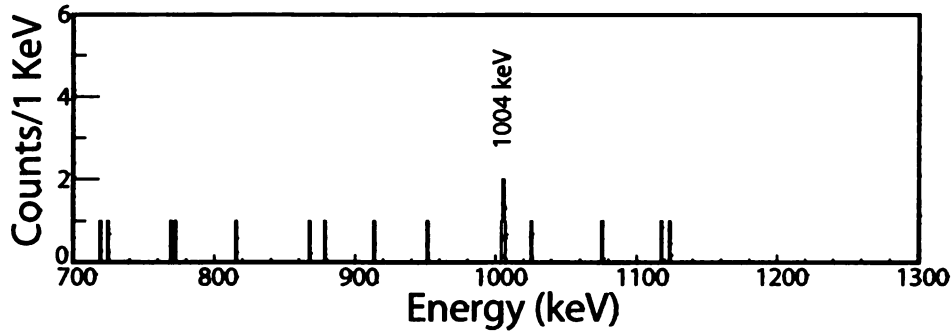
Figure 5.3: 700-1300keV section of the measured \gamma spectra in coincidence with the \beta -delayed protons from the decay of ^{101}\text{Sn} . The labeled peak corresponds to the known de-excitations in the \beta p -daughter ^{100}\text{Cd} 2^+ \rightarrow 0^+ at 1004 keV
