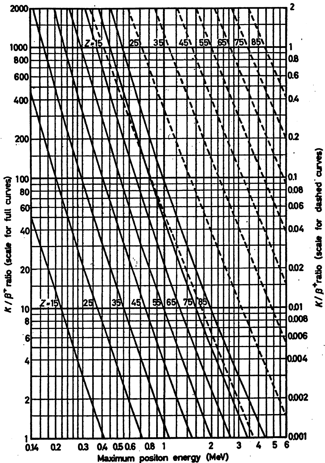
Figure C.1: Theoretical K/\beta^+ ratio for allowed transitions
