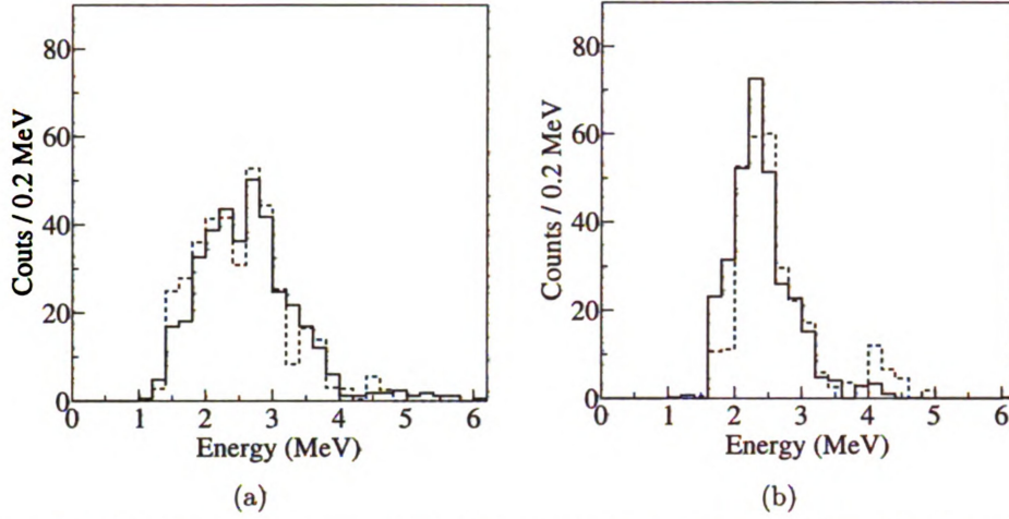
Figure 5.6: Energy spectrum of \beta p -decay events stemming from the decay of (a) the 25/2^+ isomeric state observed in this work (solid-line histogram), and the \beta p -activity observed in [2] (dashed-line histogram). An offset of about 300 keV was applied to the latter spectrum to match our data (b) the 9/2^+ ^{97}\text{Cd} ground state observed in this work, and compared to a shell model prediction (dashed line) [2].
