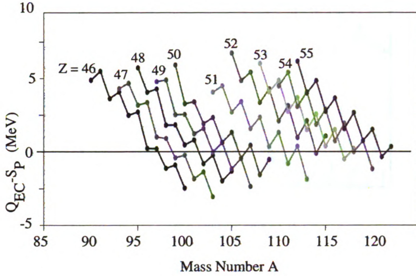
Figure 1.3: Q_{EC}-S_p window near Z = 50 .
