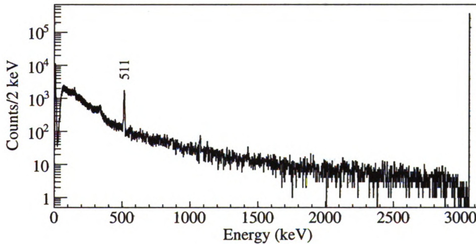
Figure 4.17: Calibrated Ge-detector \gamma -spectra in coincidence with the \beta -decay of ^{96}\text{Ag} . Besides the 511 keV annihilation peak, the spectra also shows that signals more energetic than 3 MeV overflow the ADC.
