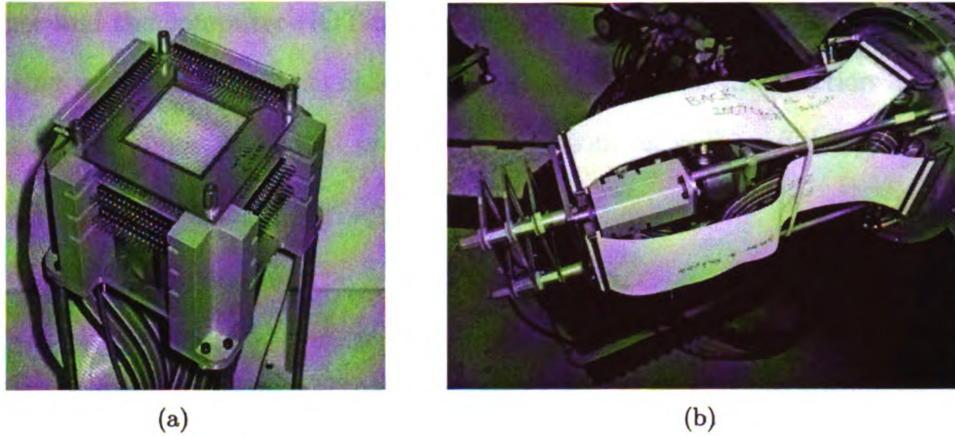
Figure 3.5: (a) up-stream view of the DSSD with its downstream SSSDs. (b) view of the entire silicon stack including the three PIN detectors, and the Ge detector which is hold in place by the copper frame clearly distinguishable in the picture.
