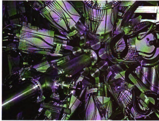
Figure 3.7: View of the Experimental setup. Eight detectors of the SeGA array upstream of the DSSD.
