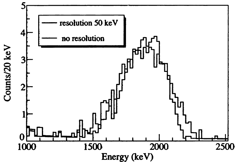
Figure 4.33: MCNP simulations of the calorimeter response including and excluding the finite energy resolution of individual detectors.
