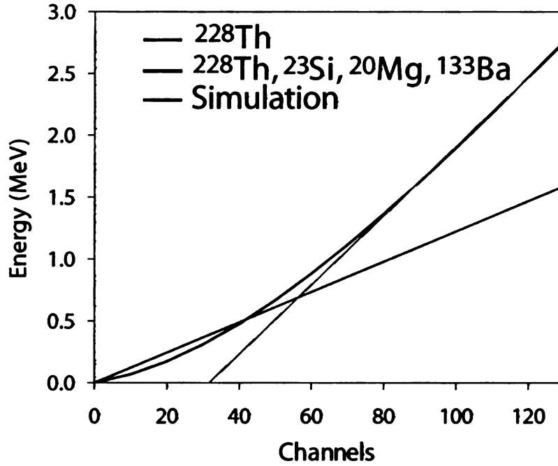
Figure 4.29: Energy calibration of a 500μm DSSD using: a ^{228}\text{Th} alpha source (green line), the sources ^{228}\text{Th} , ^{133}\text{Ba} , ^{23}\text{Si} and ^{20}\text{Mg} (black curve). The red line is a linear approximation of the black curve for energies below 1 MeV, and it is the calibration used for energies below 1 MeV.
