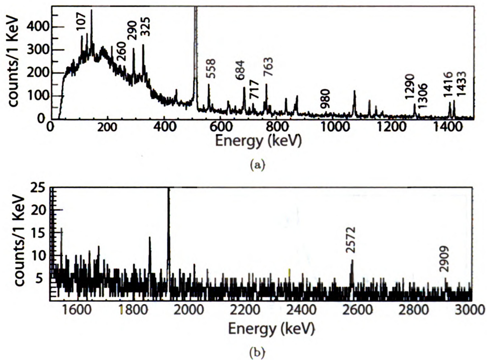
Figure 5.11: Section of the \gamma spectrum recorded in coincidence with ^{97}\text{Cd} \beta -decay events.
