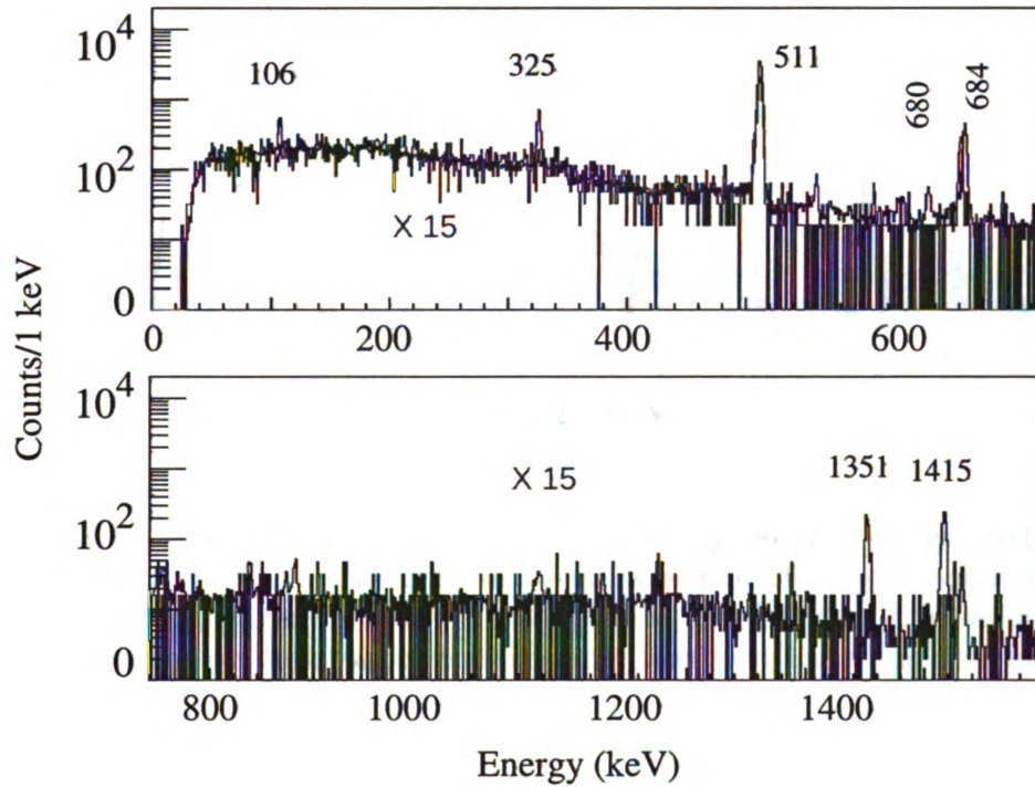
Figure 4.19: \gamma -spectrum of daughter nuclei of 96 Ag gated on \beta -decays (red) and \beta p -decays (blue) of 96 Ag. The blue histogram was multiplied by a factor of 15 to facilitate the comparison between the two spectra. The fact that the two spectra do not have common peaks shows a satisfactory identification of the \beta p -events.
