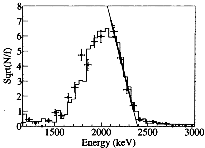
Figure 4.35: (color on line) Curie plot of the energy deposited in the \beta -calorimeter for the events in which the DSSD, SSSD1, SSSD2, SSSD3, and SSSD4 detect a particle. A simulation for these events is represented by the red histogram. The extrapolation of the linear fit of the spectra performed in the range highlighted in green allows Q-value determination.
