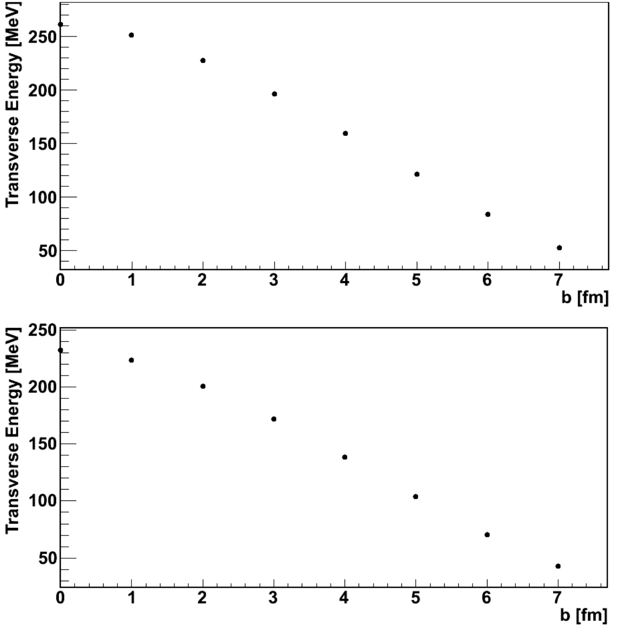
Figure 4.16: Transverse energy as a function of impact parameter for ^{40}\text{Ca}+^{40}\text{Ca} reaction (top) and ^{48}\text{Ca}+^{48}\text{Ca} reaction (bottom) for the Rostock cross section reduction.
