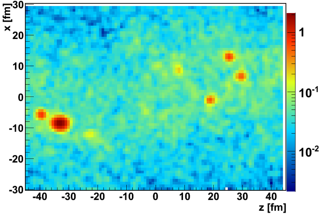
Figure 4.3: XZ plane projection of central ^{40}\text{Ca}+^{40}\text{Ca} reaction at 395 fm/ c with cluster production. The masses of the five largest residues were calculated. The sum of the residue masses is displayed in Table 4.1.
