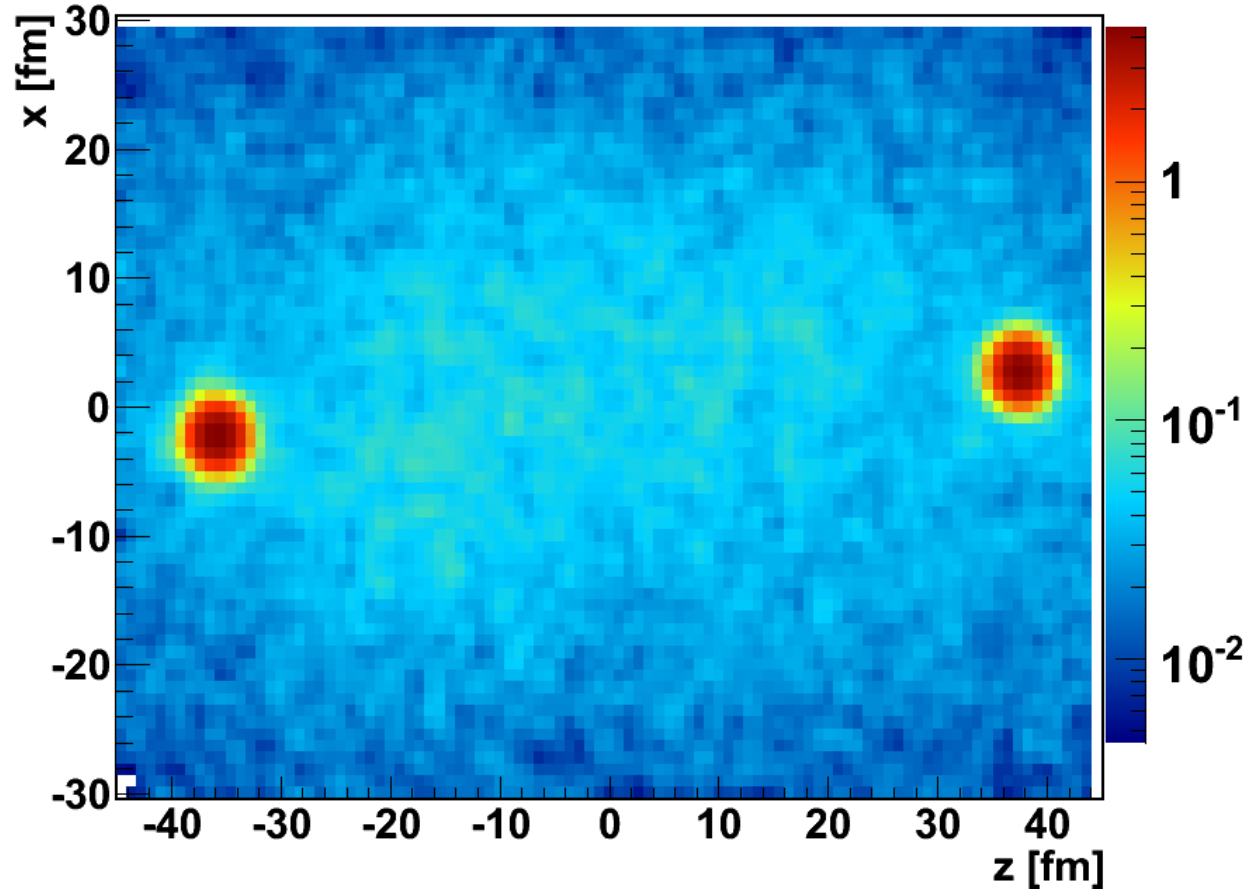
Figure 4.1: XZ plane projection of central ^{40}\text{Ca} + ^{40}\text{Ca} reaction at 395 fm/ c without cluster production. The masses of the two large residues were calculated. The sum of the residue masses is displayed in Table 4.1.
