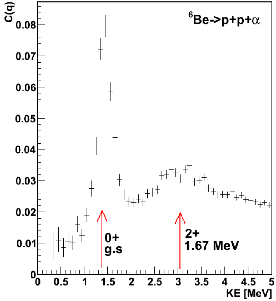
Figure 5.16: 3-particle correlation for {}^6\text{Be} \rightarrow p + p + \alpha . Known states are labeled by red arrows.
