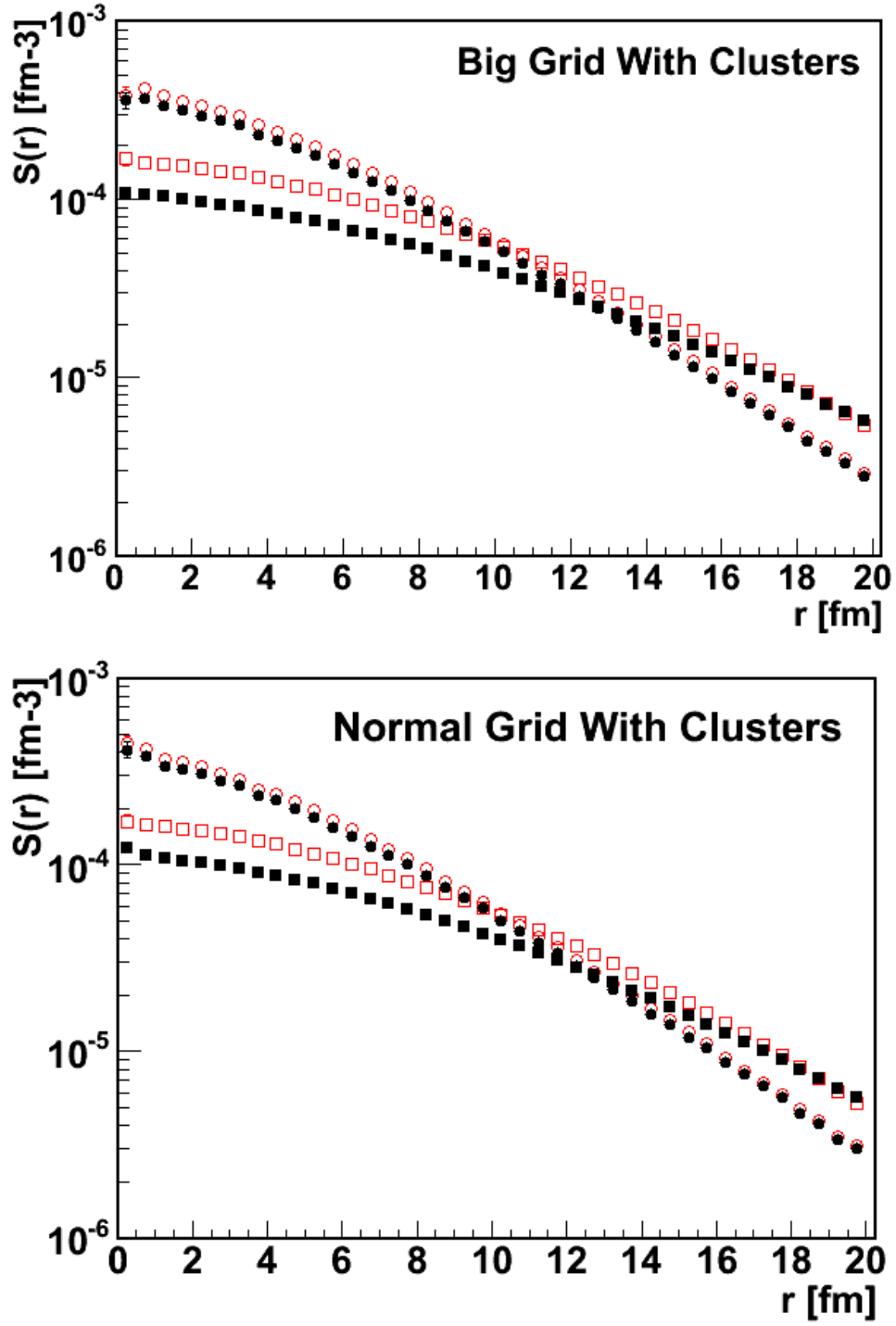
Figure 4.9: Effect of using a time cut on source functions for ^{48}\text{Ca}+^{48}\text{Ca} with cluster production. The legend is the same as the previous figure. r_{1/2} sizes for the sources are given in Table 4.2.
