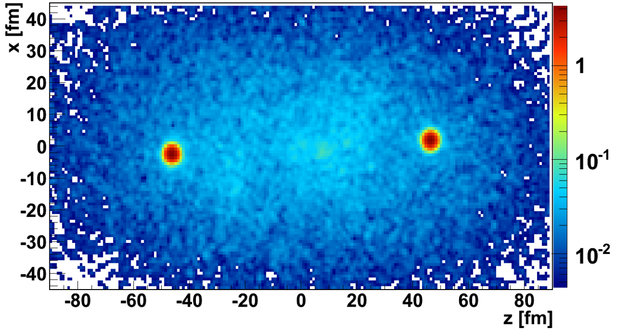
Figure 4.2: XZ plane projection of central ^{40}\text{Ca}+^{40}\text{Ca} reaction at 495 fm/ c without cluster production for a larger computational grid size. The masses of the two large residues were calculated. The sum of the residue masses is displayed in Table 4.1.
