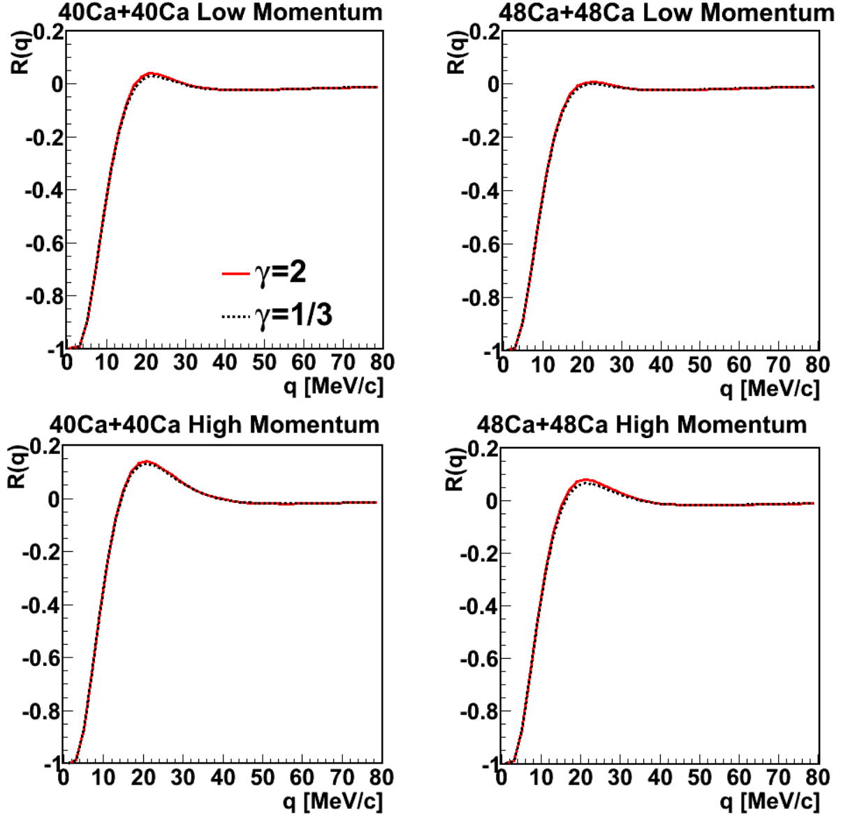
Figure 4.34: Correlation functions for stiff and soft symmetry energy. The upper quadrants are for a low total momentum cut P < 300 MeV/ c for ^{40}\text{Ca}+^{40}\text{Ca} (left) and ^{48}\text{Ca}+^{48}\text{Ca} (right). The bottom quadrants are for a high total momentum cut P > 500 MeV/ c for the same reaction systems.
