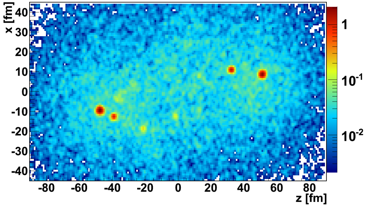
Figure 4.4: XZ plane projection of central ^{40}\text{Ca}+^{40}\text{Ca} reaction at 495 fm/ c with cluster production for a larger computational grid size. The masses of the four largest residues were calculated. The sum of the residue masses is displayed in Table 4.1.
