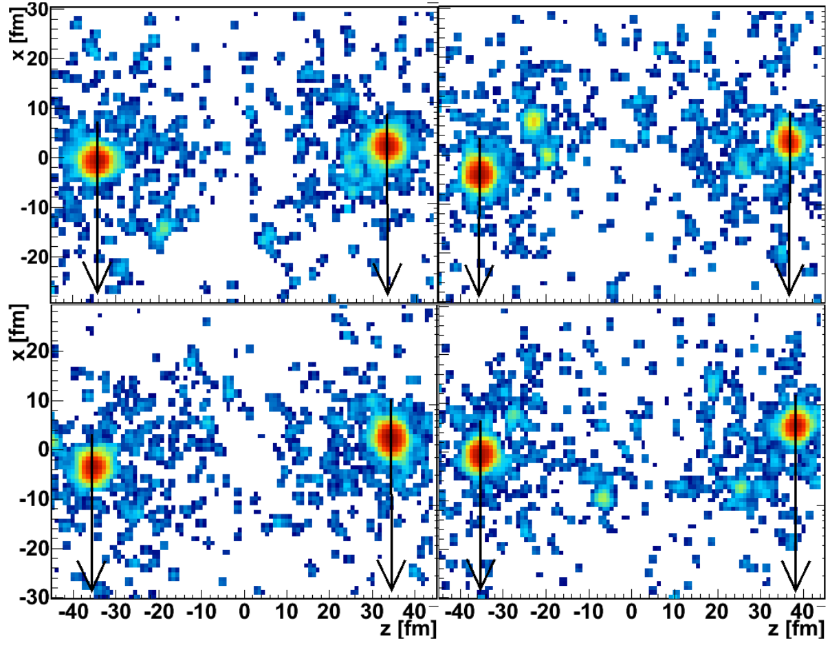
Figure 4.11: Snapshots of the ^{40}\text{Ca}+^{40}\text{Ca} reaction in the XZ plane at 300 fm/ c . Thin slices in the Y plane centered about y = 0 . All panels are for 200 test particles, with different random number seeds.
