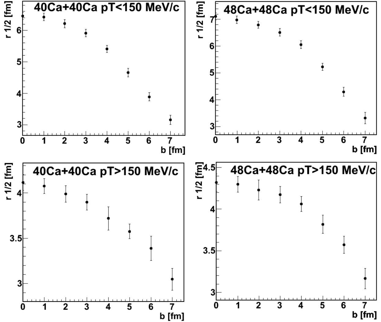
Figure 4.19: r_{1/2} of source functions resulting from Rostock cross section reductions as a function of impact parameter. The upper quadrants are for a low transverse momentum cut <150 MeV/c for ^{40}\text{Ca}+^{40}\text{Ca} (left) and ^{48}\text{Ca}+^{48}\text{Ca} (right). The bottom quadrants are for a high transverse momentum cut >150 MeV/c for the same reaction systems.
