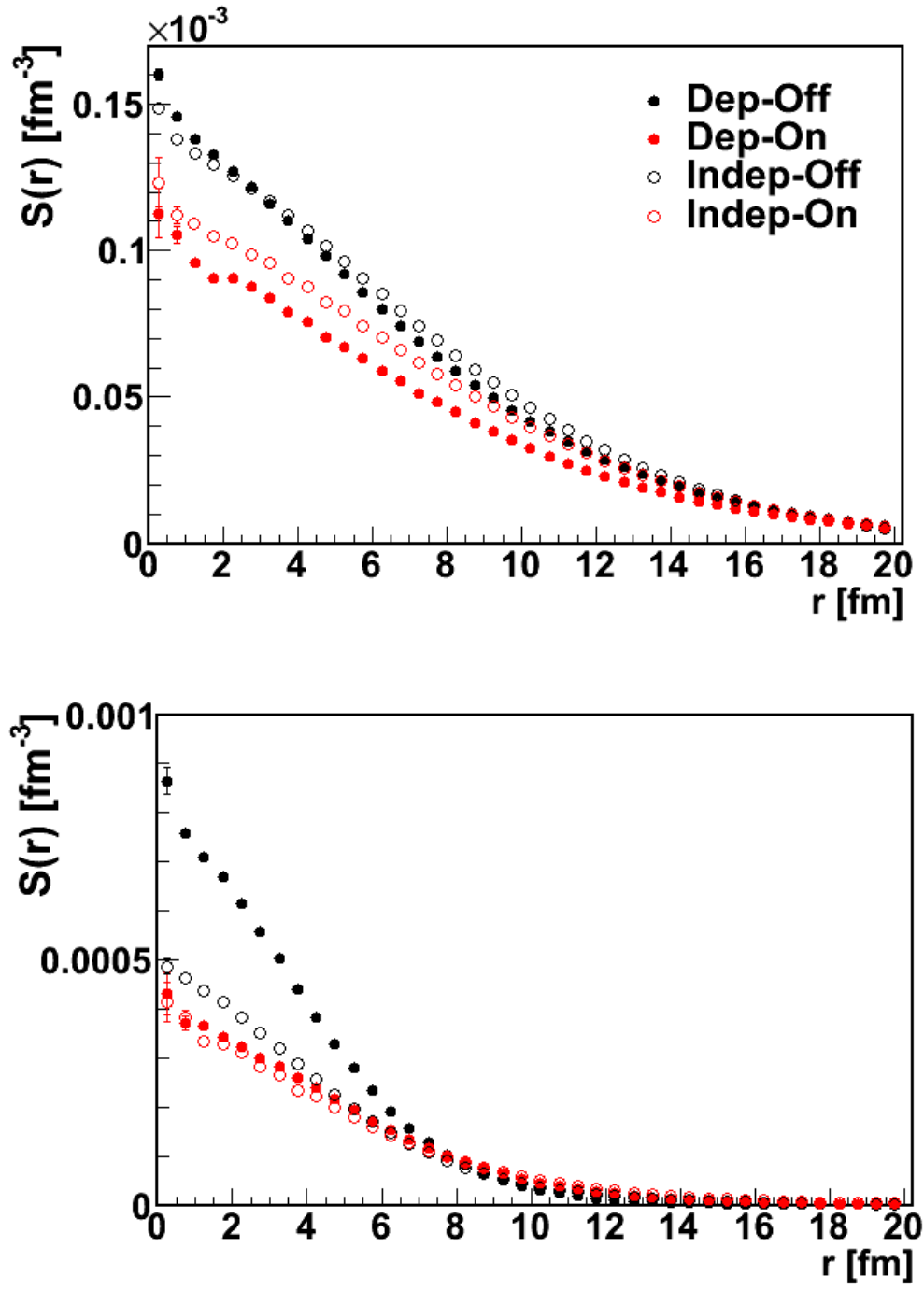
Figure 4.25: Source functions for low p_T (top) and high p_T (bottom) gates for the ^{48}\text{Ca} + ^{48}\text{Ca} reaction system.
