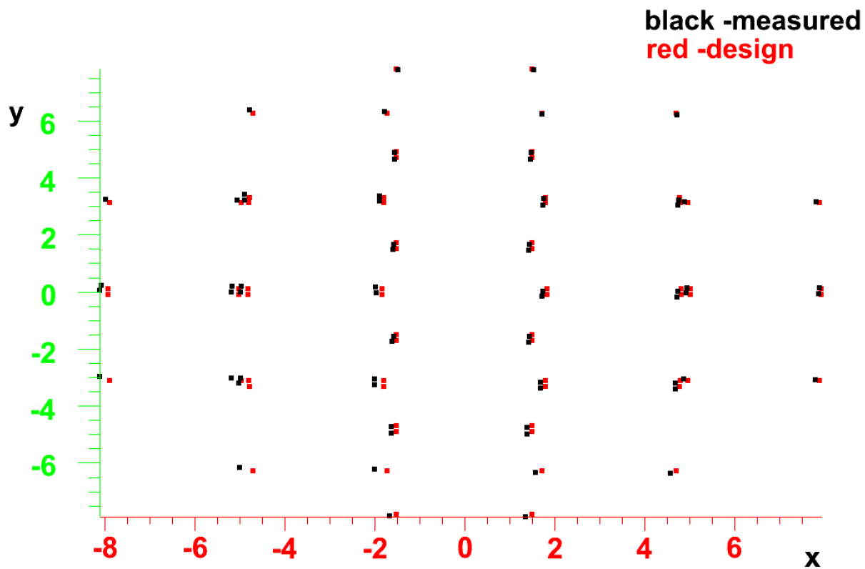
Figure A.1: The black dots are corners of the detectors as measured by LBAS. The red dots are corners of the detectors as given by the design of the mechanical setup for the array. The discrepancy shows the need for such a laser measurement. Units are in inches.
