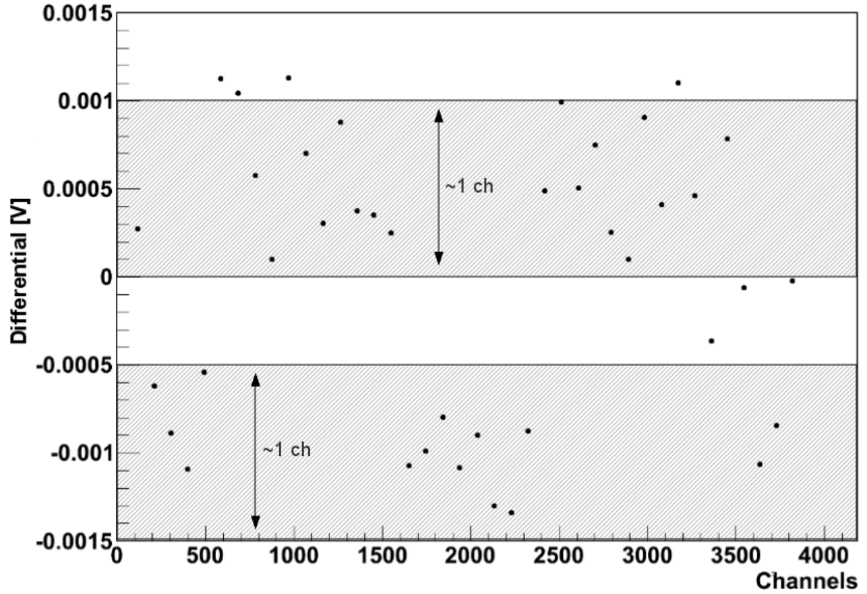
Figure 3.6: The difference between the input voltage and fit voltage is plotted as a function of channel number.
