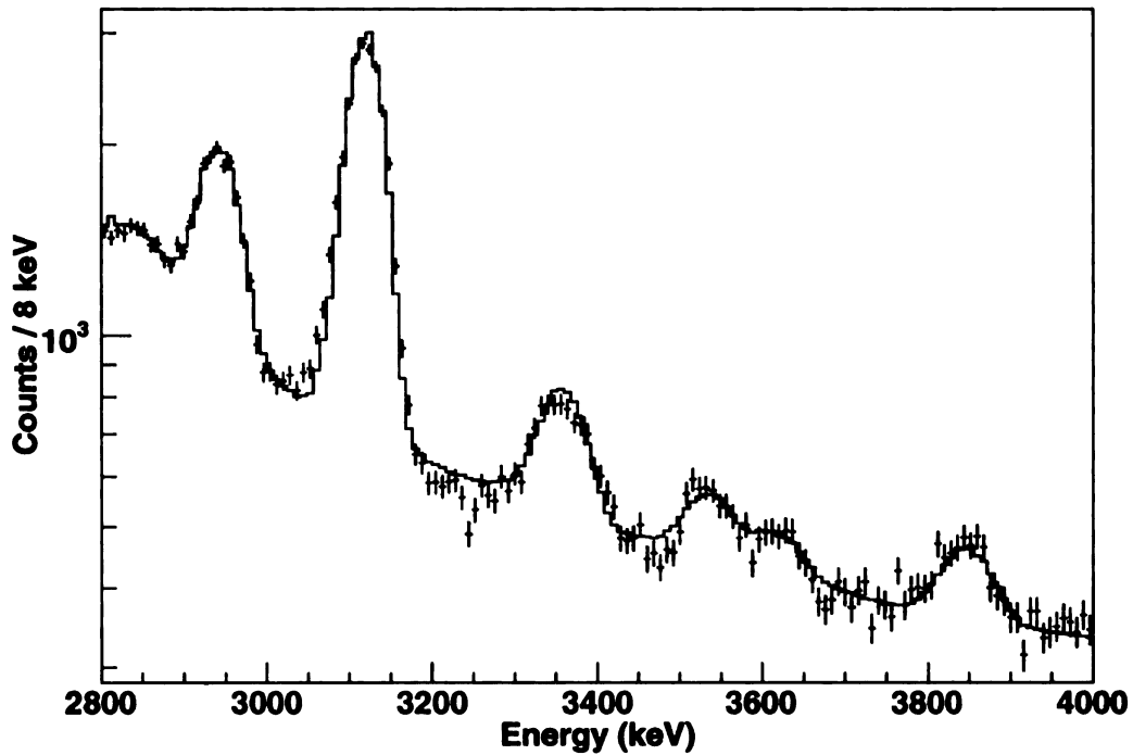
Figure 3.9: The data histogram from the 90^\circ ring in SeGA is shown as points with errors. The black curve is the fitted sum of GEANT response functions with an exponential background. Each individual response function is plotted in gray including the background.
