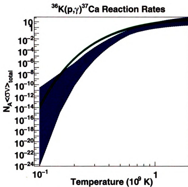
Figure 4.5: The new calculated reaction rate for ^{36}\text{K}(p,\gamma)^{37}\text{Ca} based on the measurements in this work [green] over the previously estimated reaction rate [blue]. The uncertainty of the previous rate was estimated assuming a 100keV uncertainty in the excited state energies. The uncertainties shown are due to the uncertainty in the resonance energy.
