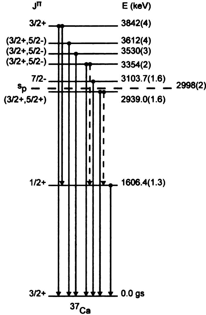
Figure 4.1: Excited states and transitions observed in the experiment. Transitions whose observation is questionable are marked with dashed rather than solid lines. Spins and parities are not measured, but rather are inferred based on the structure of the mirror nucleus, with the most tenuous inferences in parenthesis. The proton separation energy is marked by the dotted line. (Levels are not entirely to scale)
