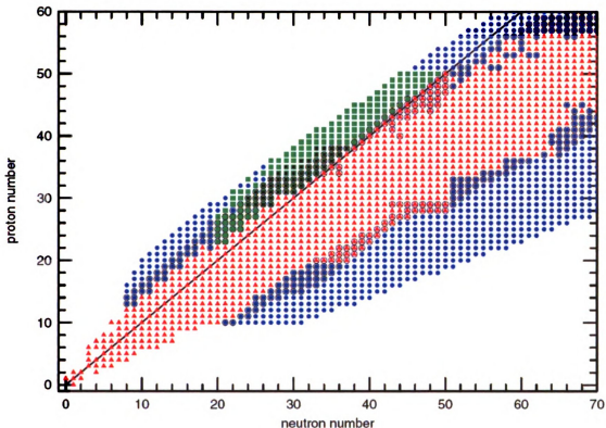
Figure 2.4: (Excerpted from [16], including internal references) Nuclear mass excesses taken from different data sources in the region of interest for the rp-process. A dark line shows the location of nuclei with Z = N . Red triangles indicate nuclei with experimentally determined mass excesses (Audi & Wapstra 1995). Nuclei with black circles surrounding a symbol indicate that an extrapolated or interpolated mass is available from Audi & Wapstra. For those circles enclosing a red triangle, these estimated values were used. Green squares, circled or not, show where data from Brown et al. (2002) and Brown (2002) was used. These add a calculated displacement energy to the Audi-Wapstra masses for N \geq Z to obtain the masses of mirror nuclei with Z > N . For a subset of these (black squares inside green squares) from Brown et al. (2002), the errors in the calculated displacement energies are \approx 100 keV. The solid green squares which cover a wider region are from Brown (2002) and have a larger error of several hundred keV in the calculated displacement energy due to the wider extrapolation and the possible effects of deformation in the A = 80 mass region. In the region of N = Z from A = 76 –100, the error in the mass excess is dominated by the error in the Audi & Wapstra extrapolations, which are on the order of 0.5 MeV. Finally, blue circles indicate mass excess data taken from Möller et al. (1995). These were used wherever shown, (circled or uncircled).
