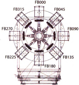
Figure 3.4: The SeGA detectors were arranged in classic configuration for this experiment with a total of 16 detectors, seven in the forward ring and nine in the 90° ring. The circle in the center of each diagram is the beam pipe. Just outside the beam pipe are the cylindrical germanium crystals of SeGA. The larger cylinders near the edge of each diagram are the liquid N 2 dewars. Shown in this diagram is the full complement of 18 detectors.
