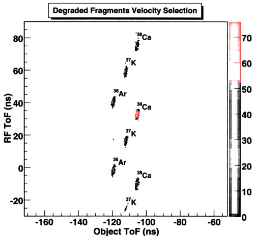
Figure 3.2: The RF ToF plotted against the Object ToF as in Figure 3.1 but in this case showing only events where the outgoing fragment is the same as the incoming fragment. The scale is the same on both axes to clearly show the slope in the degraded fragments due to the different lengths of the RF ToF and Object ToF flight paths.
