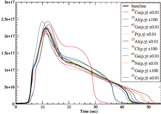
Figure 5.1: The ten most altered burst lightcurves from the single-zone sensitivity study of (p,γ) reaction rates are shown together with the baseline lightcurve generated using the standard ReacLib v1.0 reaction rate database to which they were compared.
