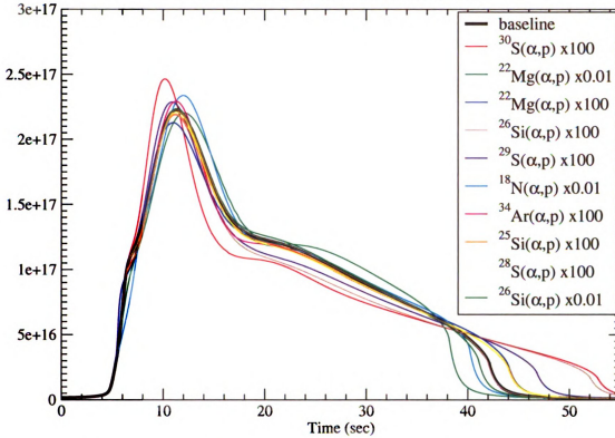
Figure 5.2: The ten most altered burst lightcurves from the single-zone sensitivity study of (\alpha, p) reaction rates are shown together with the baseline lightcurve generated using the standard ReacLib v1.0 reaction rate database to which they were compared.
