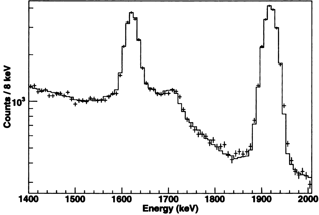
Figure 3.12: The data histogram from the 90^\circ ring in SeGA is shown as points with errors. The black curve is the fitted sum of GEANT response functions with an exponential background. Each individual response function is plotted in gray including the background.
