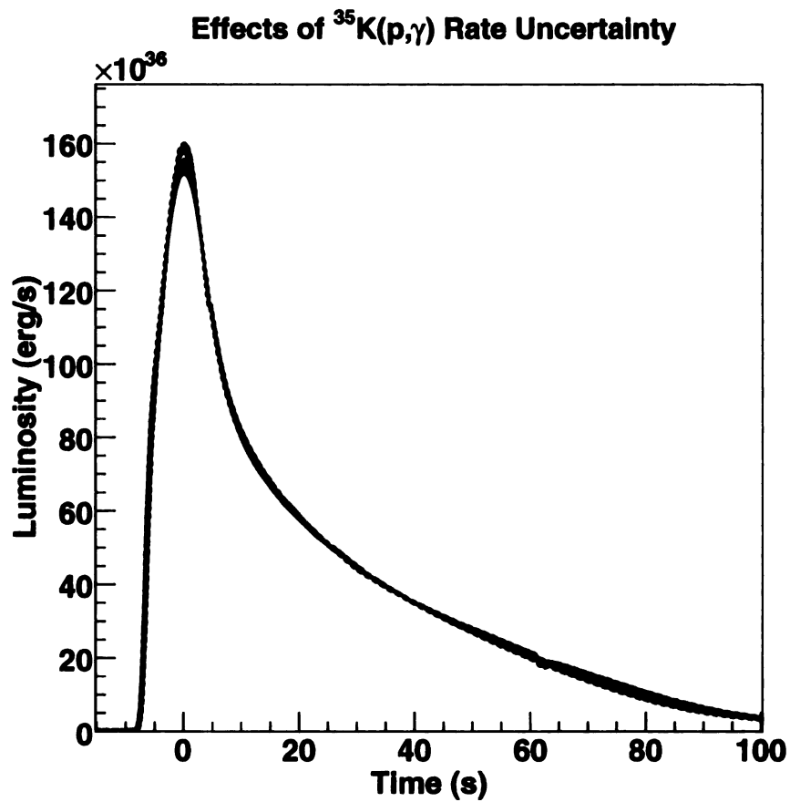
Figure 5.5: Multi-zone burst lightcurve 1\sigma confidence intervals are shown for an upper limit [green] and lower limit [red] ^{35}\text{K}(p,\gamma) rate.
