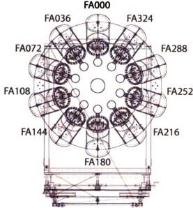
Figure 3.4: The SeGA detectors were arranged in classic configuration for this experiment with a total of 16 detectors, seven in the forward ring and nine in the 90° ring. The circle in the center of each diagram is the beam pipe. Just outside the beam pipe are the cylindrical germanium crystals of SeGA. The larger cylinders near the edge of each diagram are the liquid N 2 dewars. Shown in this diagram is the full complement of 18 detectors.
