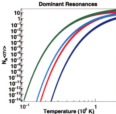
Figure 4.6: The new calculated reaction rate for ^{36}\text{K}(p,\gamma) based on the measurements in this work [green] plotted over the individual contributions to the total reaction rate due to the dominant resonances. Capture to the state at E_x = 3354 keV [magenta] (calculated assuming J^\pi = 3/2^+ ) is the greatest contribution at all burst temperatures. Other contributions shown are from E_x = 3530 keV [cyan], E_x = 3612 keV [red], and E_x = 3842 keV [blue] (all calculated assuming J^\pi = 3/2^+ ). The uncertainties shown by the bands are due to the uncertainty in the resonance energy.
