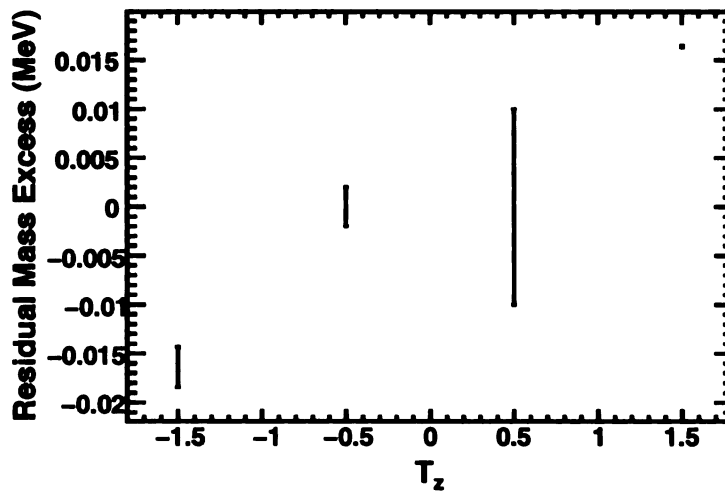
Figure 4.4: The residuals from an analytic determination of the quadratic terms of the IMME for the first excited state multiplet of A = 37 , T = 3/2 .
