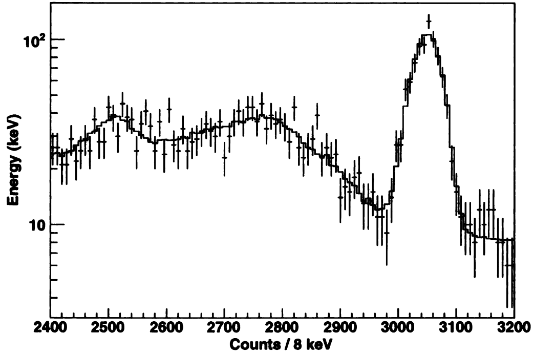
Figure 3.14: The data histogram from the 90° ring in SeGA is shown as points with errors and the fitted curve is the line. A fitted exponential background curve has been added to the simulated response function.
