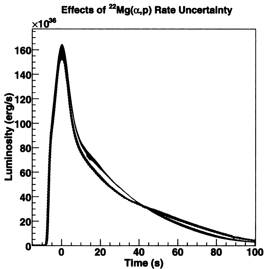
Figure 5.9: Multi-zone burst lightcurve 1\sigma confidence intervals are shown for an upper limit [green] and lower limit [red] ^{22}\text{Mg}(\alpha, p) rate.
