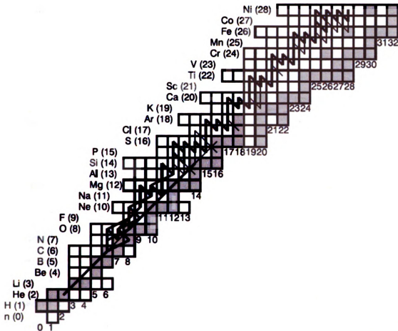
Figure 2.1: The rp -process begins with a fractional leakage from the CNO nuclei through \alpha -capture. Dominant pathways of the combined rp - and \alpha p -process are shown. Note the various possible bottlenecks and the bridging of certain \beta -decay paths by alternate ( \alpha, p ) reactions.
