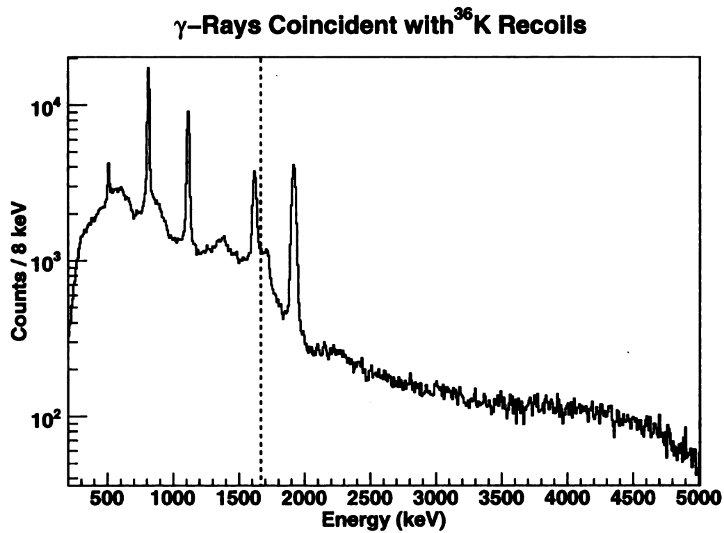
Figure 3.11: \gamma -rays observed in the 90^\circ ring of SeGA in coincidence with ^{36}\text{K} recoils in the S800 from incoming ^{37}\text{K} fragments. The proton separation energy is marked with the green dashed line.
