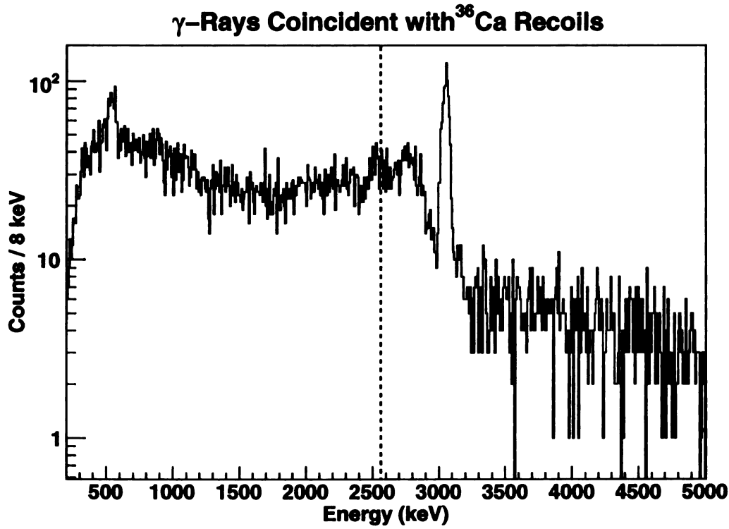
Figure 3.13: \gamma -rays observed in the 90^\circ ring of SeGA in coincidence with ^{36}\text{Ca} recoils in the S800 from incoming ^{38}\text{Ca} fragments. The proton separation energy is marked with the green dashed line.
