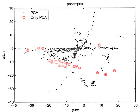
Figure 2.3. Pose variations in probe images and the pose values where matching succeeds at rank-one: red circles represent pose values where PCA succeeds.
