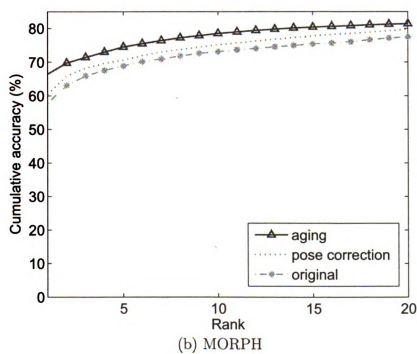
Figure 3.10. Cumulative Match Characteristic (CMC) curves showing the performance gain based on the proposed aging model.
