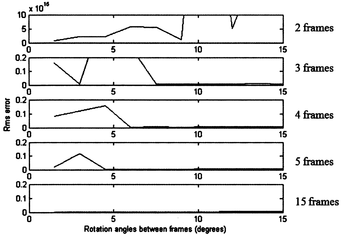
Figure 2.22. RMS error between the reconstructed and ideal rotation matrix, M_g .
