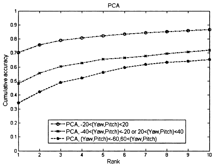
Figure 2.10. Cumulative matching scores using dynamic information (pose and motion blur) for PCA matcher.
