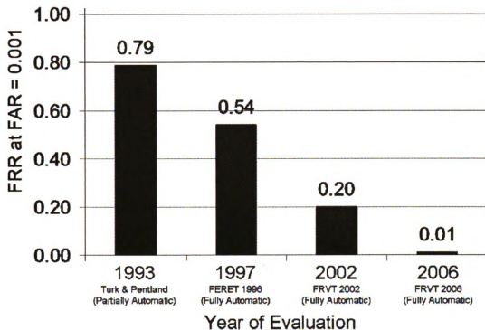
Figure 1.4. Reduction in face recognition error rates from 1993 to 2006 (Snapshot of computer screen) [92].
