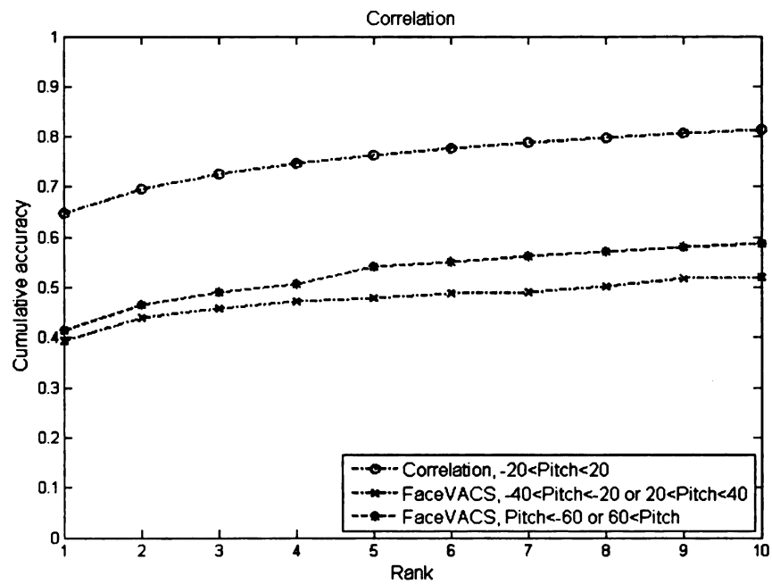
Figure 2.12. Cumulative Matching Characteristic curves with the effect of pitch for correlation matcher.
