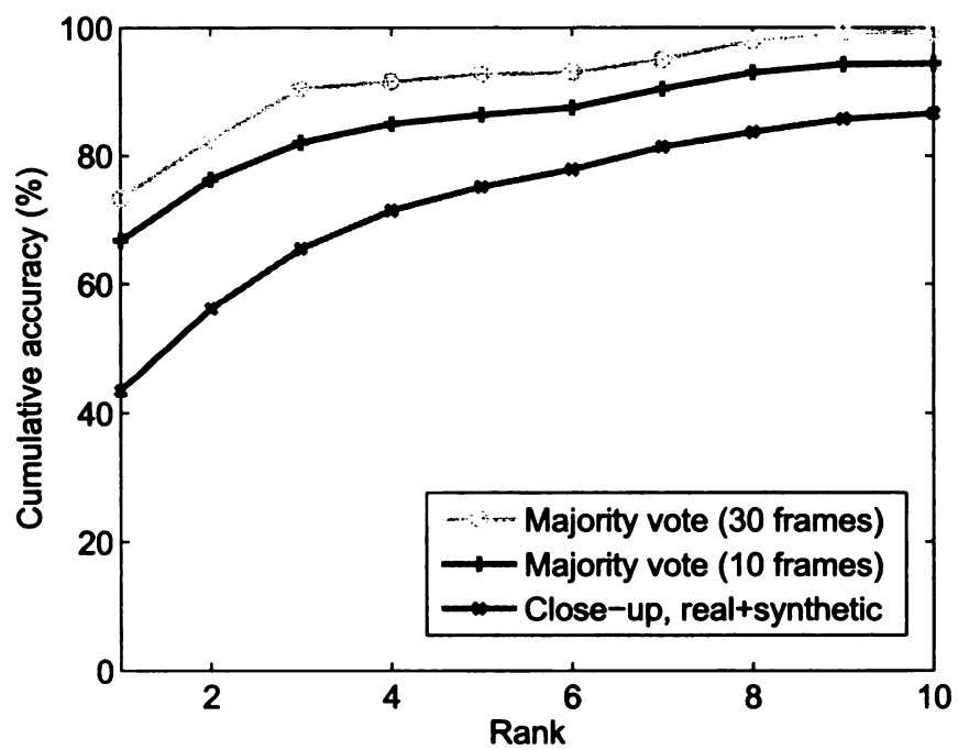
Figure 2.37. Face recognition performance using real and synthetic gallery images and multiple frames.
