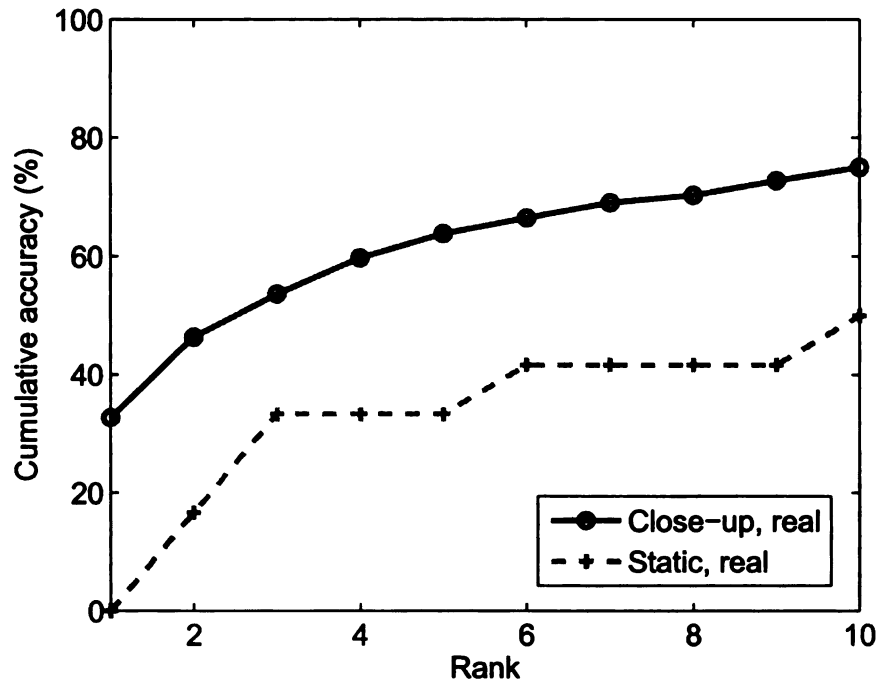
Figure 2.36. Face recognition performance with static and close-up views.
