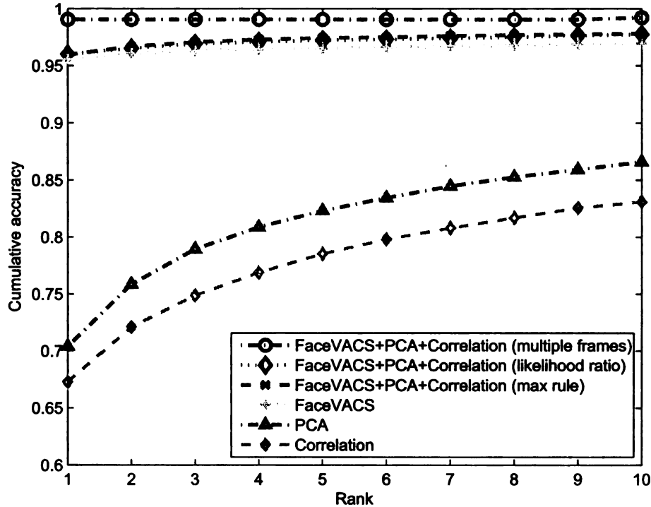
Figure 2.18. Cumulative matching scores by fusing multiple face matchers and multiple frames in near-frontal pose range ( -20^\circ \leq (\text{yaw} \ \& \ \text{pitch}) < 20^\circ ).
