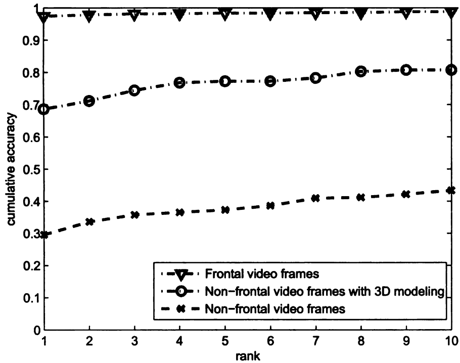
Figure 2.24. Face recognition performance with 3D face modeling.
