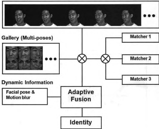
Figure 2.1. Schematic of the proposed face recognition system in video.
