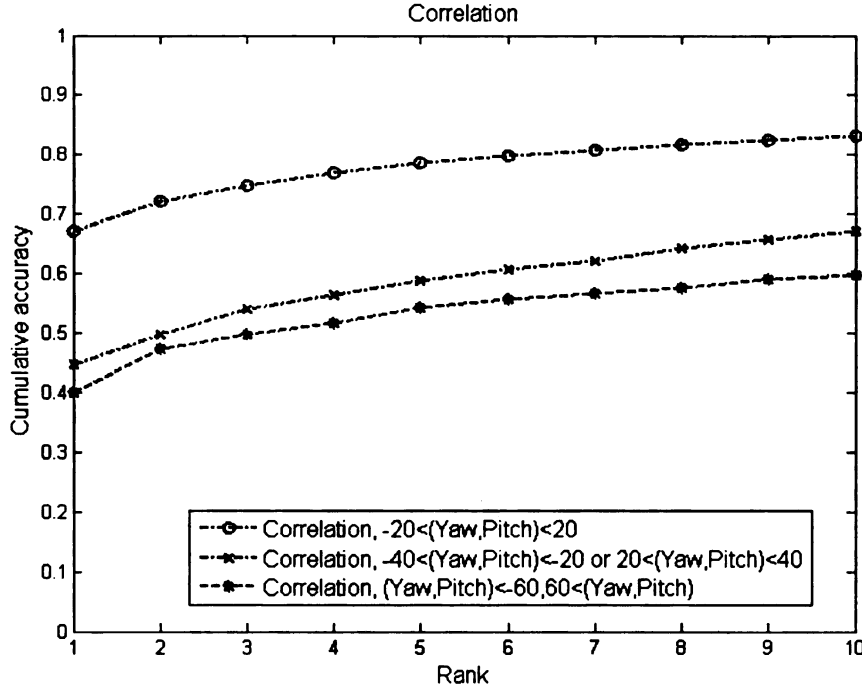
Figure 2.9. Cumulative matching scores using dynamic information (pose and motion blur) for Correlation matcher.
