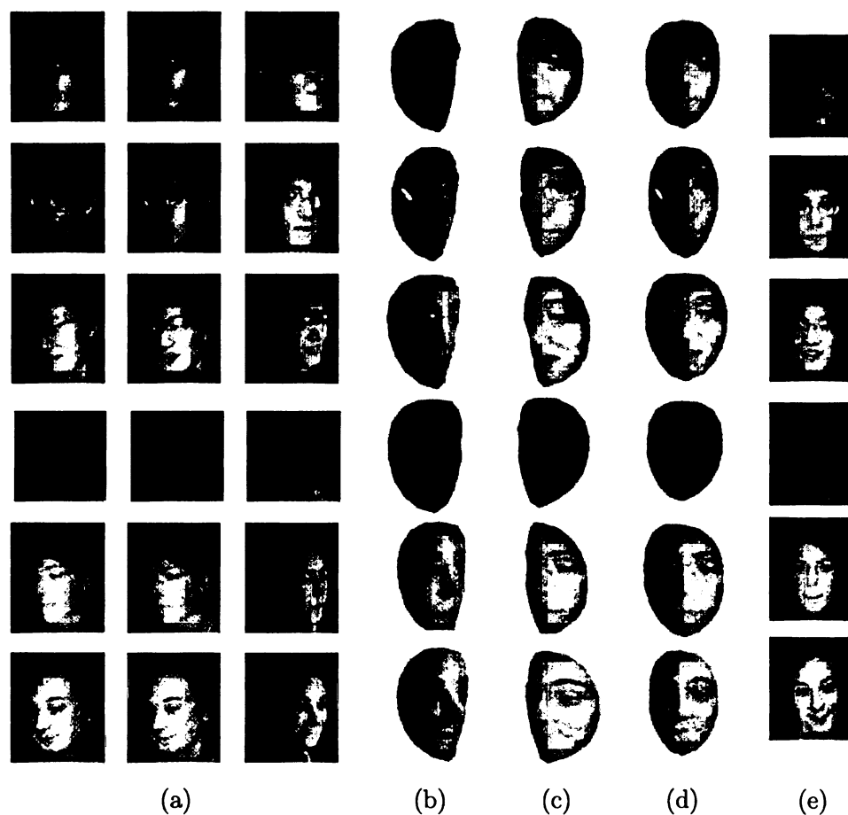
Figure 2.25. 3D model-based face recognition results on six subjects (Subject IDs in the FIA database are 47, 56, 85, 133, 198, and 208). (a) Input video frames; (b), (c) and (d) reconstructed 3D face models at right view, left view, and frontal view, respectively; (e) frontal images enrolled in the gallery database. All the frames in (a) are not correctly identified, while the synthetic frontal views in (d) obtained from the reconstructed 3D models are correctly identified for the first five subjects, and not for the last subject (#208). The reconstructed 3D model of the last subject appears very different from the gallery image, resulting in the recognition failure.
