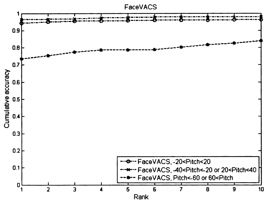
Figure 2.14. Cumulative Matching Characteristic curves with the effect of pitch for FaceVACS matcher.
