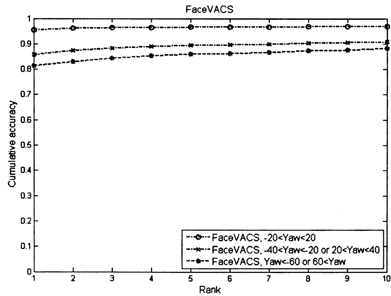
Figure 2.17. Cumulative Matching Characteristic curves with the effect of pitch for FaceVACS matcher.
