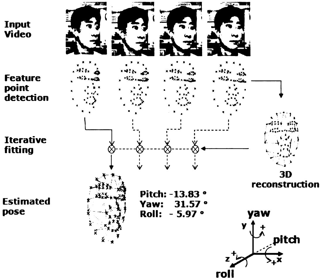
Figure 2.6. Pose estimation scheme.
