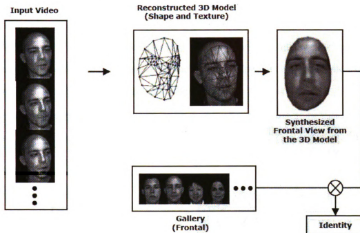
Figure 2.19. Proposed face recognition system with 3D model reconstruction and frontal view synthesis.
