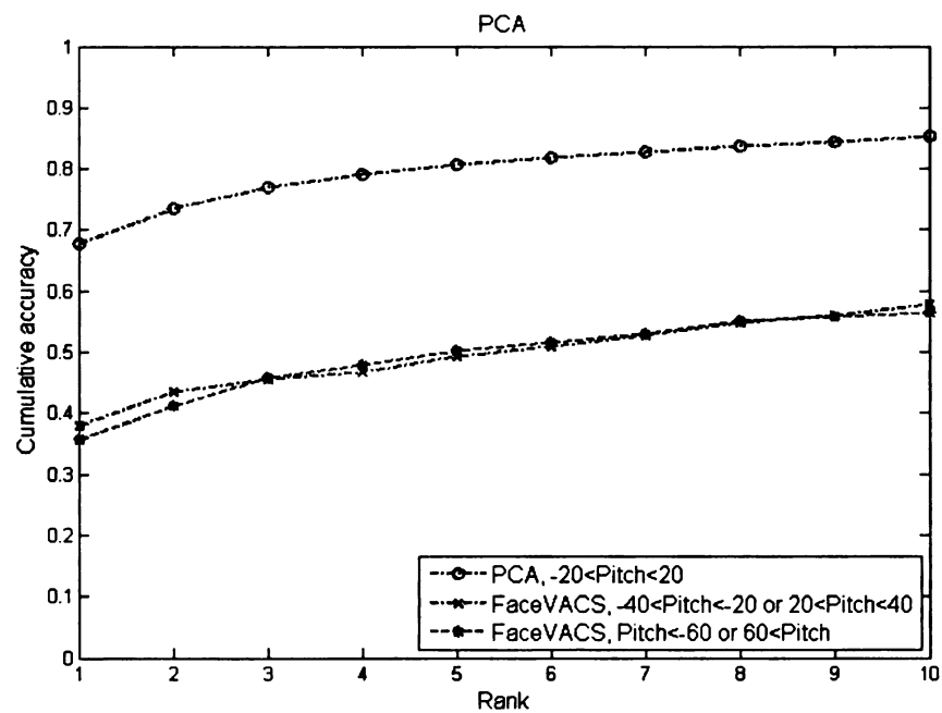
Figure 2.13. Cumulative Matching Characteristic curves with the effect of pitch for PCA matcher.
