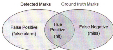
Figure 4.9. Schematic of the definitions of precision and recall.
