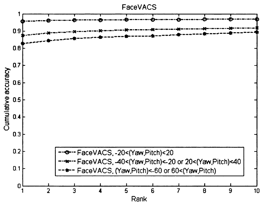
Figure 2.11. Cumulative matching scores using dynamic information (pose and motion blur) for FaceVACS matcher.
