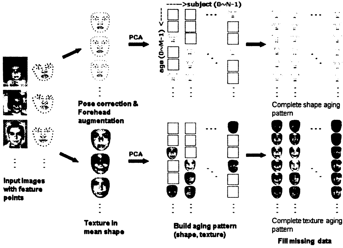
Figure 3.4. 3D aging model construction.
