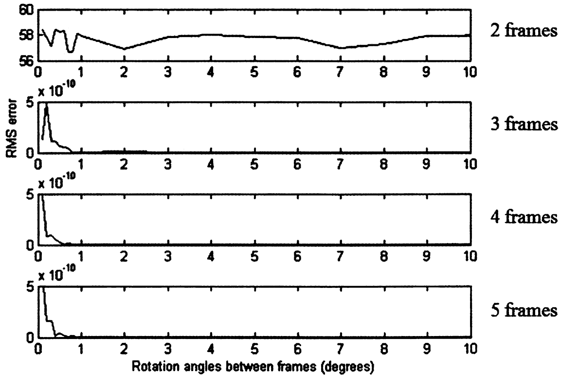
Figure 2.21. RMS error between the reconstructed shape and true model.
