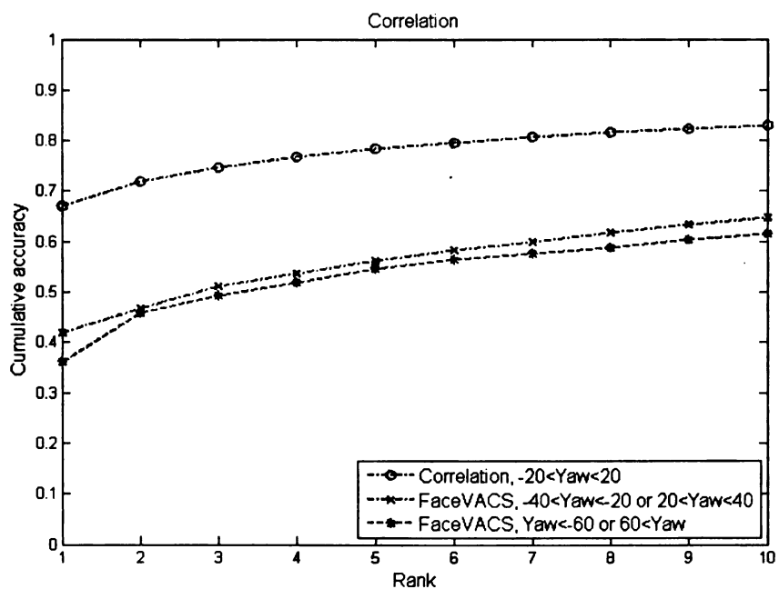
Figure 2.15. Cumulative Matching Characteristic curves with the effect of pitch for correlation matcher.
