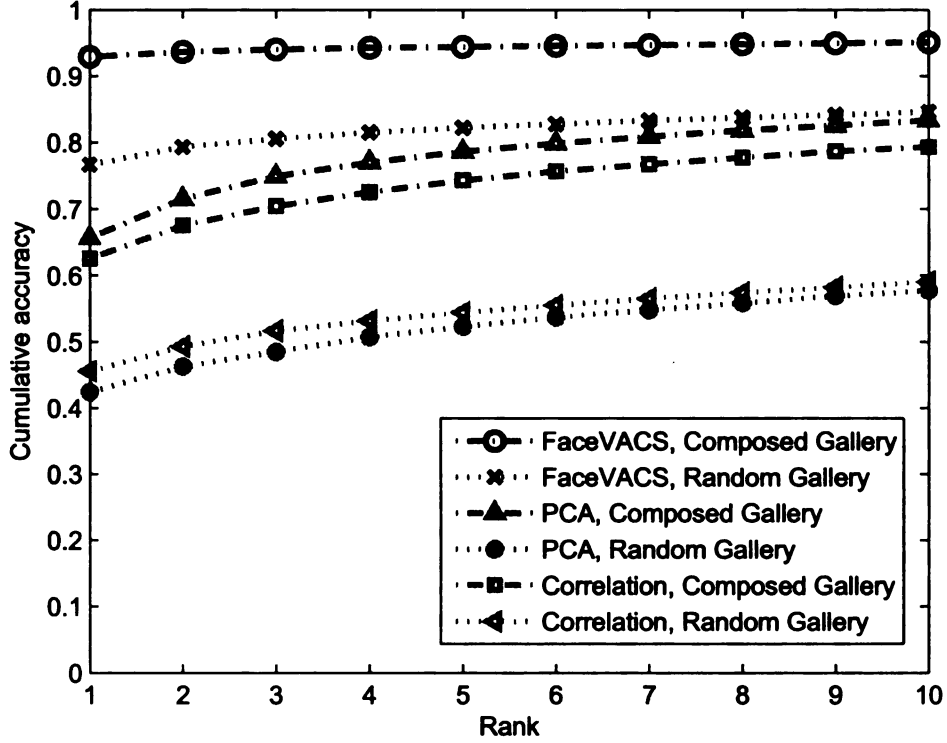
Figure 2.8. Face recognition performance on two different gallery data sets: (i) random gallery: random selection of pose and motion blur, (ii) composed gallery: frames selected based on specific pose and with no motion blur.
