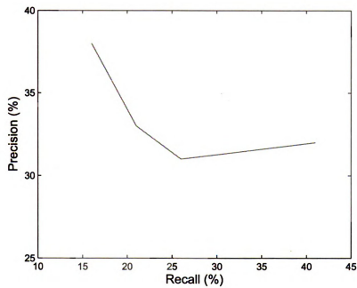
Figure 4.10. Precision and recall curve of the proposed facial mark detection method.
