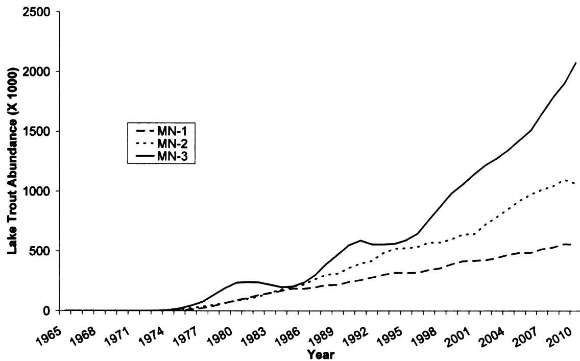
Figure 16. Model predicted wild lake trout population abundance (Ages 3-6).
