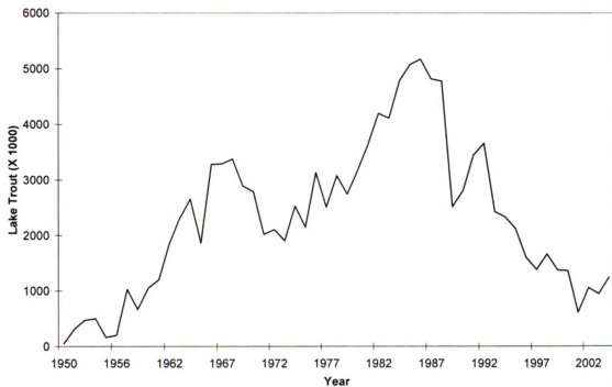
Figure 2. Number of lake trout stocked into Lake Superior.
