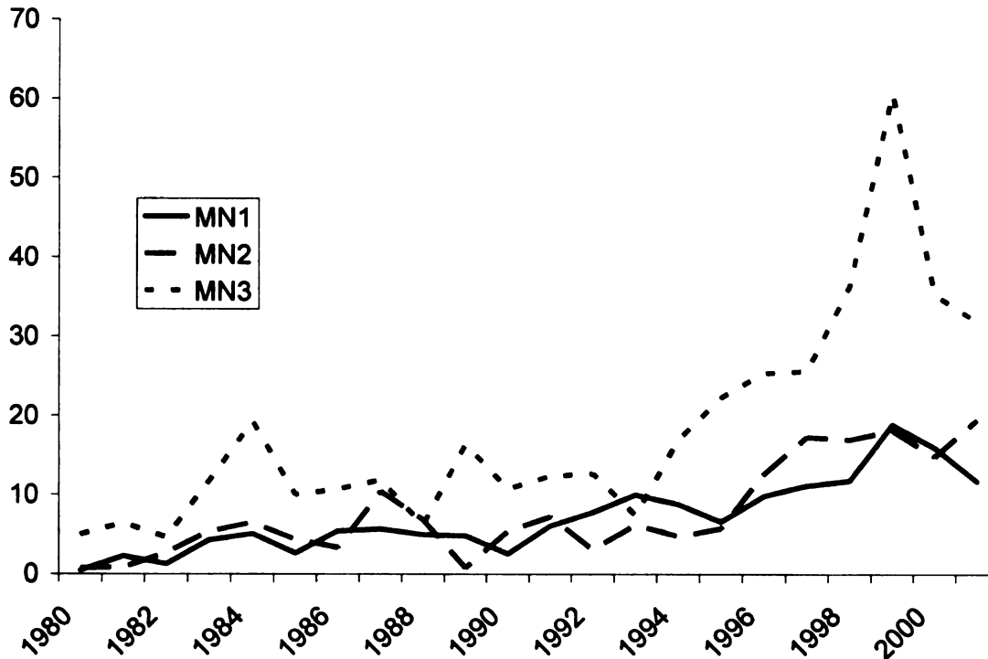
Figure 7. Smallmesh gillnet CPE of wild lake trout for management units in Minnesota waters of Lake Superior.
