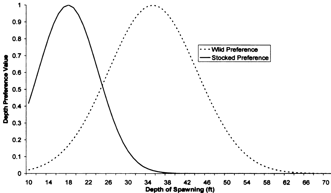
Figure 8. Depth factor of the habitat selection value of a potential spawning habitat. The curves were fit to data from the Keweenaw Peninsula area of Lake Superior (Ebener et al. 1990) with adjustments made to the wild distribution to account for the limited depth distribution of the data.
