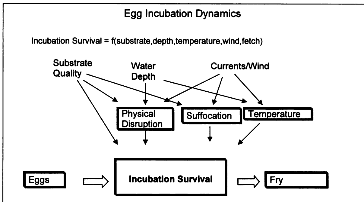
Figure 9. Schematic showing the physical factors affecting incubation survival and the interactions incorporated into the model.
