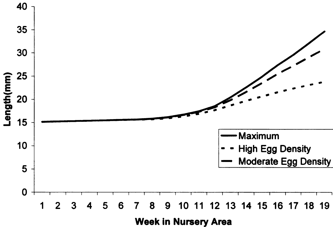
Figure 14. Projected length of lake trout fry in the nursery areas of MN-1. Maximum represents the growth level when fry are able to consume their maximum daily ration. High egg density assumes egg deposition rates of 500 eggs per meter squared, and moderate egg density is equivalent to the eggs produced by the entire Minnesota population from Negus (1995). Both scenarios assume all cobble and boulder substrates are used for spawning.
