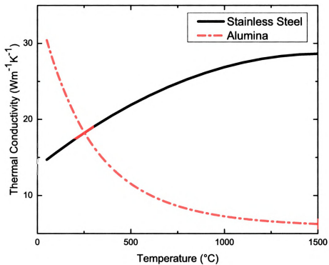
Figure 3.11: Comparison of the thermal conductivities of stainless steel [25] and alumina [26]. The advantage of using alumina for temperatures hotter than 250 °C is clear.
