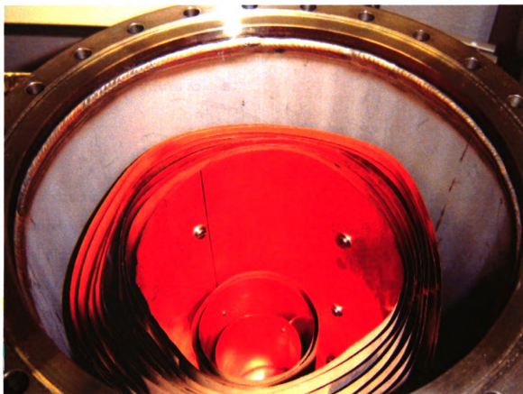
Figure 3.10: Copper thermal radiation shields placed within the vacuum vessel to reduce heat losses due to radiative heat transfer. The concentric circular assumption in modeling is an idealization.
