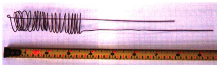
Figure 3.6: Heating element fabricated from tungsten wire using the mandrel shown in Figure 3.5. The wire used to fabricate the heating element pictured above was of diameter 7.62 \times 10^{-4} m (0.03").
