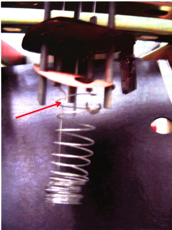
Figure 3.20: Photograph of the tungsten heating coil after the second test of the furnace. Sagging of the coil is seen, with accumulation of windings at the bottom due to gravity. The arrow shows the location of contact with the copper cylinder due to the sagging of the coil and distortion of the shape of the copper cylinder.
