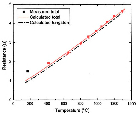
Figure 4.9: Measured total resistance and calculated total resistance for the electrical system during the test operation of the niobium sample heat treating furnace. The total resistance includes the tungsten coil resistance and the resistance of the wiring on the atmospheric side.
