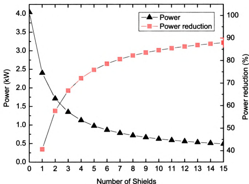
Figure 4.4: Estimated power consumption as a function of the number of radiation shields for the heat treatment furnace, for a hot-zone temperature of 1250 °C. Reduction of power consumption by the addition of each shield in comparison to the zero shields case is plotted on the right ordinate.
