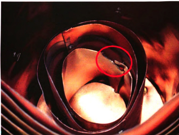
Figure 3.19: Close-up photograph of the hot-zone after the 1000 °C test. The location of contact of the tungsten heating coil with the distorted copper cylinder can be seen in the center.
