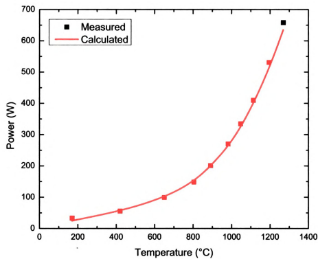
Figure 4.10: Measured and calculated power as a function of temperature for a test of the niobium sample heat treating furnace.
