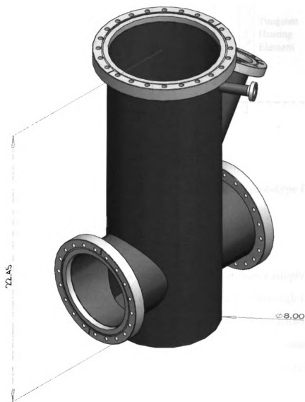
Figure 3.1: Steel vessel with pre-welded conflat flanges used for the furnace's vacuum vessel.
