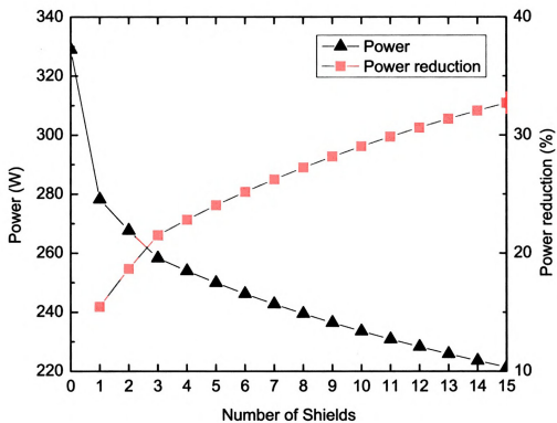
Figure 3.9: Estimated power consumption as a function of the number of radiation shields for the prototype furnace, for a hot-zone temperature of 1200 °C. Reduction of power consumption by the addition of each shield in comparison to the zero shields case is plotted on the right ordinate.
