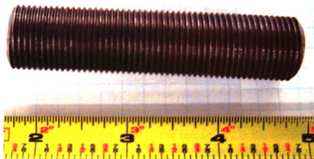
Figure 3.5: Custom fabricated stainless steel mandrel for winding tungsten wire into a coil of diameter 25.4 \times 10^{-3} m (1").
