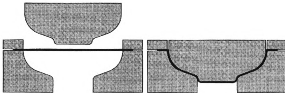
Figure 2.2: Deep drawing a niobium disk into a half cell [1].
