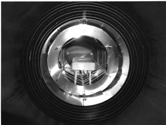
Figure 4.3: Photograph of the assembled molybdenum shields inside the vacuum vessel. The ceramic bed for placing niobium samples for heat treatment and the tungsten heating coil are also visible.
