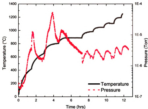
Figure 4.8: Temperature and pressure histories during a run of the furnace. Between hours 5 and 7 the furnace is set to maintain 890 °C for a soak, that is, to allow volatile components to be pumped out, causing the pressure to drop. Subsequent increases in temperature are met with small transient pressure changes.
