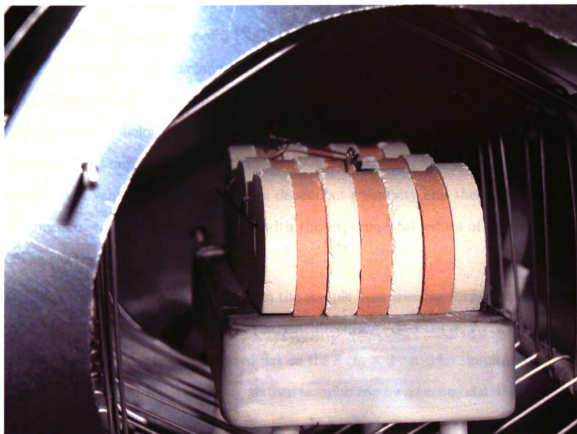
Figure 4.11: Photograph of the three rows of TempTabs used to verify the thermocouple measurements, and to check the temperature distribution within the hot zone of the niobium sample heat treating furnace. Each row contains seven TempTabs, alternating between TempTab 600 ( 1100\text{ }^{\circ}\text{C} - 1300\text{ }^{\circ}\text{C} ) and TempTab 300 ( 800\text{ }^{\circ}\text{C} - 1150\text{ }^{\circ}\text{C} ). The three rows span the length of the ceramic sample bed, and each row spans the width of the bed.
