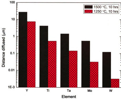
Figure 3.3: Estimated diffusion of select refractory metals into niobium at 1500 °C and 1250 °C, in comparison yttrium and titanium.
