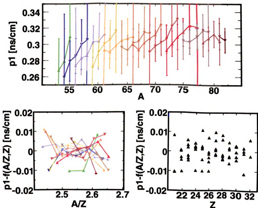
Figure 4.6: Fit for the slope ( p_1 ) of a TOF momentum correction function linear in x_{\text{mcp}} . The top plot shows the slope of fits to the spectra of individual isotopes as a function of their mass ( A ). The lower plots show the residuals of the parameterization of these slopes by the equation 4.6. The error of each data point, only shown in the first frame, was calculated from the statistics of each isotope (Equation 4.9).
