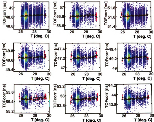
Figure 4.24: For a few isotopes the momentum corrected TOF_{corr} is shown as a function of the temperature in the S800 experimental vault. The observed correlation is of the order of 10 \text{ ps}/^\circ\text{C} for the direct TOF measurement, and about 5 \text{ ps}/^\circ\text{C} for the TOF measured with respect to a clock.
