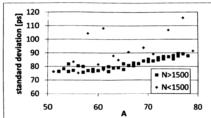
Figure 4.31: Fit results for the standard deviation of a Gaussian fit to the TOF distribution. For the isotopes with a small number of events ( N ) the width of the Gaussian function was set as a fixed fit parameter, estimating the value from the fit results of isotopes with large statistics.
