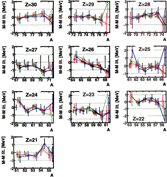
Figure 4.41: Sensitivity of the mass results to walk in the timing electronics. The mass calibration was fit using TOF corrected by t_{\text{SUSD}} and t_{\text{XDSD}} , and with different cuts in the integrated charge spectra of the PMTs (it was refitted in each case). The red circles are the mass residuals for the fit to the TOF values determined using all events, the green squares to events with a small signal from the S800 Down PMT, and the blue triangles for a large signal in the XFP Down PMT. The masses for each isotopic chain are plotted with respect to the literature data (black error bars around the zero axis), using extrapolations in [4] when they are unknown.
