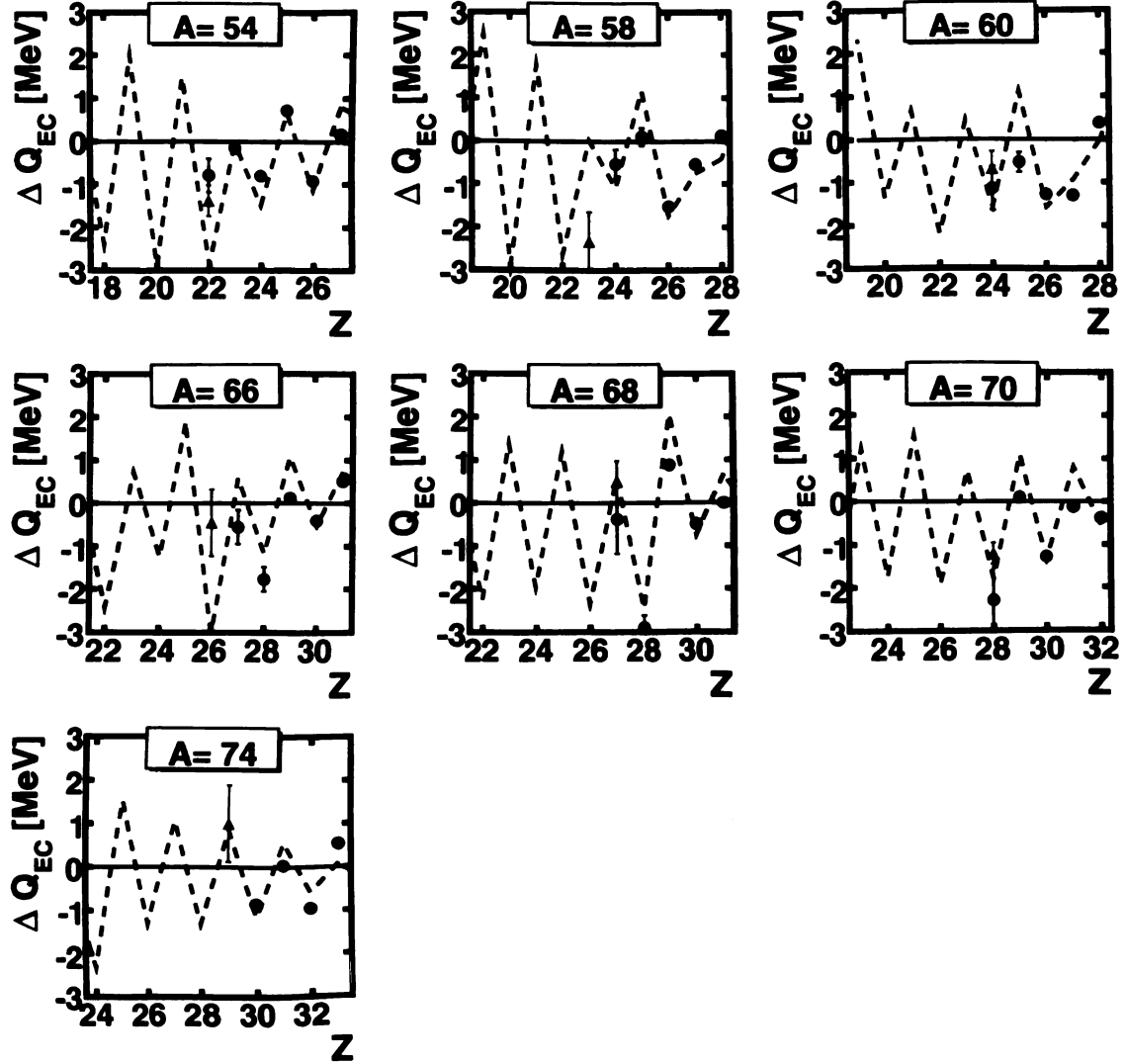
Figure 5.3: Electron capture Q-values for even A isobaric chains determined with the masses measured in this experiment. The Q-values are shown with respect to those calculated with the HFB-14 mass model ( \Delta Q_{EC} = Q_{EC}(i) - Q_{EC}(\text{HFB} - 14) ). The blue circles correspond to values calculated with the literature masses, the red triangles are calculated with the results of the present experiment. In addition, the dashed line shows the results for the FRDM model.
