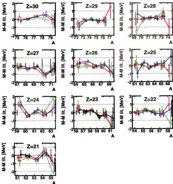
Figure 4.42: Sensitivity of the mass results to walk in the timing electronics. The mass calibration was fit using TOF corrected only by the particles momentum, and with different cuts in the integrated charge spectra of the PMTs (it was refitted in each case). The red circles are the mass residuals for the fit to the TOF values determined using all events, the green squares to events with a large signal from the S800 Down PMT, and the blue triangles for a low signal in the XFP Down PMT. The masses for each isotopic chain are plotted with respect to the literature data (black error bars around the zero axis), using extrapolations in [4] when they are unknown.
