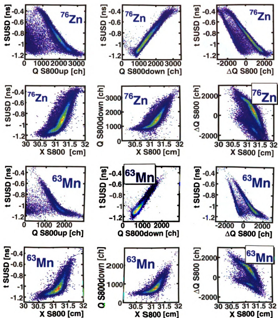
Figure 4.10: Correlations between signal amplitude from the S800 PMTs with the timing between both PMTs and the x_{\text{S800}} position for ^{76}\text{Zn} (Z=30) and ^{63}\text{Mn} (Z=25) events. The difference between both signal amplitudes is also shown ( \Delta Q_{\text{S800}} = Q_{\text{S800up}} - Q_{\text{S800down}} ).
