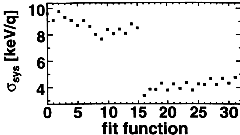
Figure 4.35: Systematic error that normalizes the \chi^2 of the fit using different polynomials as the calibration function. All functions include terms in t , t^2 , z , and z^2 , and all possible combinations of terms up to third order were tried. The additional terms can be read from the binary representation of the function ID, where each bit represents a term in the following order (z^3)(tz^2)(zt^2)(t^3)(tz) . For example, in the function 0 = 00000_2 no additional terms were included, and in 31 = 11111_2 all terms were included. The calibration function used in this experiment (4.22) corresponds to ID 16 = 10000_2 , and all other parameterizations from 17 to 31 also include the z^3 term, which clearly has the largest effect in improving the fit.
