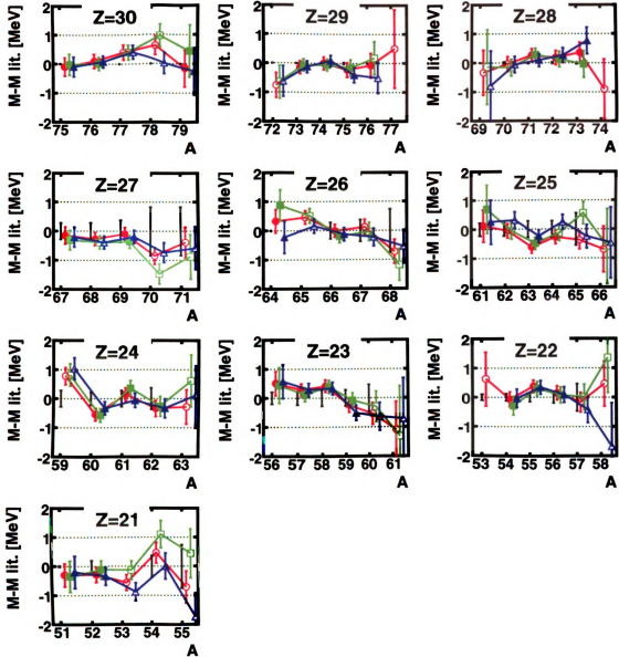
Figure 4.44: Sensitivity of the mass results to a_{S800} distribution. The mass calibration function was fitted to a set of TOF values corrected with a function quadratic in B\rho , and with different cuts in the spectrum for the dispersive angle at the S800 focal plane (it was refitted in each case). The red circles are the mass residuals for the fit to the TOF values determined using all events, the green squares to events with a negative a_{S800} angle, and the blue triangles for with a positive one. The masses for each isotopic chain are plotted with respect to the literature data (black error bars around the zero axis), using extrapolations in [4] when they are unknown.
