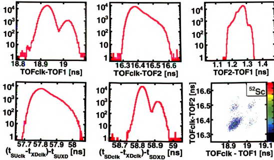
Figure 4.29: Comparison of semi-independent time-of-flight measurements (equation 4.13). About 10 % of the events are shifted by 90 ps by a glitch that was traced to the electronic logic modules that multiply the signals from the S800 timing detectors. The two dimensional spectra only shows events of one isotope ( ^{52}\text{Sc} ).
