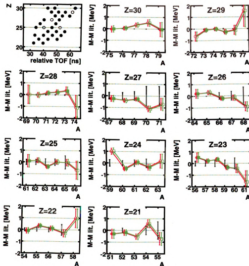
Figure 4.52: Mass fit excluding calibration isotopes with known long-lived isomer with energy below 200 keV (Table 4.2). The first figure shows the location of the reference masses in the coordinate space of the calibration function. The open circles are the isotopes excluded in the second fit. The mass residuals shown as red circles correspond to the fit when the four isotopes with known isomers are used as calibration points, and the ones shown as green squares are those for the fit when only isotopes without known long-lived isomers are used. In these mass residual plots filled symbols correspond to isotopes used as calibration points. The masses for each isotopic chain are plotted with respect to the literature data (black error bars around the zero axis), using extrapolations in [4] when they are unknown.
