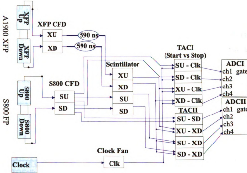
Figure 4.28: Electronics diagram for the timing subsystem.
