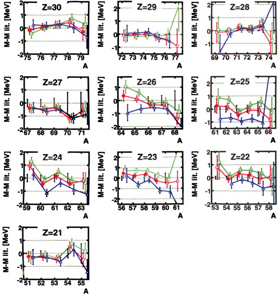
Figure 4.39: Sensitivity of the mass results to timing walk correction. The mass calibration function was fitted to a set of TOF values corrected by t_{\text{SUSD}} and t_{\text{XDSD}} , and the fit residuals are shown as red circles. The masses were then evaluated for sets of corrected TOF values that were determined with events with a small (green squares) or large (blue triangles) integrated charge values for the S800 Down PMT. The masses for each isotopic chain are plotted with respect to the literature data (black error bars around the zero axis), using extrapolations in [4] when they are unknown.
