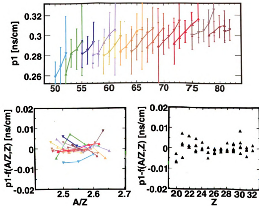
Figure 4.7: Fit for the slope ( p_1 ) of a TOF momentum correction function quadratic in x_{mcp} . The top plot shows the linear term of fits of fits to the spectra of individual isotopes as a function of their mass ( A ). The lower plots show the residuals of the parameterization of these slopes by the equation 4.7. The error of each data point, only shown in the first frame, was calculated from the statistics of each isotope (Equation 4.9).
