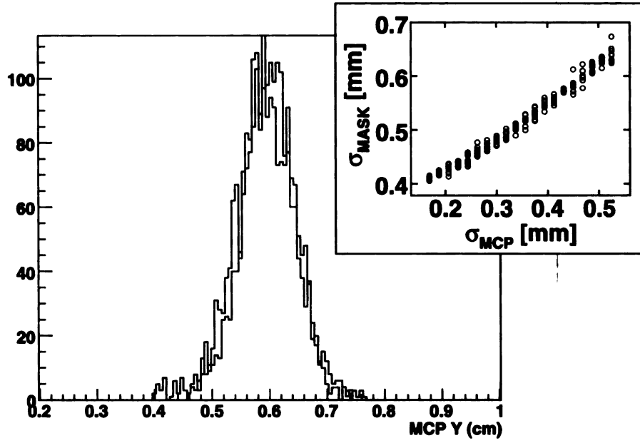
Figure 3.15: MCP position spectra for one of the mask holes ( radius = 0.75 mm) obtain during the calibration run. The experimental data (grey) is compared to a Monte Carlo simulation using a detector resolution of \sigma_{\text{mcp}} = 0.4 mm (black). The insert shows how the standard deviation of the simulated mask spectra ( \sigma_{\text{mask}} ) depends on the assumed detector resolution. The measured value of \sigma_{\text{mask}} during the calibration run is 0.45 mm.
