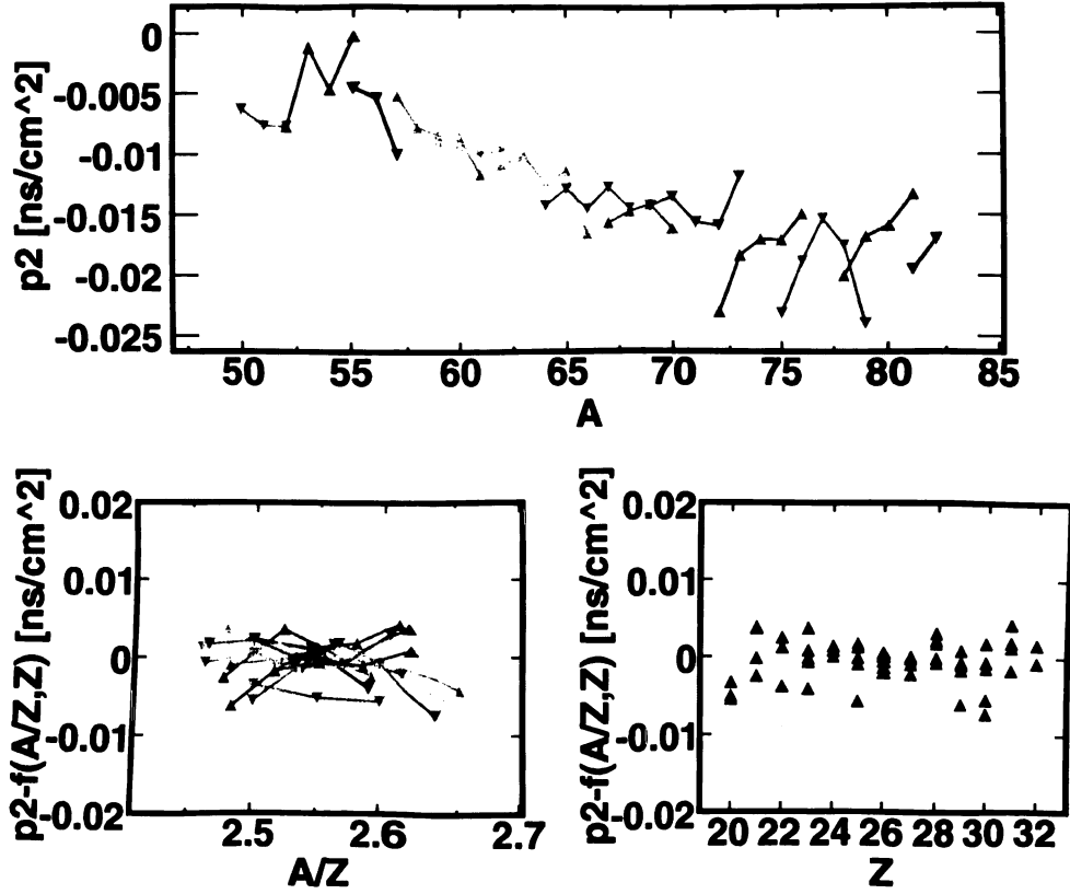
Figure 4.8: Fit for the quadratic term ( p_2 ) of a TOF momentum correction function quadratic in x_{\text{mcp}} . The top plot shows the quadratic term of fits of fits to the spectra of individual isotopes as a function of their mass ( A ). The lower plots show the residuals of the parameterization of these slopes by the equation 4.8. The weight given to each data point in the fit is the same as the one shown in Figure 4.7.
