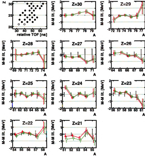
Figure 4.50: Mass fit excluding calibration isotopes with Z=21 . The first figure shows the location of the reference masses in the coordinate space of the calibration function. The open circles are the isotopes excluded in the second fit. The mass residuals shown as red circles correspond to the fit with all reference masses, and the ones shown as green squares are those for the reduced set of calibrants. In these mass residual plots filled symbols correspond to isotopes used as calibration points. The masses for each isotopic chain are plotted with respect to the literature data (black error bars around the zero axis), using extrapolations in [4] when they are unknown.
