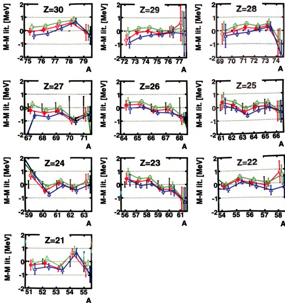
Figure 4.45: The mass calibration function was fitted to a set of TOFs obtained for events in the range of 26^{\circ}\text{C} \leq T \leq 28^{\circ}\text{C} for the S800 vault temperature (shown in red, with the reference masses indicated with filled circles). The TOFs obtained for other cuts in the S800 vault temperature spectra were evaluated using the results of this fit (without refitting the mass calibration function). The mass results when using more restrictive cut ( 26.5^{\circ}\text{C} \leq T \leq 27.5^{\circ}\text{C} ) are shown as blue triangles, and the results for no temperature cut as green squares. The mass along each isotopic chain is plotted with respect to the literature data (black error bars around the zero axis) using extrapolation in [4] when the mass is unknown.
