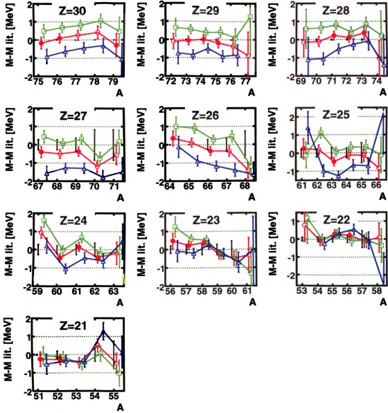
Figure 4.40: Sensitivity of the mass results to timing walk correction. The mass calibration function was fitted to a set of TOF values corrected by t_{\text{SUSD}} and t_{\text{XDSD}} , and the fit residuals are shown as red circles. The masses were then evaluated for sets of corrected TOF values that were determined with events with a small (green squares) or large (blue triangles) integrated charge values for the XFP Down PMT. The masses for each isotopic chain are plotted with respect to the literature data (black error bars around the zero axis), using extrapolations in [4] when they are unknown.
