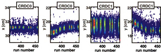
Figure 3.17: Position measurements at the S800 focal plane with the two cathode readout drift chambers (CRDCs). The calibration in the vertical position is sensitive to the pressure of the detector gas, and it was observed to drift during the experiment.
