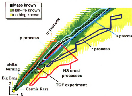
Figure 1.1: Knowledge of nuclear masses across the chart of the isotopes (data in the 2003 Atomic Mass Evaluation [4]). The region of the isotopes relevant for astrophysical calculations, and the region explored in the present time-of-flight experiment is also indicated.
