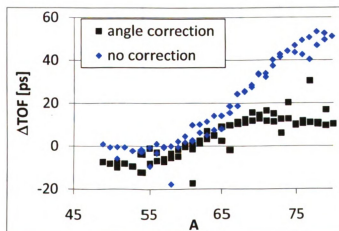
Figure 4.22: Difference in the TOF determined for events with a positive angle in the S800 focal plane versus those with negative angle. The difference is shown for the momentum corrected TOF_{corr} (light diamonds), and for the TOF_{corrA} of Equation 4.12, which is also corrected by the its dependence on the PMT signal's amplitude and the S800 angle (black squares).
