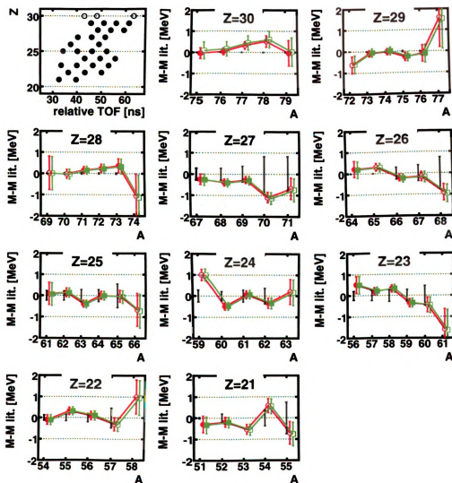
Figure 4.51: Mass fit excluding calibration isotopes with Z=30 . The first figure shows the location of the reference masses in the coordinate space of the calibration function. The open circles are the isotopes excluded in the second fit. The mass residuals shown as red circles correspond to the fit with all reference masses, and the ones shown as green squares are those for the reduced set of calibrants. In these mass residual plots filled symbols correspond to isotopes used as calibration points. The masses for each isotopic chain are plotted with respect to the literature data (black error bars around the zero axis), using extrapolations in [4] when they are unknown.
