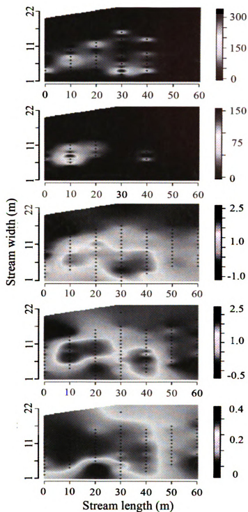
Figure 3.6. Interpolated surfaces of live eggs (time 1 and 2), random spatial effects ( w(s) time 1 and 2), and residual spatial correlation ( \rho t=1 , t=2 (s)) from model (3) for Site 4 (top to bottom). Points represent locations where there was at least one live egg in time 1.
