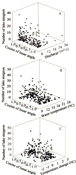
Figure 1.8. Relationship between daily numbers of lake sturgeon captured at spawning locations on the Upper Black River, Michigan and lunar angle with A) 24 hour lagged river discharge, B) 24 hour lagged water temperature and C) the magnitude and change in water temperature over the previous 48 hours.
