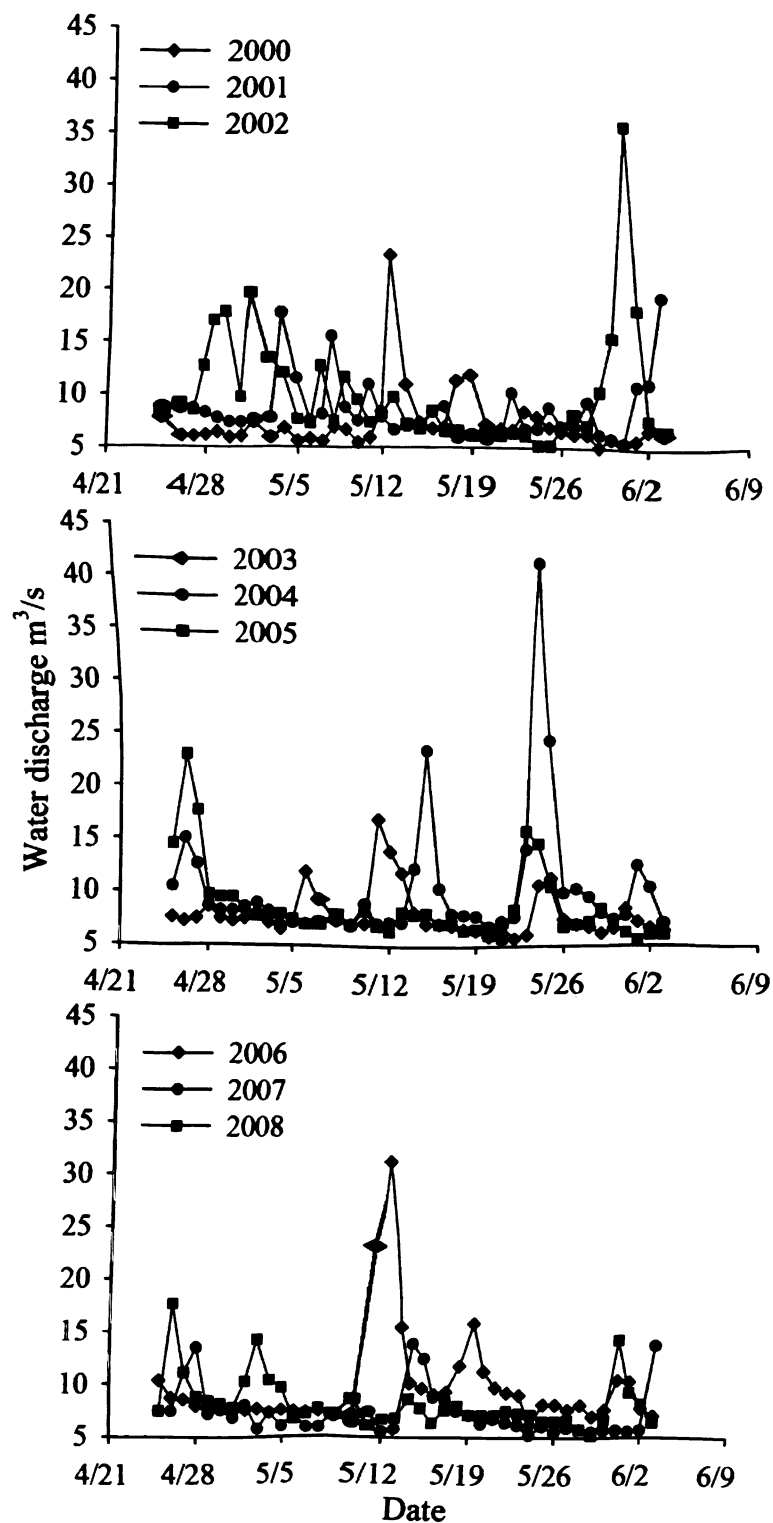
Figure 1.2. Measurements of daily river discharge ( \text{m}^3/\text{s} ) of the Upper Black River, Michigan collected from April 22 through June 5 for 2000-2002 (upper panel), for 2003-2005 (middle panel) and 2006-2008 (lower panel).
