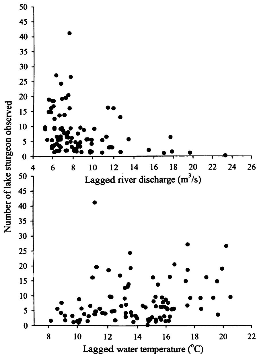
Figure 1.5. Relationship between the daily number of lake sturgeon observed entering the mouth of the Upper Black River, Michigan with 1 day lagged river discharge and 1 day lagged water temperature.
