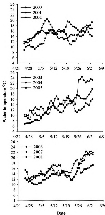
Figure 1.1. Measurements of daily water temperature ( ^{\circ}\text{C} ) of the Upper Black River, Michigan collected from April 22 through June 5 for 2000-2002 (upper panel), for 2003-2005 (middle panel) and 2006-2008 (lower panel).
