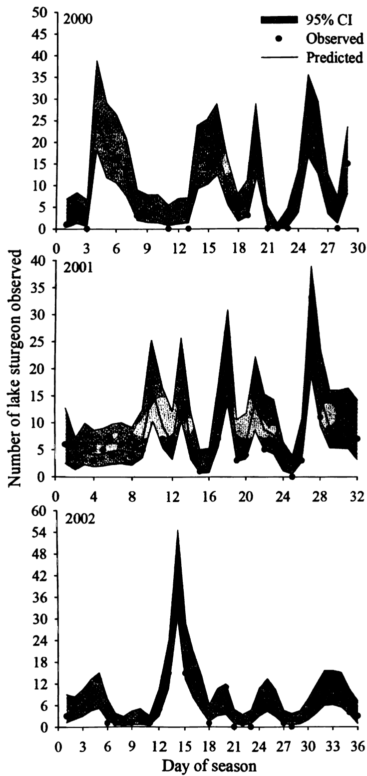
Figure 1.4. Observed, predicted and 95% confidence intervals for the daily number of lake sturgeon entering the Upper Black River, MI from 2000-2002.
