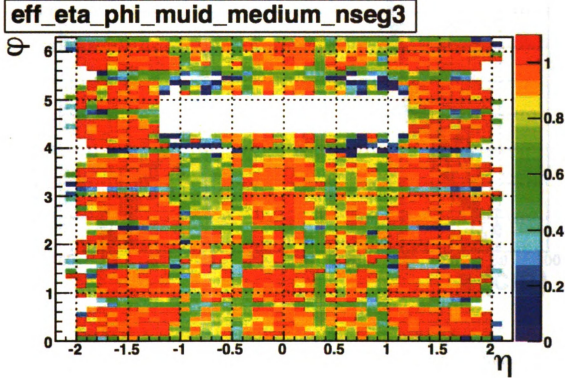
Figure 6.4: Combination \mu efficiency for local muon system, cosmic veto, and track match. The hole is due to supports for the calorimeter preventing placement of muon chambers. Figure taken from [22].
