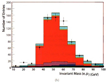
Figure 7.14: \mu e final state checking histograms: transverse mass ( e, \vec{E}_T ), invariant mass ( e, \mu ).
