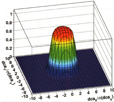
Figure 4.3: Values for the weighting function of a given track to its contribution to a particular primary vertex given a fixed \chi^2 and various impact parameter resolutions of the track-vertex system [18].
