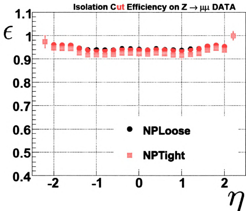
Figure 6.6: \mu isolation efficiency for NPTight isolation requirement. Figure taken from [22].
