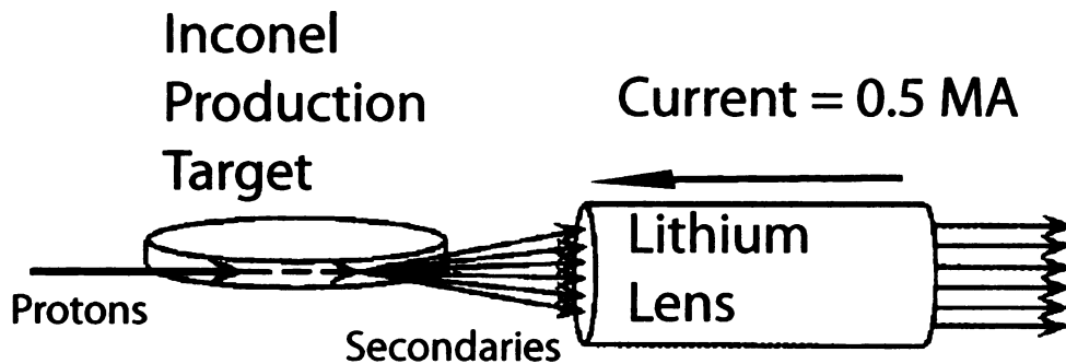
Figure 3.7: A figure showing the \bar{p} target and the lithium lens used to select antiprotons at 8 GeV [7].
