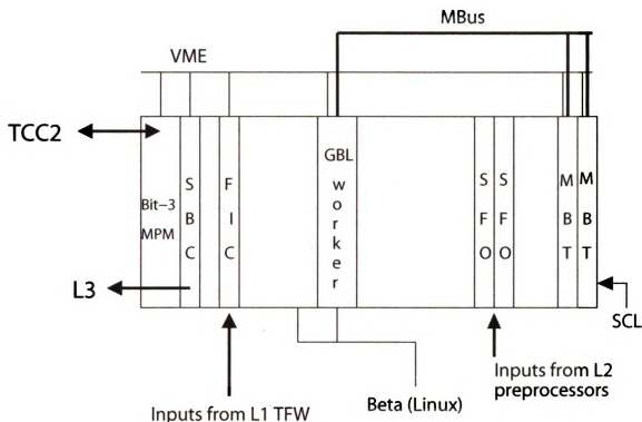
Figure A.3: Physical setup of the L2 Global cards within its VME crate.
