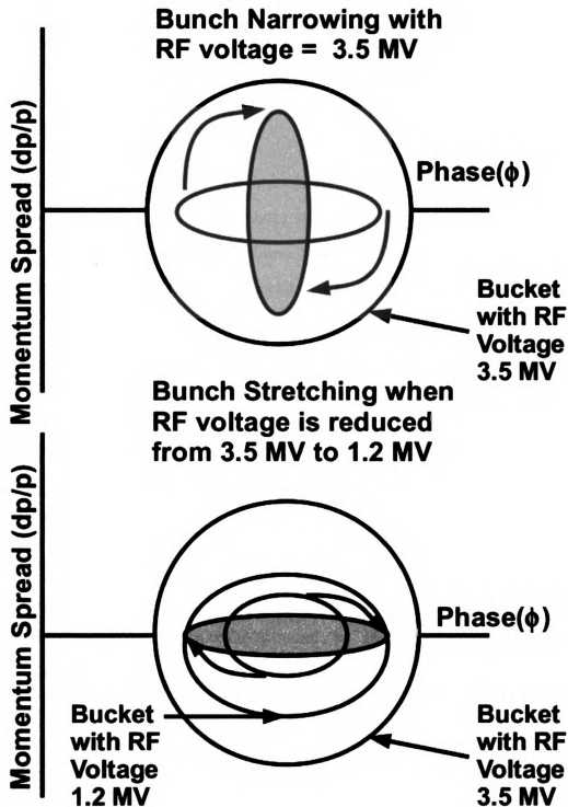
Figure 3.8: This shows the process of bunch rotation. The phase of individual particles is sacrificed to get a more consistent momentum in the beam [10].
