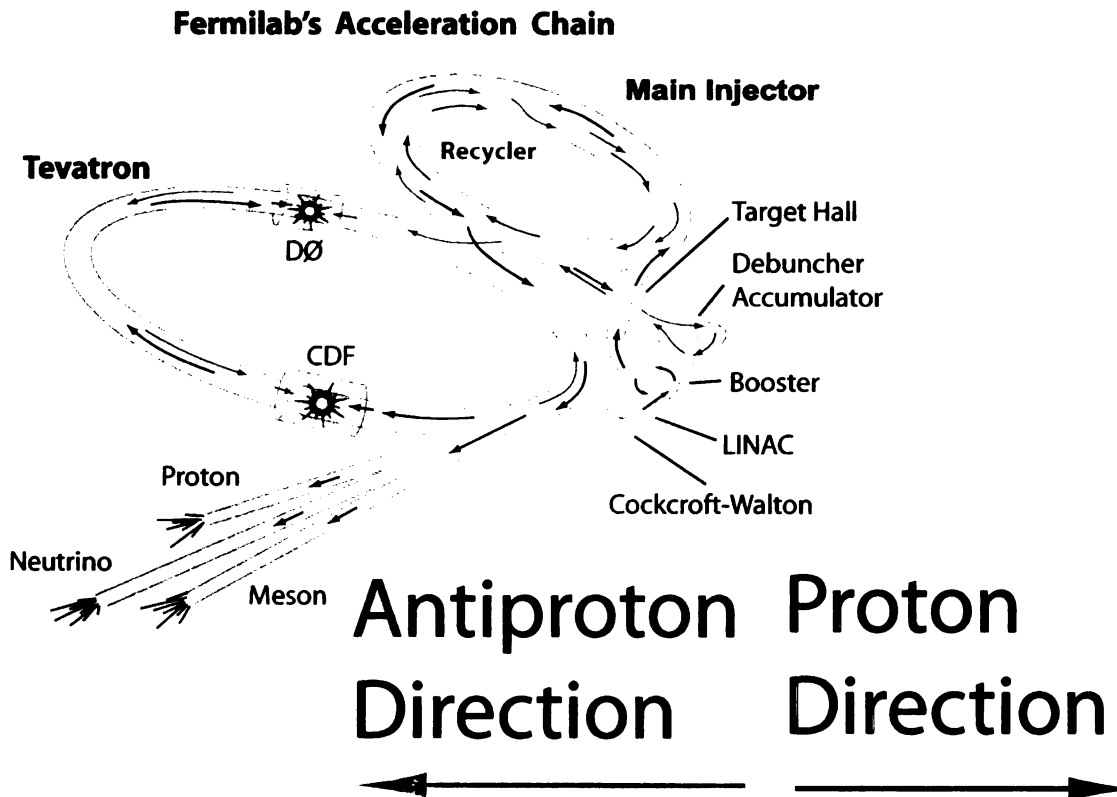
Figure 3.1: The Fermilab accelerator chain [6].
