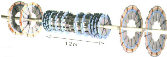
Figure 3.16: The layout of the silicon microstrip detector [13].
