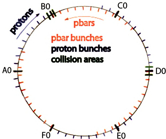
Figure 3.11: The Tevatron bunch structure. Collisions happen every 396 ns within a superbunch. There are three “Trains” of twelve bunches with an abort gap between “Trains” of 2.617 \mu s [12].
