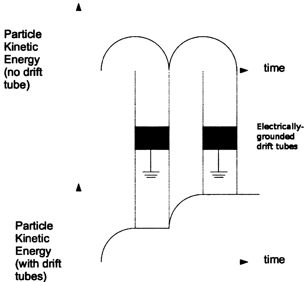
Figure 3.4: The energy of particles as they travel through the DTL [8].
