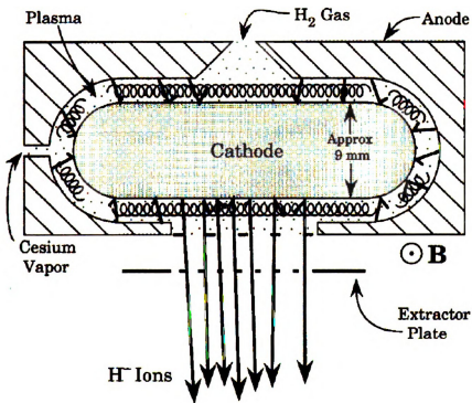
Figure 3.2: The Magnetron: Creating H^- [7].
