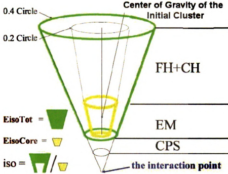
Figure 4.4: The isolation of EM objects is determined by looking at the fraction of total energy in a cone of R < 0.4 minus the amount of energy in the EM calorimeter in a cone of R < 0.2 normalized to the EM energy. The CPS is the central preshower detector [19].
