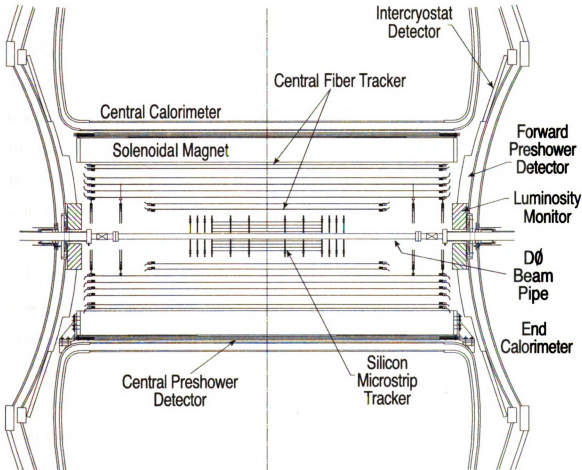
Figure 3.15: The inner tracking system showing the SMT, CFT, the solenoidal magnet and preshower detectors [13].
