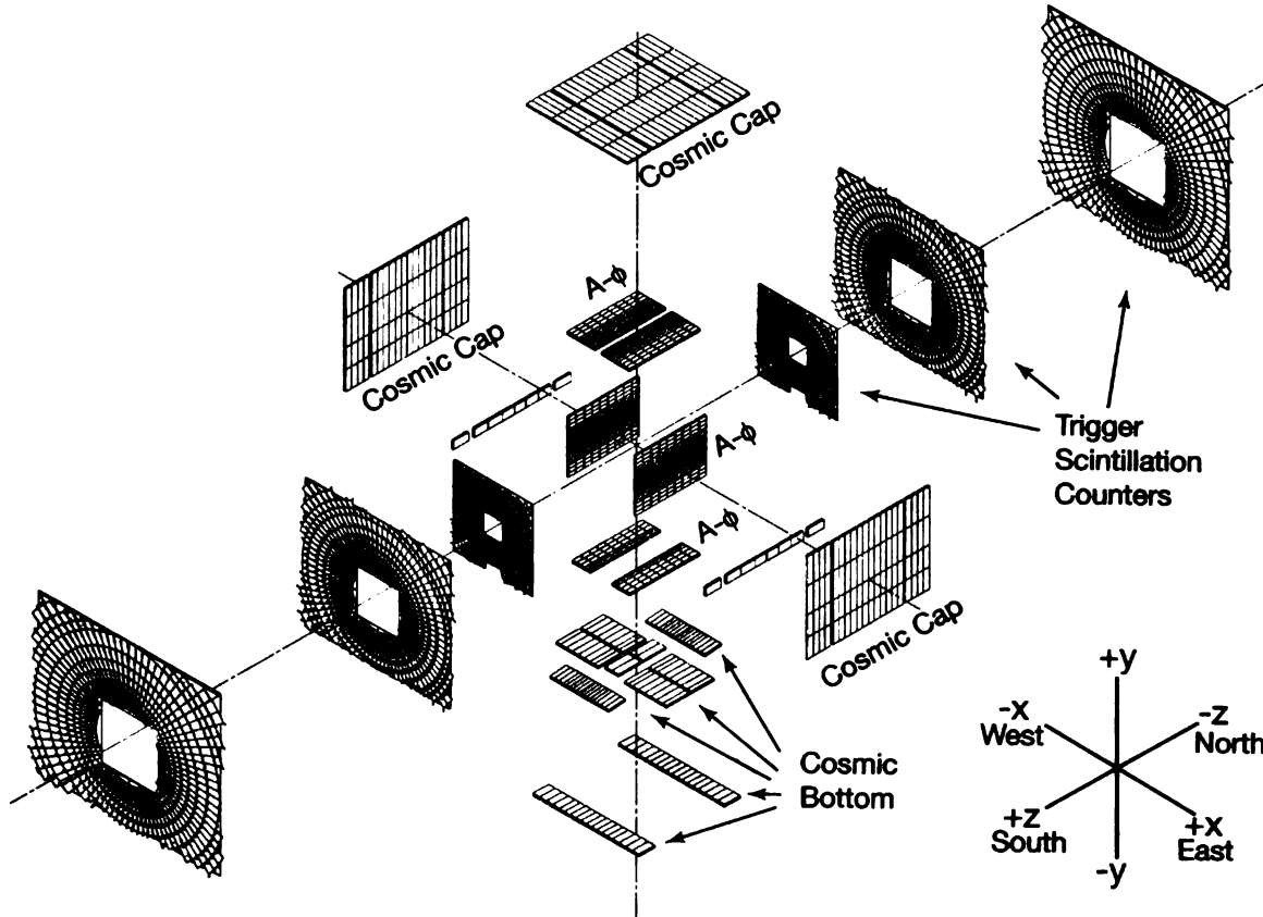
Figure 3.28: The layout of the scintillators used in the DØ muon system [13].
