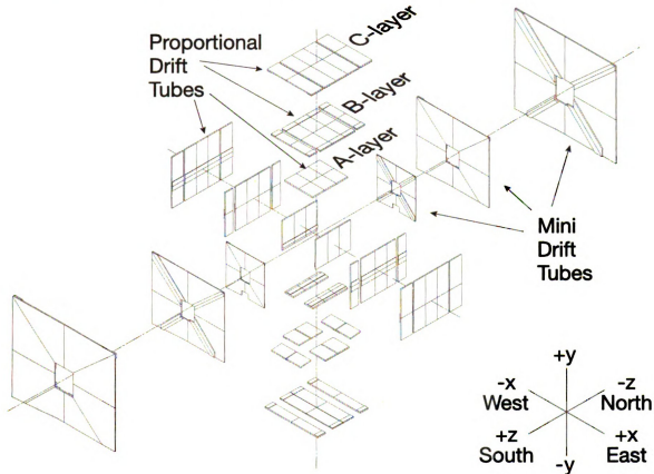
Figure 3.27: The layout of the wire chambers used in the DØ muon system [13].
