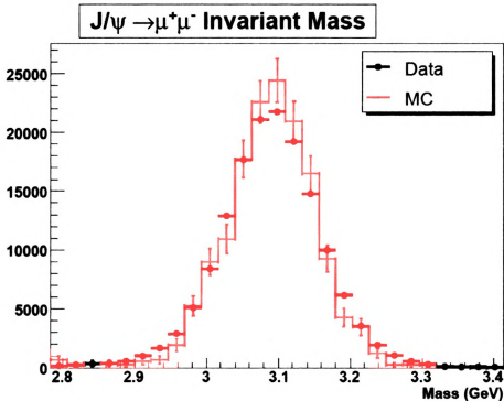
Figure 6.1: The J/\psi peak before applying muon smearing [3].
