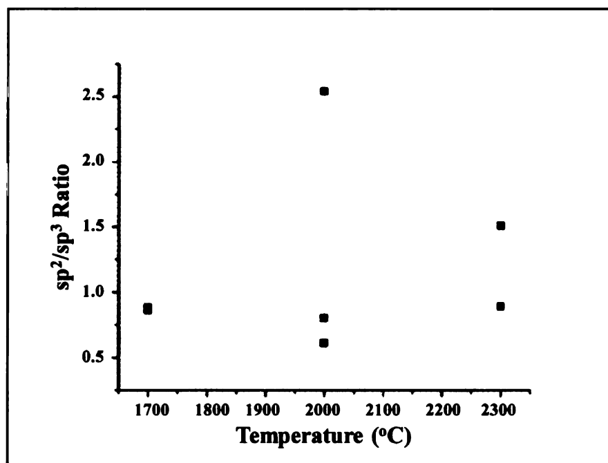
Figure 5.10 A plot of the sp^2/sp^3 ratio in carbon onions as a function of synthesis temperature. The plot is based on results obtained using approach 2.
