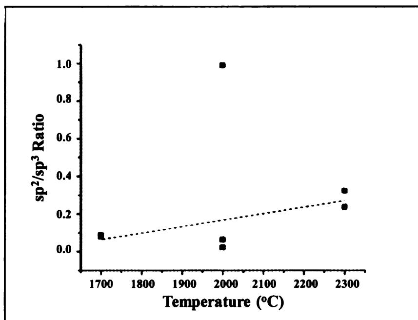
Figure 5.13 A plot showing an increase in the sp^2/sp^3 ratio in carbon onions as a function of synthesis temperature. The results from the 2000°C were variable due to synthesis uniformity issues.
