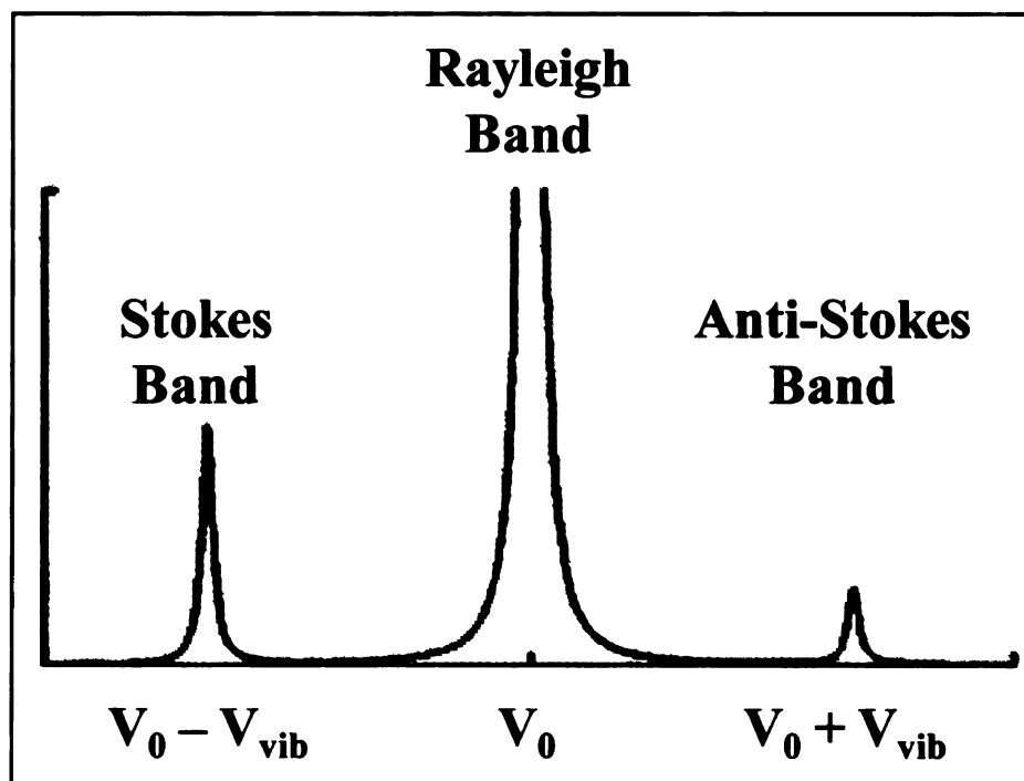
Figure 2.9 A schematic Raman scattering spectrum showing Rayleigh line, Stokes scattering, and anti-Stokes scattering 7 .
