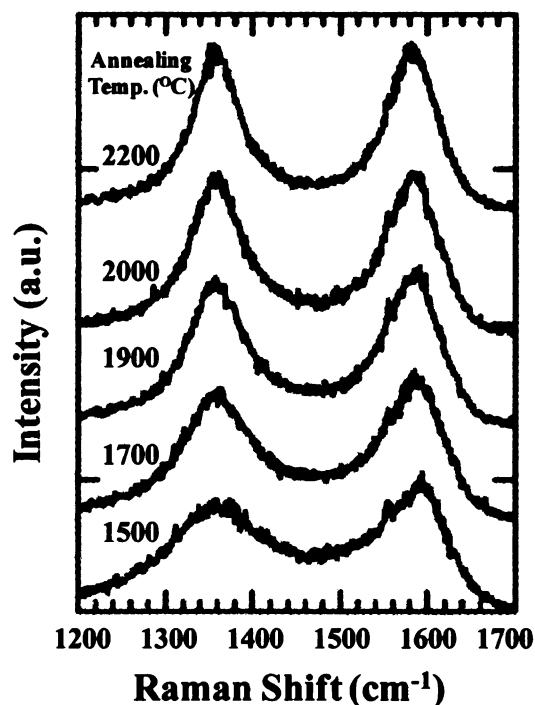
Figure 1.3 Raman spectra of carbon onion samples prepared at increasing synthesis temperature 20 .
