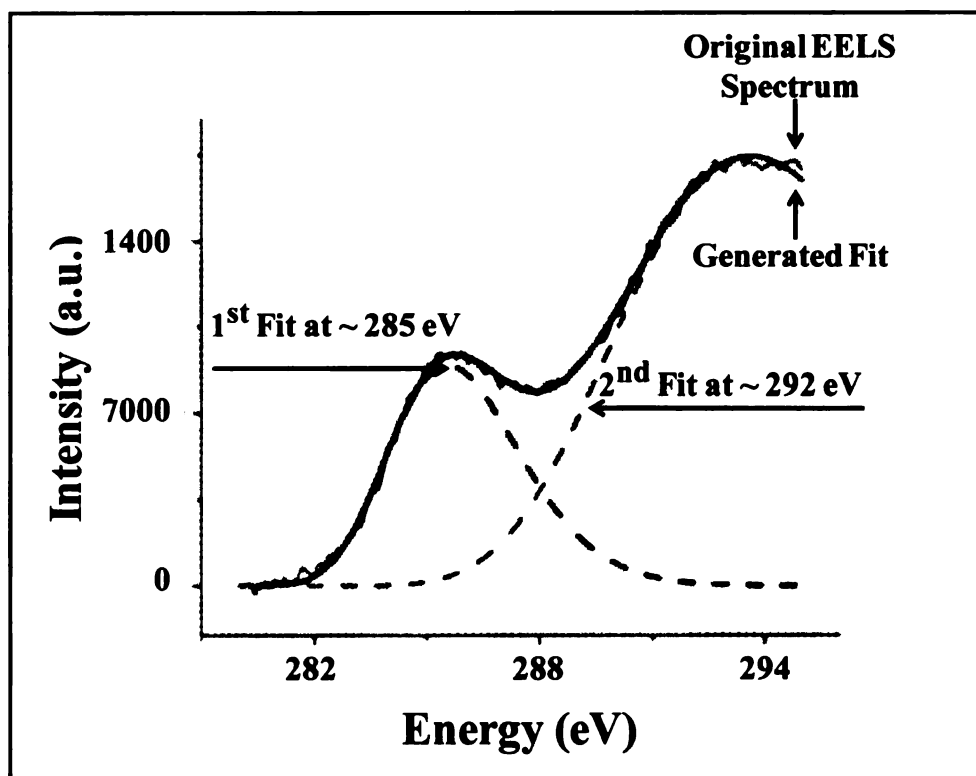
Figure 5.12 Deconvolution of the core loss EELS spectrum of carbon onions, prepared at 1700°C. The original spectrum was deconvolved using 2-peak fit and the asymmetric f-variance function.
