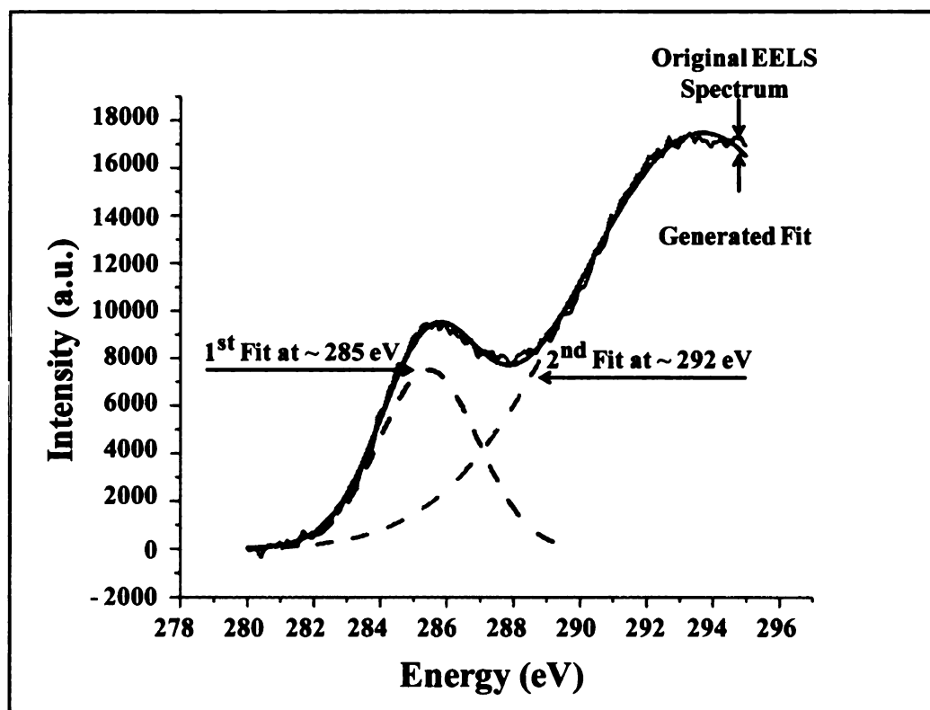
Figure 5.4 Deconvolution of the core loss EELS spectrum of carbon onions, prepared at 1700°C. The original spectrum was deconvolved using 2-peak fit and the symmetric Gaussian deconvolution.
