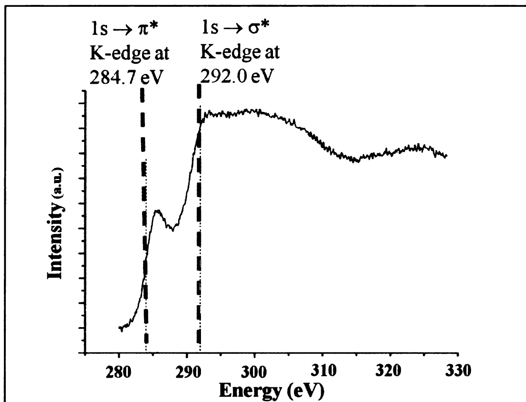
Figure 4.1 A typical EELS spectrum from a largely sp^2 carbon onion sample, synthesized at 1700^\circ\text{C} , with the transition edges marked.
