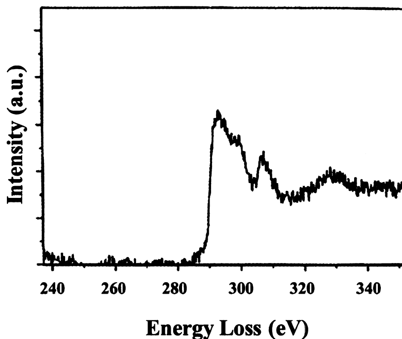
Figure 1.7 EELS core loss spectra of purified NCD particles. Results revealed a single peak at 289 eV and were free of sp^2 bonded carbon 41 .
