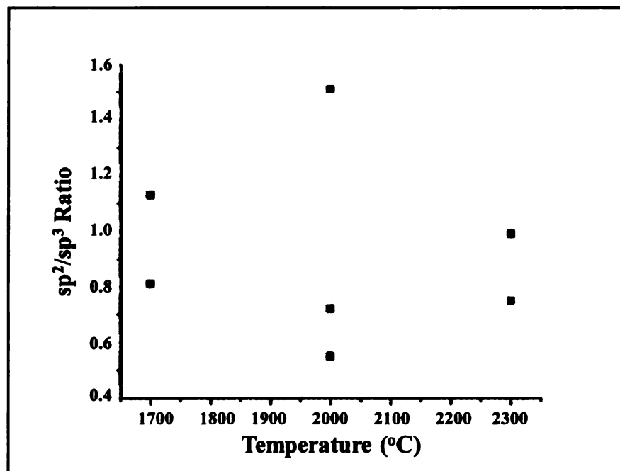
Figure 5.9 A plot of the sp^2/sp^3 ratio in carbon onions as a function of synthesis temperature. The plot is based on results obtained using approach 1.
