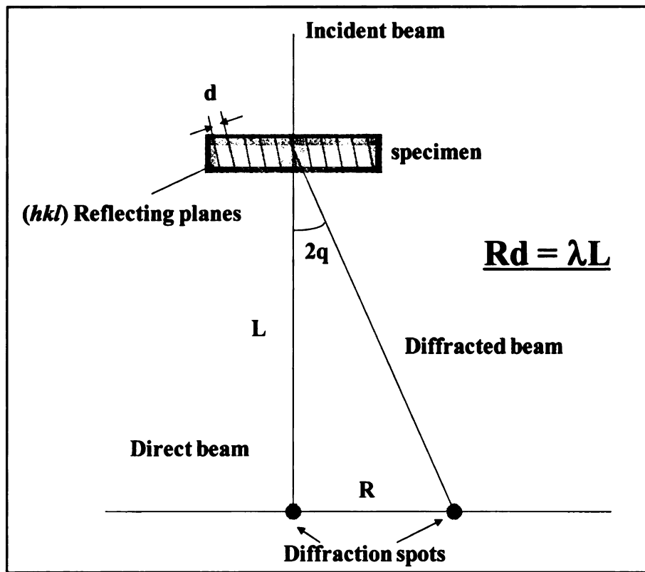
Figure 2.3 Determining the atomic lattice spacing ( d ) in diffraction mode using wave length of the electron ( \lambda ), camera length ( L ), and relative distance between the diffraction spots ( R ).
