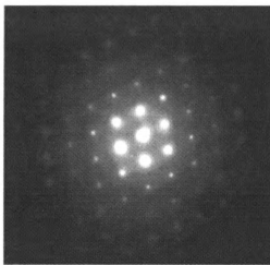
Figure 2.2 Typical diffraction pattern (single crystal pattern).
