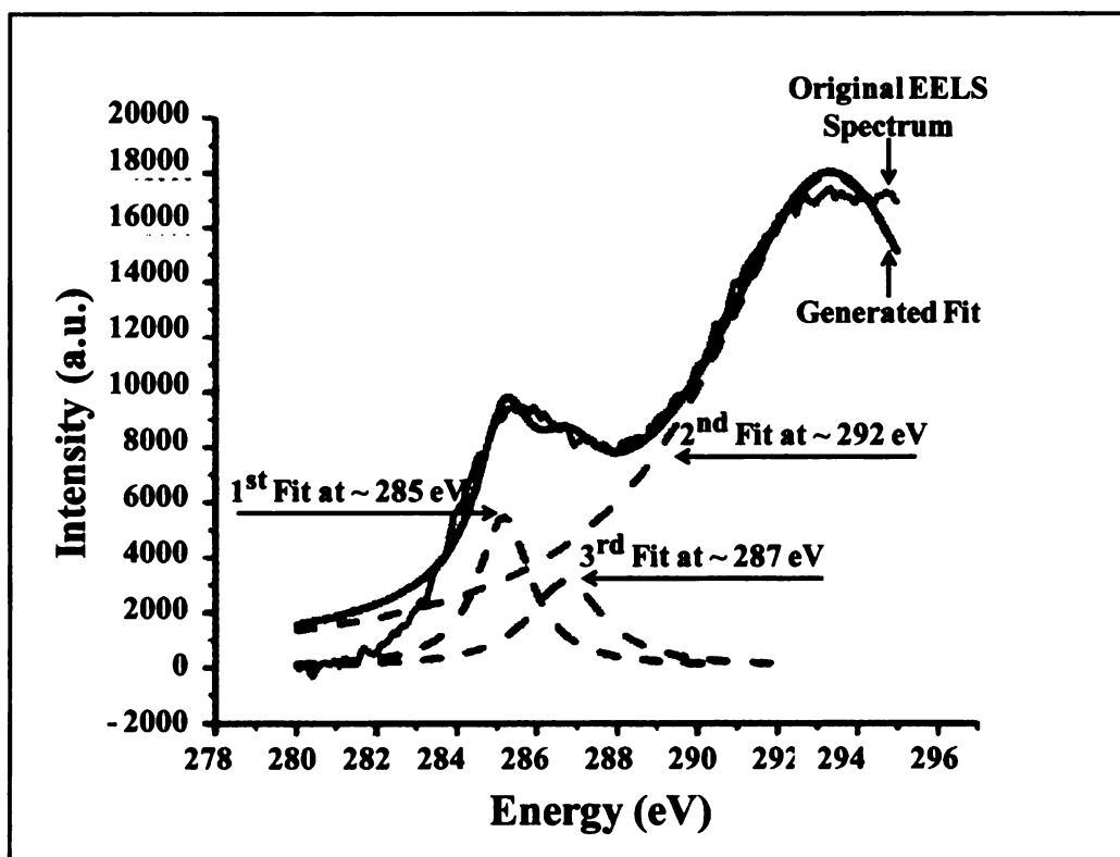
Figure 5.8 Deconvolution of the core loss EELS spectrum of carbon onions, prepared at 1700°C. The original spectrum was deconvolved using 3-peak fit and the symmetric Lorentzian area deconvolution.
