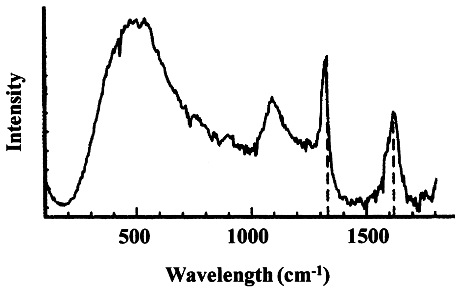
Figure 1.8 A Raman spectrum of NCD 41 .
