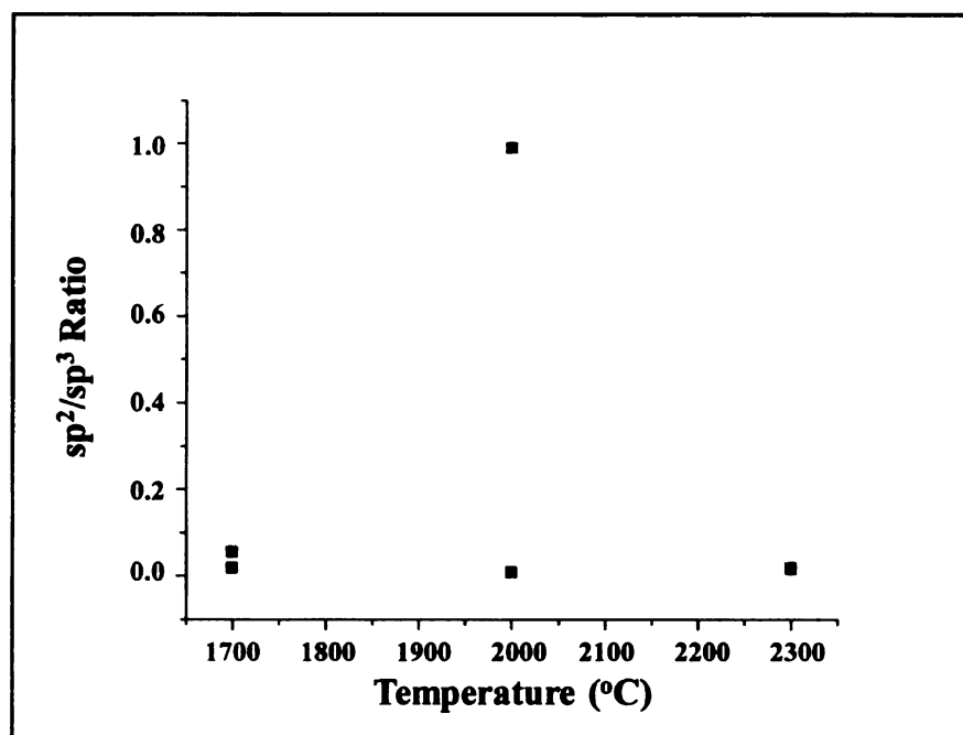
Figure 5.5 A plot of the sp^2/sp^3 ratio in carbon onions as a function of synthesis temperature. The plot is based on results obtained using 2-peak fit and the symmetric Gaussian deconvolution.
