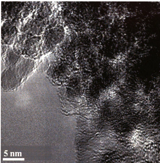
Figure 5.1 An HRTEM image of the largely \text{sp}^3 NCD. Image by: Raied A. Al-Duhileb.
