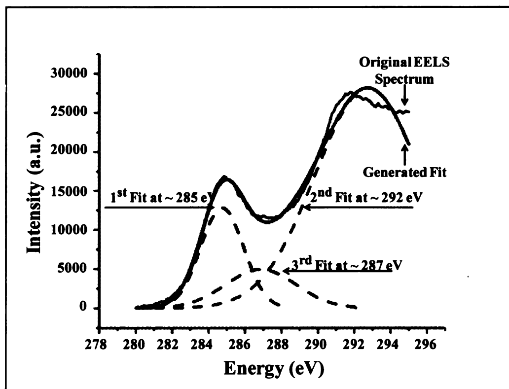
Figure 5.6 Deconvolution of the core loss EELS spectrum of carbon onions, prepared at 1700°C. The original spectrum was deconvoluted using 3-peak fit and the symmetric
