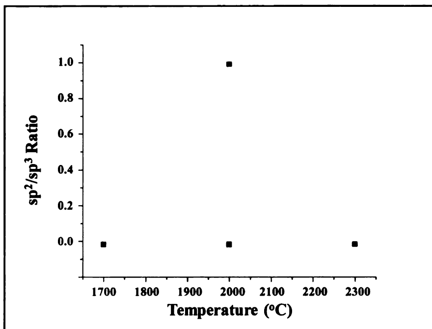
Figure 5.7 A plot of the sp^2/sp^3 ratio in carbon onions as a function of synthesis temperature. The plot is based on results obtained using 3-peak fit and the symmetric Gaussian deconvolution.
