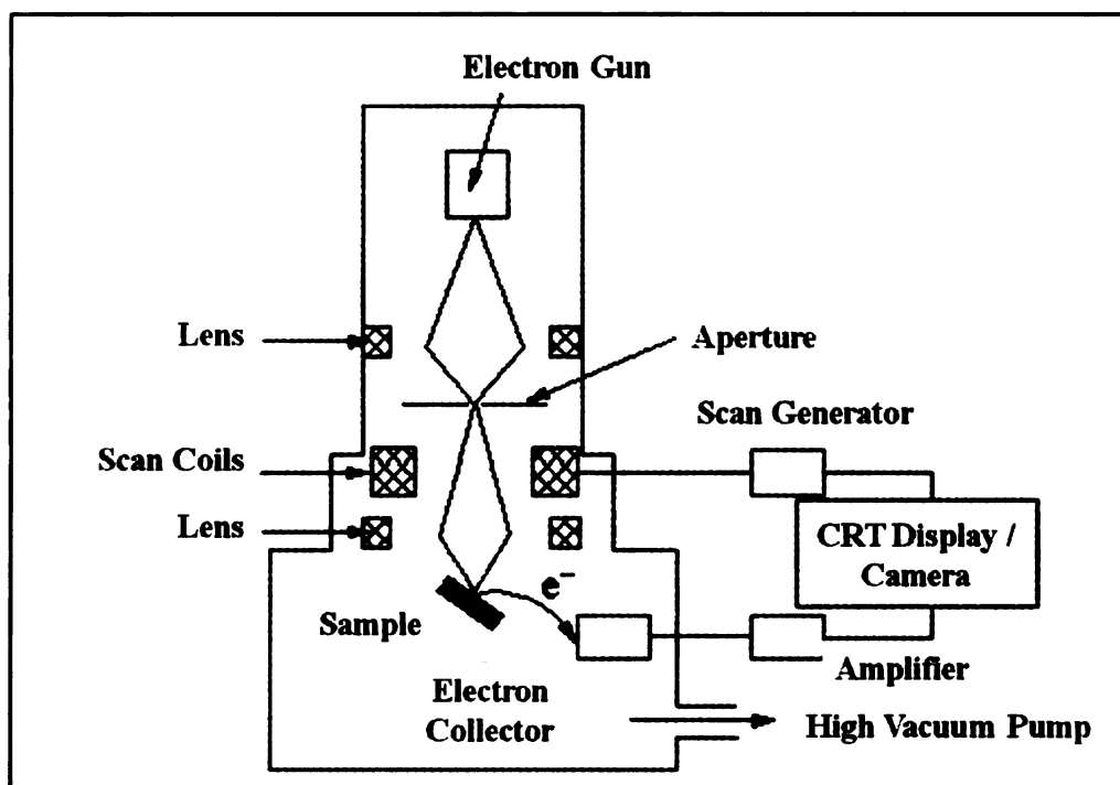
Figure 2.4 A schematic diagram illustrating the basic components and operation of an SEM. An electron gun focuses an electron beam on the surface of the sample. This results in producing secondary electrons that are collected by special electron detector and displayed as a mapped image on a screen 3 .
