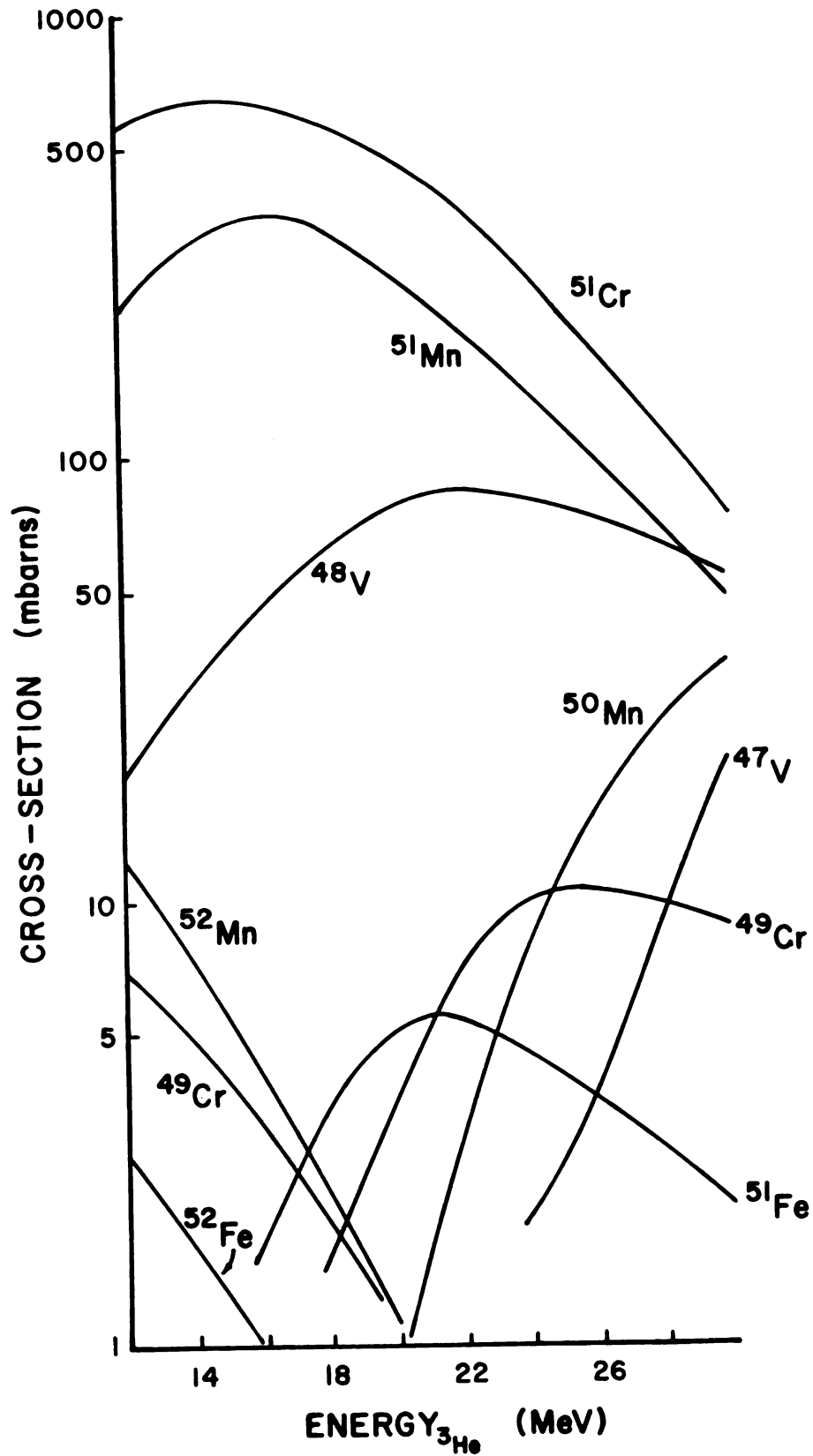
Figure 8-2. ALICE predictions for ^3\text{He} on ^{50}\text{Cr} .
