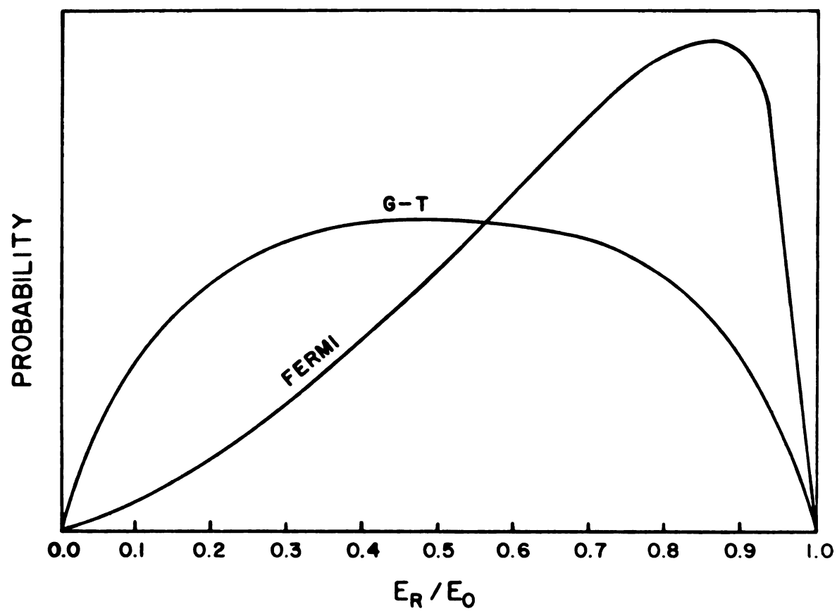
Figure 11-1. Calculated \beta -recoil energy distributions.
