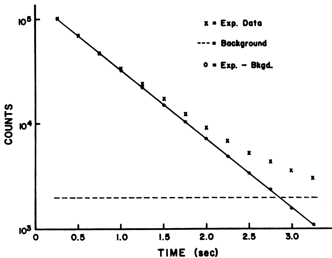
Figure 10-4. The data and the fit for the ^{47}\text{Cr} half-life measurement.
