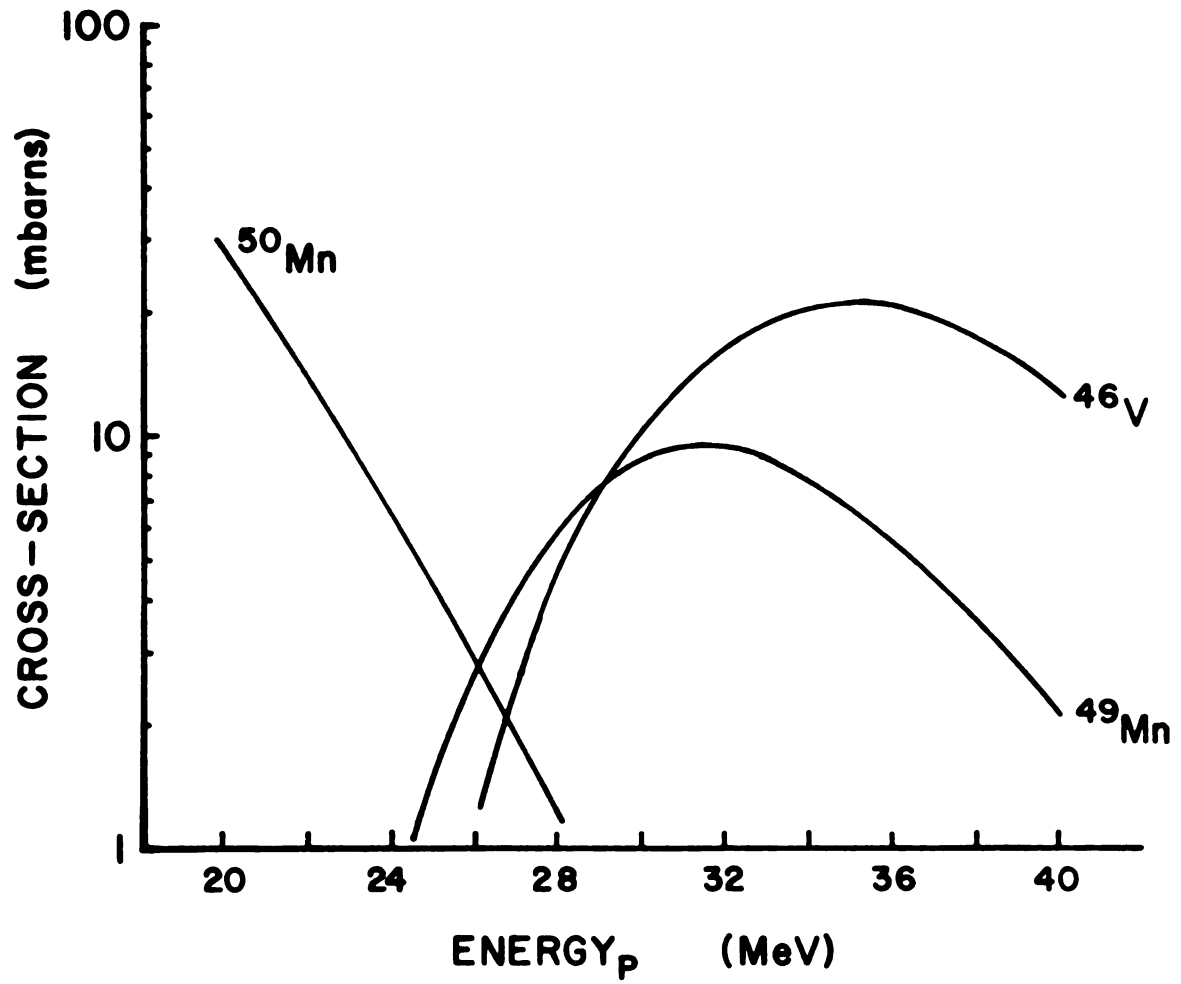
Figure 8-5. ALICE predictions for protons on ^{50}\text{Cr} .
