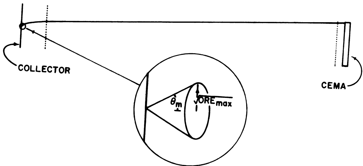
Figure 6-2. Definition of \text{ORE}_{\text{max}} and \theta_m .
