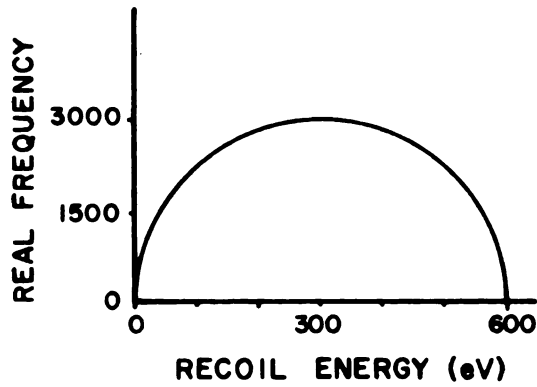
Figure 6-3a. An approximate \beta -recoil energy distribution.
