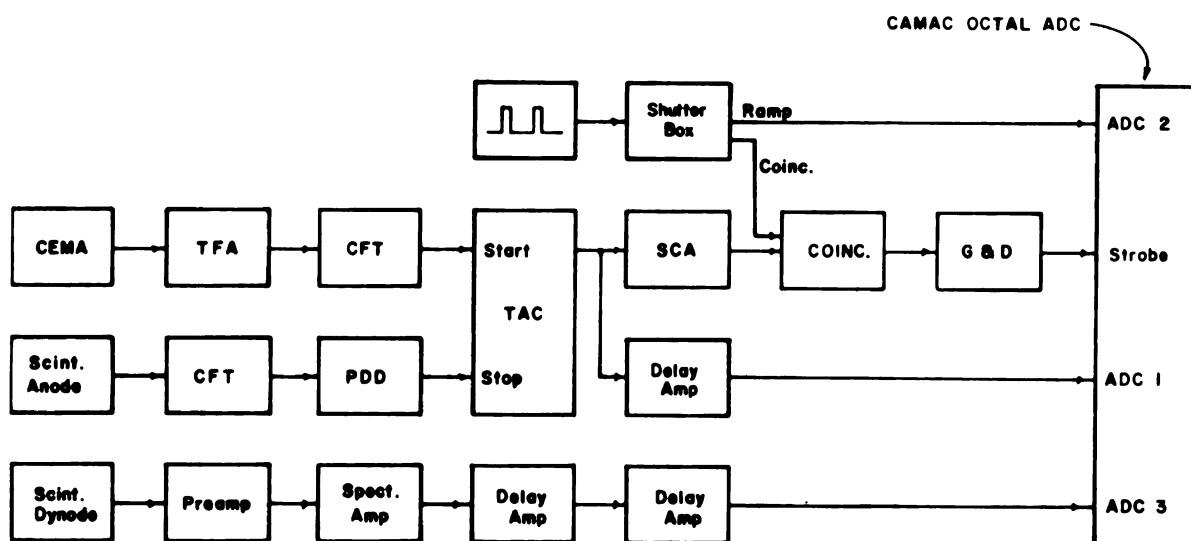
Figure 8-7. Electronics used to collect the data shown in Figure 8-8.
