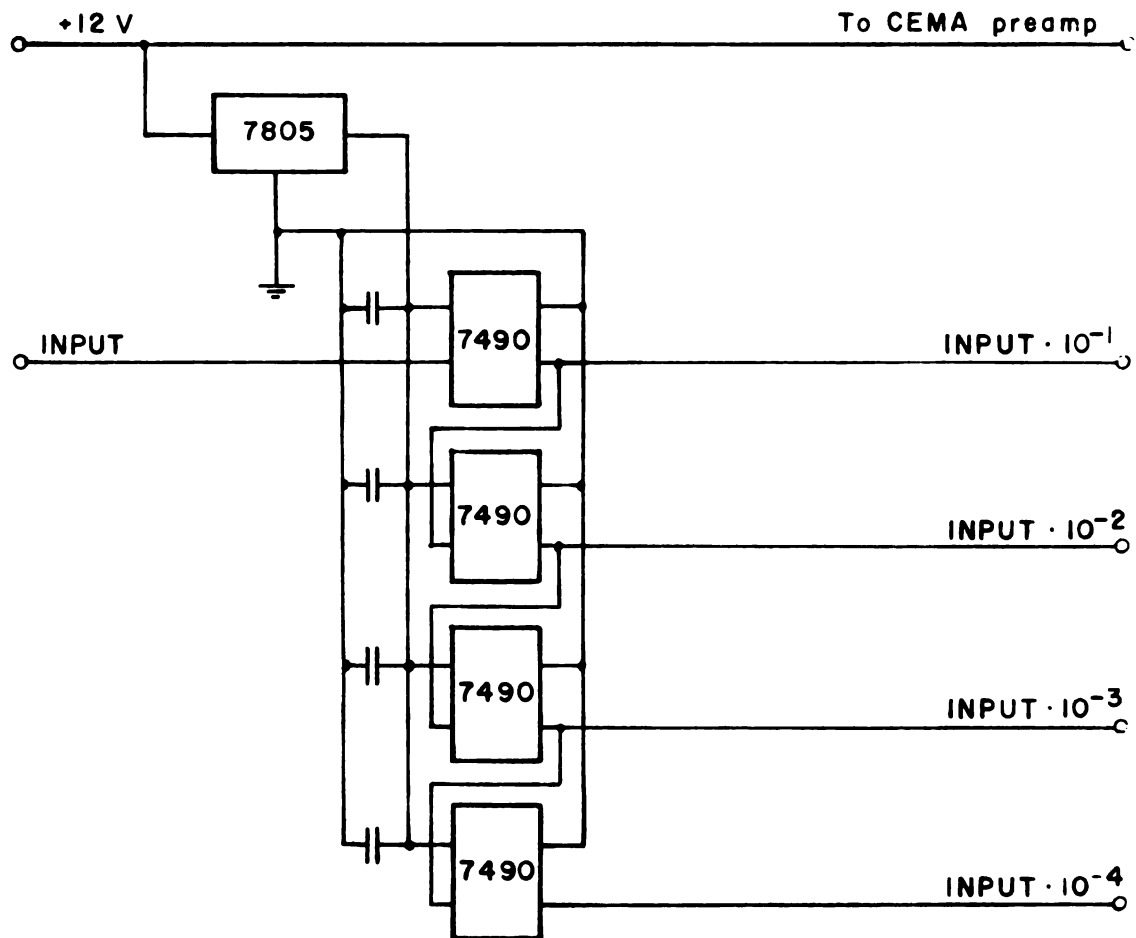
Figure D-2. Schematic of the decade dividers for the PDD oscillator.
