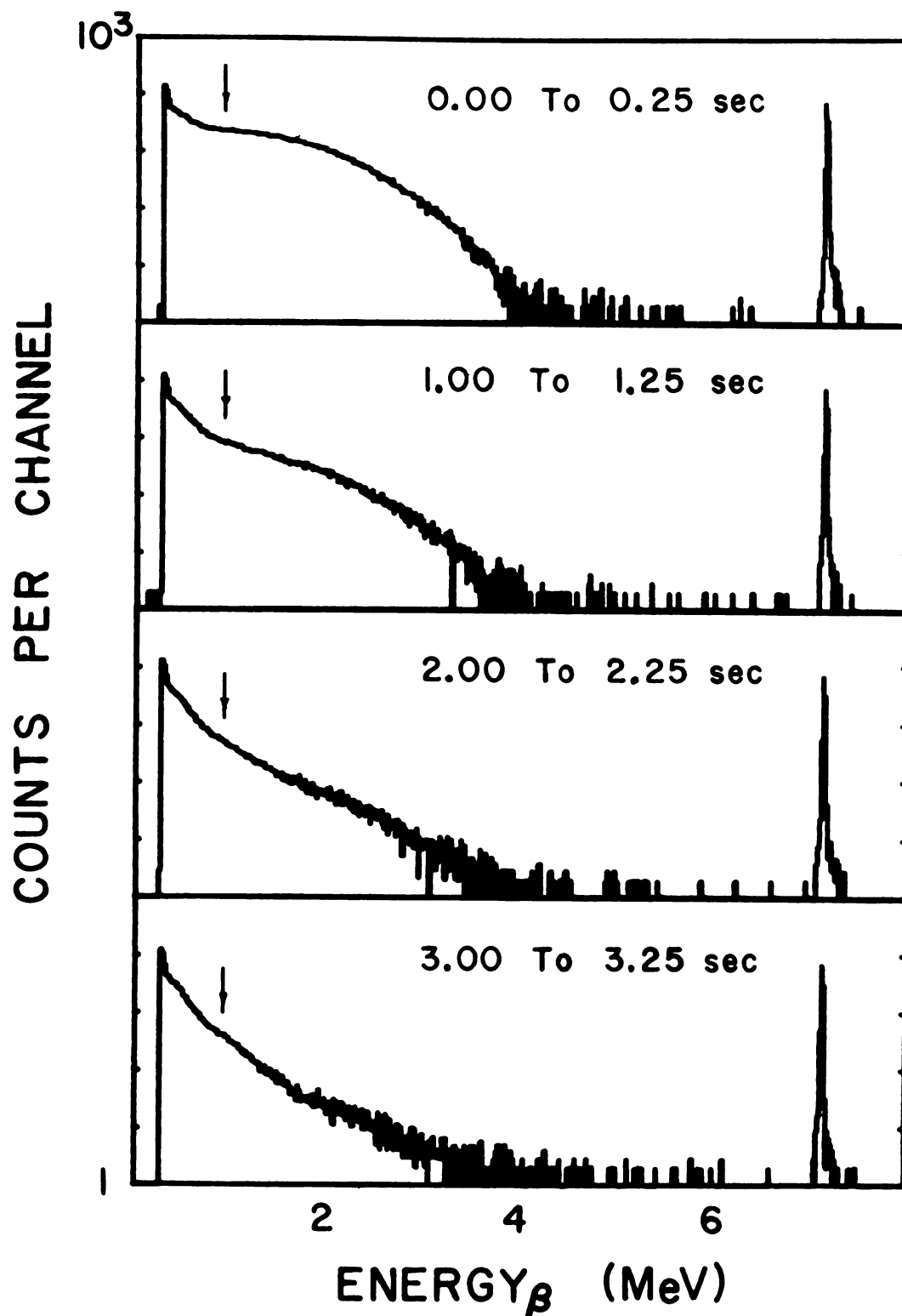
Figure 10-3. Some of the \beta spectra from the ^{47}\text{Cr} half-life measurement.
