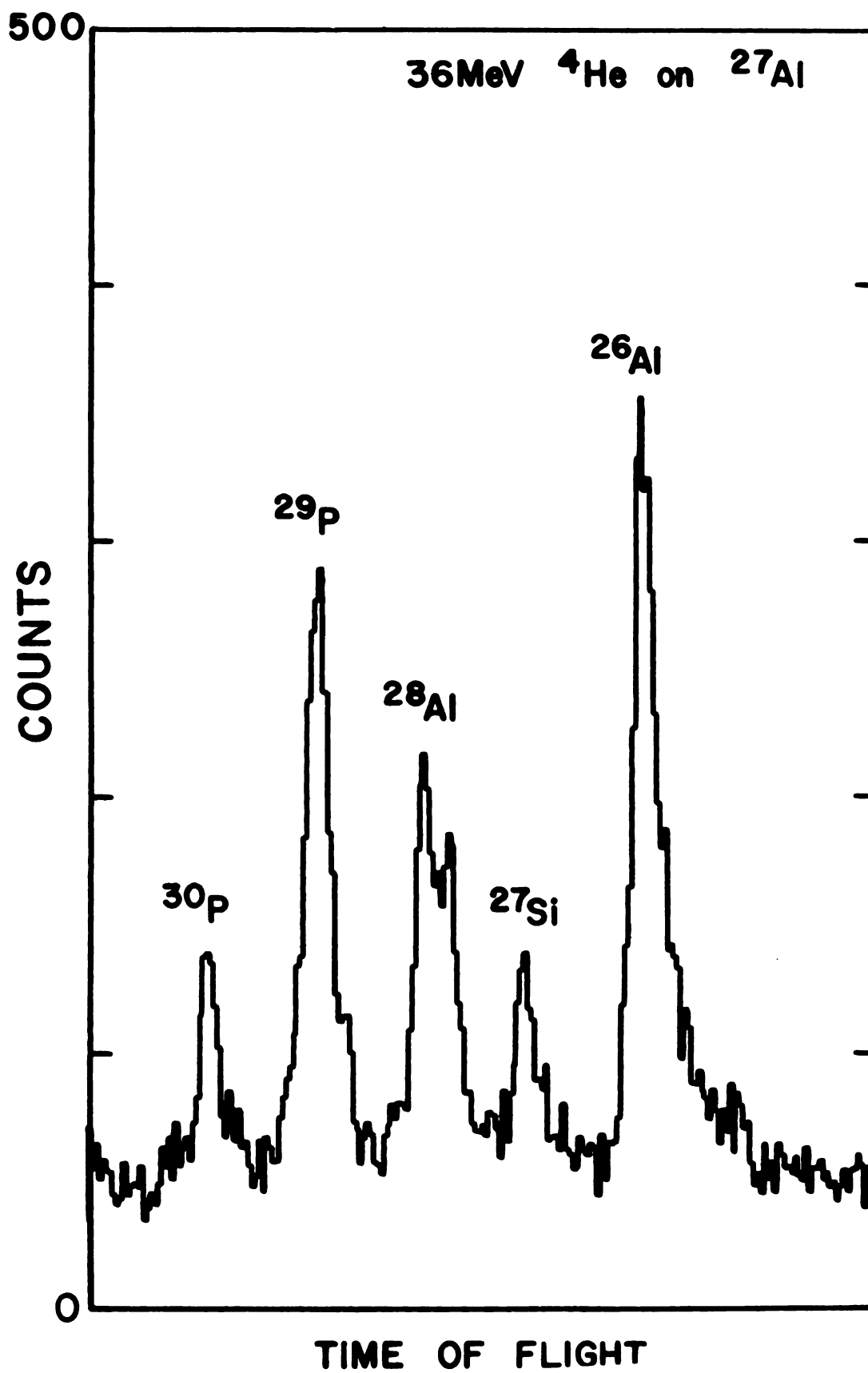
Figure 5-1. A shuttered spectrum without the delay.
