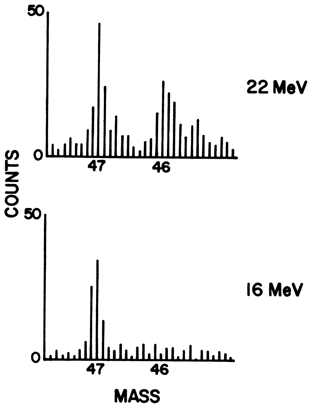
Figure 10-1. Mass spectra obtained with 22-MeV and 16-MeV ^3\text{He} on ^{46}\text{Ti} .
