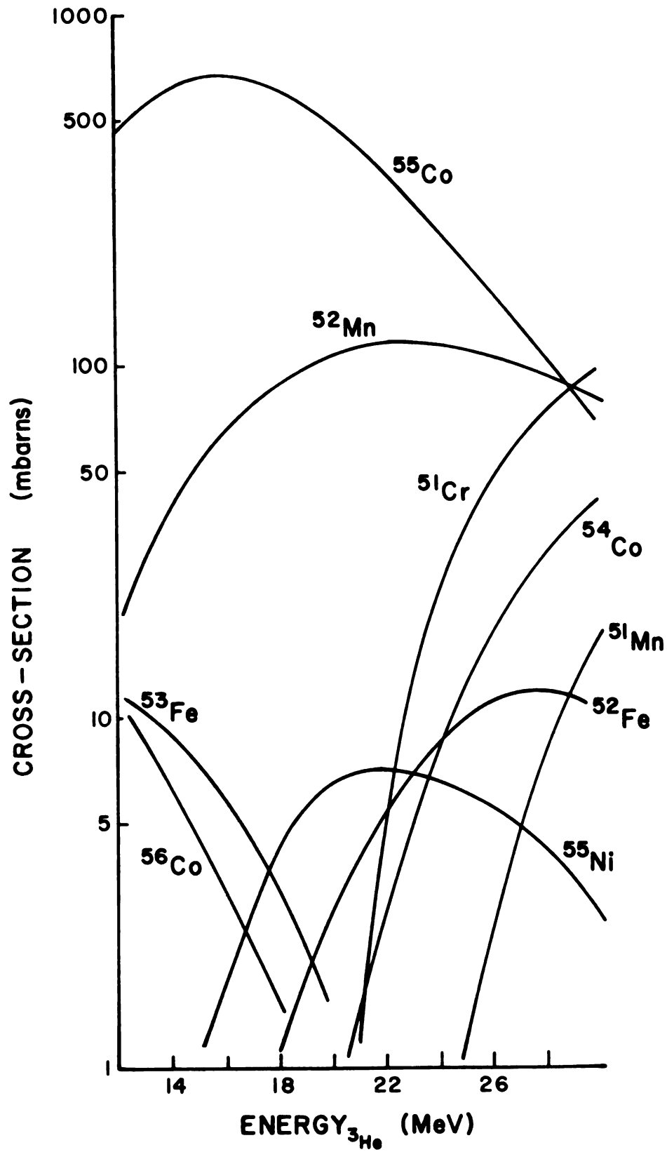
Figure 8-3. ALICE predictions for ^3\text{He} on ^{54}\text{Fe} .
