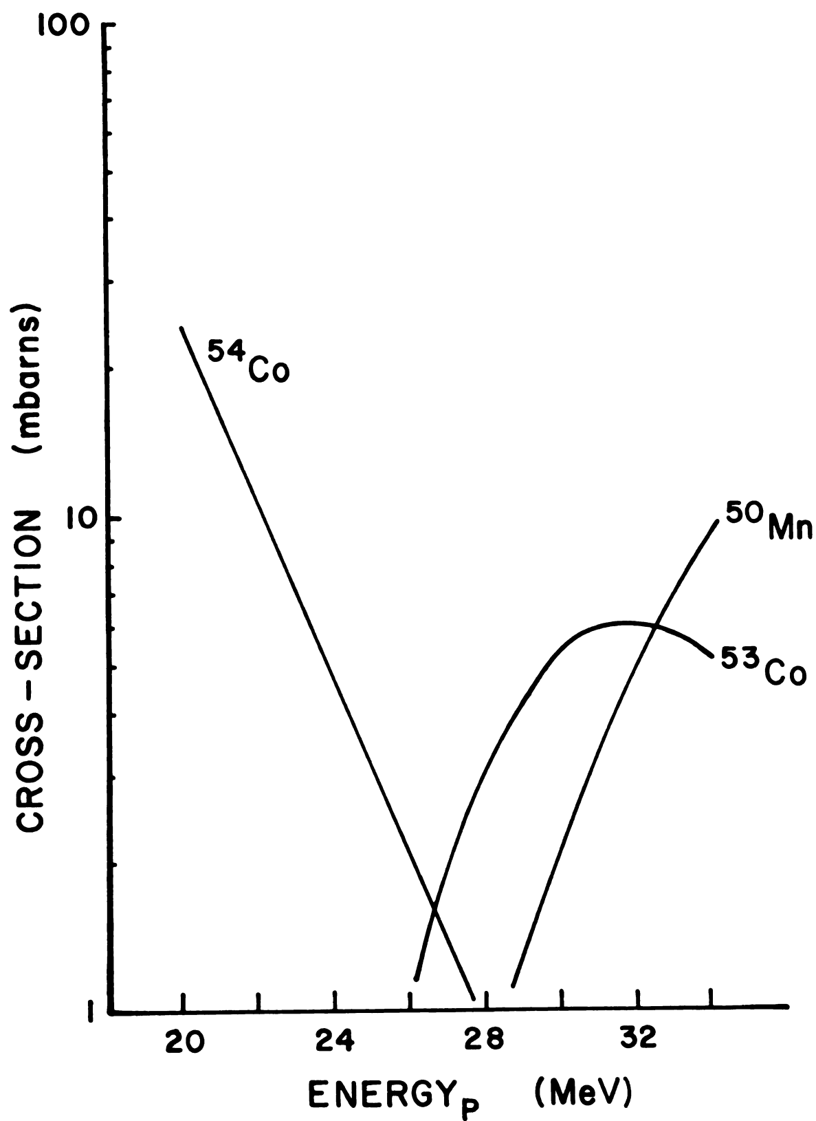
Figure 8-6. ALICE predictions for protons on ^{54}\text{Fe} .
