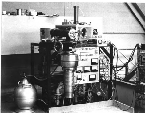
Figure H-2. Front view of SIEGFRIED. The wooden platform is raised about 1 m above the floor to allow easy access to the vacuum chambers. The fore-pumps are beneath the floor.
