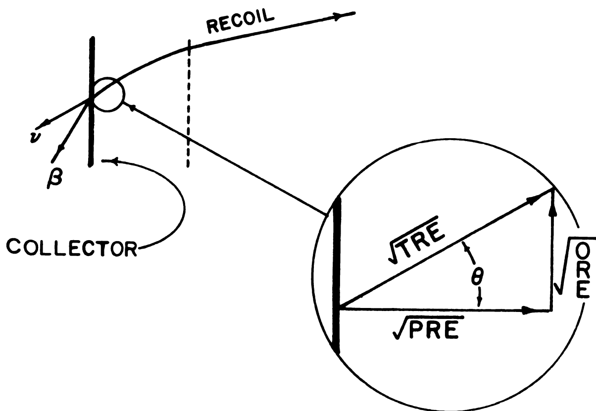
Figure 6-1. Definition of recoil components.
