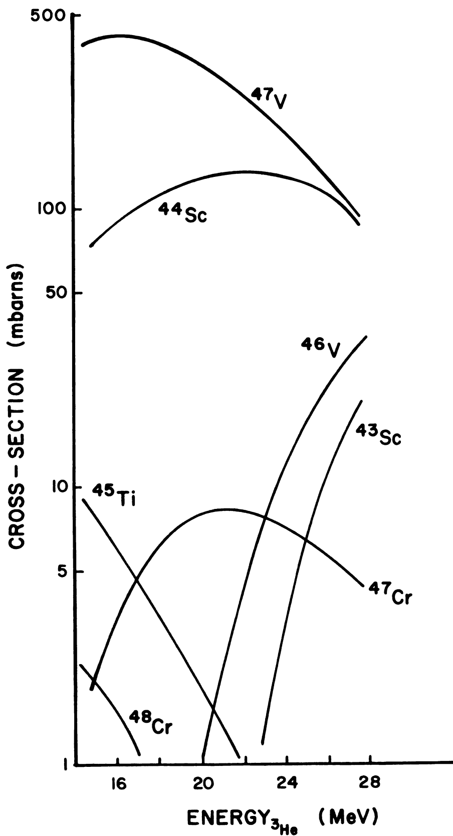
Figure 8-1. ALICE predictions for {}^3\text{He} on {}^{46}\text{Ti} .
