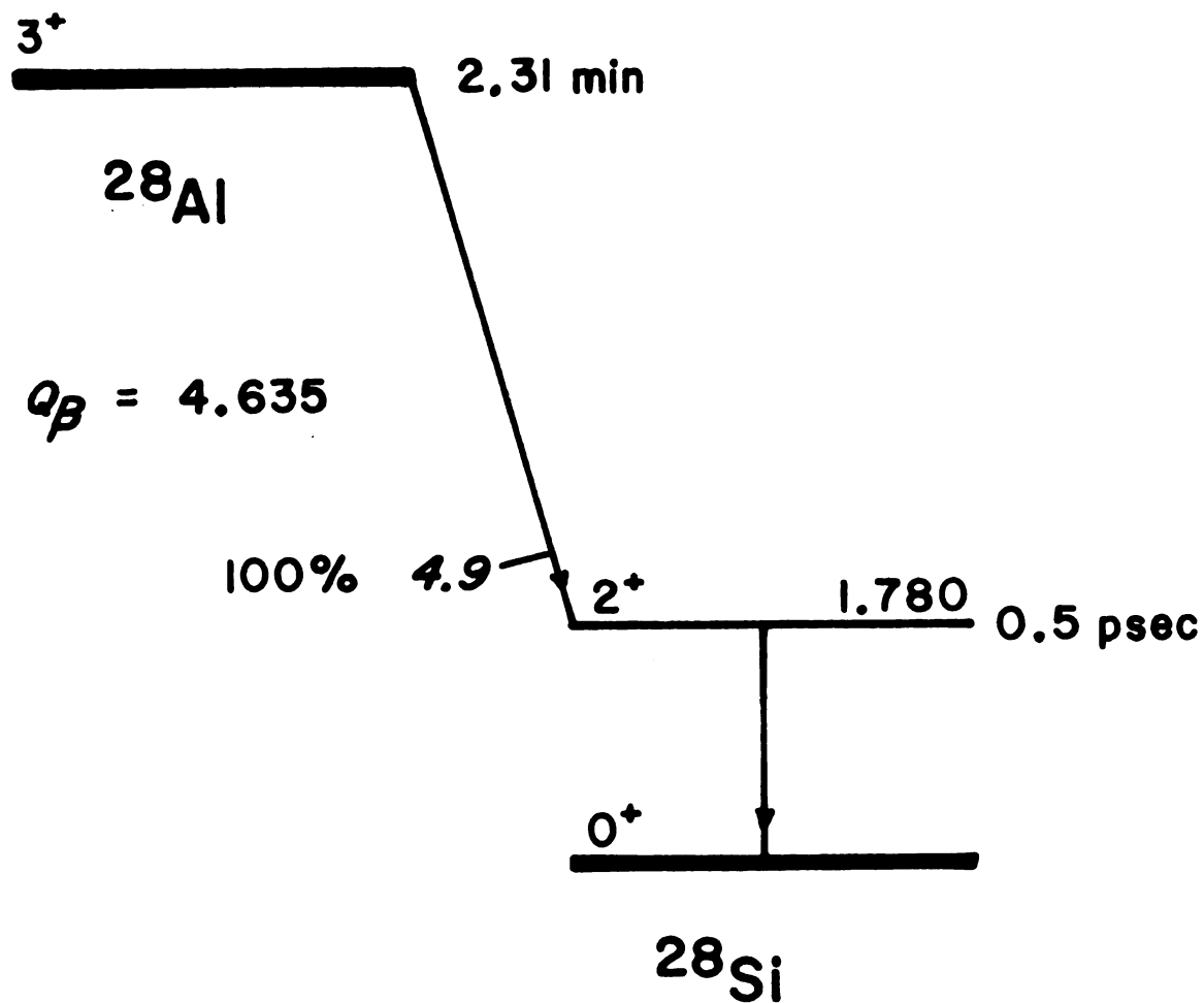
Figure 6-4. The decay of ^{28}\text{Al} .
