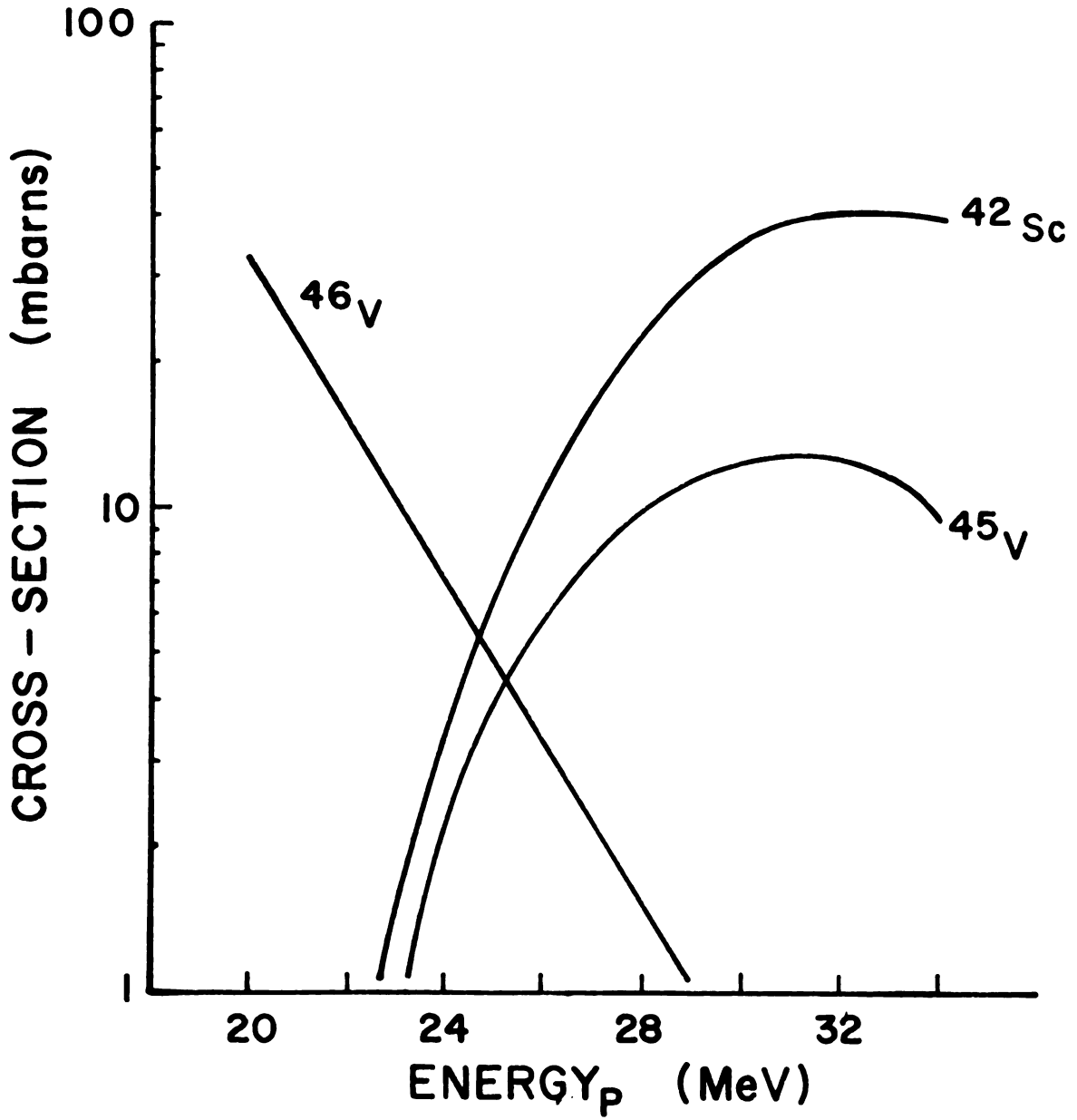
Figure 8-4. ALICE predictions for protons on ^{46}\text{Ti} .
