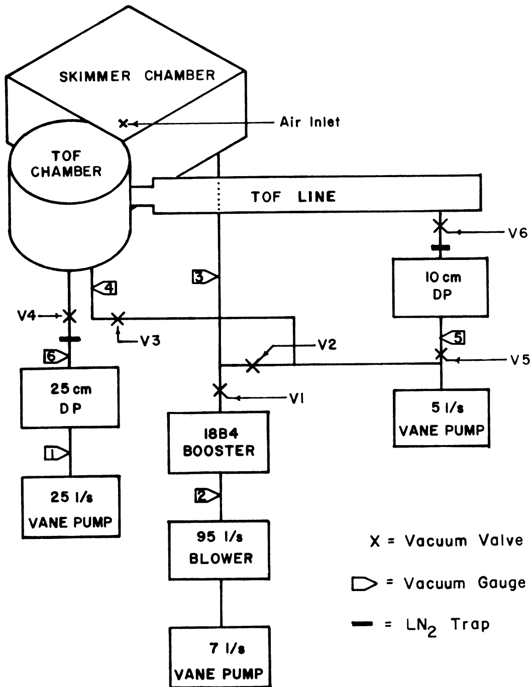
Figure A-1. SIEGFRIED's vacuum system.
