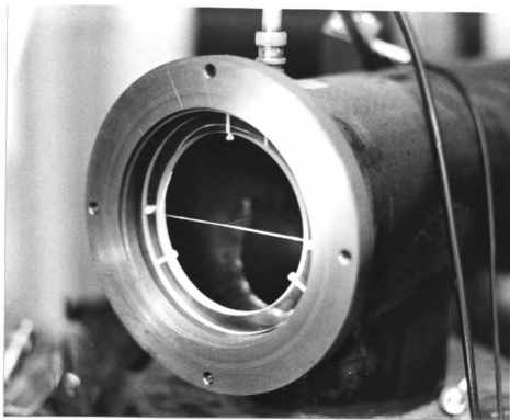
Figure H-5. The end of the flight tube showing the plexiglas ring which holds the ESGP. the ESGP wire is very thin, but it can just be seen as it leaves the support wire.
