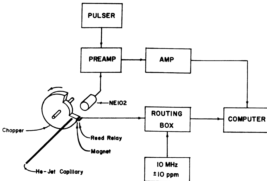
Figure 10-2. Schematic diagram of the chopper system used to measure the half-life of ^{47}\text{Cr} .
