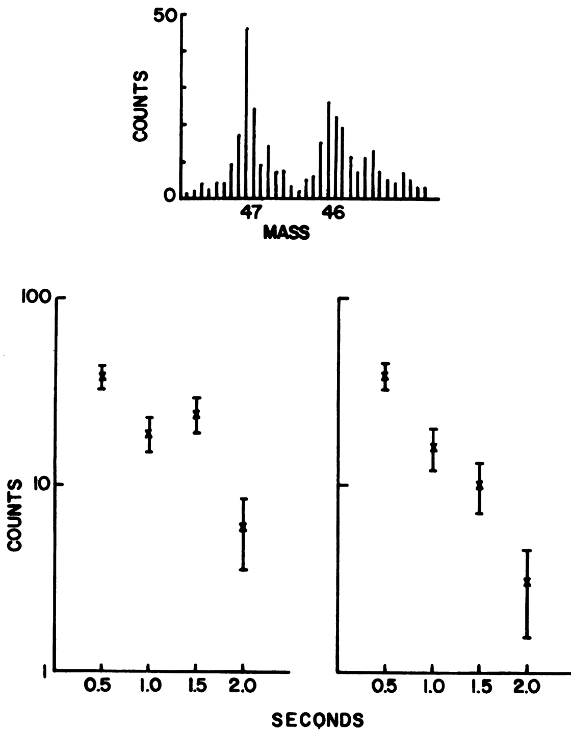
Figure 8-8. Data collected when attempting to measure the half-life of ^{47}\text{Cr} with SIEGFRIED.
