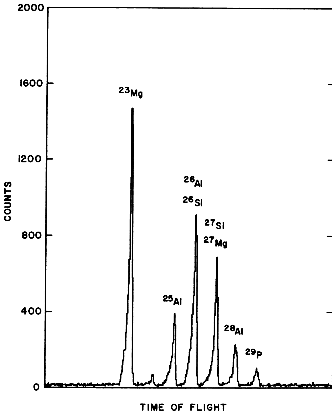
Figure 7-3. A typical spectrum from an aluminum target when SIEGFRIED is used in the usual manner. The beam was 70-MeV ^3\text{He} .
