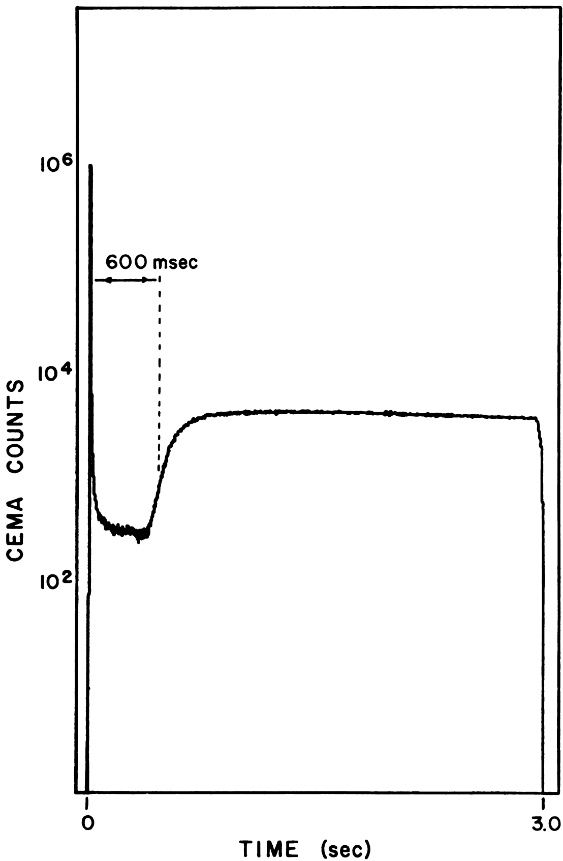
Figure 9-1. CEMA-gated ramp spectrum showing the plasma transport time.
