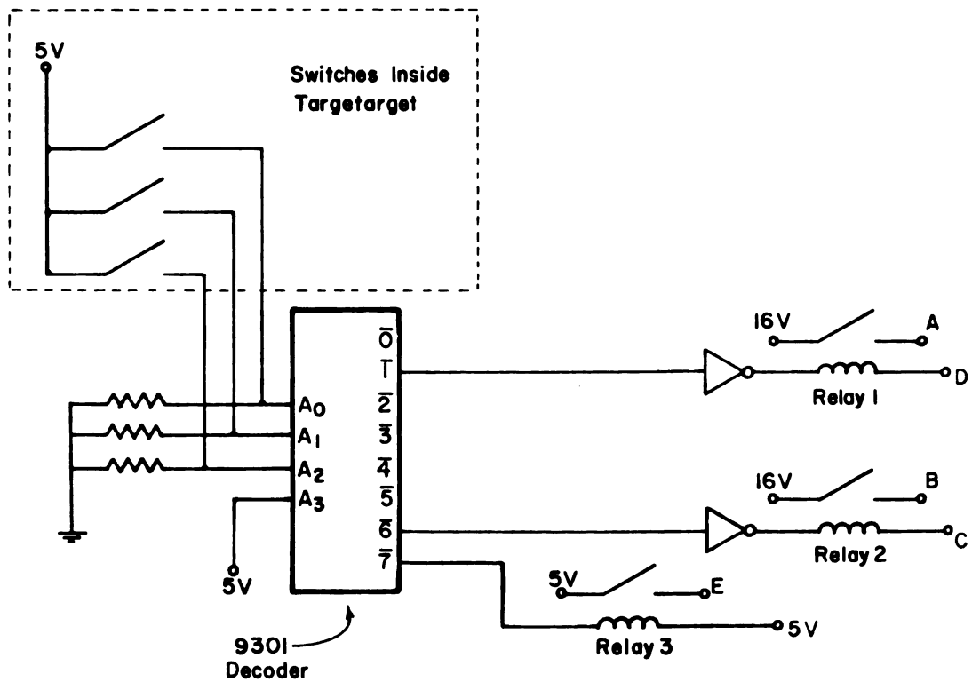
LOGIC SCHEME
