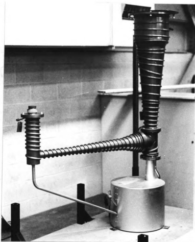
Figure H-3. The Edwards 18B4 booster pump. The pump is nearly 2 m tall and the intake is about 40 cm in diameter. The vertical part contains the diffusion stages and the horizontal part contains the ejector stage.
