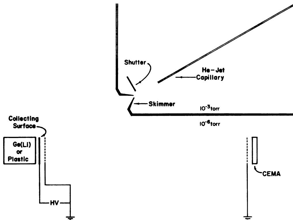
Figure 2-1. Schematic diagram of SIEGFRIED.
