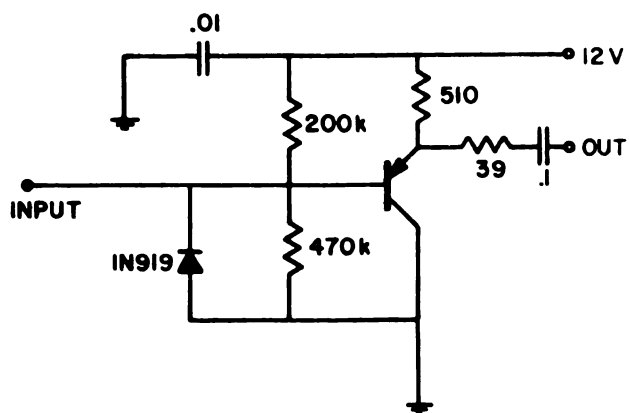
Figure B-2. Schematic of the emitter follower.
