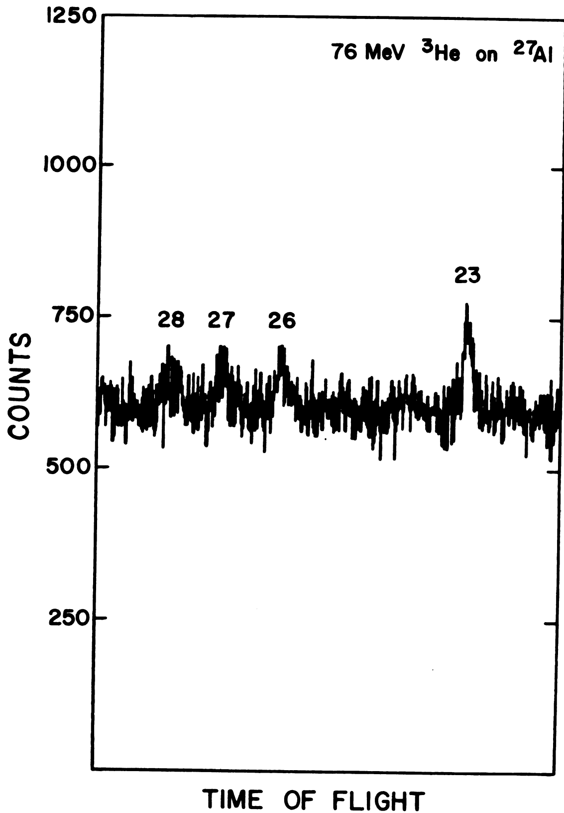
Figure 4-1. One of the first spectra obtained with SIEGFRIED.
