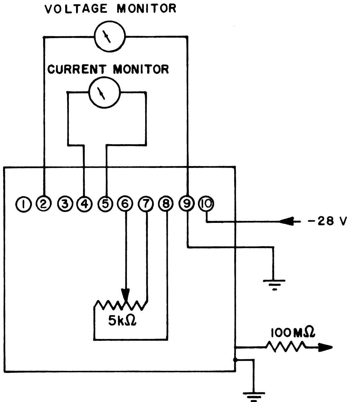
Figure E-1. Schematic of the control circuit for the Spellman supply.
