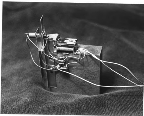
Figure H-6. The shutter and failsafe mechanism.
