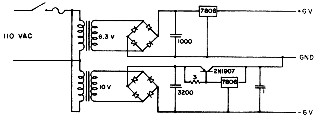
Figure D-1. Schematic of the \pm 6 -V power supply for the PDD.
