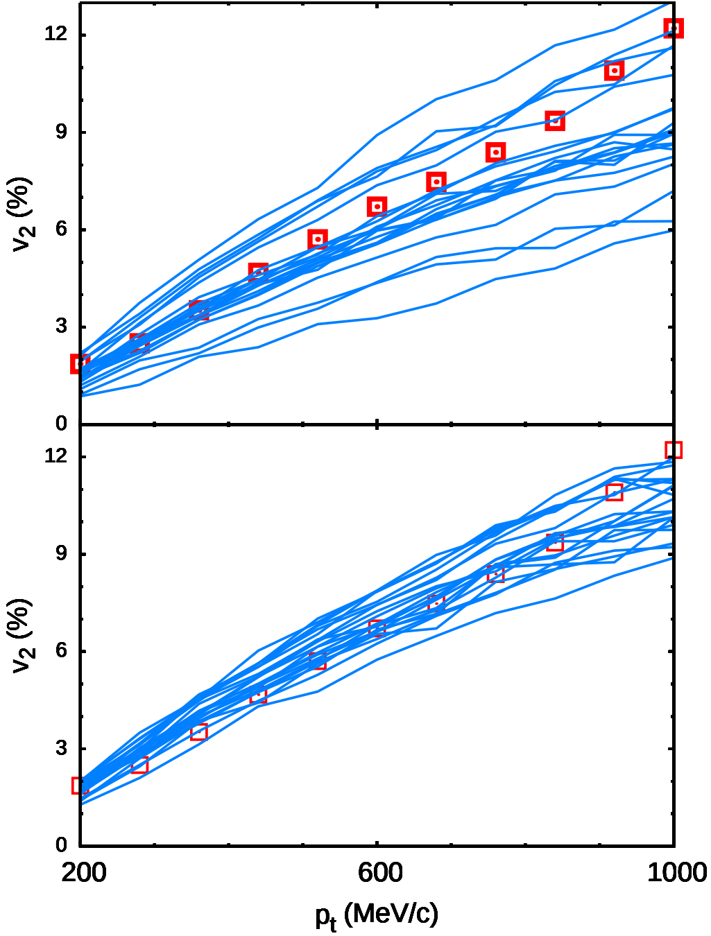
Figure 6.13: The anisotropic flow as a function of transverse momentum for pions. The (red) squares are experimental data from the STAR collaboration. The twenty (blue) lines are model runs in each panel; in the top panel they are chosen via uniform sampling of the parameter space while in the bottom panel they are taken randomly from the MCMC trace which samples more likely regions more heavily. The runs from the MCMC trace are considerably closer to the experimental data but note that the posterior distribution contains many settings that do not describe the anisotropic data with high precision.
