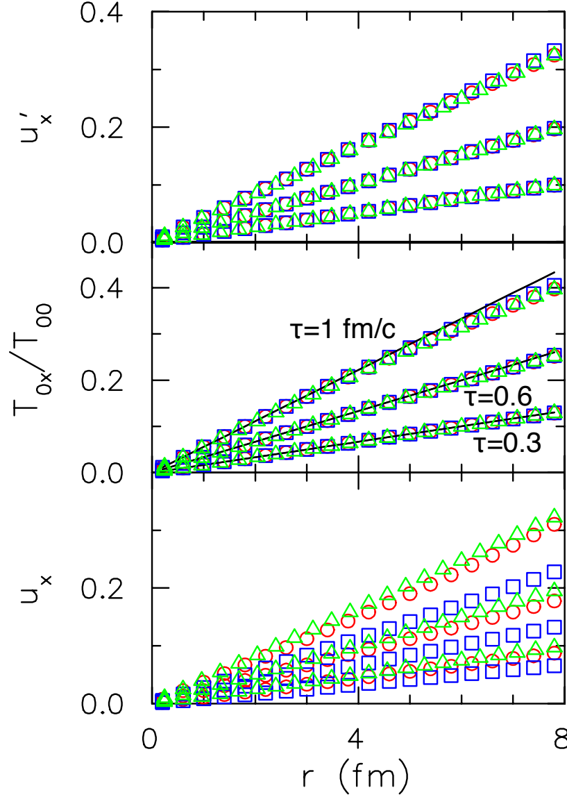
Figure 5.5: Bottom panel: The velocity of the frame in which T^{0x} = 0 for coherent electromagnetic fields (blue squares), for incoherent fields or a non-interacting gas (red circles), and for an ideal liquid (green triangles) shown at three time steps, \tau = \{0.3, 0.6, 1.0\} fm/c. The models predict significantly different amounts of radial flow, though in the opposite hierarchy suggested by the transverse pressure due to the effects of the Bjorken expansion. This quantity may change during thermalization.
