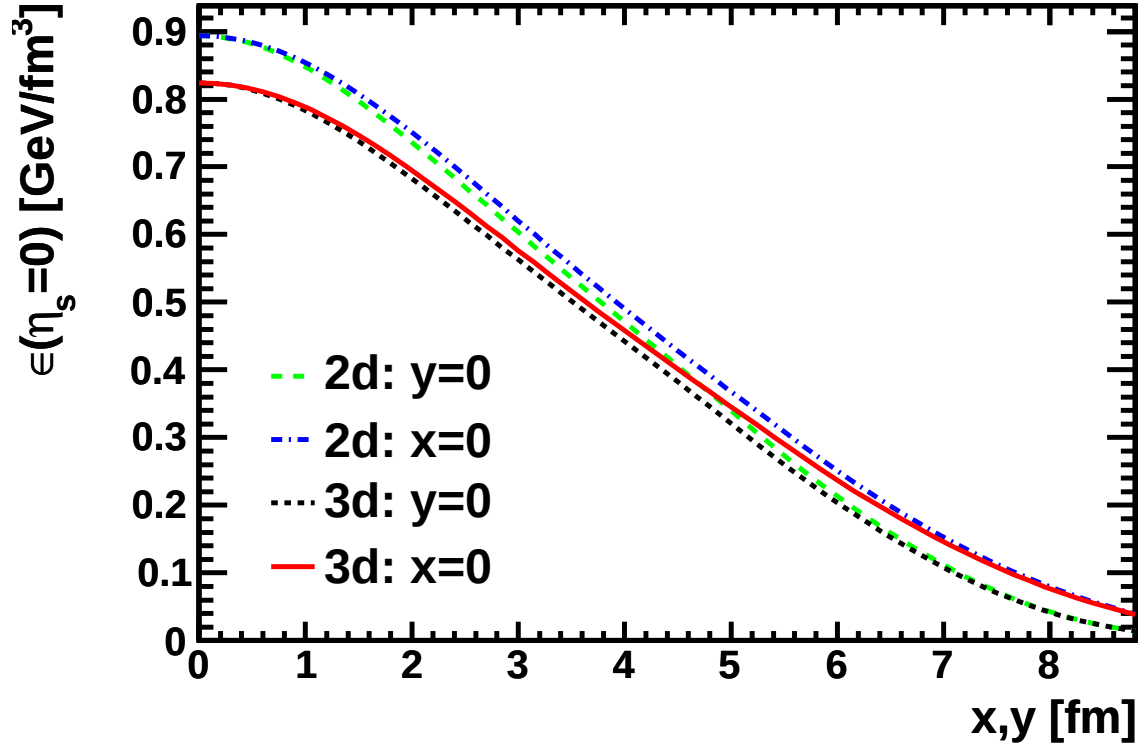
Figure 6.1: Comparison of the energy density along the x- and y-axes at midrapidity at \tau = 5.52 fm/c from a boost invariant and full 3d hydrodynamic treatment. While the central energy density falls more rapidly when the longitudinal expansion is included due to the increase in the longitudinal velocity gradient, which can be seen by observing that both 3d lines (red full and black dotted) are systematically lower than their 2d counterparts (blue dot-dashed and green dashed). The difference diminishes in the tails of the distribution but is roughly 5-10% at the center of the fireball.
