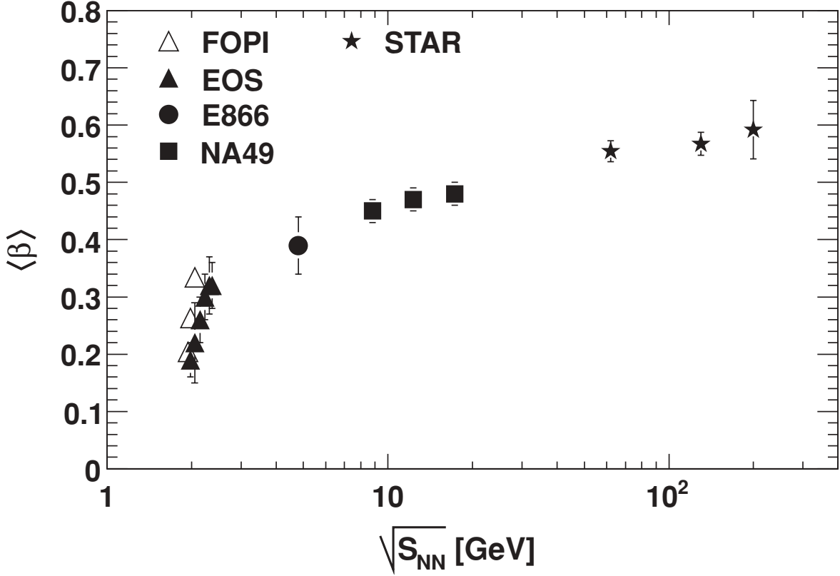
Figure 1.3: Average particle velocity extracted from the particle spectra of heavy ion collisions of various nuclei via a blast wave fit as a function of the beam energy per nucleon pair [12]. Low momentum pions ( p_T < 0.5 GeV/c) are removed from the fit due to resonance background. Strong collective velocity is a strong indicator of the onset of collective behavior for collisions at center of mass energy per nucleon pair greater than a few GeV.
