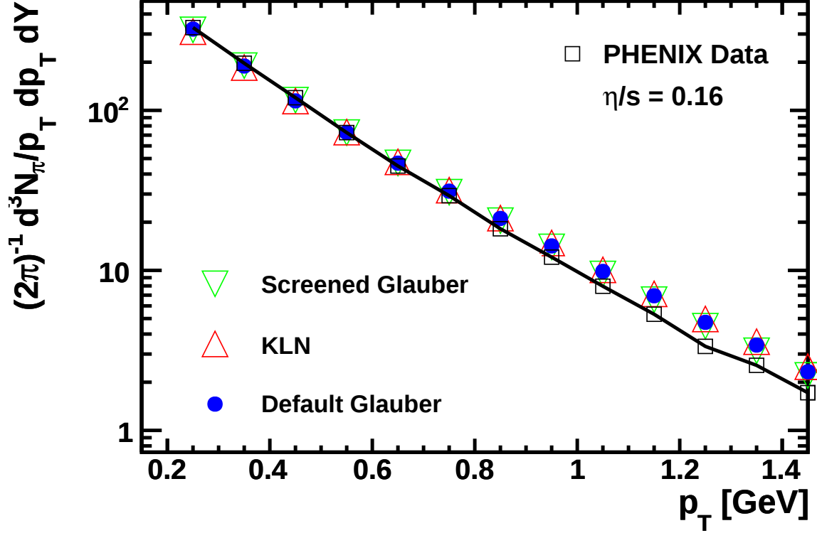
Figure 6.5: Pion spectra at midrapidity for the most central (0-5%) bin of Au+Au collisions at \sqrt{s} = 200 GeV as a function of transverse momentum. The (black) line with squares is minimum bias data from the PHENIX experiment [70] corrected for experimental acceptances and efficiencies. The colored symbols are for three model runs with different initial conditions for the energy density where all three models have been tuned to reproduce the total number of pions between p_T = 200 MeV and 1 GeV. All of the models are easily capable of reproducing the total multiplicity and there is not much variation in the slope meaning that this observable is not likely to have significant resolving power.
