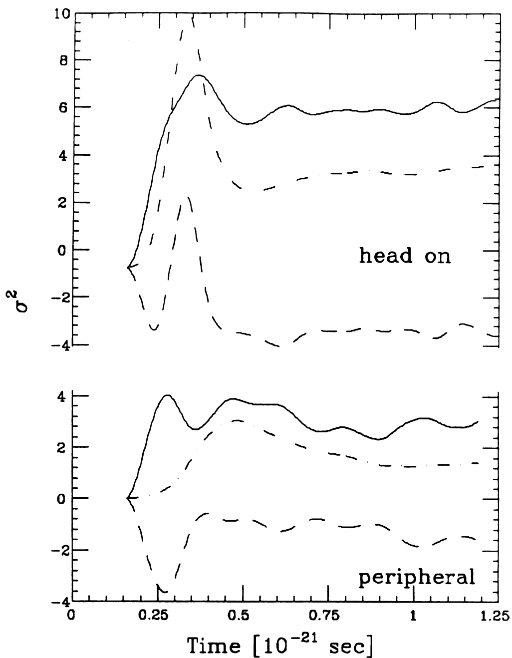
Figure 5.11: \sigma_R^2 calculated with Eq. 5.25 (dot-dashed line), Eq. 5.26 (dashed line) and the sum of both (solid line). The unit of \sigma_R^2 is [amu] 2 .
