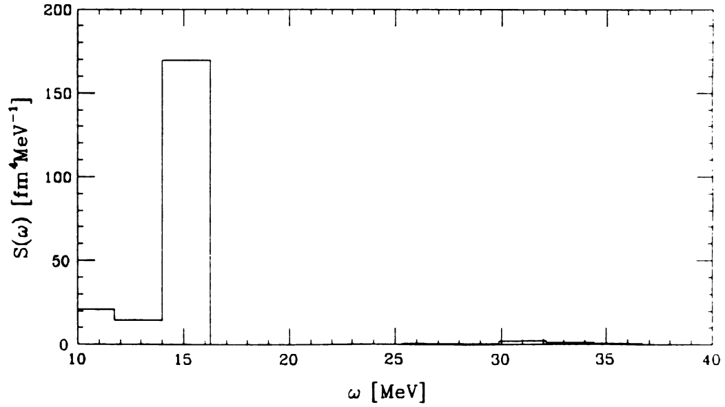
Figure 4.14: Quadrupole strength distribution calculated in TDHF for ^{40}\text{Ca} .
