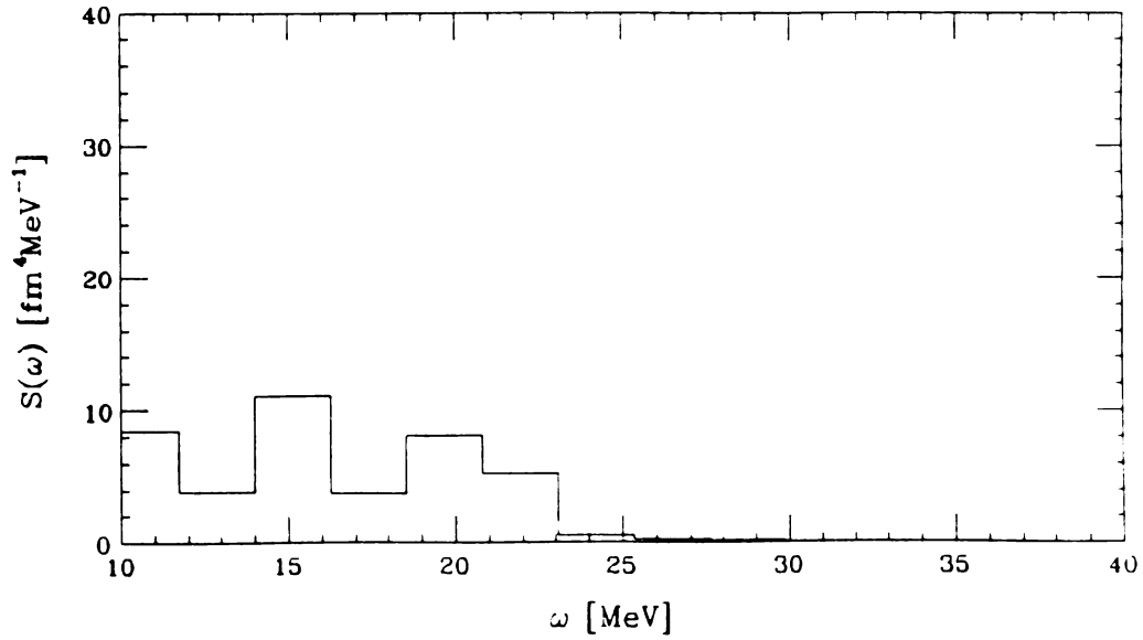
Figure 4.11: Quadrupole strength distribution calculated in TDDM for ^{16}\text{O} .
