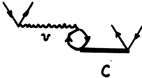
Figure 2.1: Typical diagrams in each term of Eq. 2.23; the wavy lines are interactions and the thick lines are two-body correlations.
