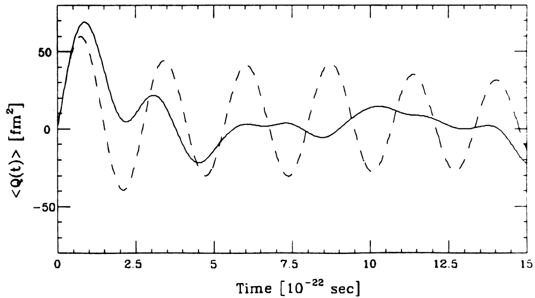
Figure 4.10: Quadrupole moments as function of time for ^{40}\text{Ca} , the solid line is calculated in TDDM and the dashed line in TDHF .
