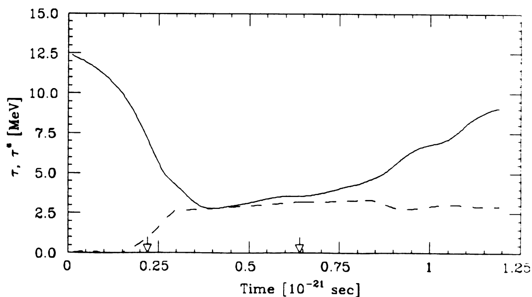
Figure 5.7: Same as Figure 5.6 but for peripheral collision.
