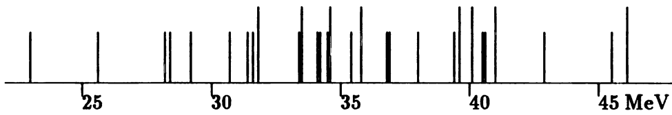
Figure 4.16: The excitation energies at the unperturbed states are shown for the isoscalar E2^+ transition in ^{16}\text{O} . The long vertical lines are those of 1p - 1h states and the short lines are those of 2p - 2h states.
