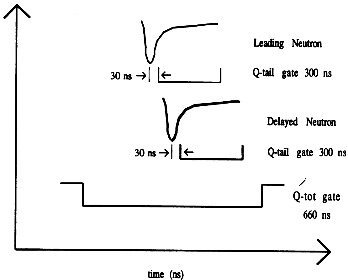
Figure F.2: Schematic of the timing for the leading and delayed neutron. Each signal has a separately timed gate for the Q_{tail} signal. Both the gate and the analog signal are put into the Linear Gate module. The Q_{tot} gate is used in the ADC modules for both the Q_{tot} and Q_{tail} signal.
