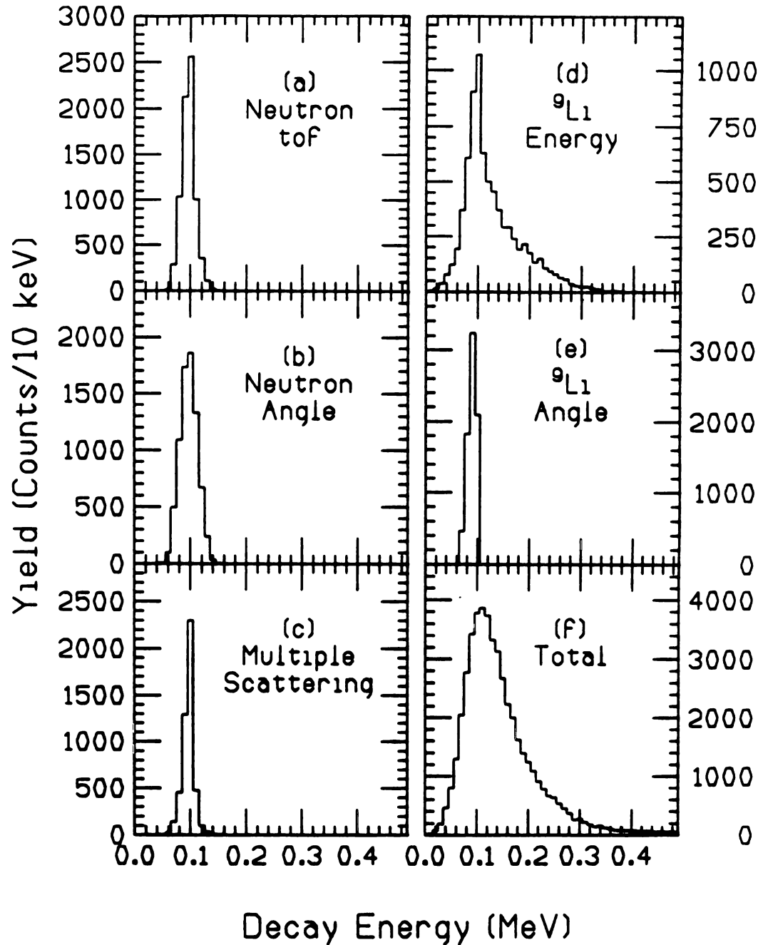
Figure B.2: Contributions to the response function for 100 keV decay energies due to neutron timing resolution, neutron angular resolution, multiple scattering in the target, energy loss in the target, and the ^9\text{Li} angular resolution. The total resolution function is shown in (f).
