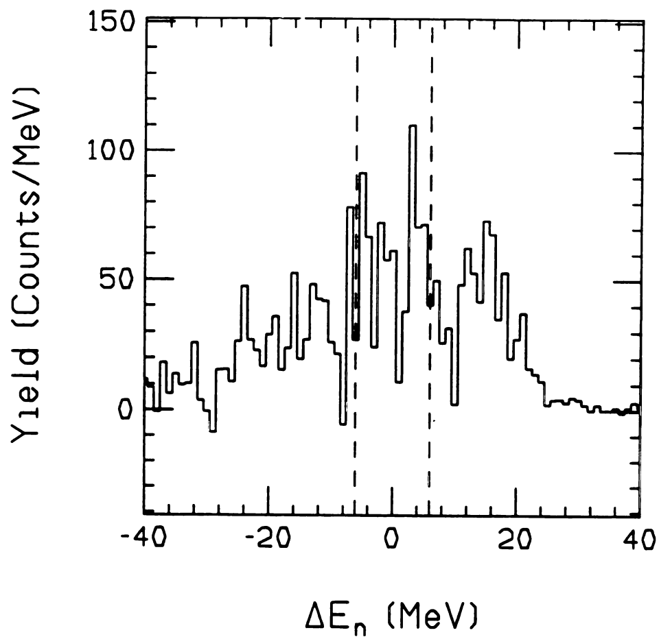
Figure D.4: \Delta E_n spectrum from the ^{11}\text{Li} data. Here, the events are a mixture of cross-talk and true coincidences. The vertical dashed lines indicate the gate used for rejecting cross-talk events.
