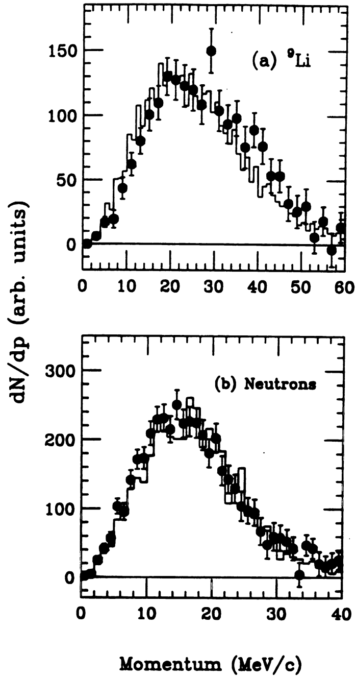
Figure 5.8: (a) {}^9\text{Li} momentum distribution determined in the {}^{11}\text{Li} rest frame. The histogram is the result of a simulation of {}^{11}\text{Li} breakup with the decay energy partitioned by a 3-body phase space distribution. (b) Neutron momentum distribution in the {}^{11}\text{Li} rest frame. The histogram is the result from the simulation.
