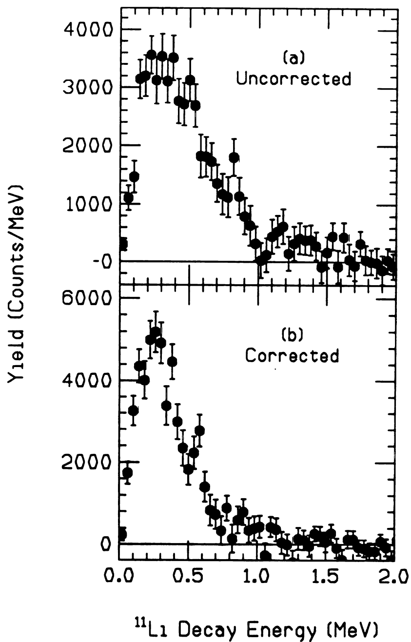
Figure C.2: (a) Decay energy spectrum before correcting for post-breakup Coulomb acceleration. (b) Decay energy spectrum after the correction.
