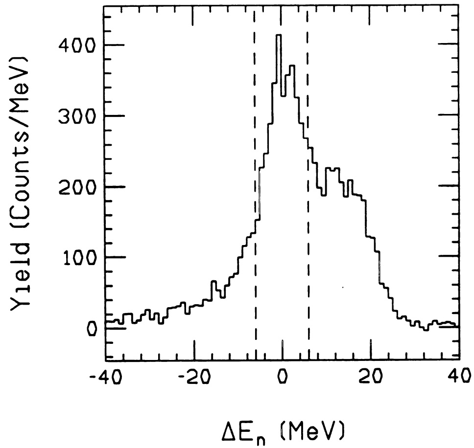
Figure D.2: \Delta E_n spectrum constructed from the pure cross talk events from the {}^7\text{Li}(p,n) reaction. The dashed vertical lines indicates the gate used for cross talk rejection in the \Delta E_n spectrum from the {}^{11}\text{Li} data
