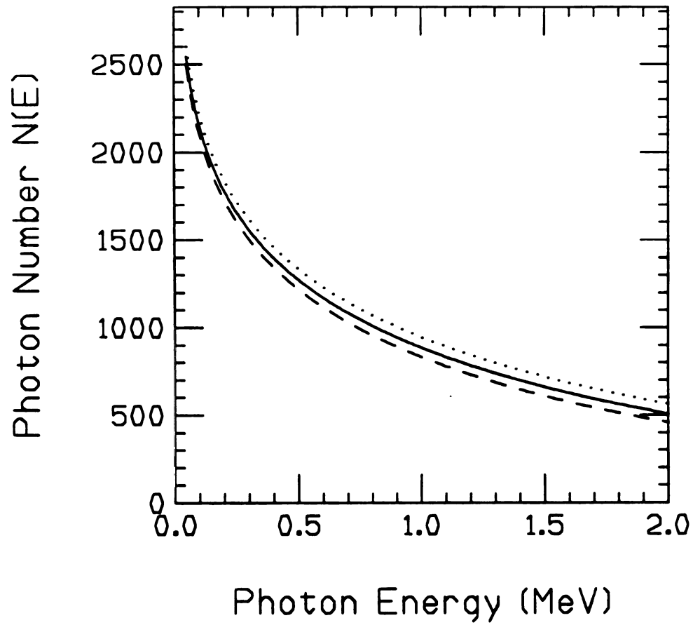
Figure E.2: Calculation of the equivalent photon spectrum using the relativistic approximation for b_{min} = 9 fm (dotted line), b_{min} = 10 fm (solid line), and b_{min} = 11 fm (dashed line).
