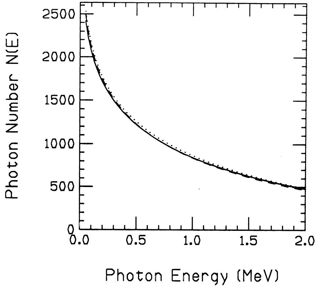
Figure E.1: Three different calculations are shown for the equivalent photon spectrum. (a) The solid line uses the expression valid for all beam projectile energies, the dotted line is the result of an approximation for intermediate energies [50] and the dashed line is the result of a relativistic approximation
