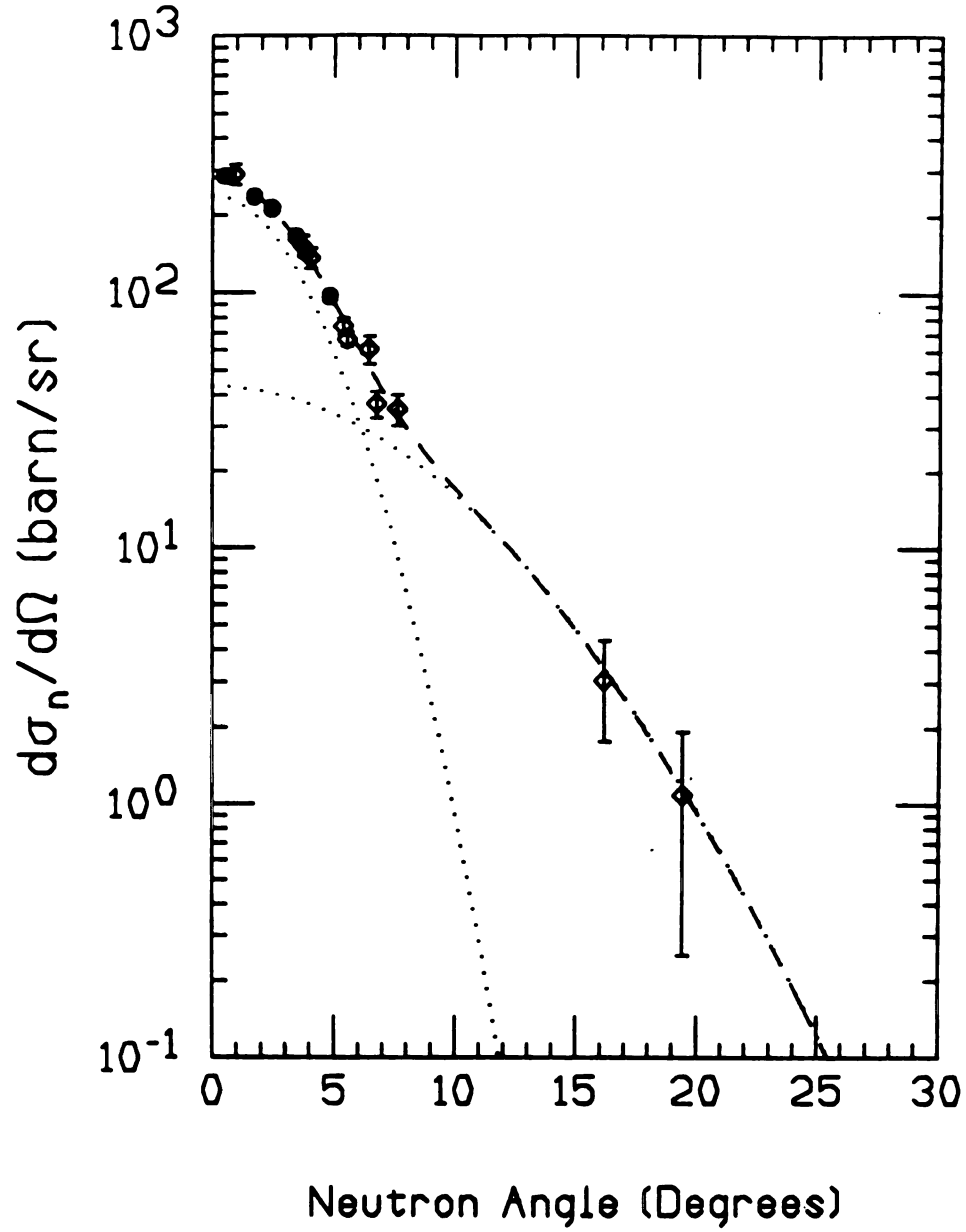
Figure 4.2: Measured angular distribution for ^{11}\text{Li} + \text{Au} at 29 MeV/nucleon taken from [32] is shown with the open diamonds. The solid points represent the angular distribution for ^{11}\text{Li} + \text{Pb} at 28 MeV/A (this work). The dotted lines are fits using narrow and broad gaussians. The dashed line is the sum of both components.
