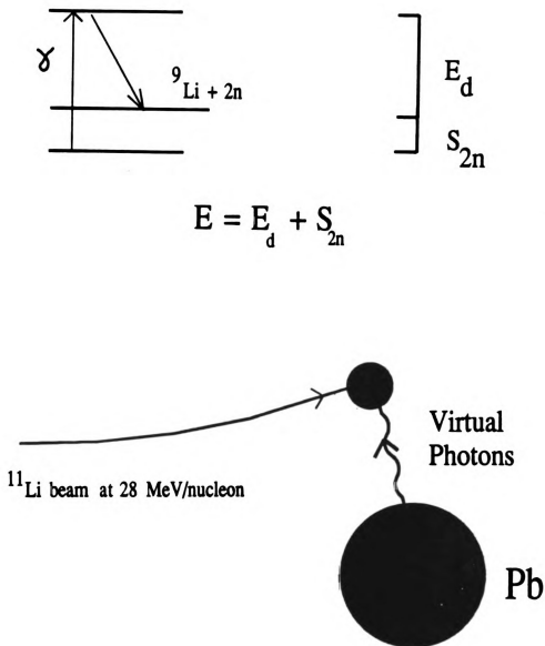
Figure 1.1: Coulomb excitation of a ^{11}\text{Li} projectile. The \text{Pb} target acts as a source of virtual photons. An excitation to the continuum followed by decay to ^9\text{Li} and two neutrons, with decay energy E_d is also shown.
