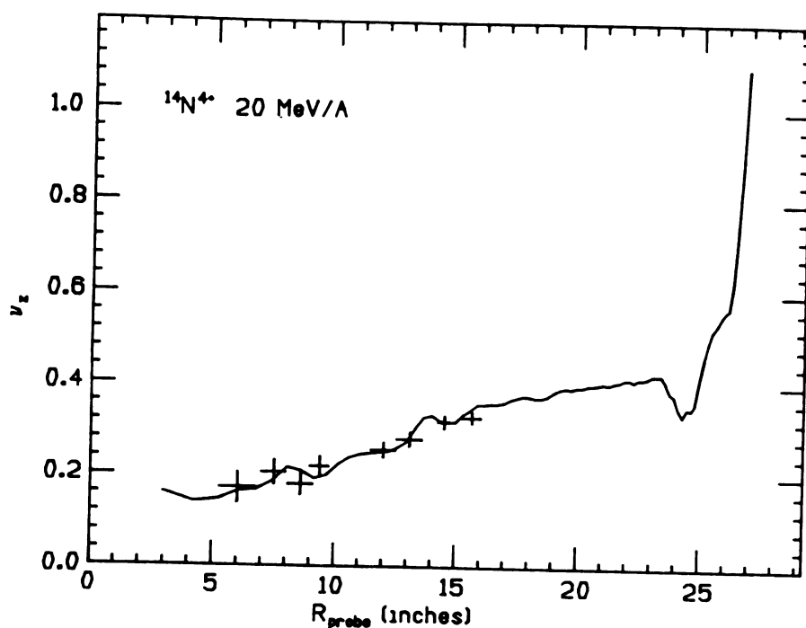
Figure 5-17. The values of the axial focusing frequency as computed by the equilibrium orbit code, and the values obtained from probe traces such as the one shown in Figure 5-14. The horizontal bars indicate the region over which the value of \nu_z was averaged. The vertical bars indicate the possible error in determining the number of turns in a precession cycle.
