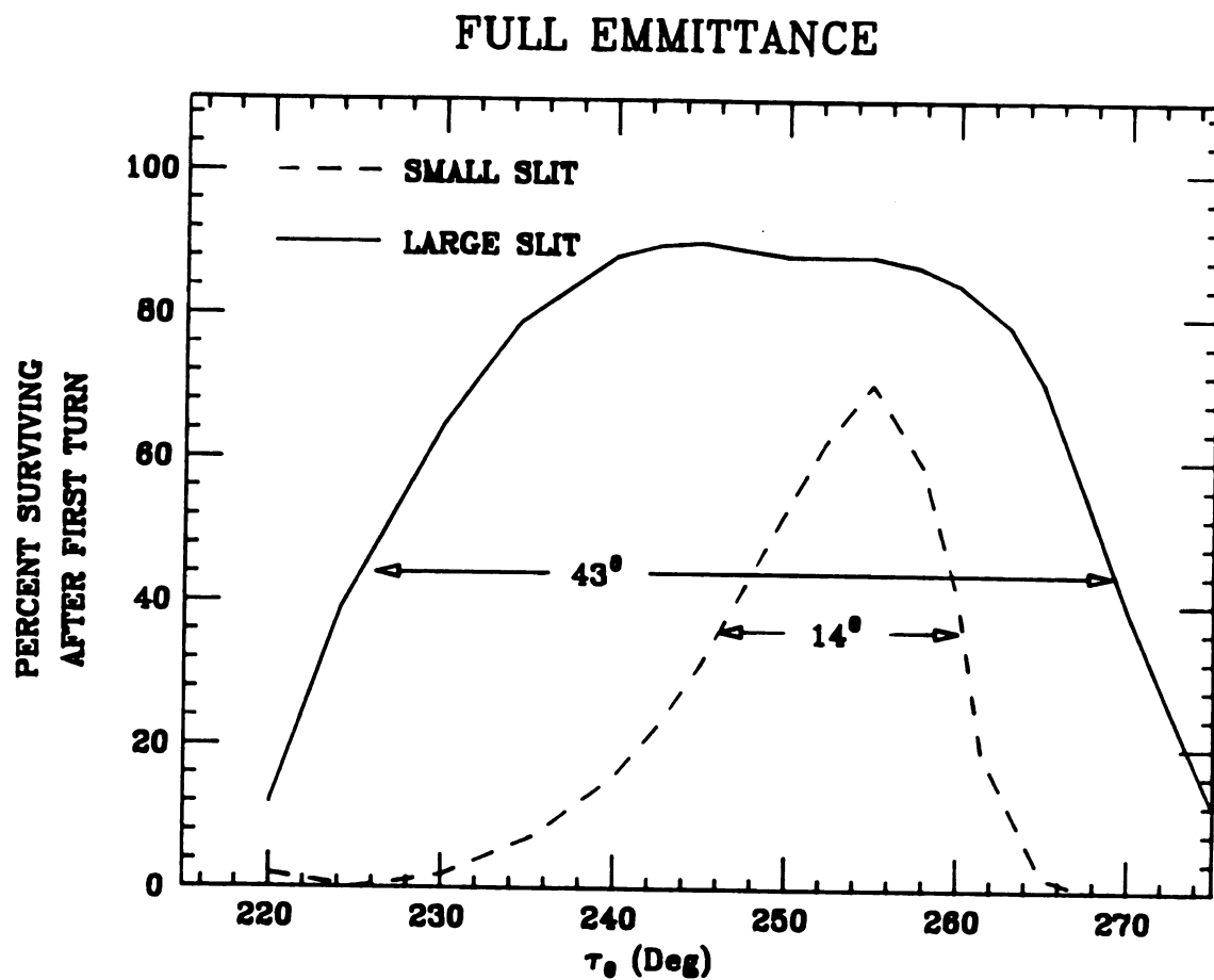
Figure 5-3. A calculation of the percent beam which survives the first turn in the cyclotron for the wide and narrow first turn slits. The inflector collimator is 4 mm in diameter.
