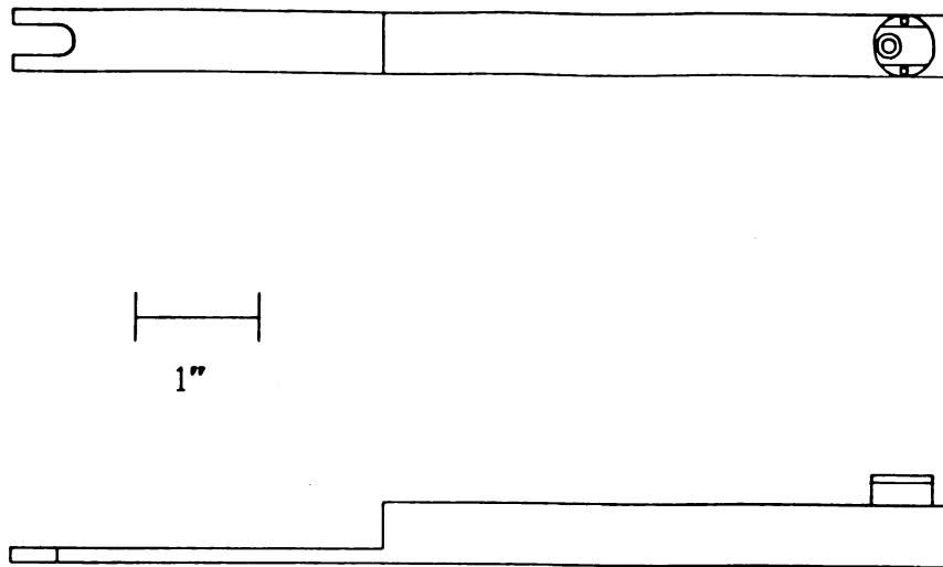
Figure 4-7. The fixture used for setting the angle of the drive. The cap on the end fits over the end of the shaft when the normal cap with pin is removed. The notch fits over the post on the center locating fixture so the rotation of the shaft is determined at either 0^{\circ} or 180^{\circ} .
