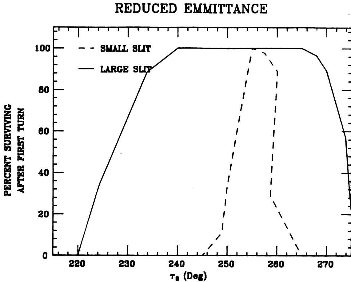
Figure 5-4. A calculation of the percent beam which survives the first turn in the cyclotron for the wide and narrow first turn slits. The inflector collimator is 1 mm in diameter.
