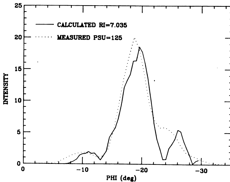
Figure 5-13. The weighted SOMA calculations are compared to the measurements for two different locations of the upper slit. Note the relative intensities of the peaks. These calculations assumed 100\pi mm-mrad initial emittance
