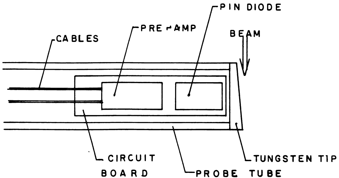
Figure 4-13. A schematic drawing of the phase probe. The PIN diode is used to detect gamma rays produced when the beam strikes the probe tip. The small size of the diode and amplifier allows it to be located near the probe tip so the count rates are high and the source is distinct from the background.
