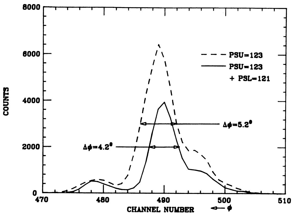
Figure 5-11. The phase widths at extraction with one slit inserted, and the combination of two slits. The extracted current is reduced by a factor of two when the second slits is inserted.
