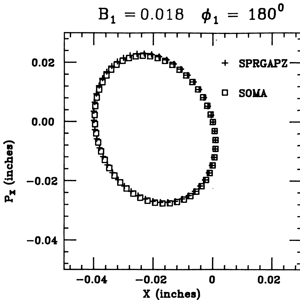
Figure 2-8. A sample precession cycle as calculated by SPRGAPZ and SOMA for a field with a first harmonic. The orbit began on the EO.
