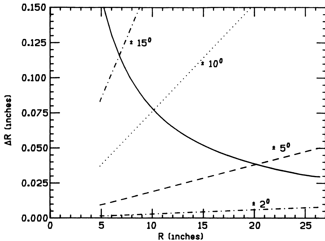
Figure 3-1. Plots of simple estimates of the turn separation and turnwidths associated with different phase widths. The turn separation (solid curve) is estimated using \Delta R = \Delta E \cdot R / 2 \cdot E while the full width of a turn with a given \Delta\theta is found using \Delta R = (\Delta\theta)^2 \cdot R / 4 .
