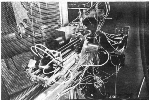
Figure 4-10. A photo of the new drive installed on the cyclotron. In this photo the drive is in the 'running' position and a probe has been installed.
