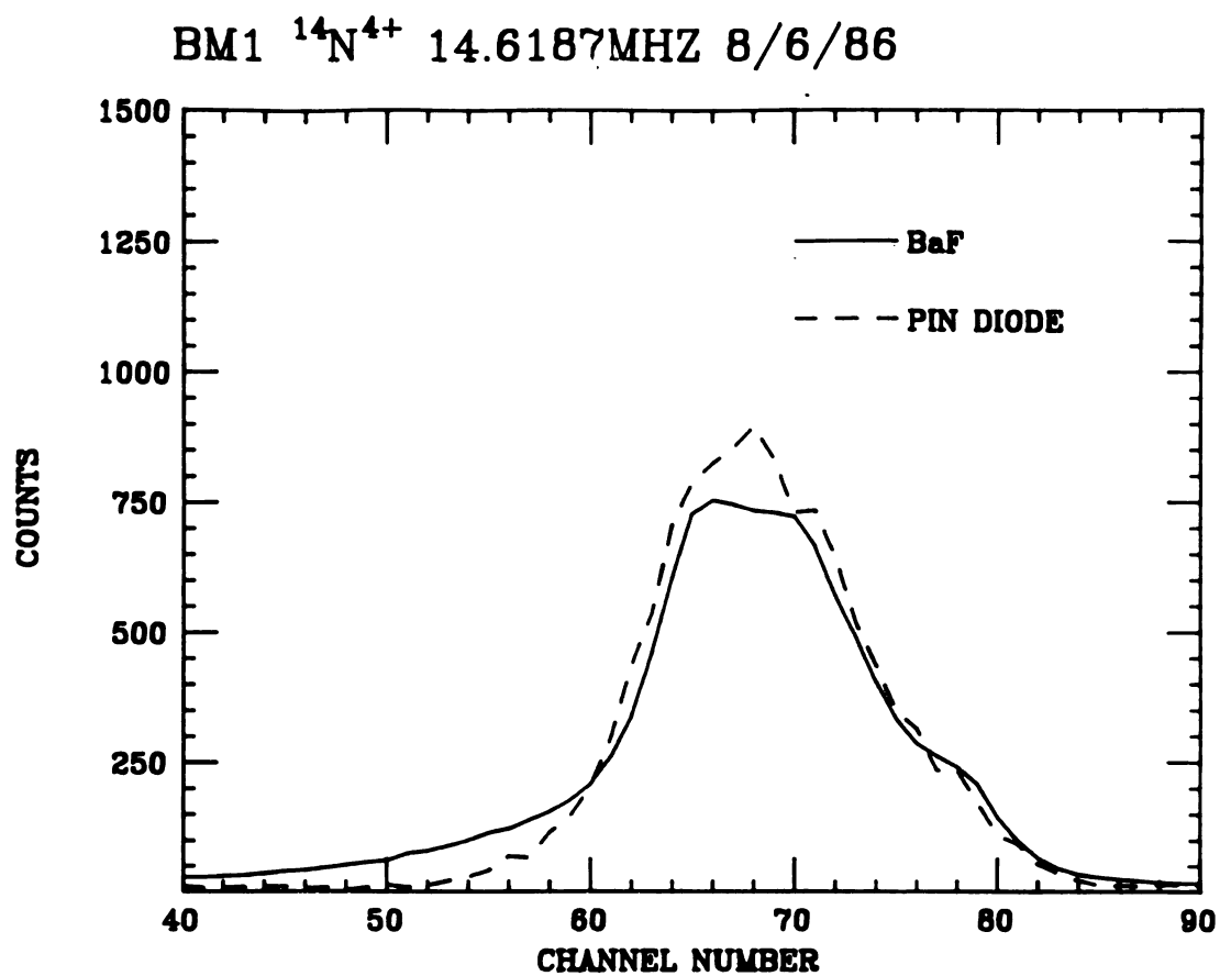
Figure 4-15. A comparison between the PIN diode and a BaF detector. Both detectors measured the same beam, which was striking beam stop 1. The measured beam widths are very similar.
