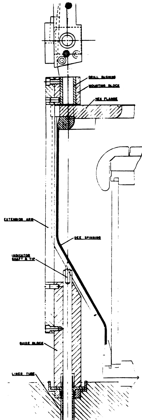
Figure 4-6. The fixture used for locating the hole in the dee stem spinning. The other end of the indicator shaft was at the median plane so it could be tapped with a hammer to mark the spinning with the sharpened point. The drill bushings provided alignment of the clearance hole and the two threaded holes for mounting the air cylinder on the hex flange.
