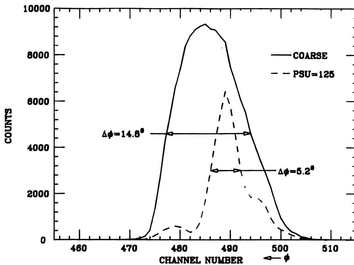
Figure 5-10. A comparison of the phase width at extraction with and without the upper slit. In both cases the narrow first turn slit is present.
