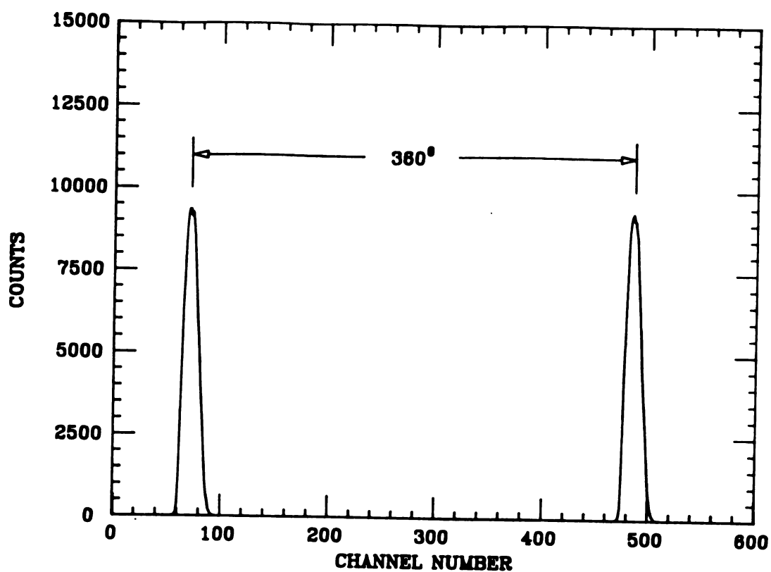
Figure 4-14. A typical spectrum of intensity versus time, as measured with the gamma probe. Notice that the divide by two of the RF stop signal causes all features to appear 360^\circ apart
