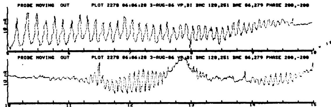
Figure 5-5. A differential probe trace, taken with the narrow first turn slit in place. The cyclotron was tuned for good extraction.
