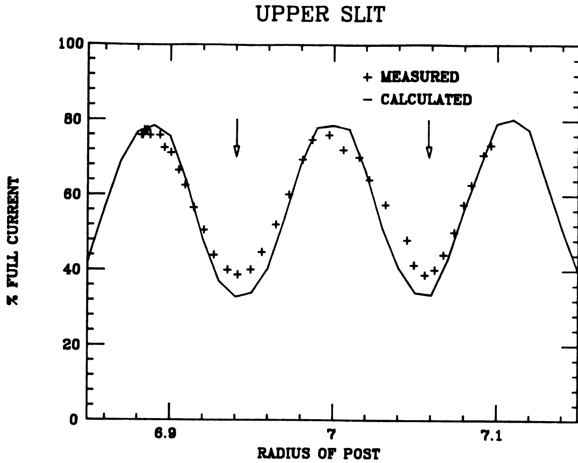
Figure 5-7. The current intercepted by the upper slit as a function of its radial position. The calculation values were obtained with the code SOMA.
