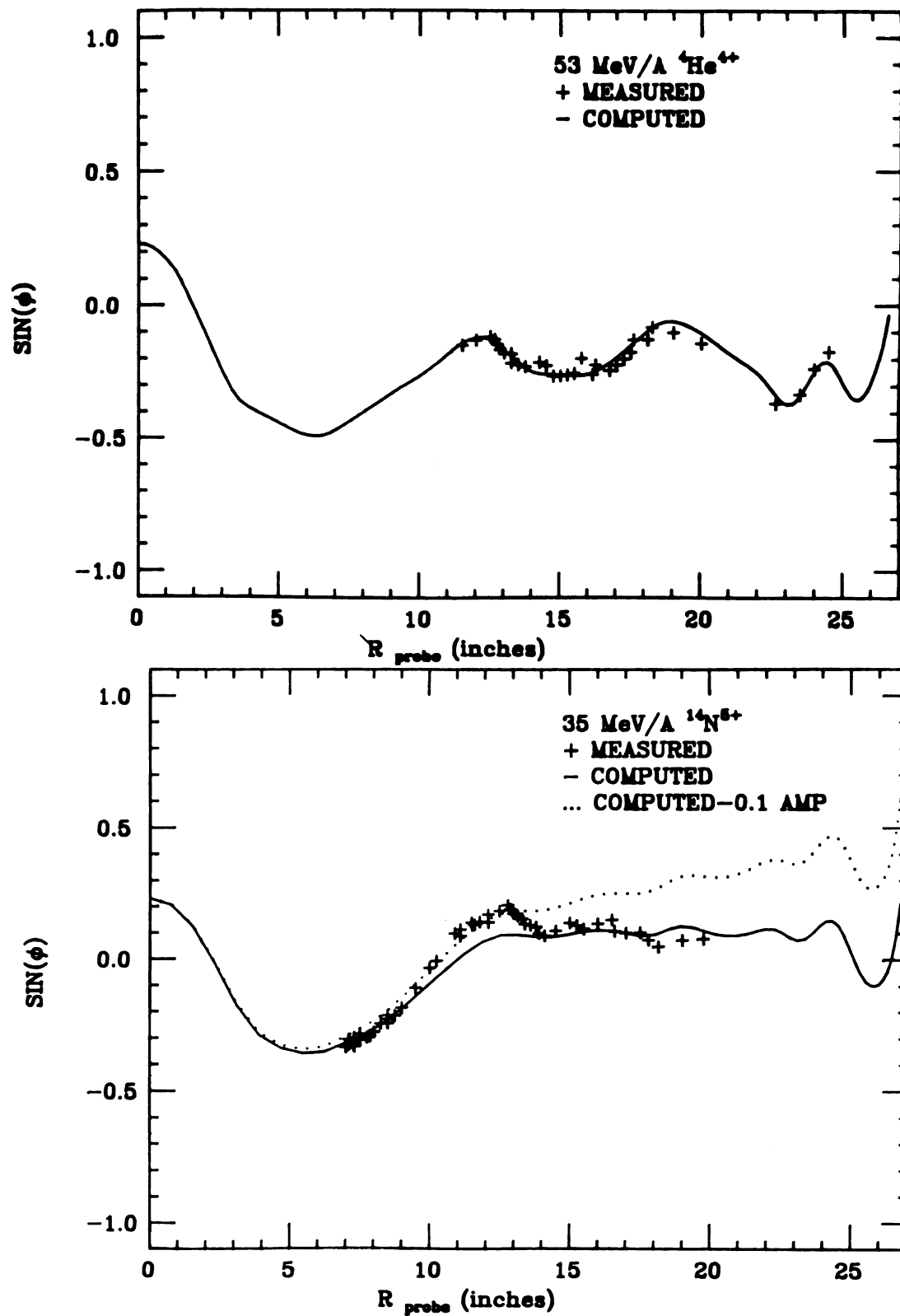
Figure 5-1. The calculated and measured phase curves for two different magnetic fields. The dashed curve for the \text{N}^{5+} case is the calculated phase curve when the mail coil currents are changed by 0.1 Amps.
