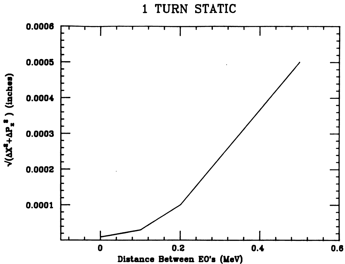
Figure 2-5. The differences between SOMA and SPRGAPZ when the spacing between stored values is changed. The initial displacement was \approx 0.03'' and run for one turn without acceleration.
