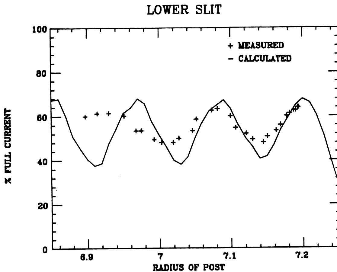
Figure 5-8. The current intercepted by the lower slit as a function of its radial position. The calculation values were obtained with the code SOMA. The poor agreement at lower radii is due to an encoder mal function.
