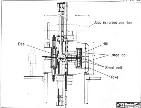
Figure 1-1. Vertical section of the K500 cyclotron.
