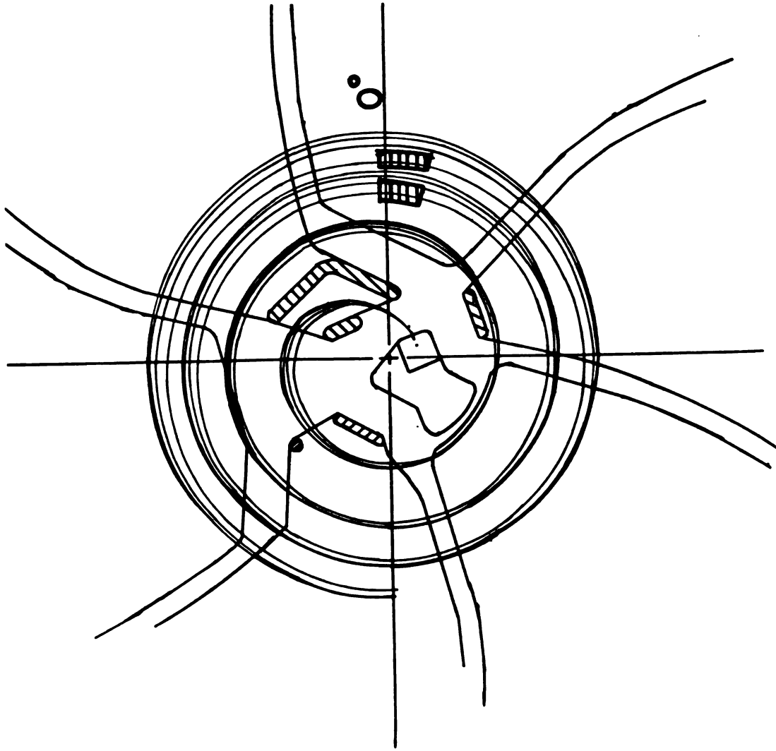
Figure 3-3. Electrode structure for the K500 first harmonic central region using a PIG source. Four orbits are shown corresponding to starting times (from outermost at \theta=0^\circ to innermost), \tau_0=230, 240, 250 , and 260 degrees. The peak electric field between the source and puller is achieved at \tau_0=270 . A slit is located on the 0^\circ hill extension of the center plug allowing easy installation and removal. This slit removes all particles whose starting times do not fall between 230 and 250 degrees.
