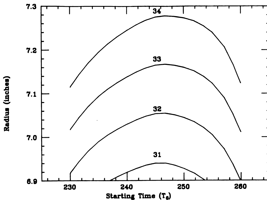
Figure 3-2 The radius of the central ray, shown as a function of starting time, for four successive turns. Note the typical horse-shoe shape resulting from the \cos(\theta) dependence of the energy gain.
