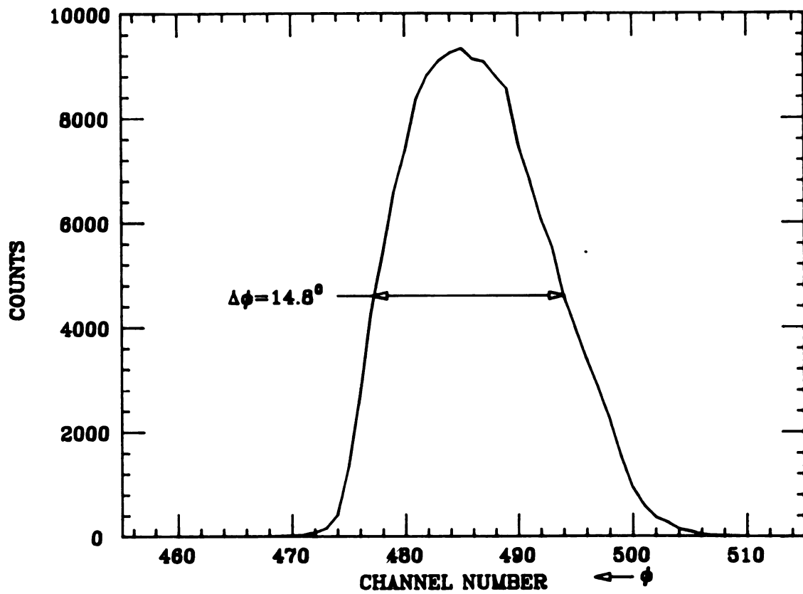
Figure 5-2. The phase width of the internal beam as measured with the gamma probe at extraction radius when the narrow first turn slit is installed
