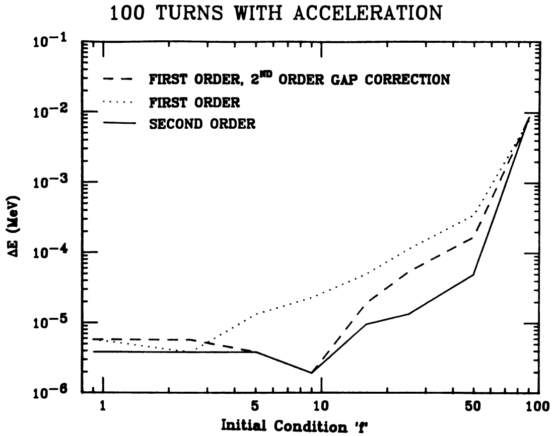
Figure 2-7. The difference in energy for rays for the same rays shown in Figure 2-6.
