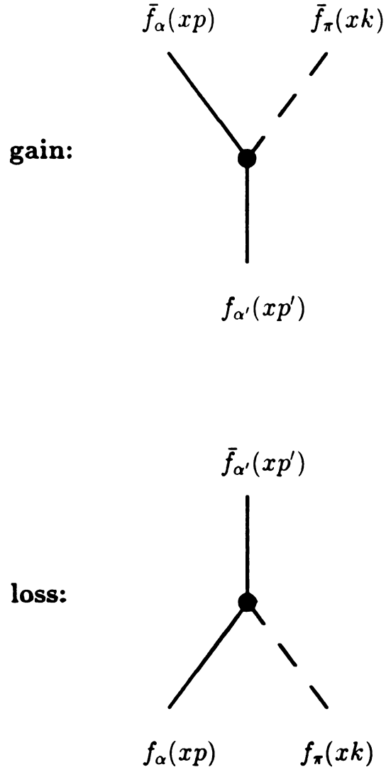
Figure 2.2: Diagrammatic representation of the gain and loss terms responsible for changing the pion phase-space distribution f_\pi(x, k) as a result of baryon-pion collisions.
