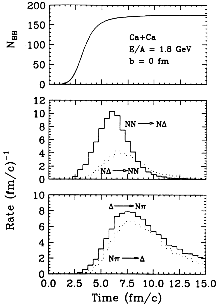
Figure 4.1: Upper figure: Accumulation of the total number of baryon-baryon collisions in the reaction of Ca+Ca at E/A = 1.8 \text{ GeV} and impact parameter b = 0 \text{ fm} . Lower figure: Time evolution of the reaction rate for the specified processes in the same reaction.
