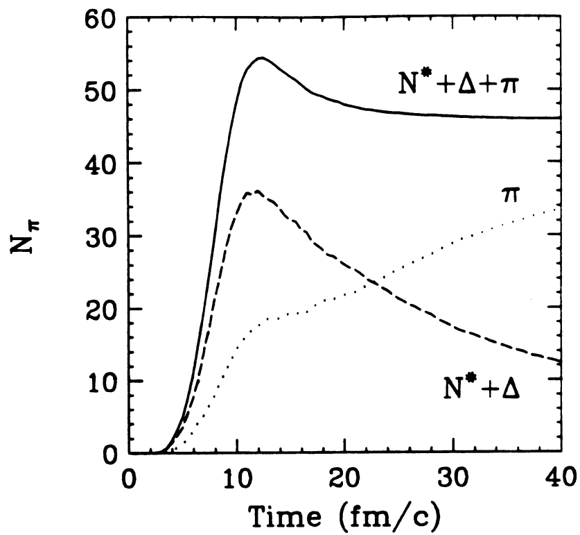
Figure 4.2: Time evolution of the population of free pions, \Delta 's and N^* 's in central collisions of La + La at E/A = 1350 MeV.
