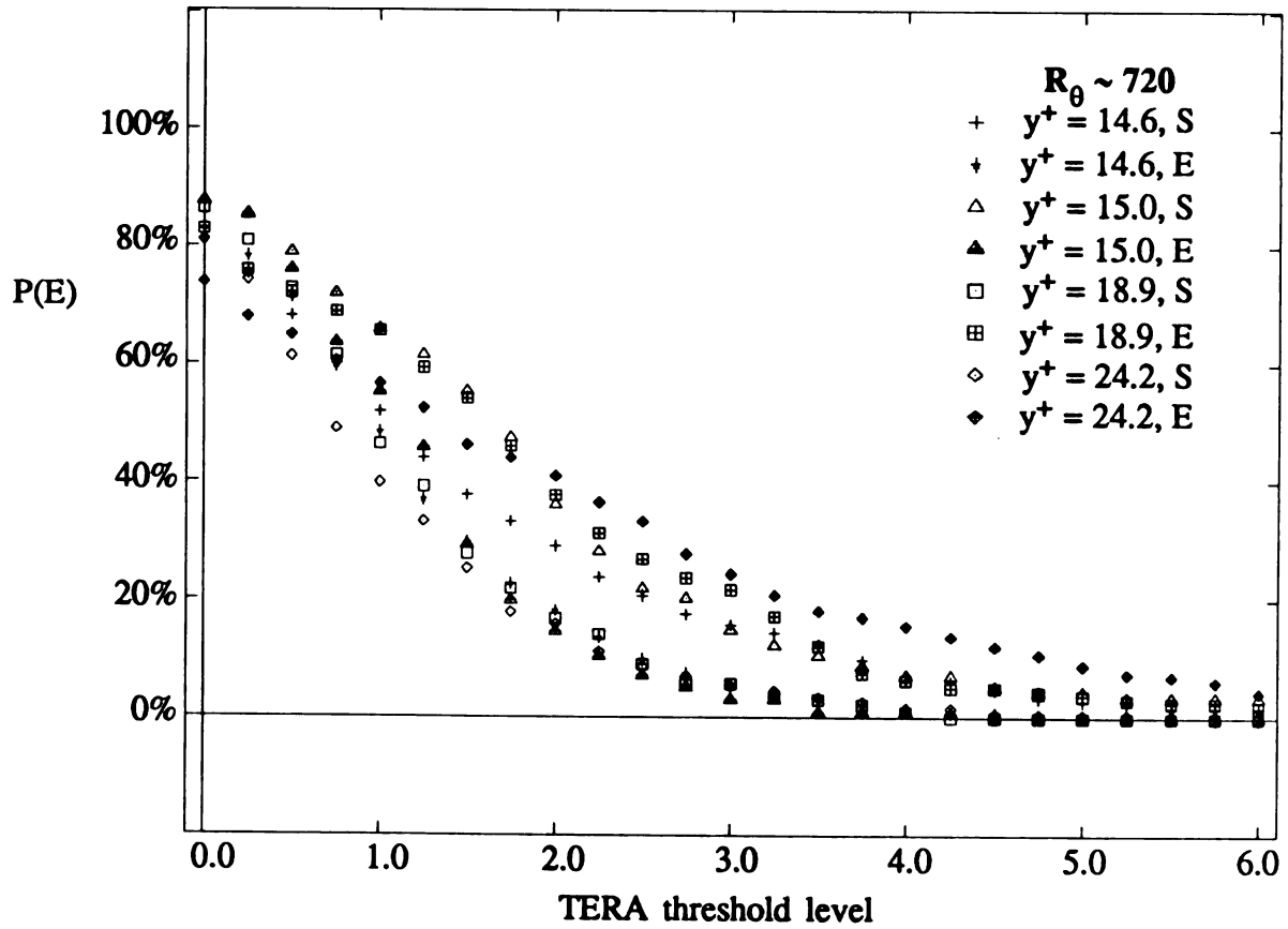
Figure 4.3.5 P(E): Probability of a TERA Detection Occurring During an Inner-Region Visual Detection vs. Threshold
