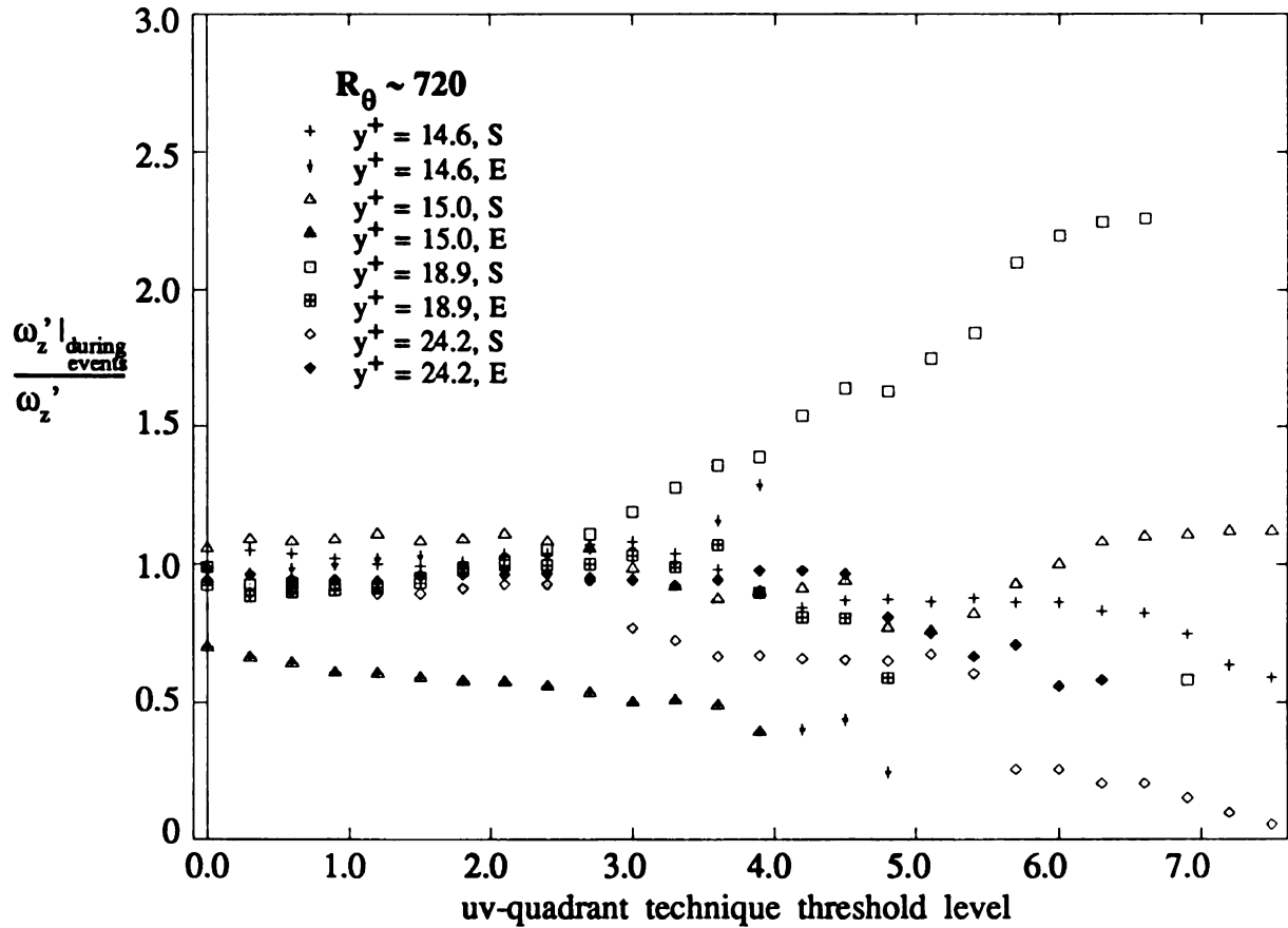
Figure 3.4.28 RMS \omega_z During uv-quadrant Events Normalized by \omega_z' vs. Threshold (Inner-region data)
