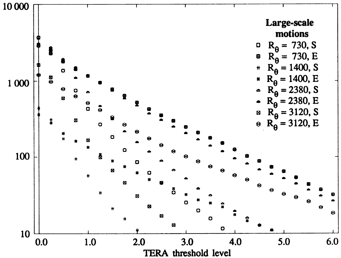
Figure 3.5.9 Total TERA Event Time (Mixed Scaling) vs. Threshold (LSM data set)
