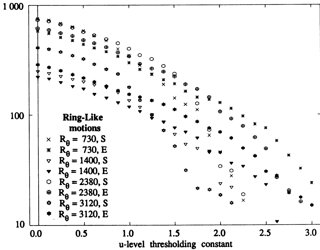
Figure 3.6.8 Total u-level Event Time (Mixed Scaling) vs. Threshold (RLM data set)
