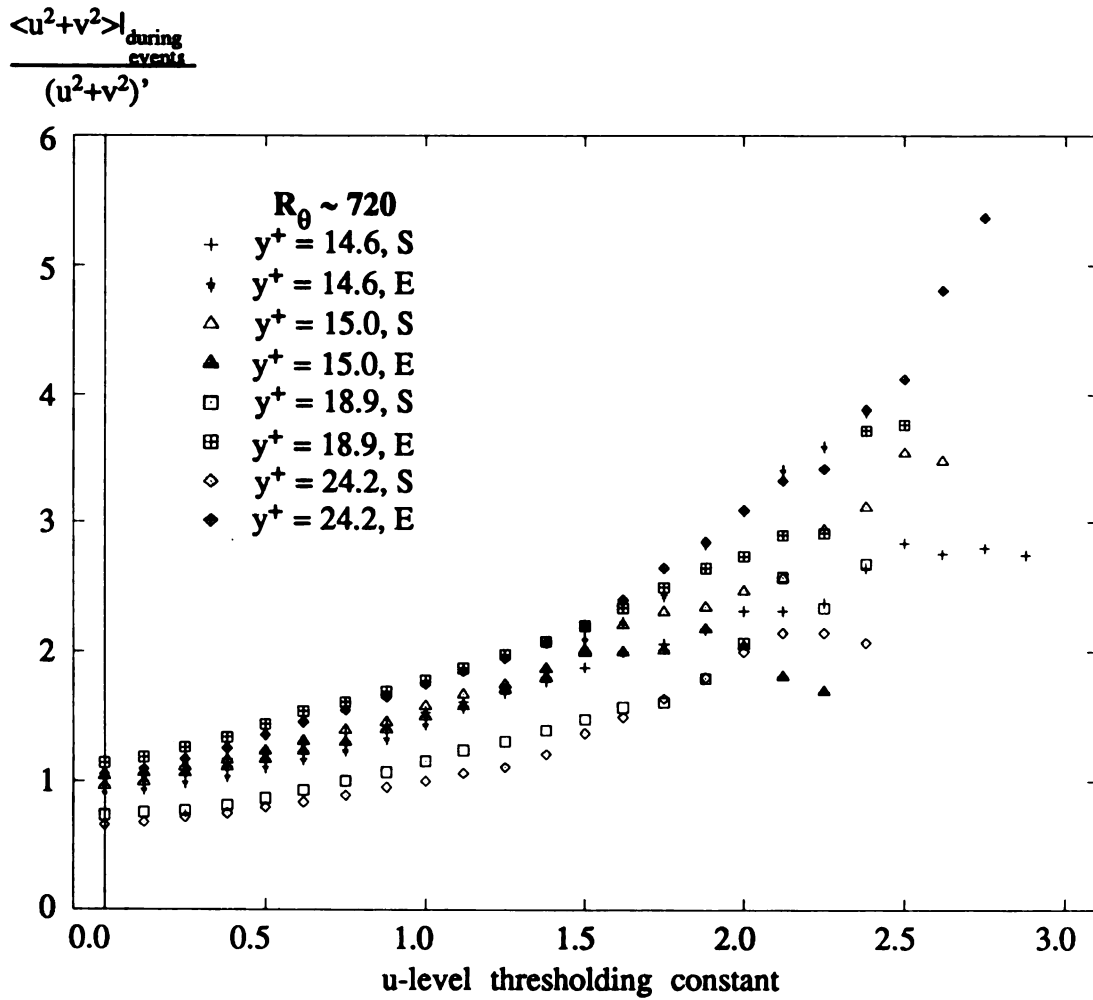
Figure 3.6.30 Average TKE During u-level Events Normalized by TKE' vs. Threshold (Inner-region data)
