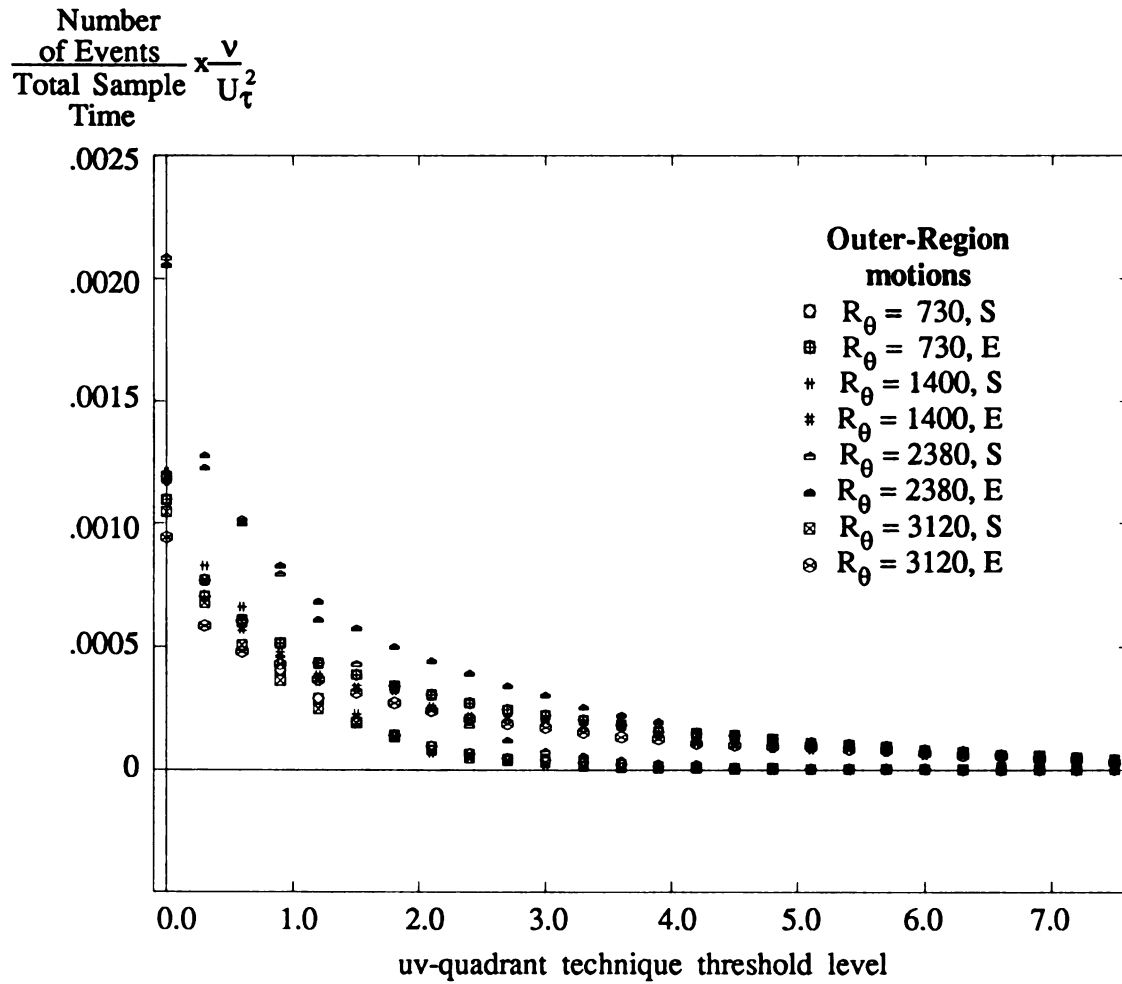
Figure 3.4.16 Inner-scaled uv-quadrant Event frequency vs. Threshold level (LSM data set)
