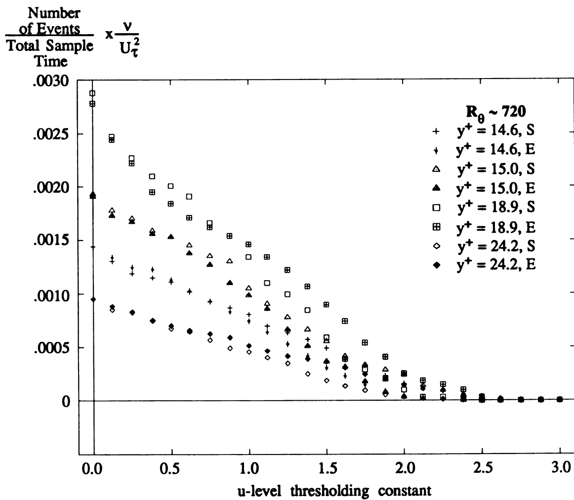
Figure 3.6.13 Inner-scaled u-level Event frequency vs. Threshold level (Inner-region data)
