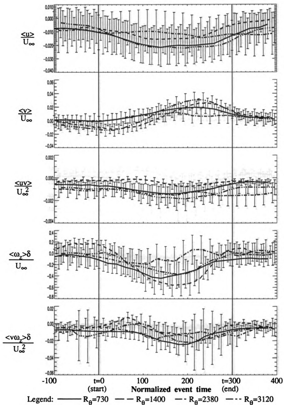
Figure 3.2.4 Outer-scaled RLM ejection ensembles. Error bars indicate 25% of an ensemble's standard deviation at each point in time
