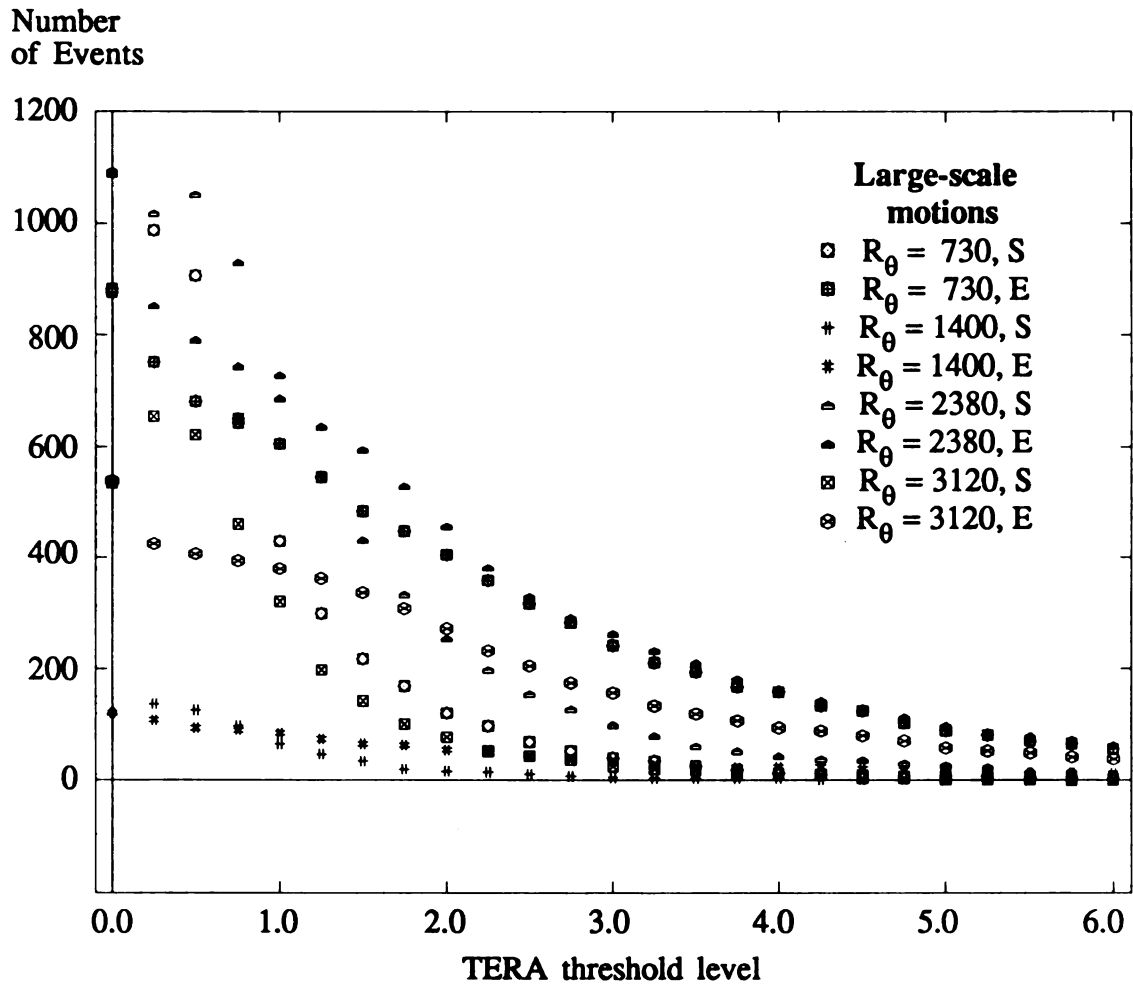
Figure 3.5.3 Number of TERA Events vs. Threshold level (LSM data set)
