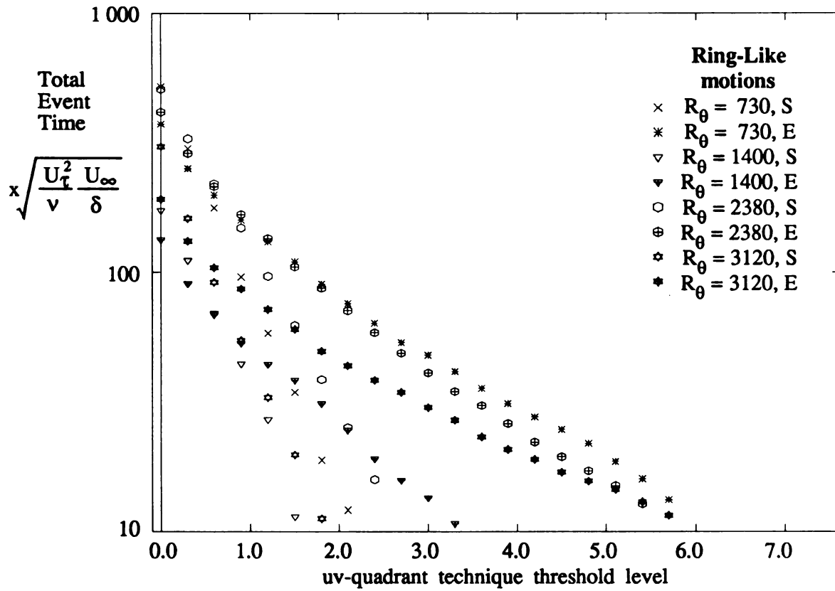
Figure 3.4.8 Total uv-quadrant Event Time (Mixed Scaling) vs. Threshold (RLM data set)
