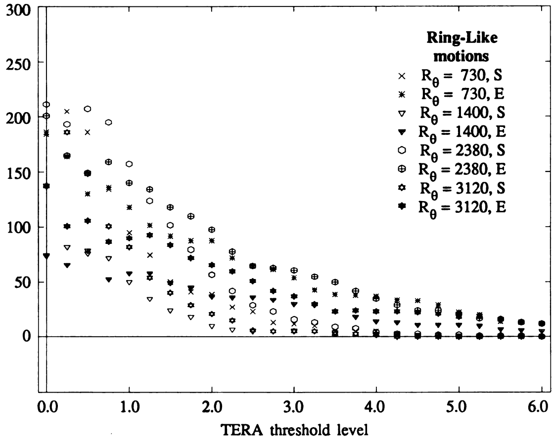
Figure 3.5.2 Number of TERA Events vs. Threshold level (RLM data set)
