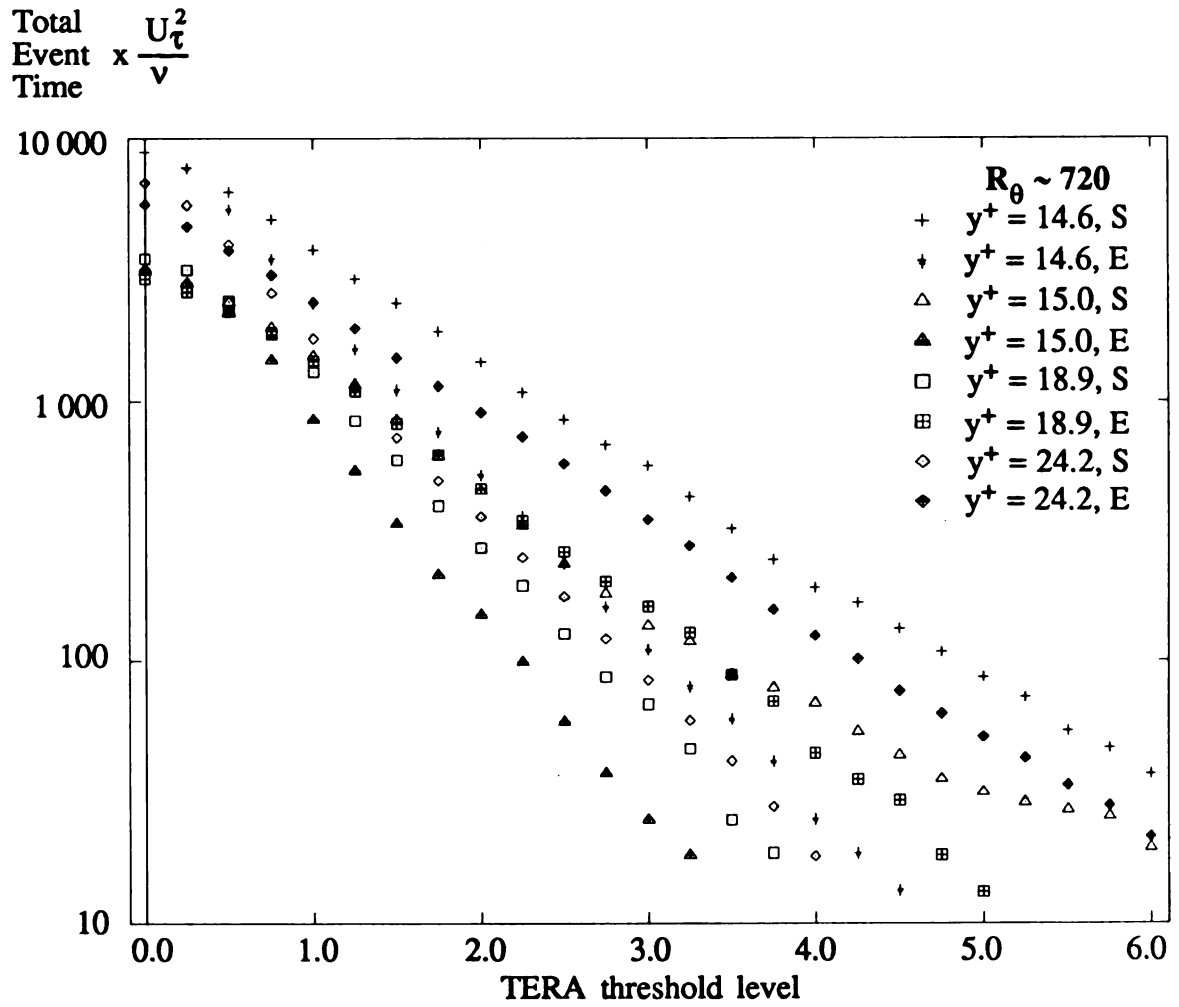
Figure 3.5.4 Inner-Scaled Total TERA Event Time vs. Threshold (Inner-region data)
