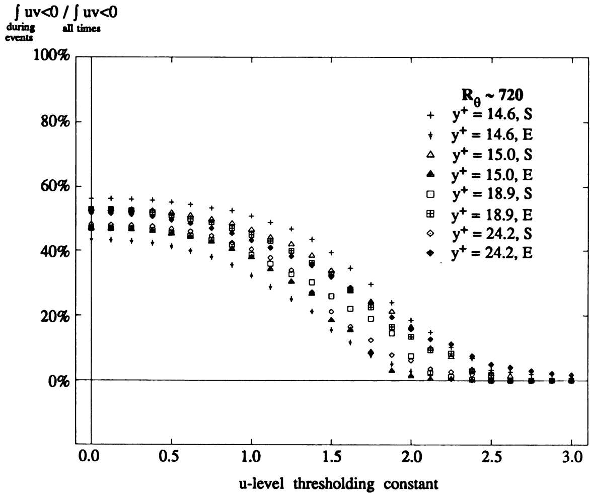
Figure 3.6.26 Percent Reynolds Stress "captured" during u-level events vs. Threshold (Inner-region data)
