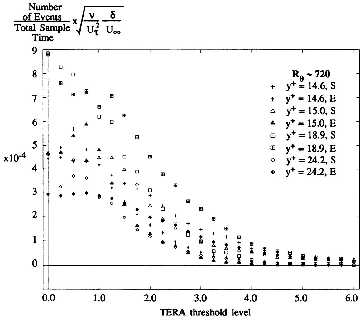
Figure 3.5.14 TERA Event frequency (Mixed-scaling) vs. Threshold level (Inner-region data)
