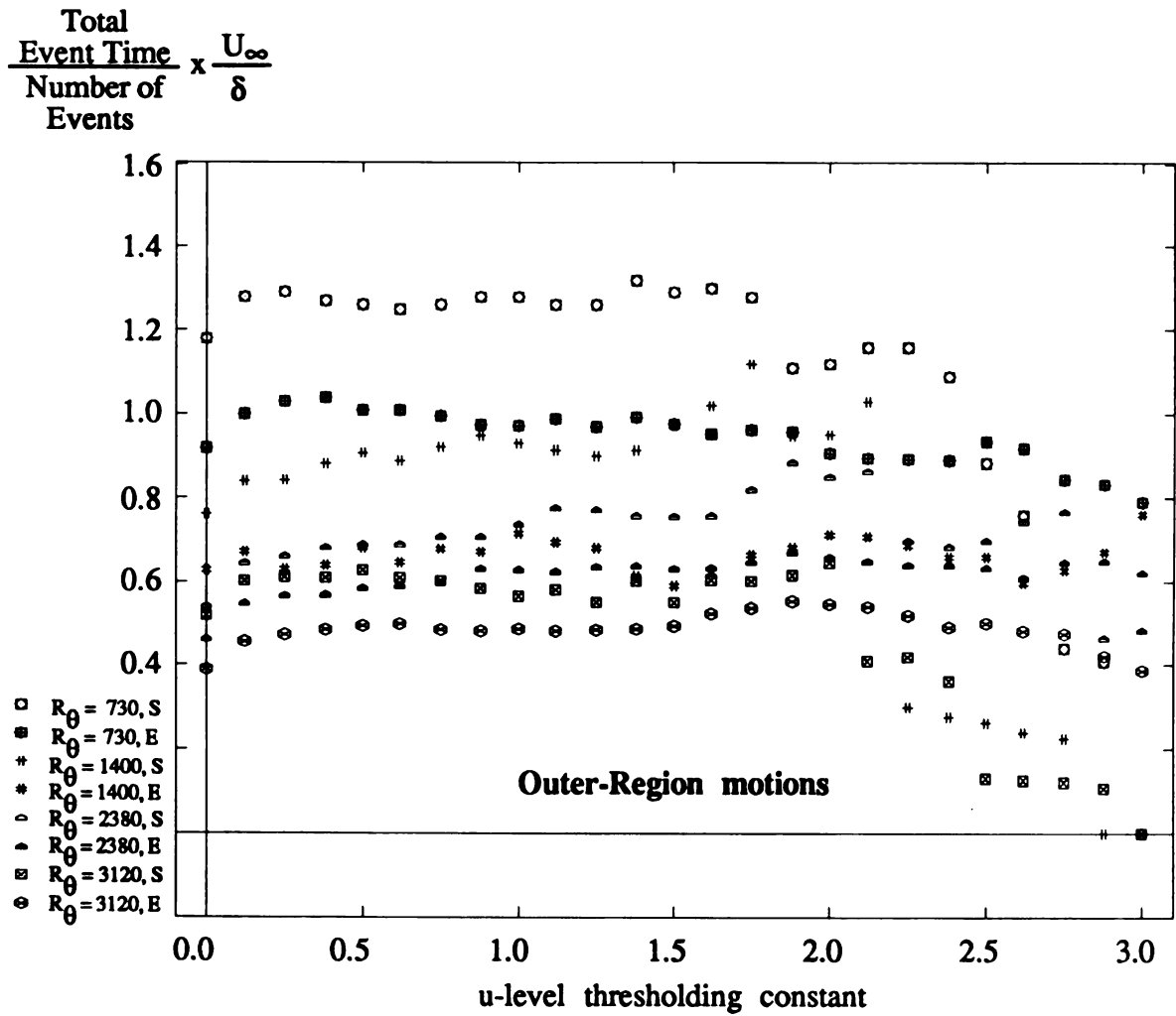
Figure 3.6.24 Outer-Scaled Average u-level Event Length vs. Threshold (LSM data set)
