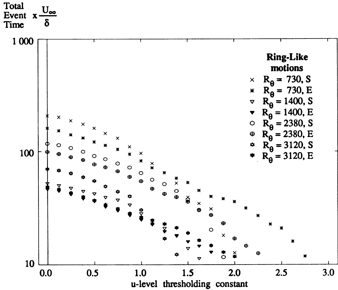
Figure 3.6.11 Outer-Scaled Total u-level Event Time vs. Threshold (RLM data set)
