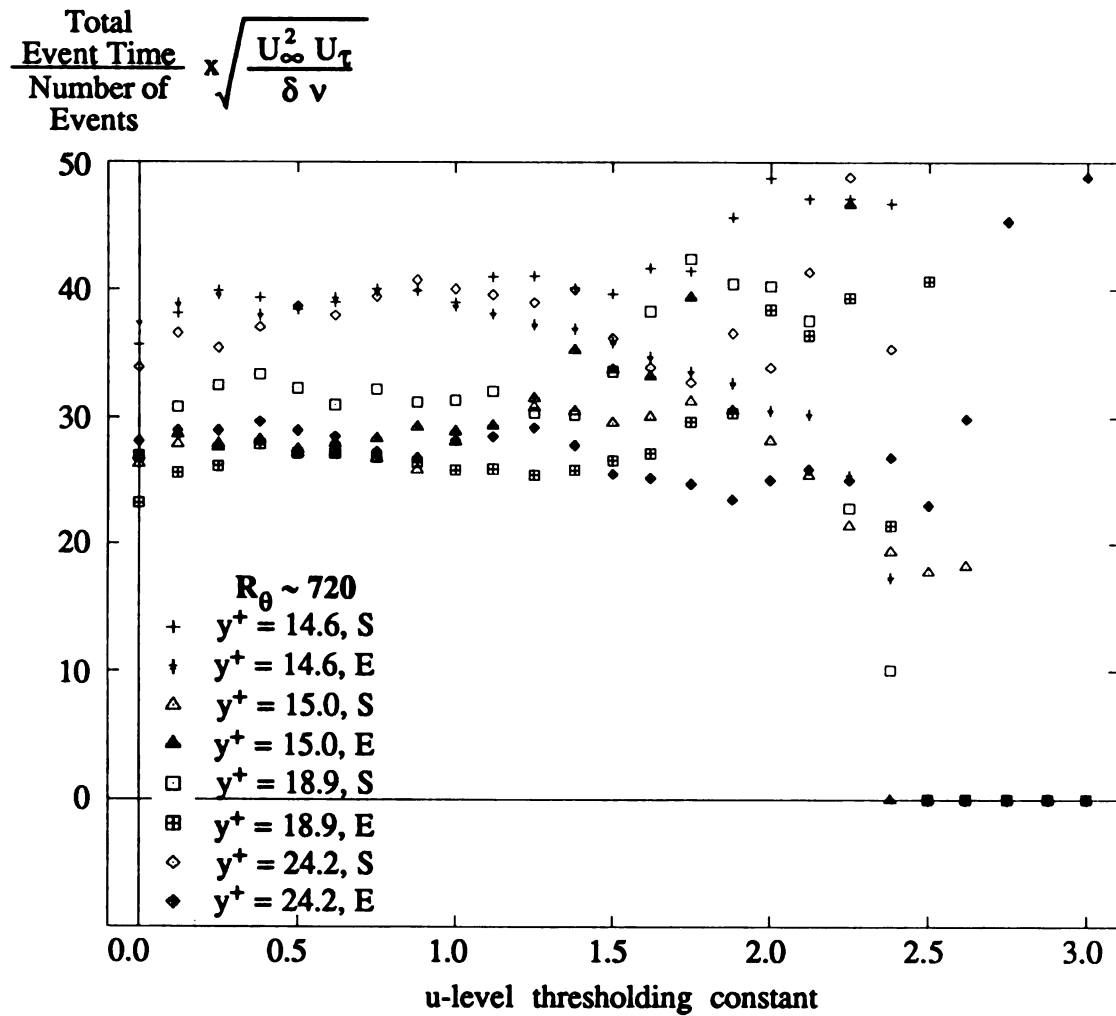
Figure 3.6.20 Average u-level Event Length (Mixed Scaling) vs. Threshold (Inner-region data)
