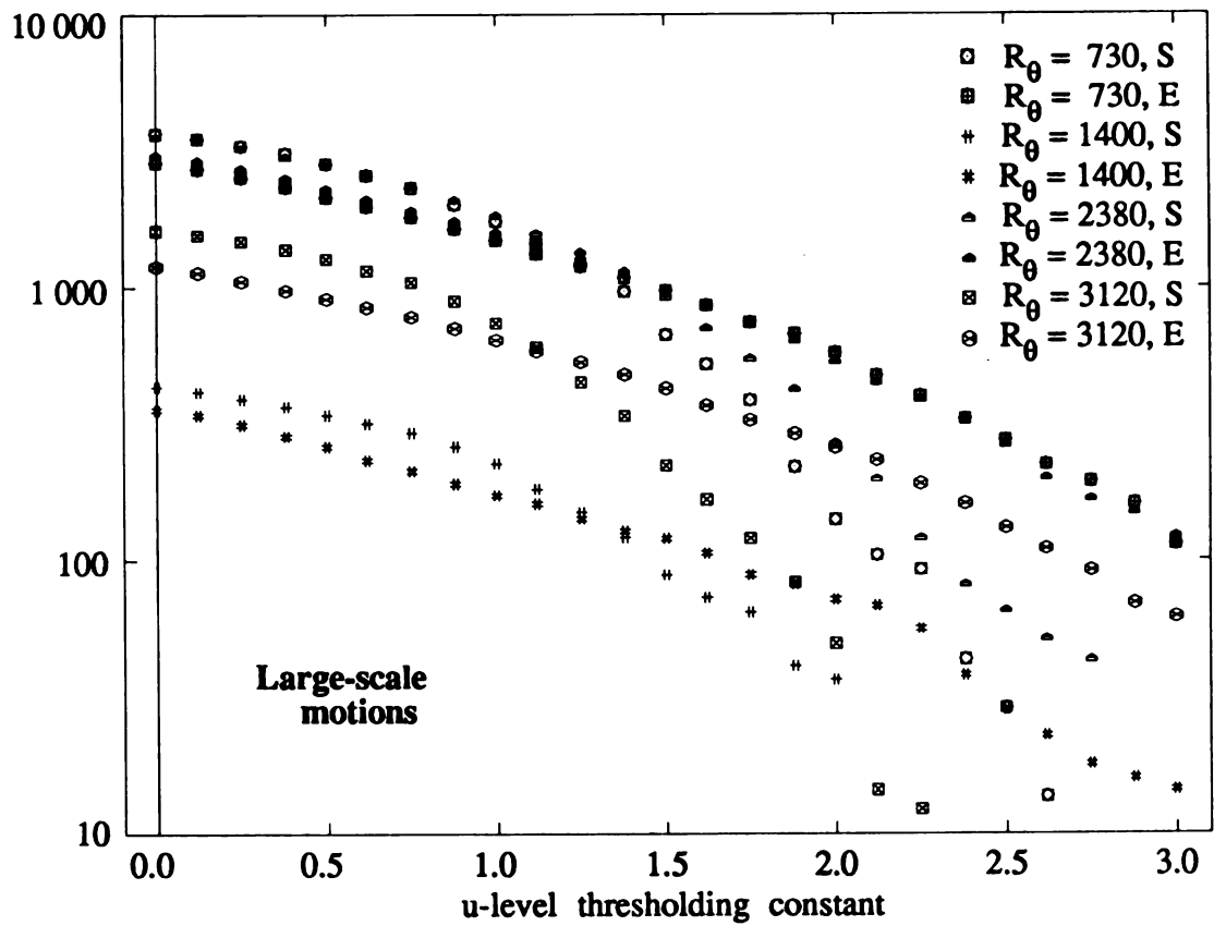
Figure 3.6.9 Total u-level Event Time (Mixed Scaling) vs. Threshold (LSM data set)
