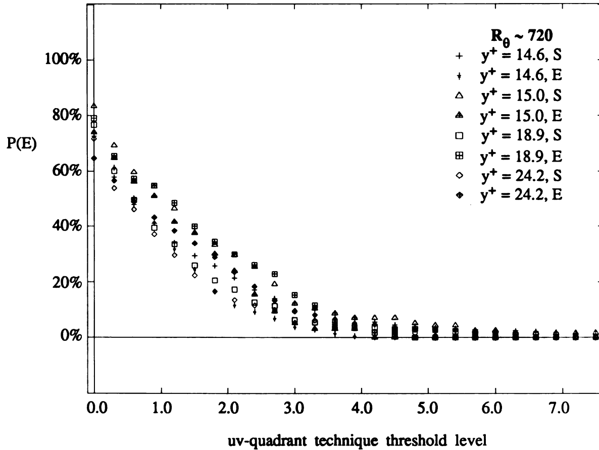
Figure 4.3.4 P(E): Probability of a uv-quadrant Detection Occurring During an Inner-Region Visual Detection vs. Threshold
