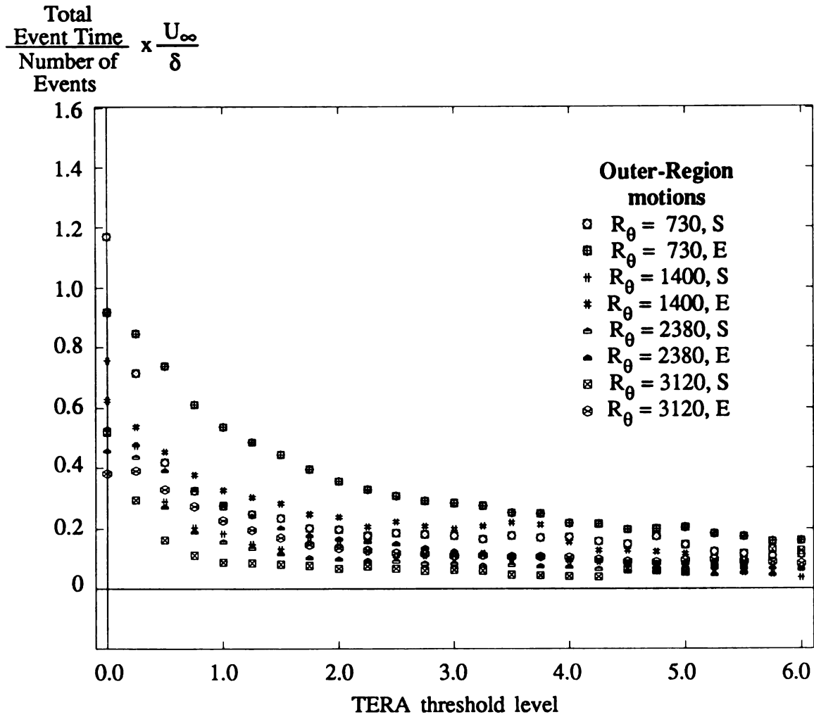
Figure 3.5.24 Outer-Scaled Average TERA Event Length vs. Threshold (LSM data set)
