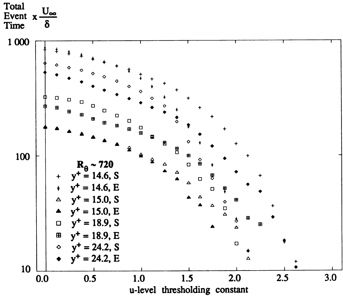
Figure 3.6.10 Outer-Scaled Total u-level Event Time vs. Threshold (Inner-region data)
