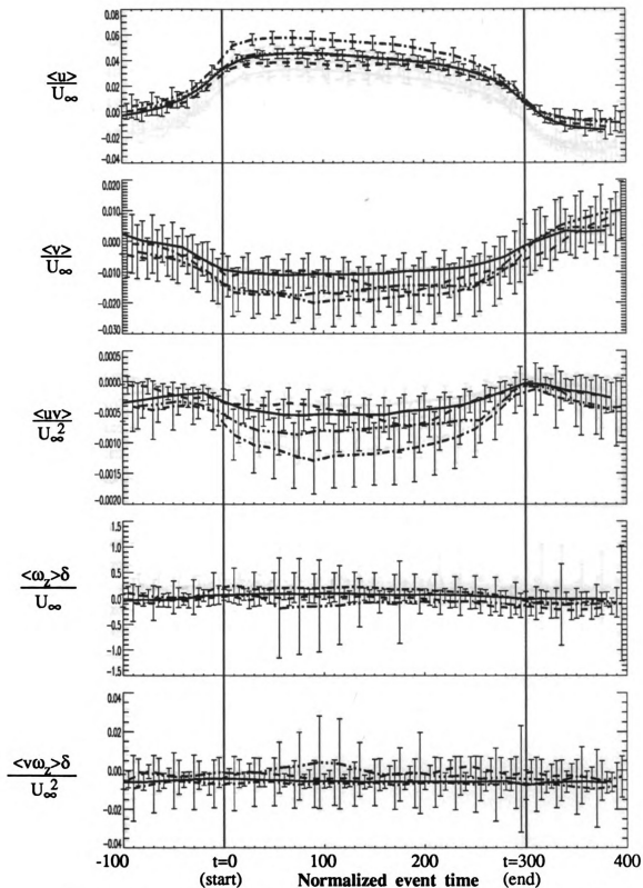
Figure 3.6.32 Outer-scaled u-level sweep ensembles. Error bars indicate 25% of an ensemble's standard deviation about each point in time
