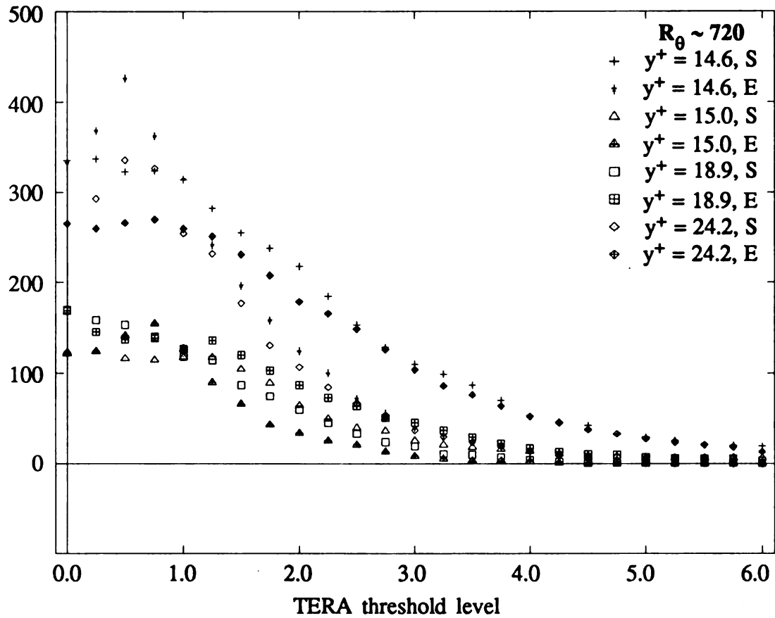
Figure 3.5.1 Number of TERA Events vs. Threshold level (Inner-region data)
