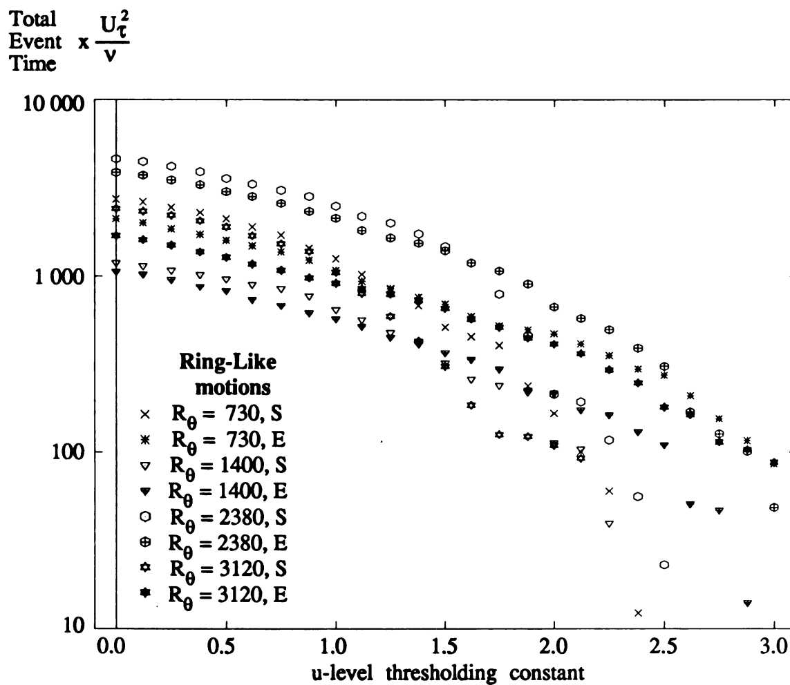
Figure 3.6.5 Inner-Scaled Total u-level Event Time vs. Threshold (RLM data set)
