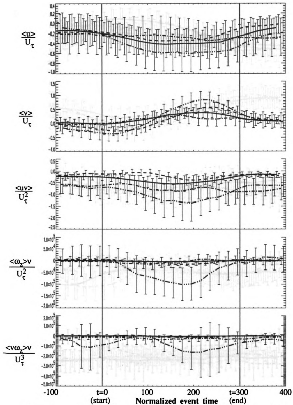
Figure 3.2.6 Inner-scaled RLM ejection ensembles. Error bars indicate 25% of an ensemble's standard deviation at each point in time
