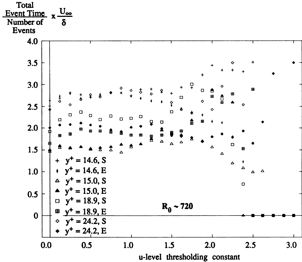
Figure 3.6.21 Outer-Scaled Average u-level Event Length vs. Threshold (Inner-region data)
