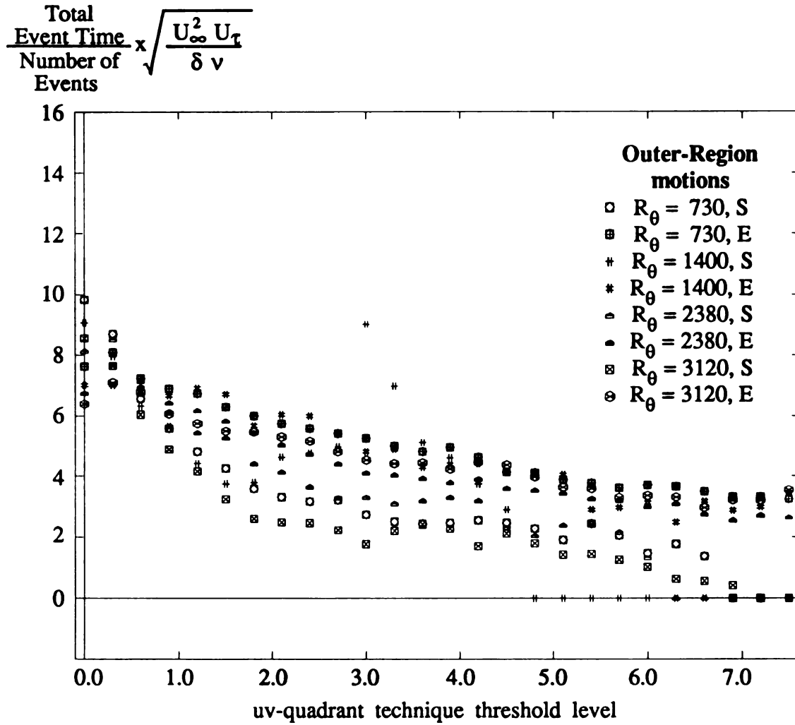
Figure 3.4.23 Average Event uv-quadrant Length (Mixed Scaling) vs. Threshold (LSM data set)
