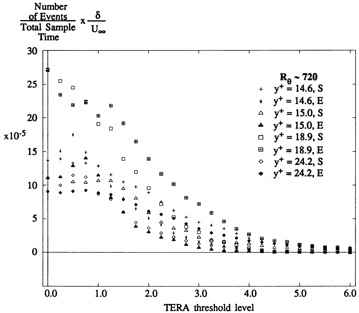
Figure 3.5.15 Outer-scaled TERA Event frequency vs. Threshold level (Inner-region data)
