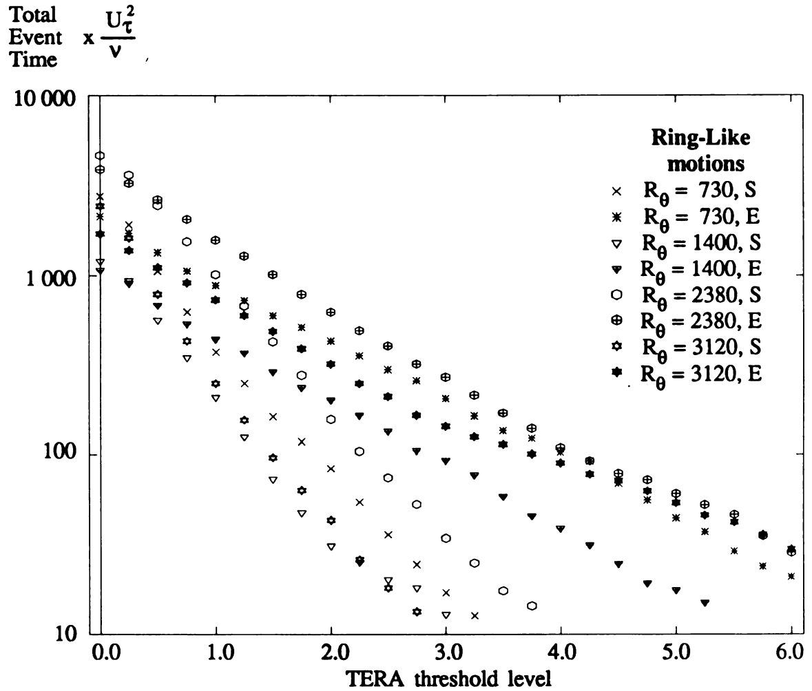
Figure 3.5.5 Inner-Scaled Total TERA Event Time vs. Threshold (RLM data set)
