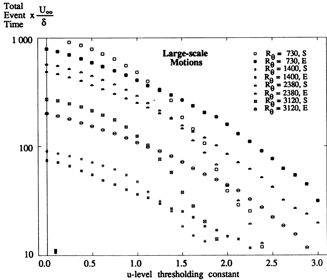
Figure 3.6.12 Outer-Scaled Total u-level Event Time vs. Threshold (LSM data set)
