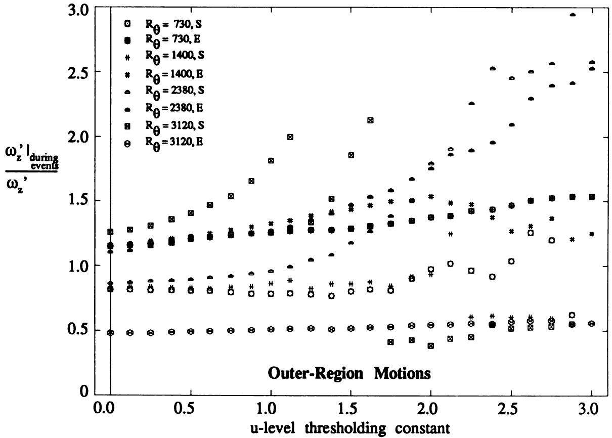
Figure 3.6.29 RMS \omega_z During u-level Events Normalized by \omega_z' vs. Threshold (LSM data set)
