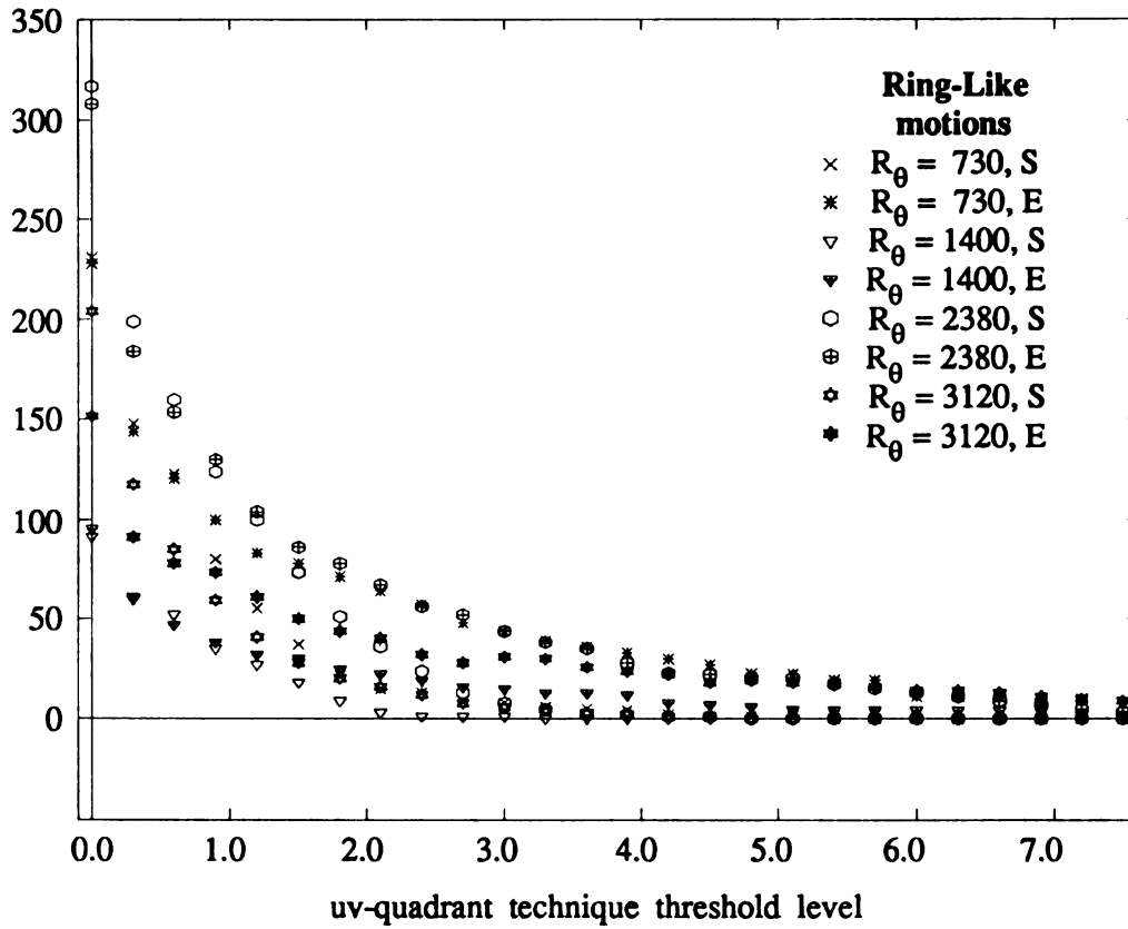
Figure 3.4.2 Number of uv-quadrant Events vs. Threshold level (RLM data set)
