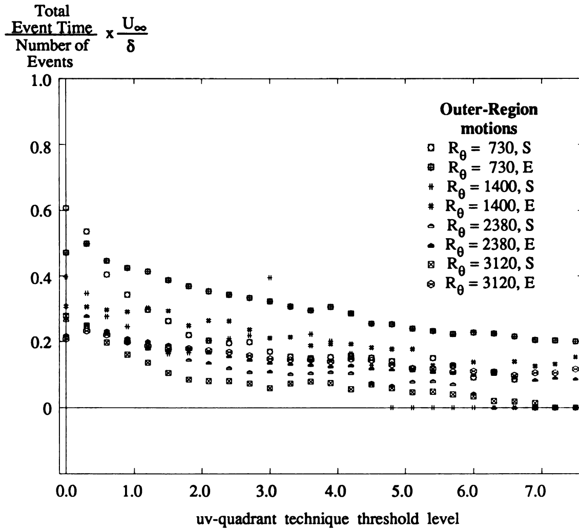
Figure 3.4.24 Outer-Scaled Average uv-quadrant Event Length vs. Threshold (LSM data set)
