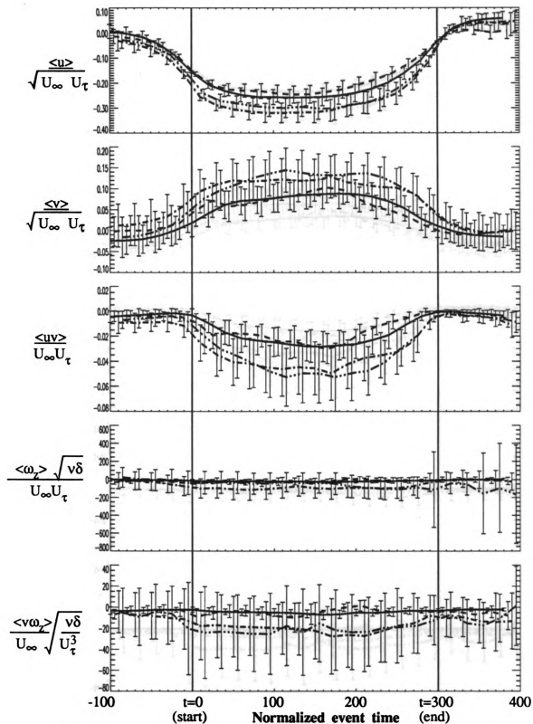
Figure 3.6.36 Mixed-scaled u-level ejection ensembles. Error bars indicate 25% of an ensemble's standard deviation about each point in time
