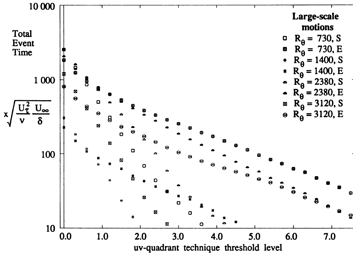
Figure 3.4.9 Total uv-quadrant Event Time (Mixed Scaling) vs. Threshold (LSM data set)
