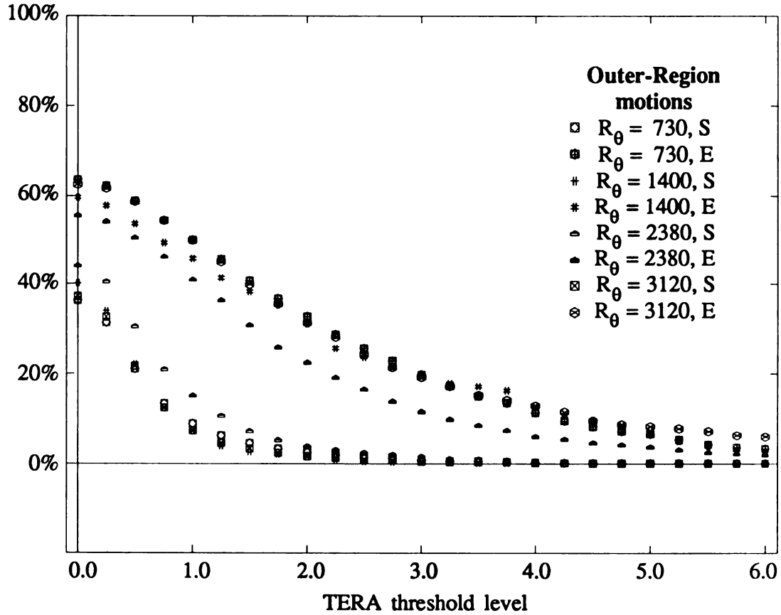
Figure 3.5.27 Percent Reynolds Stress "captured" during TERA events vs. Threshold (LSM data set)
