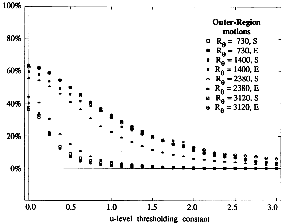
Figure 3.6.27 Percent Reynolds Stress "captured" during u-level events vs. Threshold (LSM data set)
