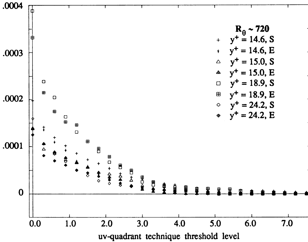
Figure 3.4.15 Outer-scaled uv-quadrant Event frequency vs. Threshold level (Inner-region data)
