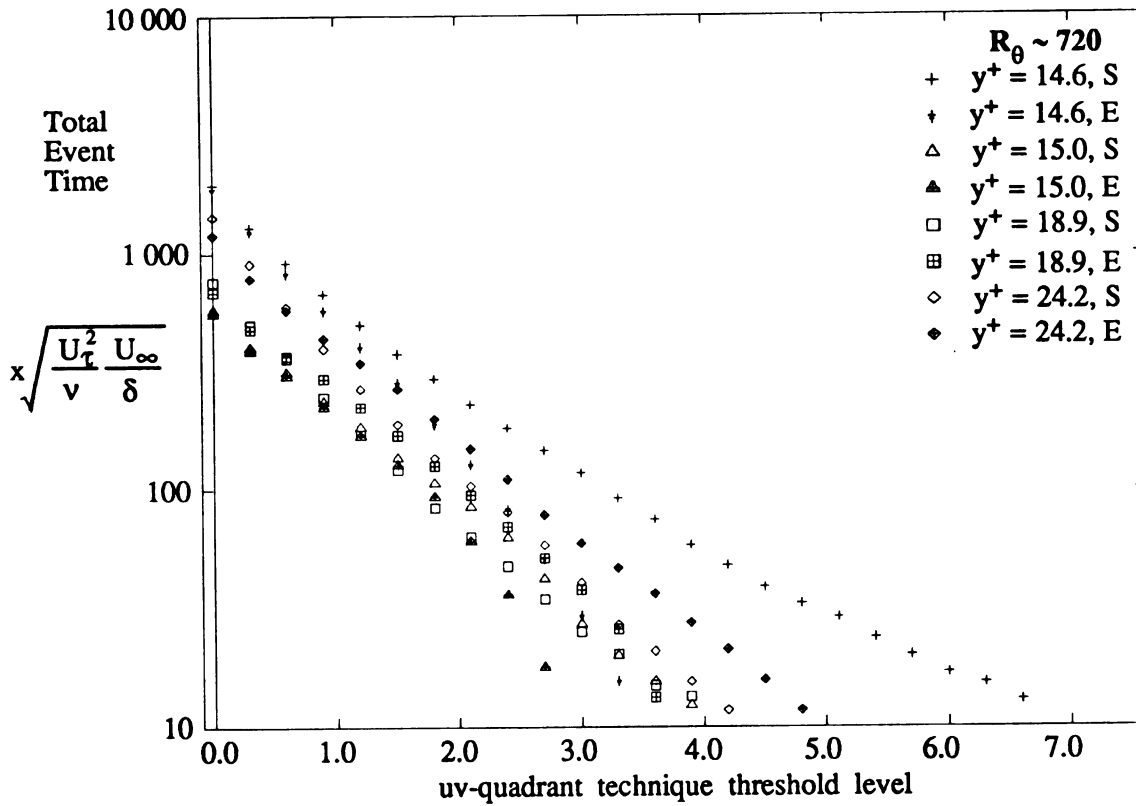
Figure 3.4.7 Total uv-quadrant Event Time (Mixed Scaling) vs. Threshold (Inner-region data)
