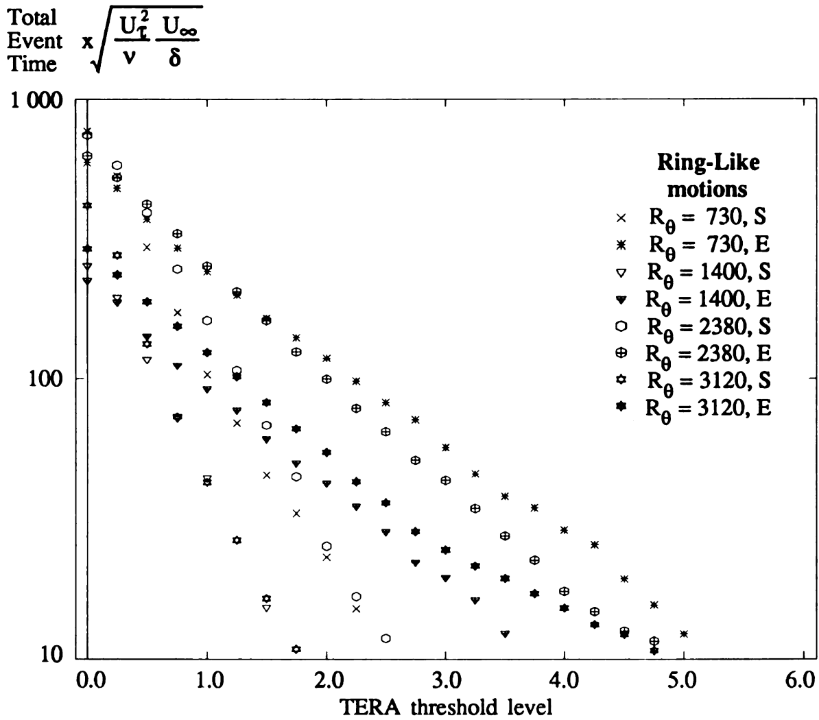
Figure 3.5.8 Total TERA Event Time (Mixed Scaling) vs. Threshold (RLM data set)
