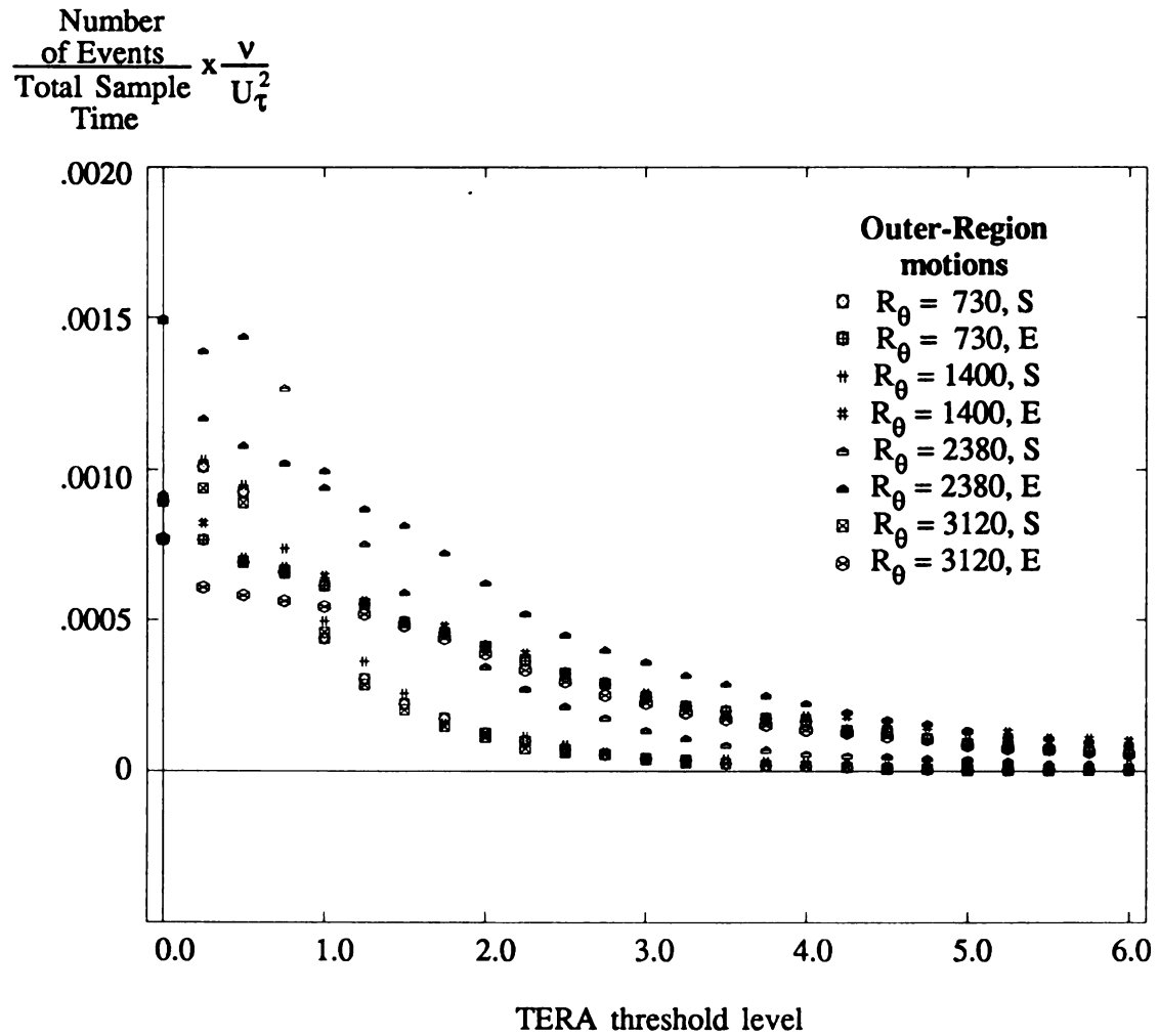
Figure 3.5.16 Inner-scaled TERA Event frequency vs. Threshold level (LSM data set)
