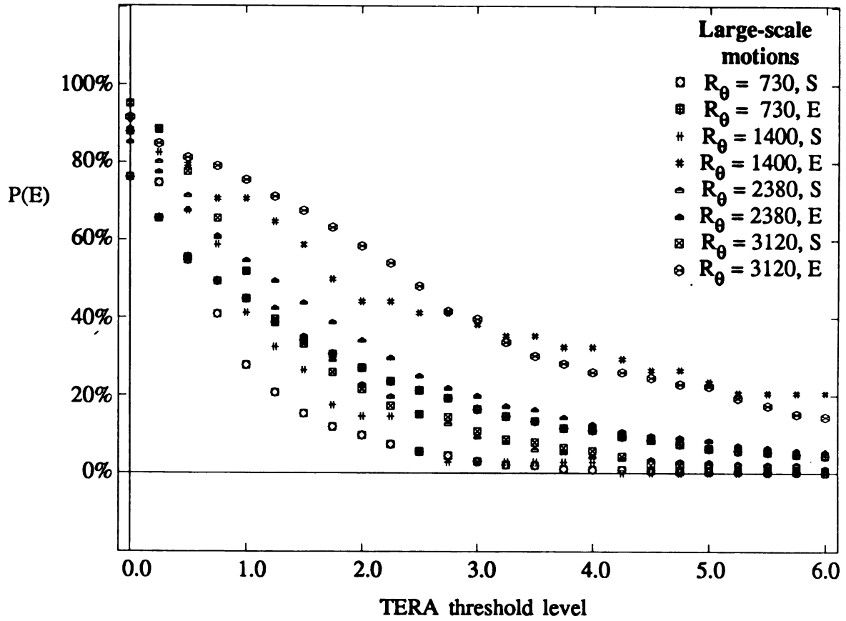
Figure 4.1.5 P(E): Probability of a TERA Detection Occurring During an LSM Detection vs. Threshold
