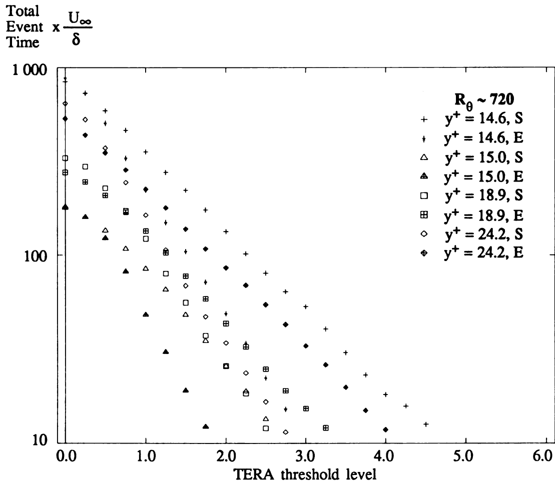
Figure 3.5.10 Outer-Scaled Total TERA Event Time vs. Threshold (Inner-region data)
