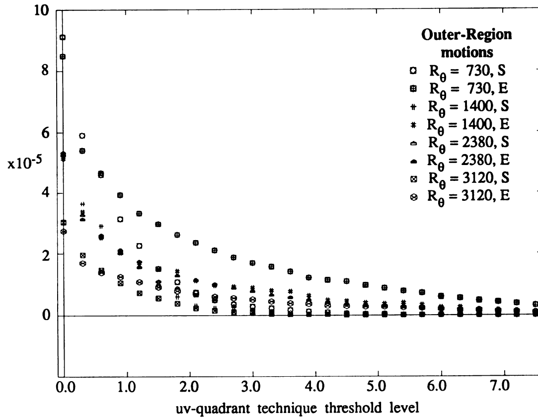
Figure 3.4.18 Outer-scaled uv-quadrant Event frequency vs. Threshold level (LSM data set)
