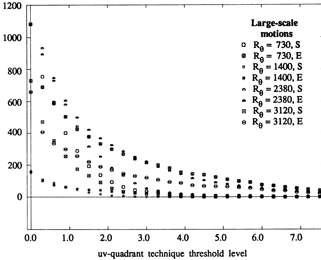
Figure 3.4.3 Number of uv-quadrant Events vs. Threshold level (LSM data set)
