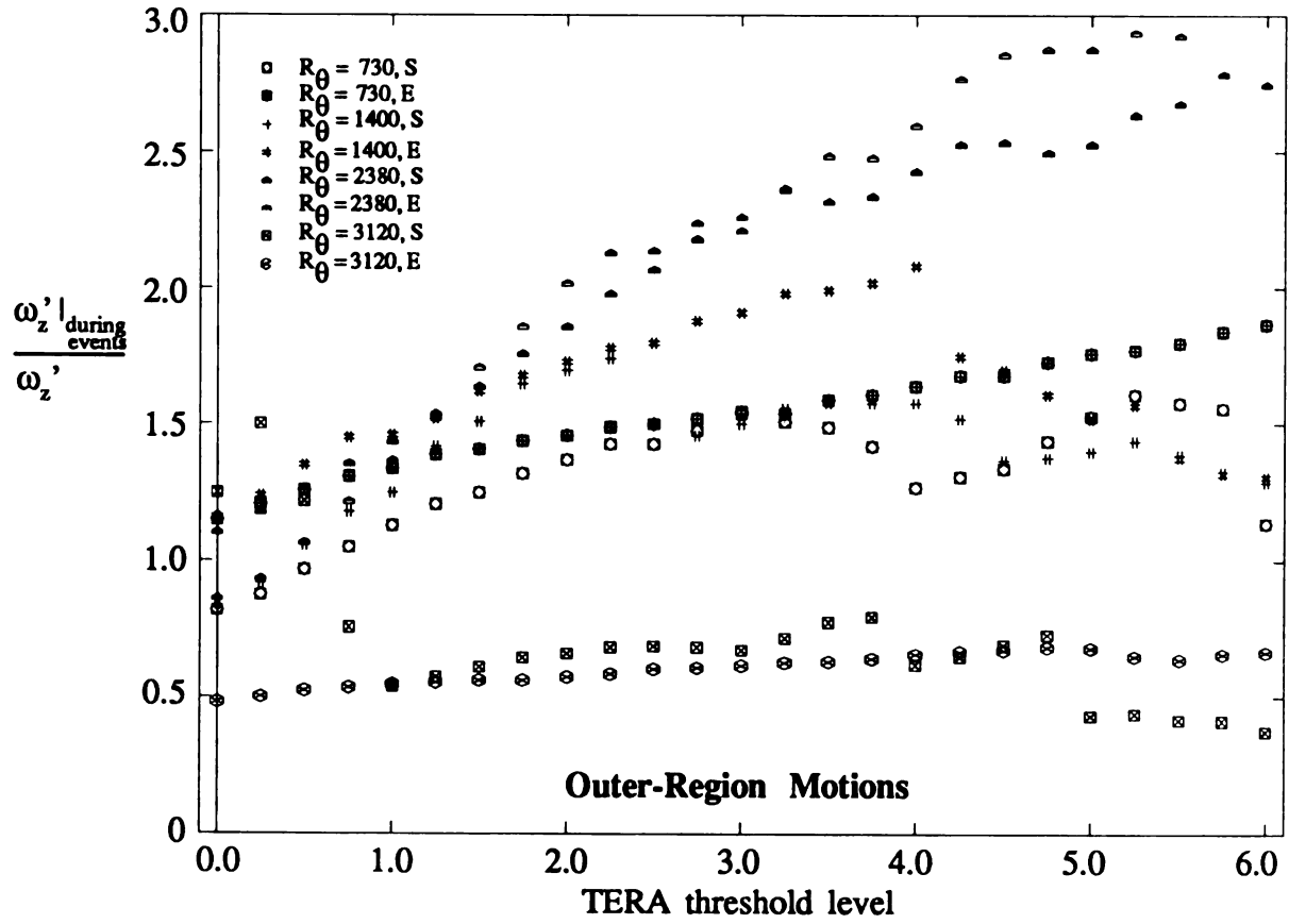
Figure 3.5.29 RMS \omega_z During TERA Events Normalized by \omega_z' vs. Threshold (LSM data set)
