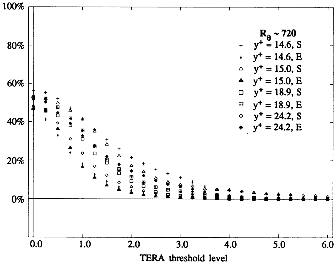
Figure 3.5.26 Percent Reynolds Stress "captured" during TERA events vs. Threshold (Inner-region data)
