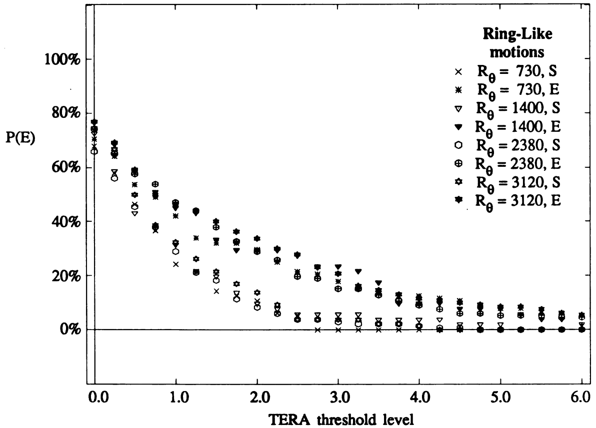
Figure 4.2.5 P(E): Probability of a TERA Detection Occurring During an RLM Detection vs. Threshold
