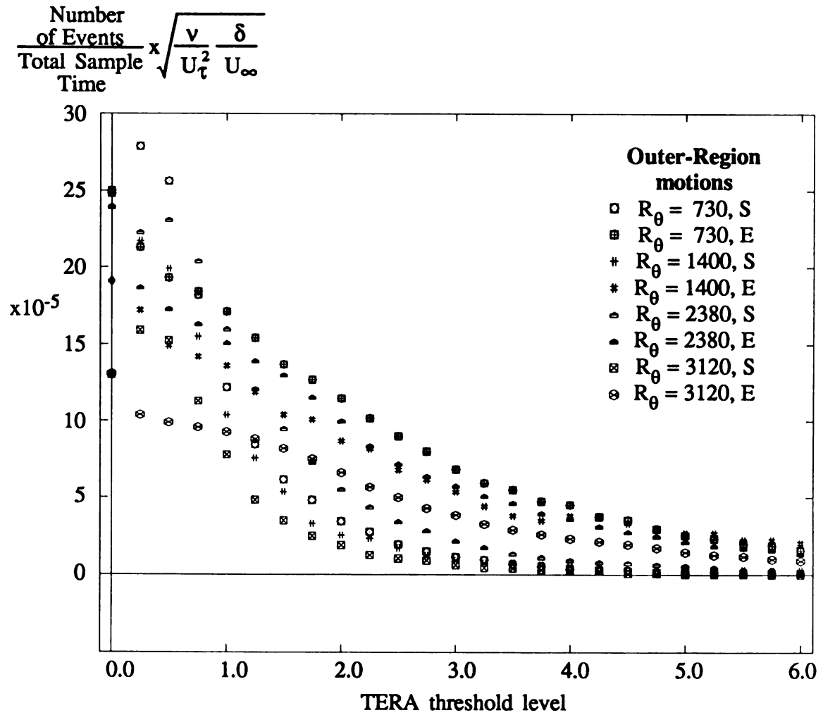
Figure 3.5.17 TERA Event frequency (Mixed-scaling) vs. Threshold level (LSM data set)
