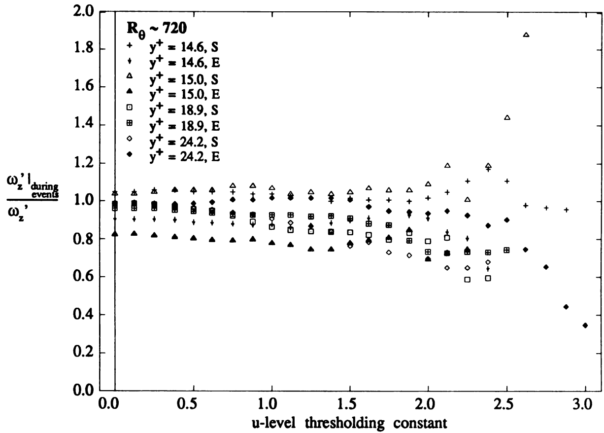
Figure 3.6.28 RMS \omega_z During u-level Events Normalized by \omega_z' vs. Threshold (Inner-region data)
