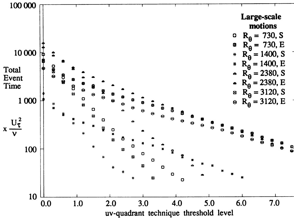
Figure 3.4.6 Inner-Scaled Total uv-quadrant Event Time vs. Threshold (LSM data set)
