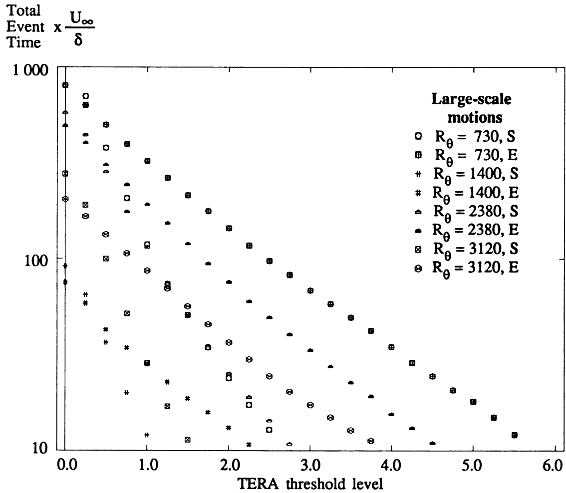
Figure 3.5.12 Outer-Scaled Total TERA Event Time vs. Threshold (LSM data set)
