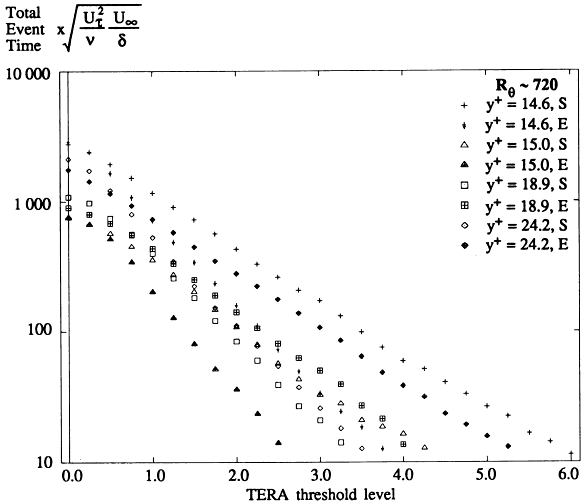
Figure 3.5.7 Total TERA Event Time (Mixed Scaling) vs. Threshold (Inner-region data)
