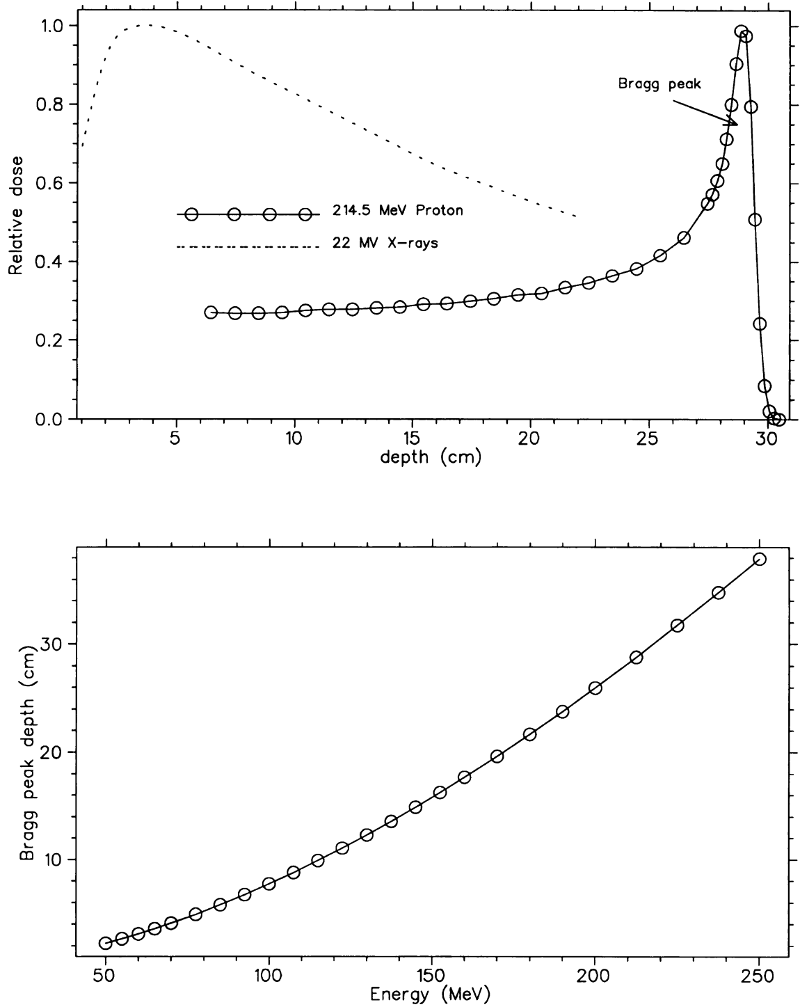
Figure 1.1: Top: experimental depth-dose curve for 214.5 MeV protons from the Paul Scherrer Institute (solid curve) [27]. The dose deposition is normalized such that the dose deposition is equal to one unit at the Bragg peak. Dash line gives dose curve for 22 MV X-rays, normalized to peak, from Ref. [28]. Bottom: Bragg peak depth as function of proton energy [27].
