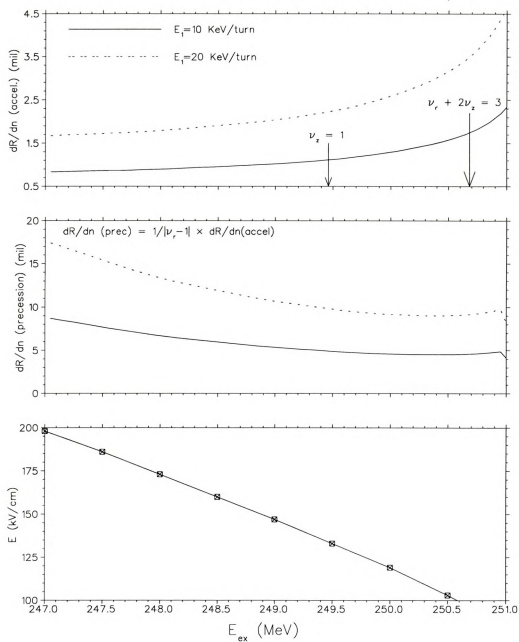
Figure 8.1: Top: dR/dn (accel.) vs. energy. Middle: dR/dn (precession) vs. energy. Bottom: required electric deflector field strength vs. final energy.
