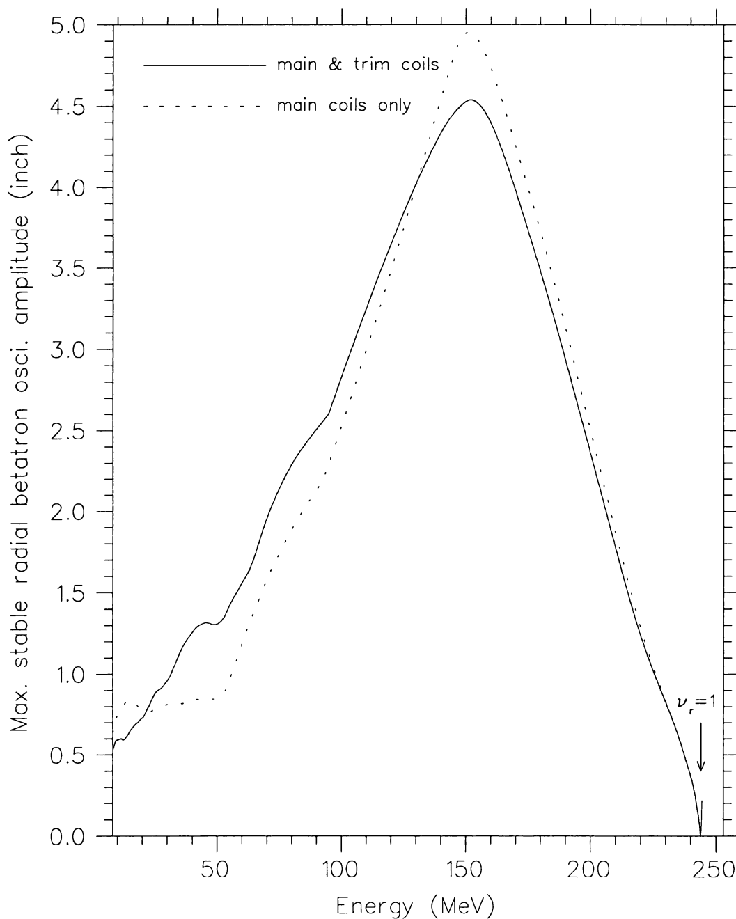
Figure 3.7: Plot of maximum stable radial betatron oscillation amplitude A_c (the radial distance in the phase space from the equilibrium orbit to the furthest unstable fixed point) calculated by using the EO code, as function of energy in the K250 synchrocyclotron perfect field. The solid curve is associated with trim coils on, the dotted curve with all trim coils off. Recall that A_c \propto |\nu_r - 1| .
