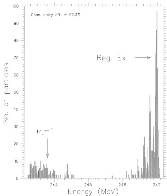
Figure 6.14: Distribution of energies for the particles entering successfully the first extraction channel at \theta = 336^\circ .
