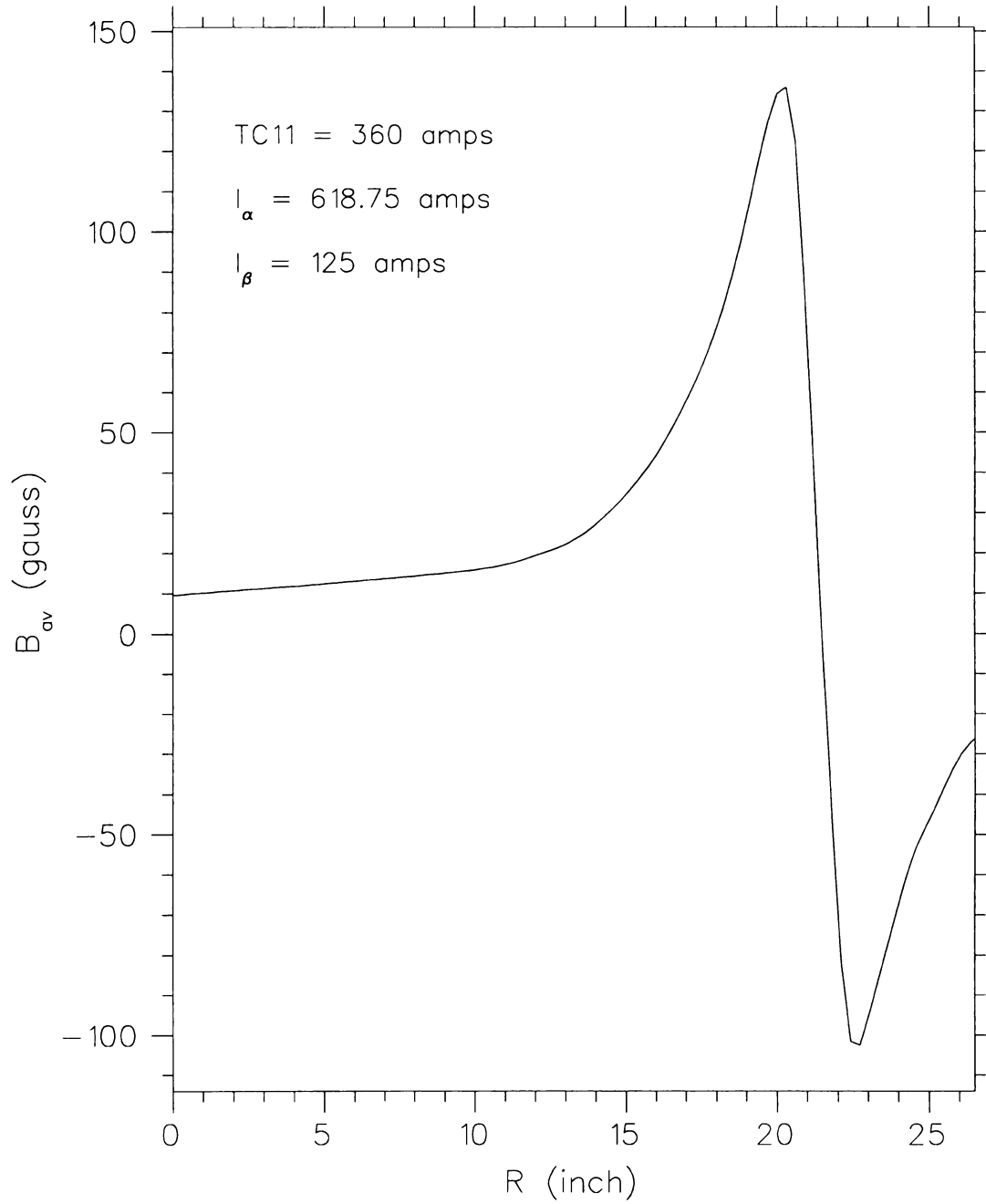
Figure 3.2: Average field ( B_{av}(r) \equiv \int_0^{2\pi} B(r_o, \theta, z=0) d\theta / 2\pi ) at excitation 360 A, equal currents in three sectors, for the trim coil 11, measured at main coil currents (amps) I_{\alpha}/I_{\beta} = 618.75/125 , from Ref. [54].
