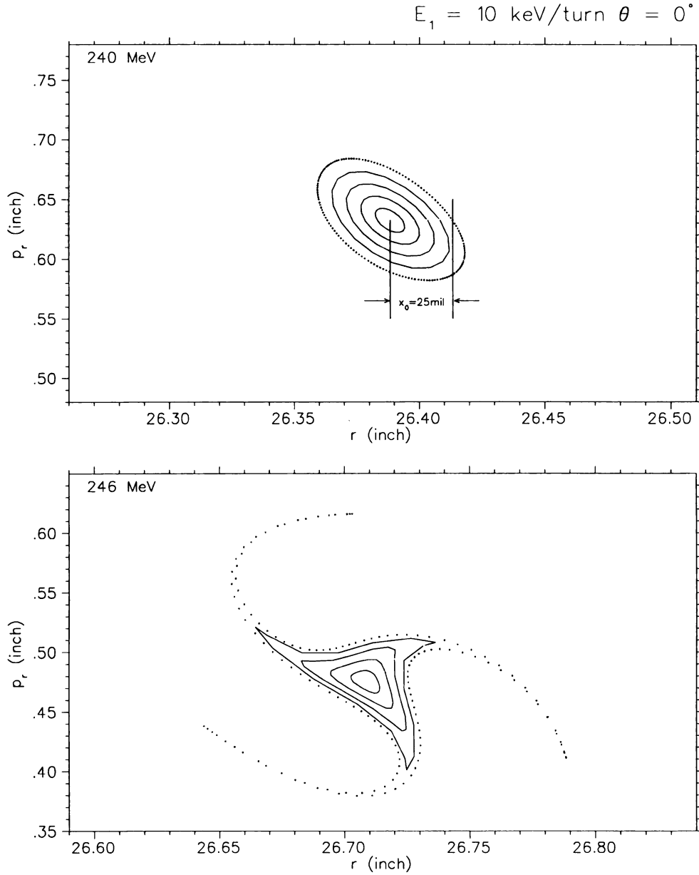
Figure 3.13: Radial phase plots at E=240 \text{ MeV} and 246 \text{ MeV} , \theta = 0^\circ , in the K250 120^\circ field. Upper panel shows five coasting orbits associated with initial displacements in radius of 5, 10, 15, 20 and 25 mil relative to the equilibrium orbit. Lower panel shows the corresponding orbits at E=246 \text{ MeV} , which start on the eigenellipses in the upper frame and are accelerated, assuming constant energy gain 10 keV per turn. The dotted curves indicate the estimated acceptance of radial space region inside which most of the orbits can be recaptured by the renewed central stable region after passing \nu_r = 1 .
