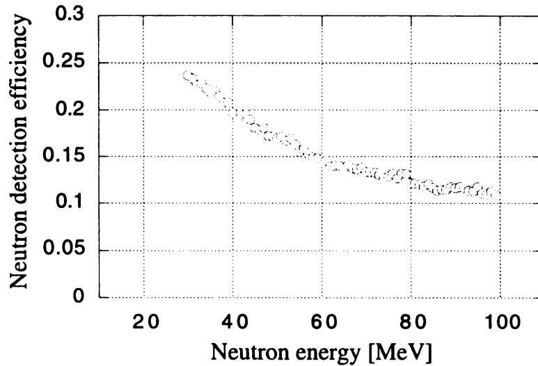
Figure 3.5: Simulated efficiency curve of the neutron detector with a sideways geometry. It was calculated with the code KSUEFF [Cec79].
