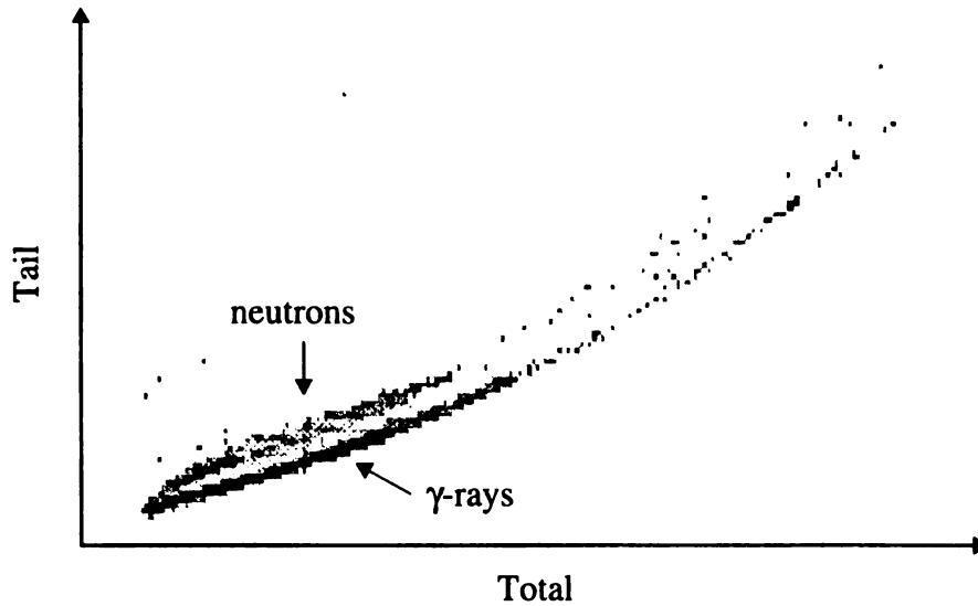
Figure 4.9: Two dimensional plot of the neutron detector signal. A ^{239}\text{Pu} -Be source was used to supply \gamma -rays and neutrons along with ^{60}\text{Co} \gamma -ray source.
