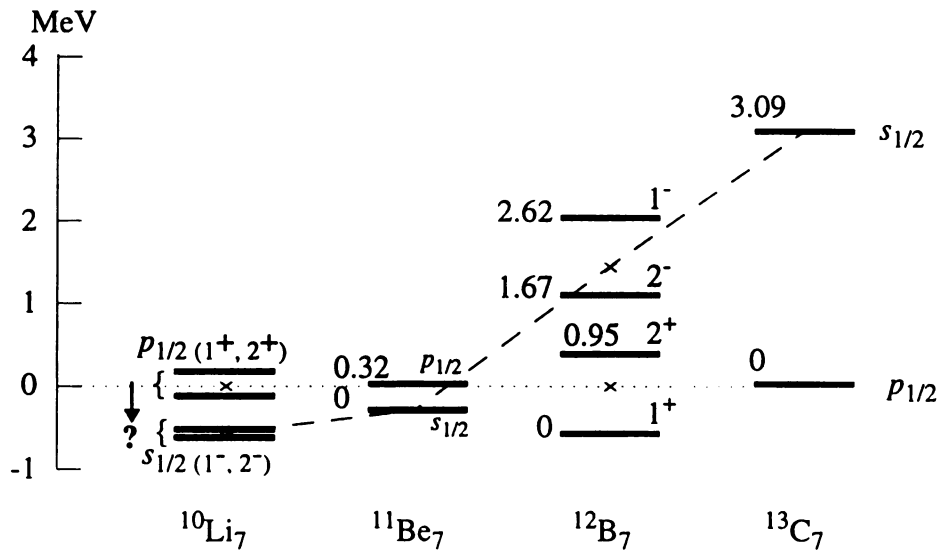
Figure 2.8: Competition between s_{1/2} and p_{1/2} levels among N=7 nuclei [Tal60]. The levels are shifted to match the lowest p_{1/2} state. Extrapolation implies the non-normal parity ground state of ^{10}\text{Li} [Bar77].
