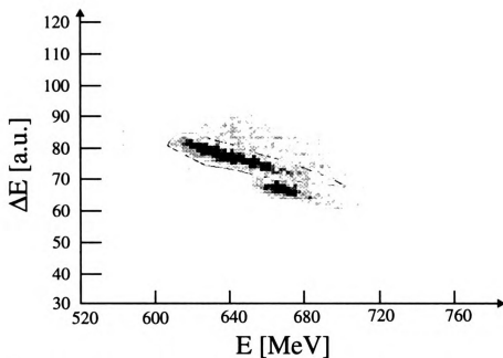
Figure 4.14: \Delta E_1 (first quadrant of \Delta E ) vs. E3 plot of the Li group. The contour shows a {}^9\text{Li} isotope gate.
