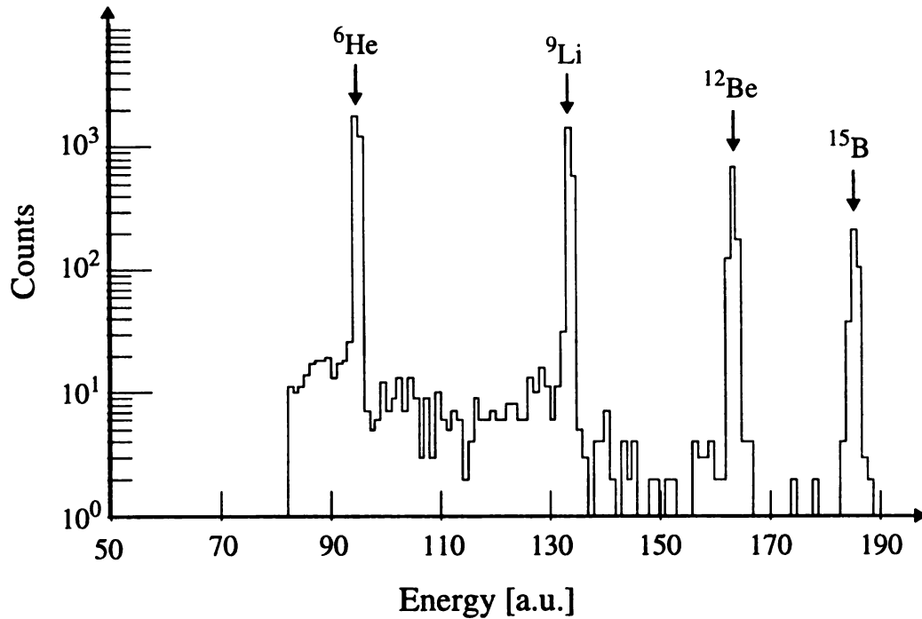
Figure 4.3: Energy spectrum of the calibration beam with an A/Z=3 gate.
