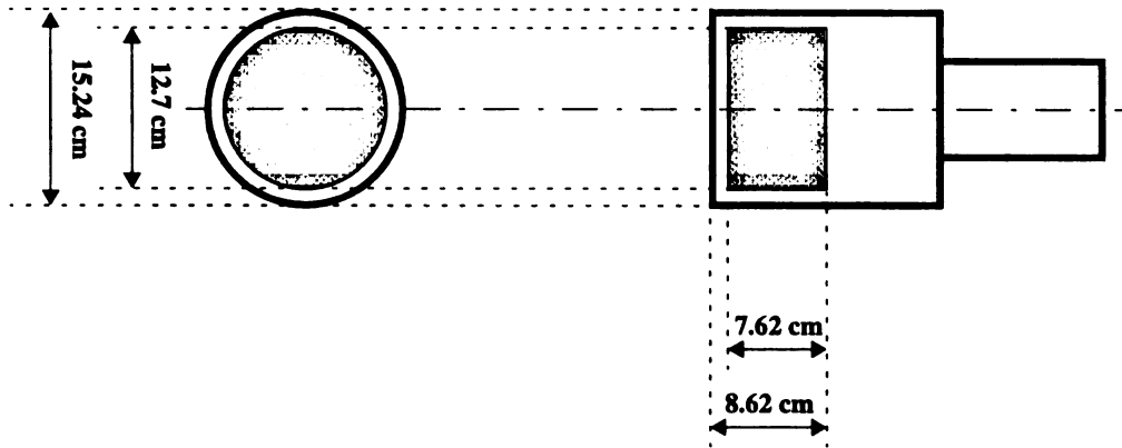
(a) Neutron detector dimension
