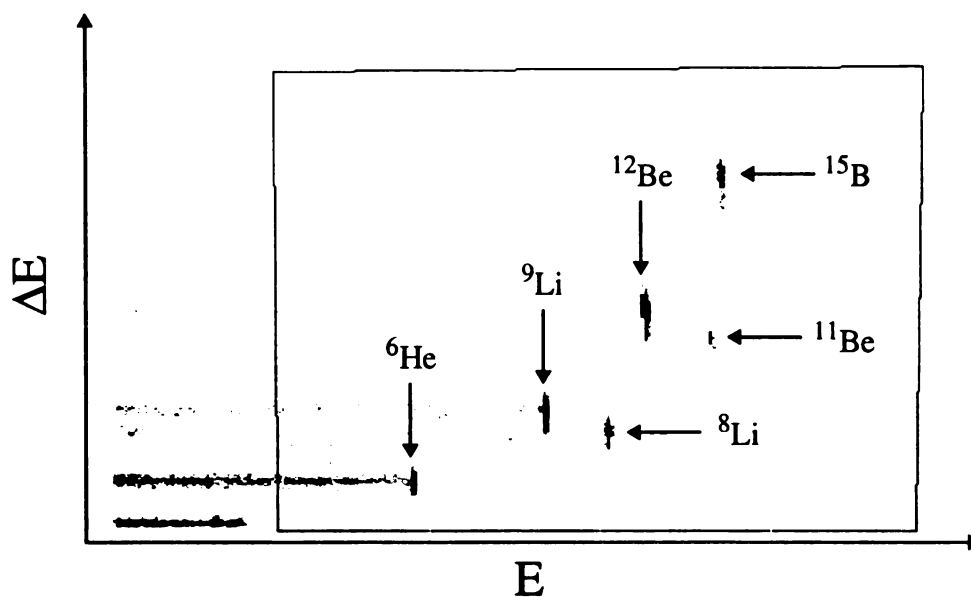
Figure 4.2: Two dimensional histogram of energy loss in the \Delta E2 detector's quadrant number 1 versus total energy in the E3 detector of the fragments. The large square gate in the plot was applied to select the valid signal for a projection.
