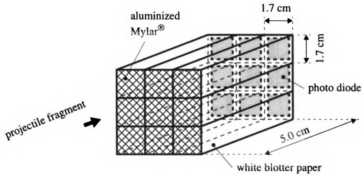
Figure 3.9: Structure of CsI(Tl) E detector array. Each of the nine crystals were wrapped with white blotter paper independently to optically isolate them from each other.
