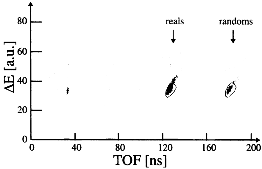
Figure 4.13: \Delta E_1 (first quadrant of \Delta E ) vs. TOF (thin plastic time) plot of He group. The contour gates show the {}^6\text{He} reals gate and the {}^6\text{He} randoms gate.
