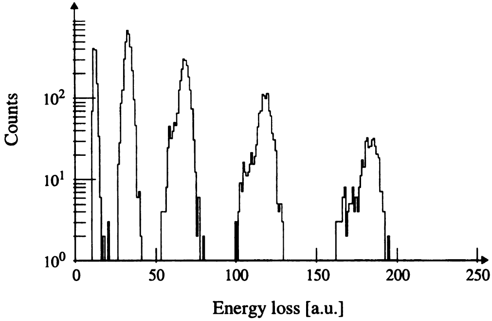
Figure 4.7: Energy loss spectrum of the calibration beam with A/Z=3 gate.
