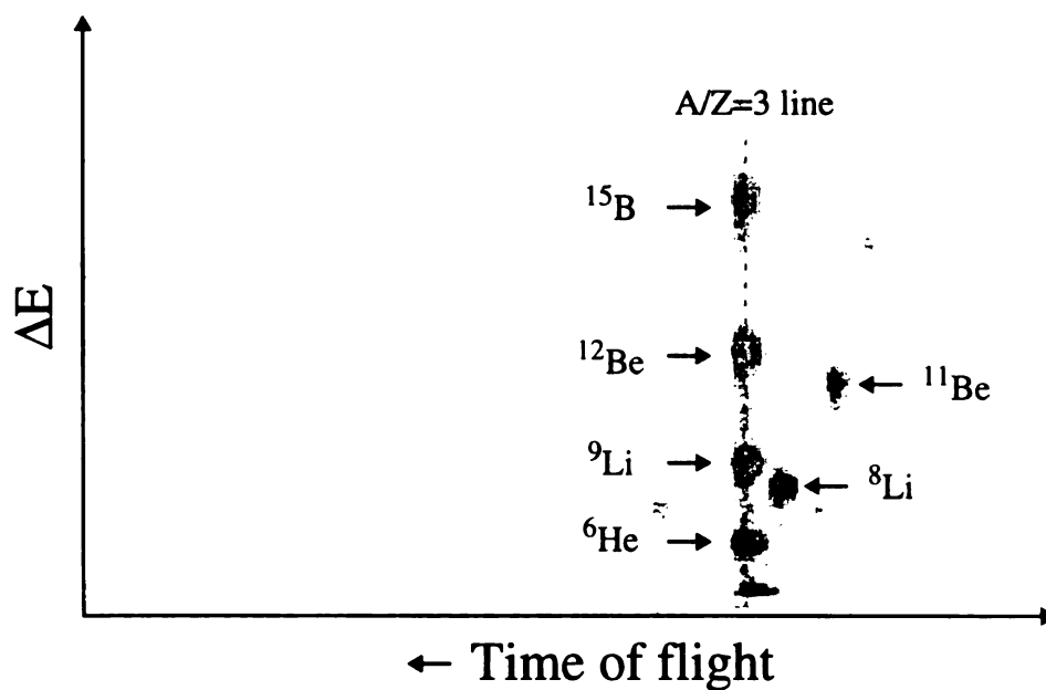
Figure 4.1 Two dimensional histogram of energy loss in the \Delta E2 detector's quadrant number 1 versus time of flight of the fragments. m/q = isotopes are selected using the A1200 mass analyzer.
