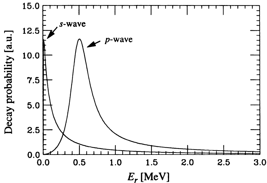
Figure 5.8: The ^{10}\text{Li} lineshapes used for the best fit of the simulation to the data. The relative population of the s -wave and p -wave is 33% and 67%, respectively.
