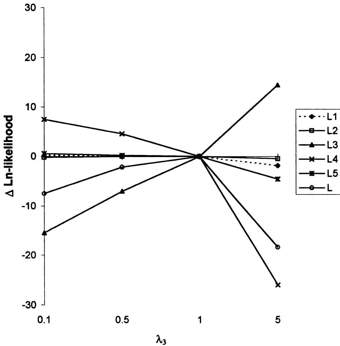
Figure 23. Changes in log e -likelihood components for catch-at-age model fit due to varying emphasis of fishery age composition data ( \lambda_3 ). Likelihood components: L1= fishery harvest, L2= survey CPUE, L3= fishery age composition, L4= survey age composition, L5= fishery effort, L= total.
