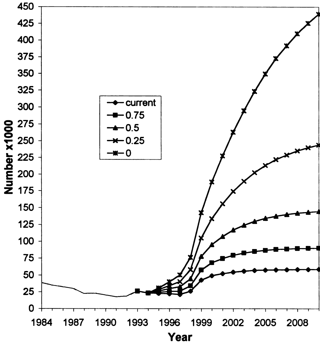
Figure 39. Model estimates of ages 8+ lake trout abundance in central Lake Huron from 1984-2010. Projections were based on a zero fishing management scenario according to varying levels of sea lamprey-induced mortality ( Z_L ): Current= average Z_L for 1991-1993; 0.75= 75% of current; 0.50= 50% of current; 0.25= 25% of current; 0.0= Z_L is 0.
