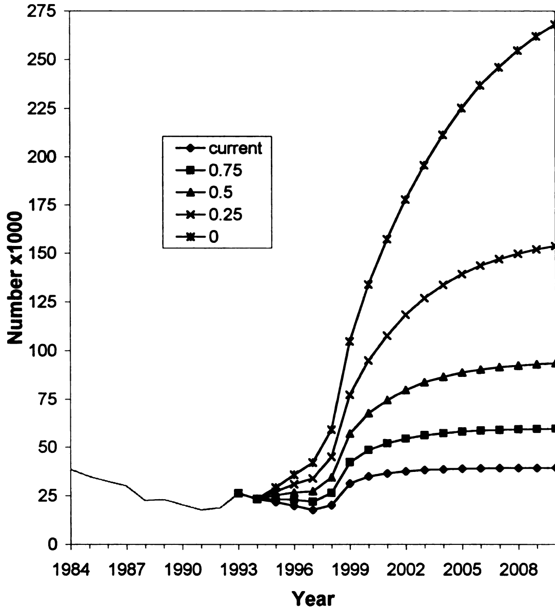
Figure 37. Model estimates of ages 8+ lake trout abundance under a constant fishing mortality management scenario in central Lake Huron from 1984-2010. Fishing mortality rates for projections were based on the average of 1991-1993 rates.
