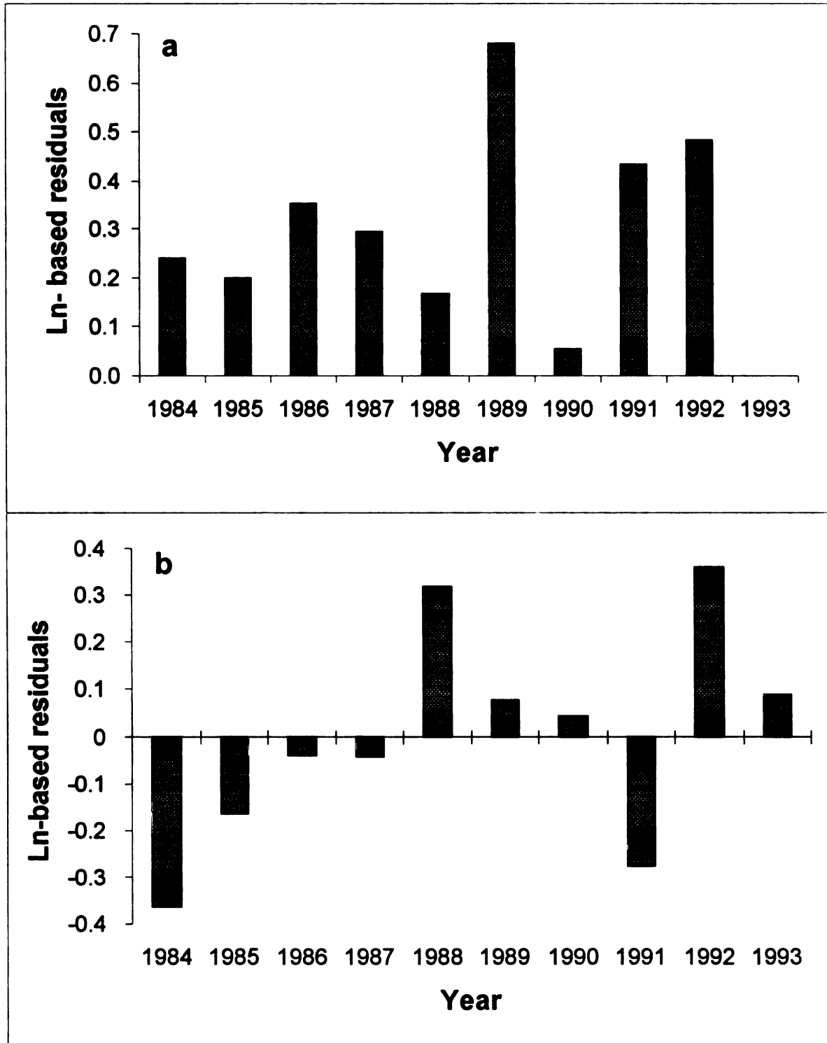
Figure 14. Log e -based residuals from catch-at-age analysis CAA1 of the southern Lake Huron lake trout population model. (a) fishery harvest. (b) survey total CPUE.
