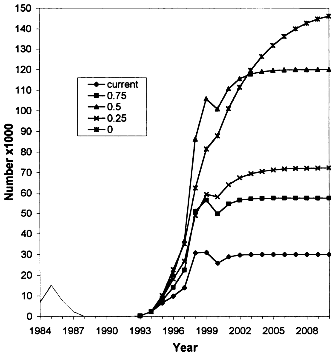
Figure 40. Model estimates of ages 8+ lake trout abundance under a total allowable catch (TAC) management scenario in northern Lake Huron from 1984-2010. Maximum total instantaneous mortality for projections was 0.59 \text{ year}^{-1} . Projections (1994-2010) were according to varying levels of sea lamprey-induced mortality ( Z_L ): Current= average Z_L for 1991-1993; 0.75= 75% of current; 0.50= 50% of current; 0.25= 25% of current; 0.0= Z_L is 0.
