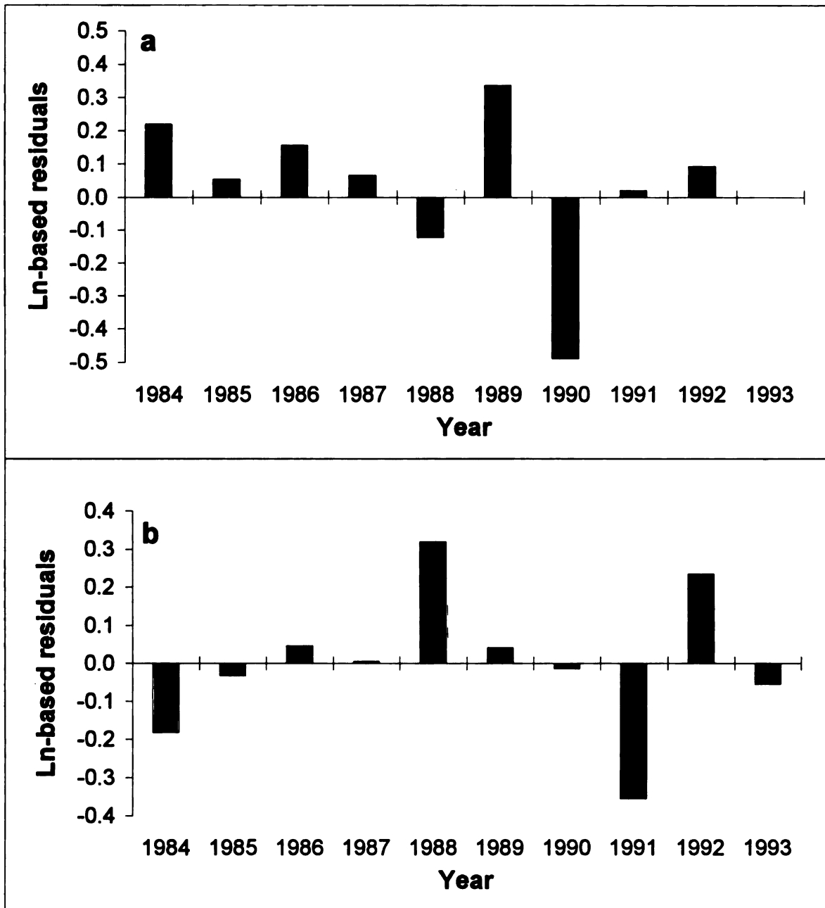
Figure 18. Log e -based residuals from catch-at-age analysis CAA5 of the southern Lake Huron lake trout population model. (a) fishery harvest. (b) survey total CPUE.
