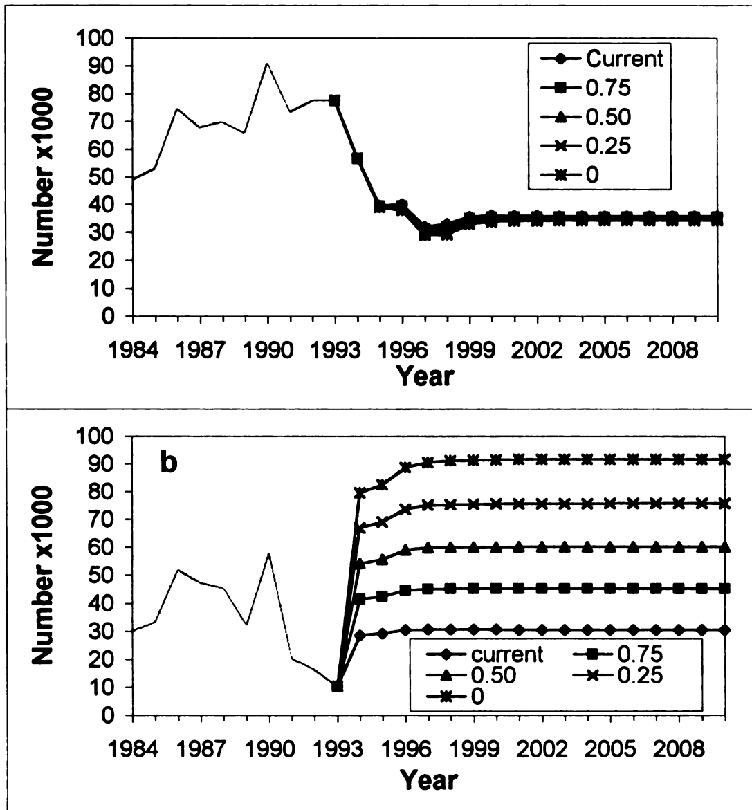
Figure 32. Model estimates of lake trout (a) abundance for ages 8+, and (b) total harvest under a total allowable catch (TAC) management scenario in southern Lake Huron from 1984-2010. Maximum total instantaneous mortality for projections was 0.59 \text{ year}^{-1} . Projections (1994-2010) were according to varying levels of sea lamprey-induced mortality ( Z_L ): Current= average Z_L for 1991-1993; 0.75= 75% of current; 0.50= 50% of current; 0.25= 25% of current; 0.0= Z_L is 0.
