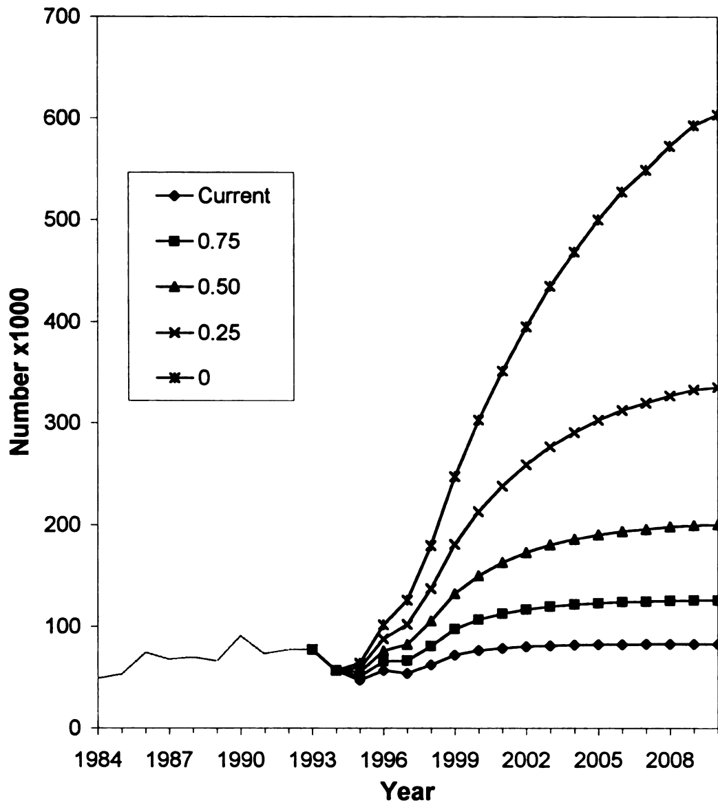
Figure 34. Model estimates of ages 8+ lake trout abundance in southern Lake Huron from 1984-2010. Projections were based on a no fishing management scenario according to varying levels of sea lamprey-induced mortality ( Z_L ): Current= average Z_L for 1991-1993; 0.75= 75% of current; 0.50= 50% of current; 0.25= 25% of current; 0.0= Z_L is 0.
