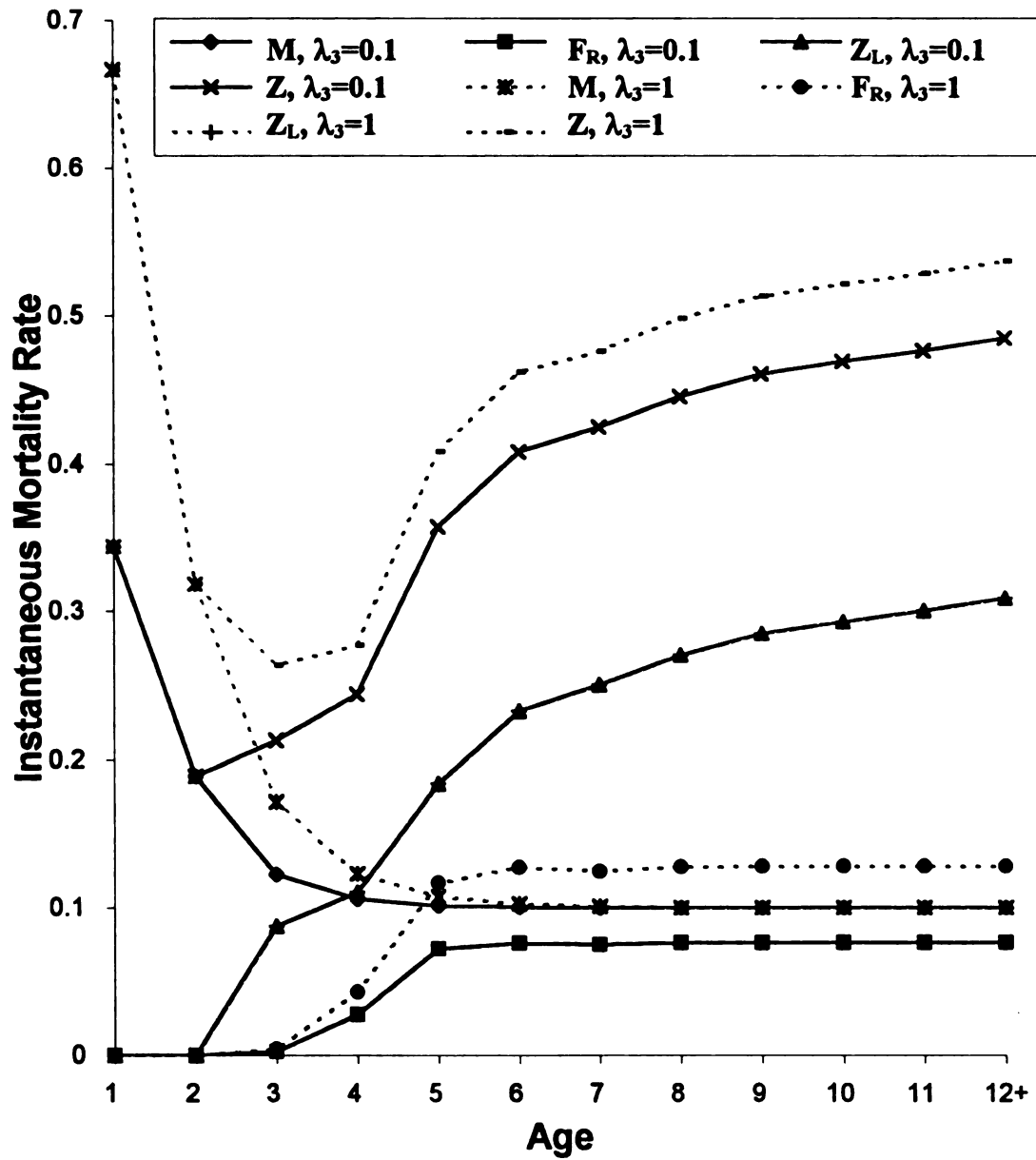
Figure 27. Differences in estimated age-specific instantaneous mortality rates ( \text{year}^{-1} ) with emphasis factor for fishery age composition data ( \lambda_3 ) set at 0.1 and 1. Mortality rates averaged from 1984-1993. M =natural mortality, F_R = recreational fishing mortality, Z_L = sea lamprey-induced mortality, and Z = total mortality.
