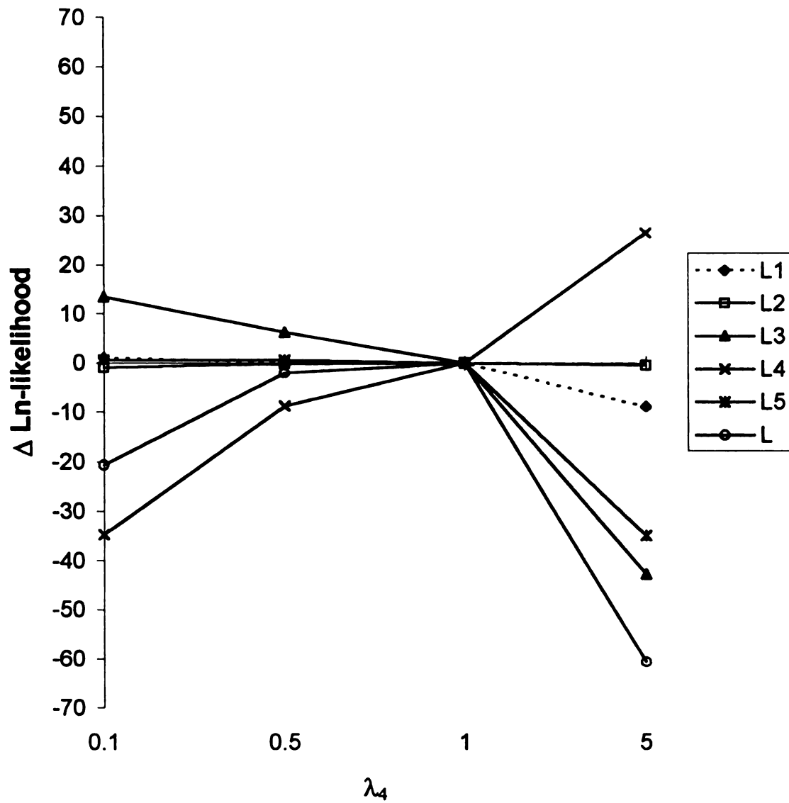
Figure 24. Changes in log e -likelihood components for catch-at-age model fit due to varying emphasis of survey age composition data ( \lambda_4 ). Likelihood components: L1= fishery harvest, L2= survey CPUE, L3= fishery age composition, L4= survey age composition, L5= fishery effort, L= total.
