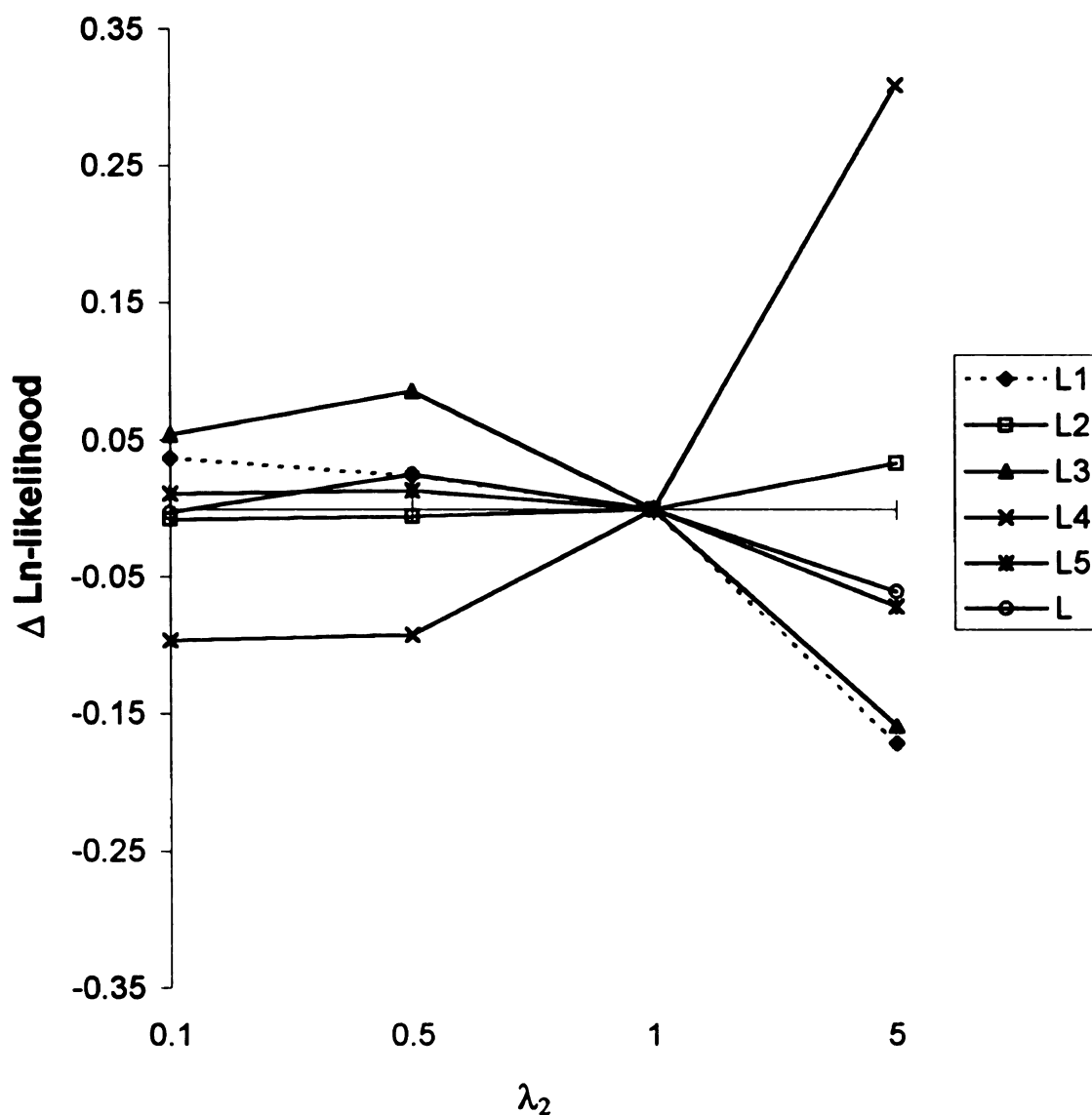
Figure 22. Changes in log-likelihood components for catch-at-age model fit due to varying emphasis of survey CPUE data ( \lambda_2 ). Likelihood components: L1= fishery harvest, L2= survey CPUE, L3= fishery age composition, L4= survey age composition, L5= fishery effort, L= total.
