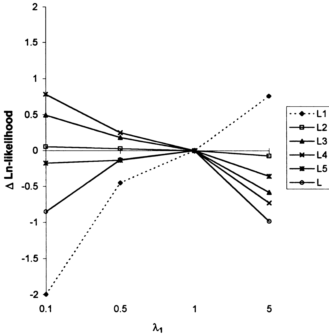
Figure 21. Changes in log e -likelihood components for catch-at-age model fit due to varying emphasis of fishery harvest data ( \lambda_1 ). Likelihood components: L1= fishery harvest, L2= survey CPUE, L3= fishery age composition, L4= survey age composition, L5= fishery effort, L= total.
