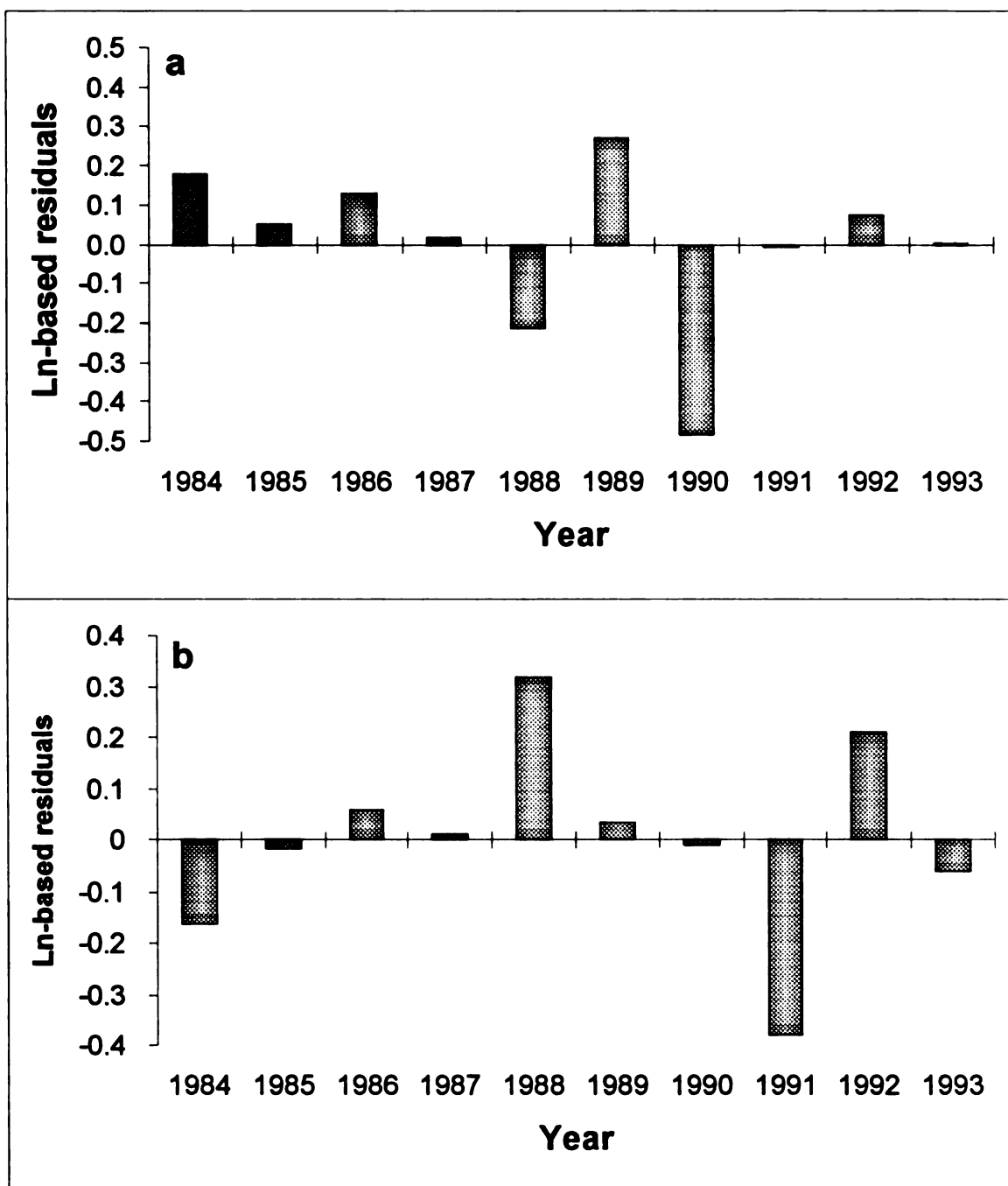
Figure 15. Log-based residuals from catch-at-age analysis CAA3 of the southern Lake Huron lake trout population model. (a) fishery harvest. (b) survey total CPUE.
