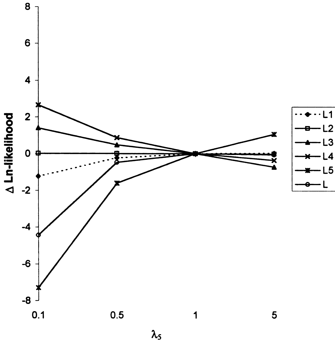
Figure 25. Changes in log e -likelihood components for catch-at-age model fit due to varying emphasis of fishery effort data ( \lambda_5 ). Likelihood components: L1= fishery harvest, L2= survey CPUE, L3= fishery age composition, L4= survey age composition, L5= fishery effort, L= total.
