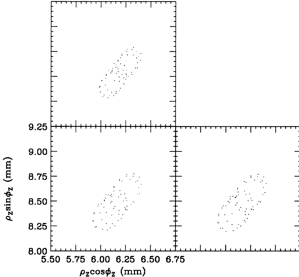
Figure 4.2: Three maps of an orbit that has the same initial conditions as those of the orbit # 3 in the top diagram of Fig. 3.2. These were obtained by plotting \rho_z \sin \phi_z vs. \rho_z \cos \phi_z at every sector \theta = 2n\pi/3 for 100 turns using the three different options of the Z^{2N} Orbit Code with N = 2 (top diagram), N = 3 (bottom left diagram), and N = 4 (bottom right diagram). The length and width of the small blur of points expand by less than 1 % compared with the average \rho_z values of the points. It is clear from this figure that inclusion of higher order terms does not significantly affect the location of the “stable fixed points”.
