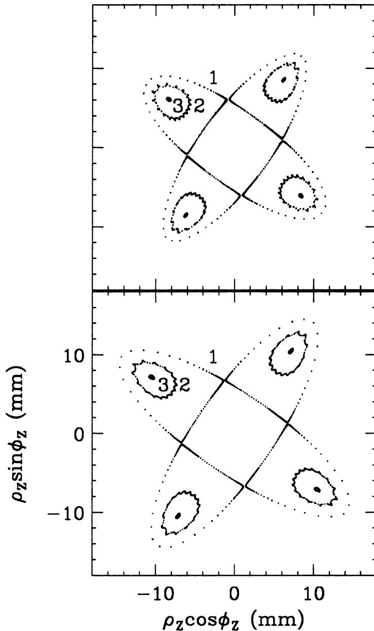
Figure 3.2: Two z -space diagrams (just like those in Fig. 3.1) for two sets of three orbits obtained by plotting once per sector, again at 34.8 MeV/u where \nu_z = 0.740 . The set at the top was obtained using the Z^{2N} Orbit Code with N=2 , while the set at the bottom was derived from the Hamiltonian in Eq. 3.9 that includes the third-order coupling terms. In contrast to the comparable situation in Fig. 3.1, the results presented here show that this Hamiltonian provides a relatively good explanation of the orbit code results, including the location of the fixed points and the fine structure in the phase plots. Note that all the orbits from the Z^{2N} Orbit Code with N = 2 reflect coupling effects. Unlike the situation predicted by the simple theory in Fig. 3.1, the stable and unstable fixed points are not sharply defined due to the coupling effects.
