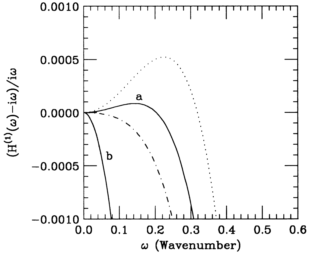
Figure A.1: Plot of (H^{(1)}(\omega) - i\omega)/i\omega over the range 0 \leq \omega \leq 0.6 for the old differentiator (real line “b”), and that for the improved differentiator (solid line “a”) with Q = 1.70 . The dotdash line corresponds to Q = 1.65 and the dotted line to Q = 1.75 . Composition of the central difference scheme “b” with the filter improves the low frequency behavior significantly, which results in “a” with Q = 1.70 .
