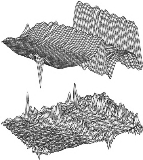
Figure 5.2: A map of \nabla_2^2 B \times 0.5^2/2! evaluated at z = 0.5 (in) by using the improved differentiators (at the top) and a map of difference between this and the map for the same term computed using the “old differentiator” (at the bottom) for the magnetic field shown in Fig. 5.1. The maximum and minimum values of the map at the top are (248 G, -352 G) respectively while those of the difference map at the bottom are (13.0 G, -11.9 G). Note that the two maps are not plotted to the same scale. The map at the bottom depicting the difference shows the relative defects of the old differentiators in suppressing noise.
