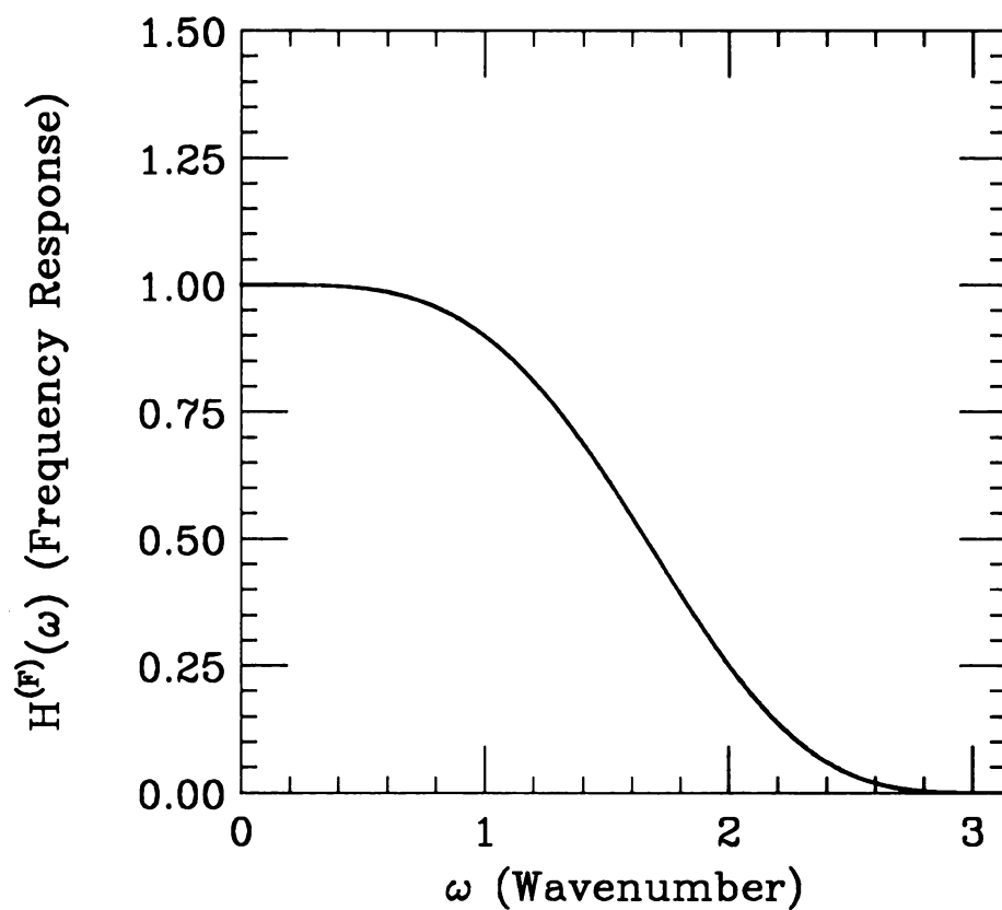
Figure A.5: Plot of the frequency response, H^{(F)}(\omega) over the range 0 \leq \omega \leq \pi , of the filter used for the improved partial differentiators with Q = 1.01 as a function of wavenumber, \omega . The nice low frequency response and the suppression of high frequency signals are shown.
