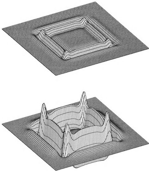
Figure A.12: Two maps of the difference between exact values and those from the two differentiators for \nabla_2^4 B \times 0.5^4/4! term over the range -4 \leq x \leq 4 and -4 \leq y \leq 4 with \Delta x = \Delta y = 0.1 . The top map depicts the difference between theory and the improved differentiators, while the bottom map portrays the difference between theory and the old differentiators. Both of these are plotted to the same scale. The maximum and the minimum of the top map are 2.9 \text{ G} and -2.0 \text{ G} respectively, while those of the bottom map are 16.3 \text{ G} and -10.9 \text{ G} . Clearly, the improved differentiators are about five times more accurate than the old differentiators for the fourth-order term in B_z at z = 0.5 .
