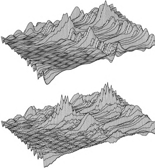
Figure 5.3: A map of \nabla^4 B \times 0.5^4/4! evaluated at z = 0.5 (in) by using the improved differentiators (at the top) and a map of difference between this and the map for the same term computed using the “old differentiator” (at the bottom) for the magnetic field shown in Fig. 5.1. The maximum and minimum values of the map at the top are (82.3\text{ G}, -104\text{ G}) respectively while those of the difference map at the bottom are (33.9\text{ G}, -28.5\text{ G}) . Note that the two maps are not plotted to the same scale. Because useful slowly varying components of data are washed out to an appreciable extent by the “old differentiators” when they are applied twice to get the fourth-order term, the values of the bottom map depicting the difference are significant compared with those of the fourth-order term itself at the top. (See Figs. A.10 and A.12 in the appendix for the wash-out of physically important slowly varying components of data.) Moreover it is not easy to observe the rapidly varying small noise because it is buried in the washed out data.
