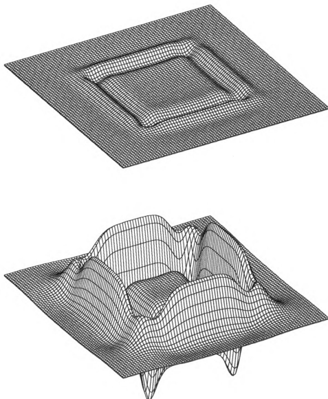
Figure A.10: Two maps of the difference between exact values and those from the two differentiators for \nabla_2^2 B \times 0.5^2/2! term over the range -4 \leq x \leq 4 and -4 \leq y \leq 4 with \Delta x = \Delta y = 0.1 . The top map depicts the difference between theory and the improved differentiators, while the bottom map portrays the difference between theory and the old differentiators. Both of these are plotted to the same scale. The maximum and the minimum of the top map are 1.1 \text{ G} and -1.5 \text{ G} respectively, while those of the bottom map are 13.2 \text{ G} and -19.4 \text{ G} . Clearly, the improved differentiators are about twelve times more accurate than the old differentiators.
