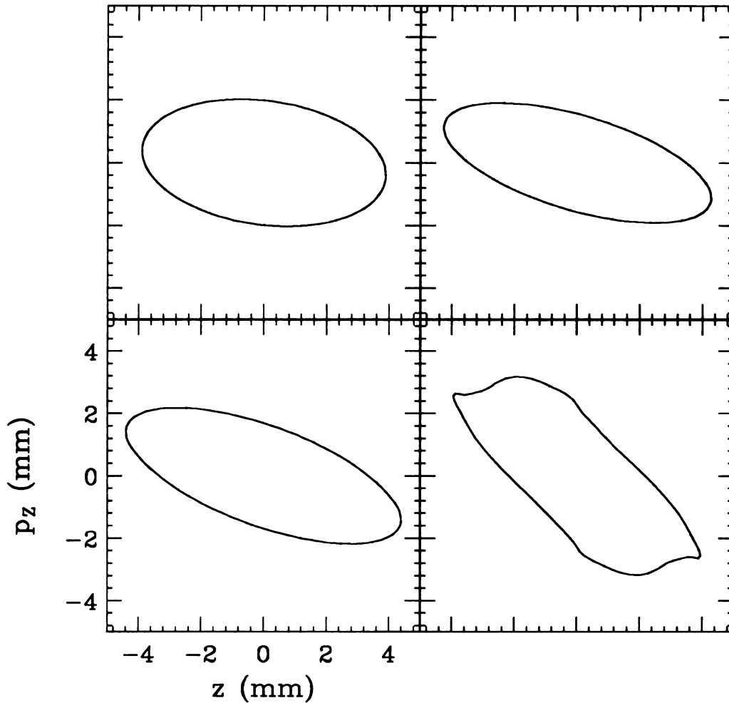
Figure 4.3: Evolution of an eigenellipse in z -phase space starting at 10 MeV/u (top left diagram) depicted at every 10 MeV/u during its acceleration for 619 turns after which the central ray reaches the final energy E_f = 40 MeV/u (bottom right diagram). These plots obtained by using the Z^{2N} Orbit Code with N = 2 show the evolution of the ellipse at 20 MeV/u (top right diagram), at 30 MeV/u (bottom left diagram) and at 40 MeV/u (bottom right diagram). It should be noted that the initial emittance is 2\pi J_z/p = 7.64 \pi \text{ mm-mrad} (assuming p = 1.0 \text{ m} ) for the initial eigenellipse at 10 MeV/u. (These diagrams should be compared with the those in Fig. 1.2 which are the results of a similar calculation.) Initially, all the points on the eigenellipse share the same values of (r_0, p_{r0}) which is on the accelerated equilibrium orbit at 10 MeV/u. The bottom right diagram is deformed appreciably due to the traversal of the \nu_z = 3/4 resonance between 30 MeV/u and 40 MeV/u. Almost exactly the same results were obtained with the N = 3 , and N = 4 options for the Z^{2N} Orbit Code. (The same is true for the results in Fig. 4.4 below.)
