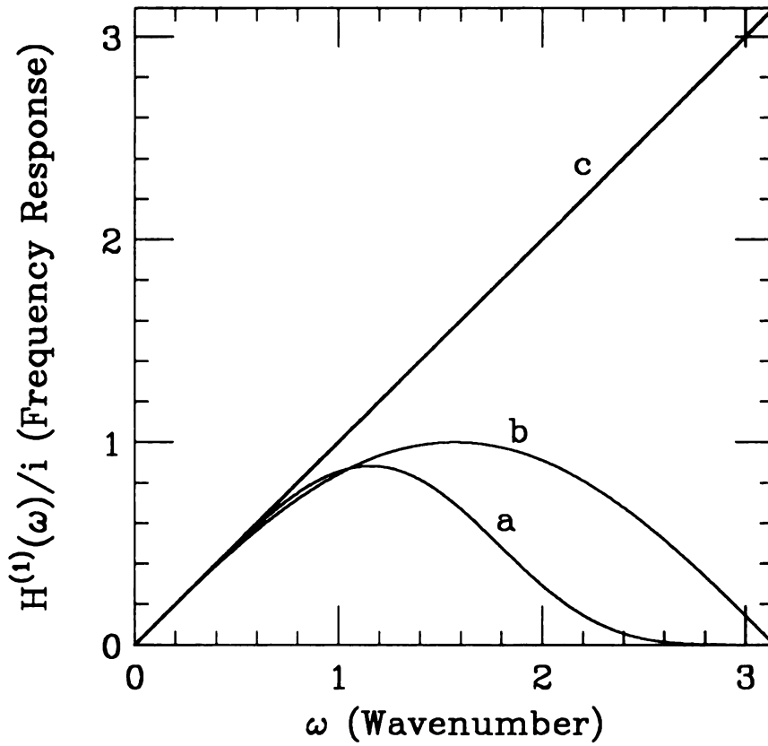
Figure A.2: Plots of H^{(1)}(\omega)/i , as a function of the wavenumber \omega over the range 0 \leq \omega \leq \pi . Curve “a” is for our improved differentiator, curve “b” for the old differentiator, and curve “c” for the mathematical first-order differentiator. “a” is superior to “b” in suppressing high frequency signals and shows a frequency response reasonably close to that of the mathematical differentiator for low frequency as well. It should be pointed out that the cutoff frequency \omega_{cutoff} is about 1.05.
