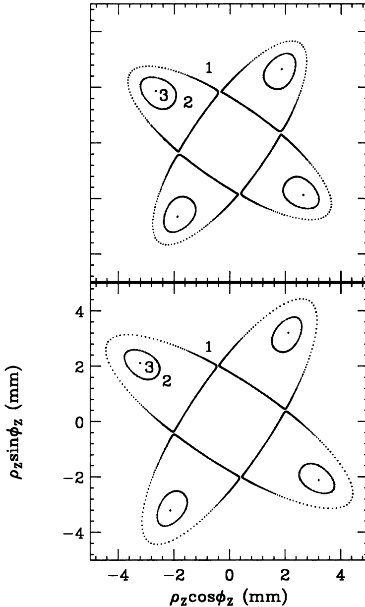
Figure 3.5: Two z -space diagrams (like those in Fig. 3.2) for two sets of three orbits obtained by plotting \rho_z \sin \phi_z vs. \rho_z \cos \phi_z once per turn at 35.5 MeV/u where \nu_z = 0.749 . But Fig. 3.2 was plotted once per sector and its scale is 3.6 times larger. The set at the top was obtained using the Z^{2N} Orbit Code with N = 2 , while the set at the bottom was derived from the Hamiltonian in Eq. 3.15 that includes the third-order coupling terms. The plots are very similar except for the scale and the turn numbers of the orbits compared with those in Fig. 3.2. Even though the fine structure may not be observable for the given scale, it becomes apparent when the plots are magnified.
