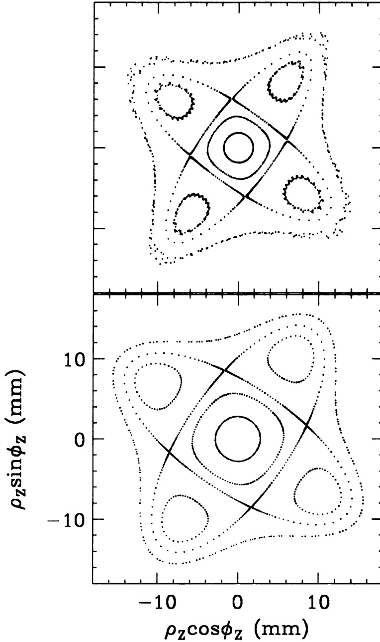
Figure 3.1: Two z -space diagrams at \nu_z = 0.740 ( E = 34.8 MeV/u) obtained by plotting \rho_z \sin \phi_z vs. \rho_z \cos \phi_z once per sector for two sets of five orbits. One set (shown at top) is obtained from the Z^{2N} Orbit Code with N = 2 and the other set (shown at bottom) is derived from the simple Hamiltonian in Eq. 3.1 with its constants evaluated at the given energy. The simple theory obviously fails to reproduce quantitatively the results from the orbit code, including the location of the fixed points. It also fails to account for the fine structure in the phase plots from the orbit code which, as shown below, are produced by the coupling effects. Note that (\phi, J) are angle-action variables and that \rho = (2J)^{1/2} corresponds to a “radius” in phase space.
