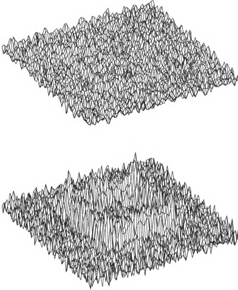
Figure A.14: Two maps of the difference in \nabla_2^4 B \times 0.5^4/4! between the exact derivatives for the field without the noise and those obtained from the two numerical differentiators applied to the field with the random noise within \pm 0.1 G . These are plotted to the same scale over the range -4 \leq x \leq 4 and -4 \leq y \leq 4 with \Delta x = \Delta y = 0.1 . This figure should be compared with Fig. A.12. The top (bottom) map depicts the difference for the improved (old) differentiators. The maximum and the minimum of the top map are 6.1 G and -5.8 G respectively, while those of the bottom map are 20.3 G and -15.7 G . These figures again show the combined effects of the errors produced by the two numerical differentiators for the field without the noise and the additional errors due to the noise. The surface of the bottom map is even sharper than that at the top, and the height of individual spikes is larger.
