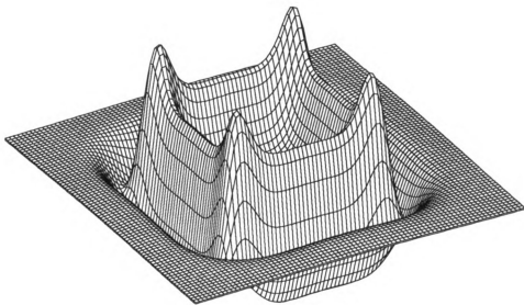
Figure A.11: Map of \nabla_2^4 B \times 0.5^4/4! obtained from the analytical expression. This is plotted over -4 \leq x \leq 4 and -4 \leq y \leq 4 with \Delta x = \Delta y = 0.1 . The maximum and the minimum are 140\ G and -86.5\ G , respectively.
