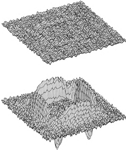
Figure A.13: Two maps of the difference in \nabla^2 B \times 0.5^2/2! between the exact derivatives for the field without the noise and those obtained from the two numerical differentiators applied to the field with the random noise within \pm 0.1 G. The magnitude of the noise is very small compared with the maximum field value of 12.6 kG of B . These are plotted to the same scale over the range -4 \leq x \leq 4 and -4 \leq y \leq 4 with \Delta x = \Delta y = 0.1 . This figure should be compared with Fig. A.10. The top (bottom) map depicts the difference for the improved (old) differentiators. The maximum and the minimum field values of the top map are 2.4 G and -2.4 G respectively, while those of the bottom map are 14.8 G and -20.5 G. These figures show the combined effects of the errors produced by the two numerical differentiators for the field without the noise and the additional errors due to the noise. The surface of the top map is smoother than that at the bottom.
