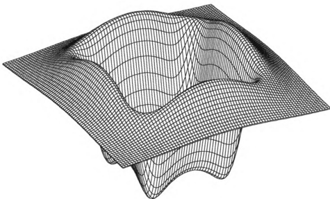
Figure A.9: Map of \nabla_2^2 B \times 0.5^2/2! obtained from the analytical expression. This is plotted over -4 \leq x \leq 4 and -4 \leq y \leq 4 with \Delta x = \Delta y = 0.1 . The maximum and the minimum are 446 \text{ G} and -948 \text{ G} , respectively.
