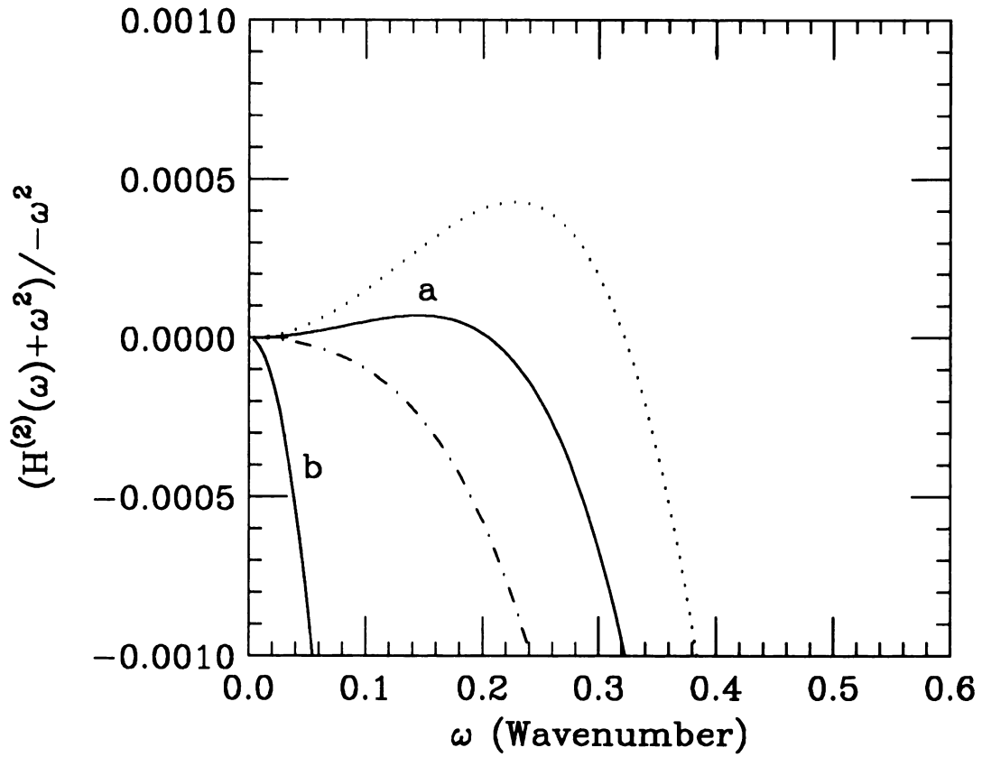
Figure A.3: Plot of (H^{(2)}(\omega) + \omega^2) / -\omega^2 over the range 0 \leq \omega \leq 0.6 for the old differentiator (solid line “b”), and that for the improved differentiator (solid line “a”) with Q = 1.36 . The dotdash line corresponds to Q = 1.30 and the dotted line to Q = 1.40 . Composition of the central difference scheme with the filter improves the low frequency behavior significantly, which results in “a” with Q = 1.36 .
