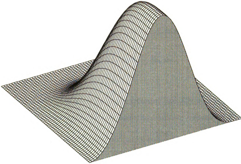
Figure A.7: Plot of the frequency response of the improved second-order partial differentiator with respect to x multiplied by (-1) , -H_x^{(2)}(\omega_x, \omega_y) , for 0 \leq \omega_x \leq \pi and 0 \leq \omega_y \leq \pi . The suppression of high frequency signals both in x and y should be noted. It shows the correct quadratic behavior for low frequency components as well.
