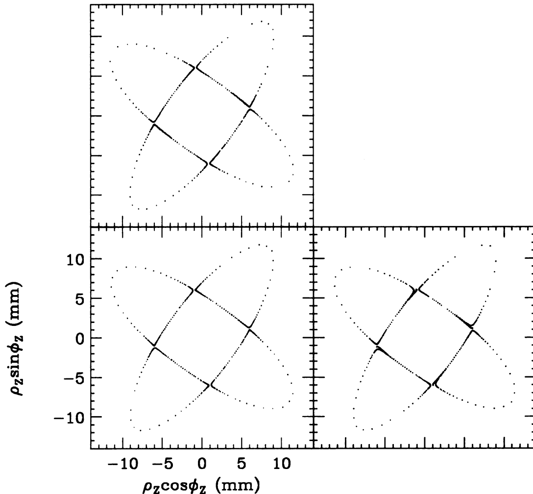
Figure 4.1: Three maps of orbits for which one can get as close as possible to the separatrices at \nu_z = 0.740 without jumping out of the island. These were obtained by plotting \rho_z \sin \phi_z vs. \rho_z \cos \phi_z at every sector \theta = 2n\pi/3 for 190 turns. The orbit at the top (with N = 2 ) has the same initial conditions as those of the orbit # 1 in the top diagram of Fig. 3.2, which are (z_0 = 3.9192, p_{z0} = 0) . The orbit at the bottom left (right) has the initial conditions (z_0 = 3.9243 (3.9522), p_{z0} = 0) for N = 3 ( N = 4 ). Here all the initial values are in units of mm. The variation in the initial conditions is less than 1 % and the basic features, such as the location of the unstable fixed points remain almost unchanged even with inclusion of higher order terms proportional up to z^6 and z^8 .
