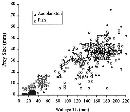
Figure 27. Relationship between walleye size and size of prey observed in gut for 1994 and 1995 diets pooled. Zooplankton sizes are total lengths while fish prey sizes are standard length.
