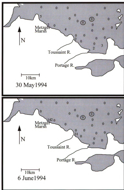
Figure 17. Distribution and density (#/1,000 m 3 ) of pelagic walleye larvae in western Lake Erie based on catches in neuston samples 30 May (top) and 6 June (bottom) 1994. Circles identify reef sites where egg sampling occurred.
