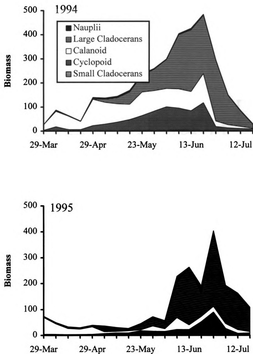
Figure 22. Mean zooplankton dry-weight biomass ( \mu\text{g/l} ) in western Lake Erie estimated from vertical tows at 3 to 7 sites in spring of 1994 (top) and 1995 (bottom).
