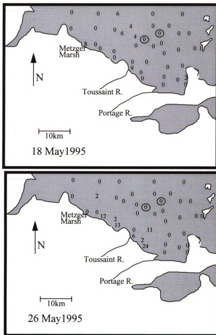
Figure 20. Distribution and density (#/1,000 m 3 ) of pelagic walleye larvae in western Lake Erie based on catches in neuston samples 18 May (top) and 26 May (bottom) 1995. Circles identify reef sites where egg sampling occurred.
