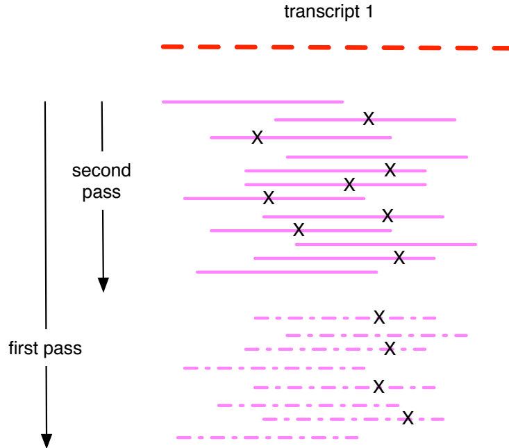
Figure 4.7 Diagram of semi-streaming error detection. In a first pass over the read data, reads are loaded in until the graph locus to which they belong is saturated. From that point on, reads are examined for errors and not loaded into the graph. In a second pass, only the subset of reads loaded into the graph are examined for errors.
