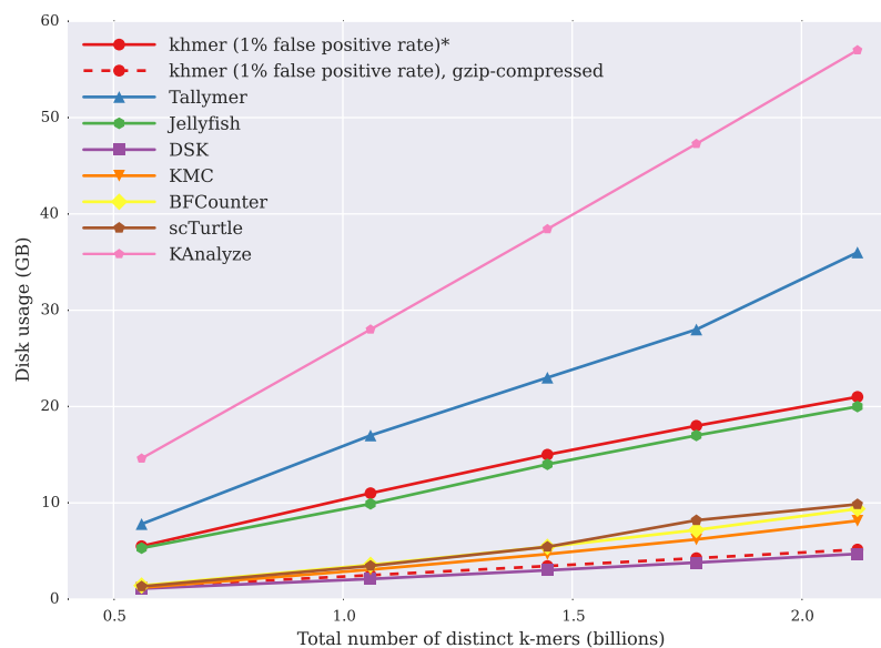
Figure 3.3 Disk storage usage of different k-mer counting tools to calculate k-mer abundance histograms in GB (y axis), plotted against the number of distinct k-mers in the data set (x axis). *Note that khmer does not use the disk during counting or retrieval, although its hash tables can be saved for reuse.
