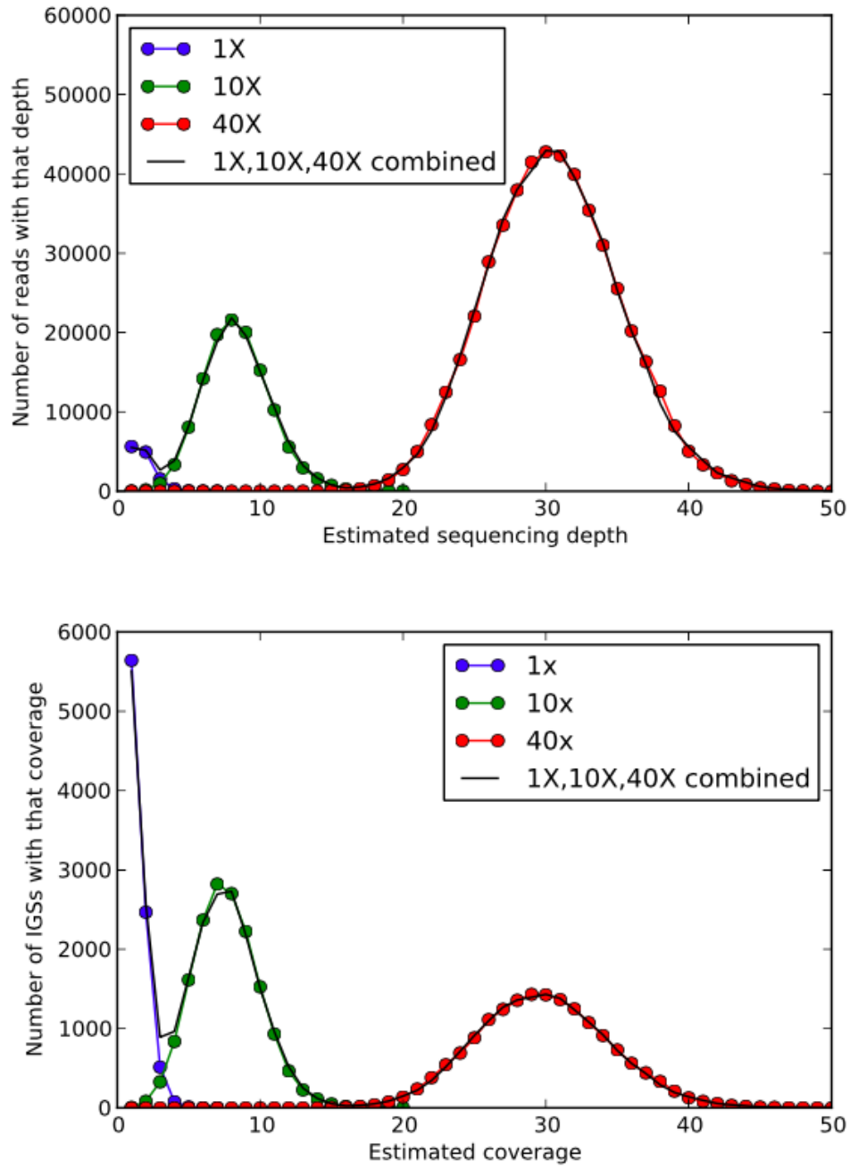
Figure 5.1 Transforming reads into IGSs.
