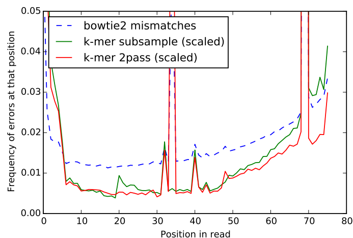
Figure 4.10 Error spectrum of reads in the mouse RNAseq data set. The sublinear k-mer spectrum analysis is calculated based on saturation of a fraction of the data set, while the two-pass spectral analysis uses all of the data, and bowtie2 mismatches are based on all mapped reads. The peak of errors at position 34 in the bowtie2 mapping reflects errors that in the first part of the data set are called as Ns, and hence are ignored by the sublinear error analysis; see text for details. Note, the bowtie2 mismatch rates are larger than the spectral rates, so for ease of comparison the y values for the k-mer spectral analyses are scaled by a factor of four.
