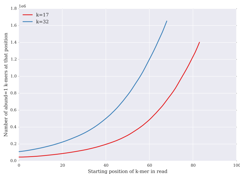
Figure 4.6 Number of unique k-mers (y axis) by starting position within read (x axis) in an untrimmed E. coli 100-bp Illumina shotgun data set, for k=17 and k=32. The increasing numbers of unique k-mers are a sign of the increasing sequencing error towards the 3' end of reads. Note that there are only 69 starting positions for 32-mers in a 100 base read.
