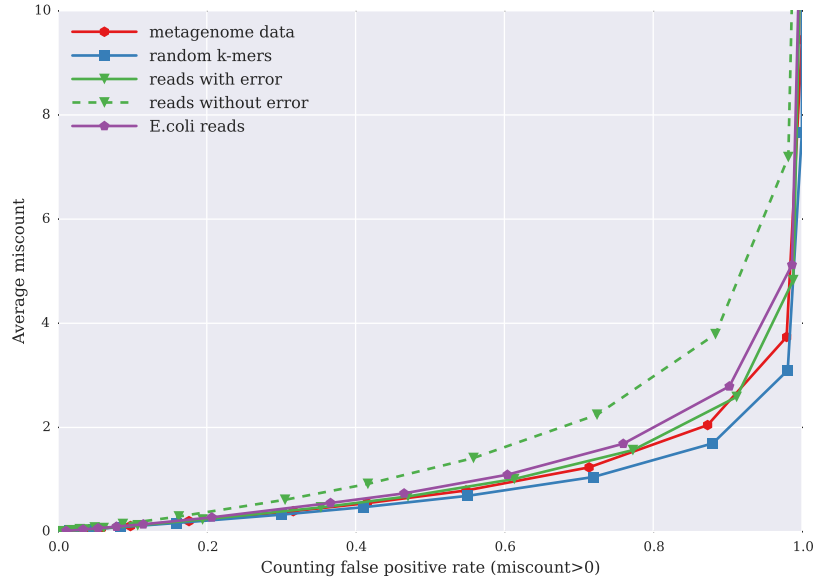
Figure 3.5 Relation between average miscount — amount by which the count for k-mers is incorrect — on the y axis, plotted against false positive rate (x axis), for five data sets. The five data sets were chosen to have the same total number of distinct k-mers: one metagenome data set; a set of randomly generated k-mers; a set of reads, chosen with 3x coverage and 1% error, from a randomly generated genome; a simulated set of error-free reads (3x) chosen from a randomly generated genome and a set of E. coli reads.
