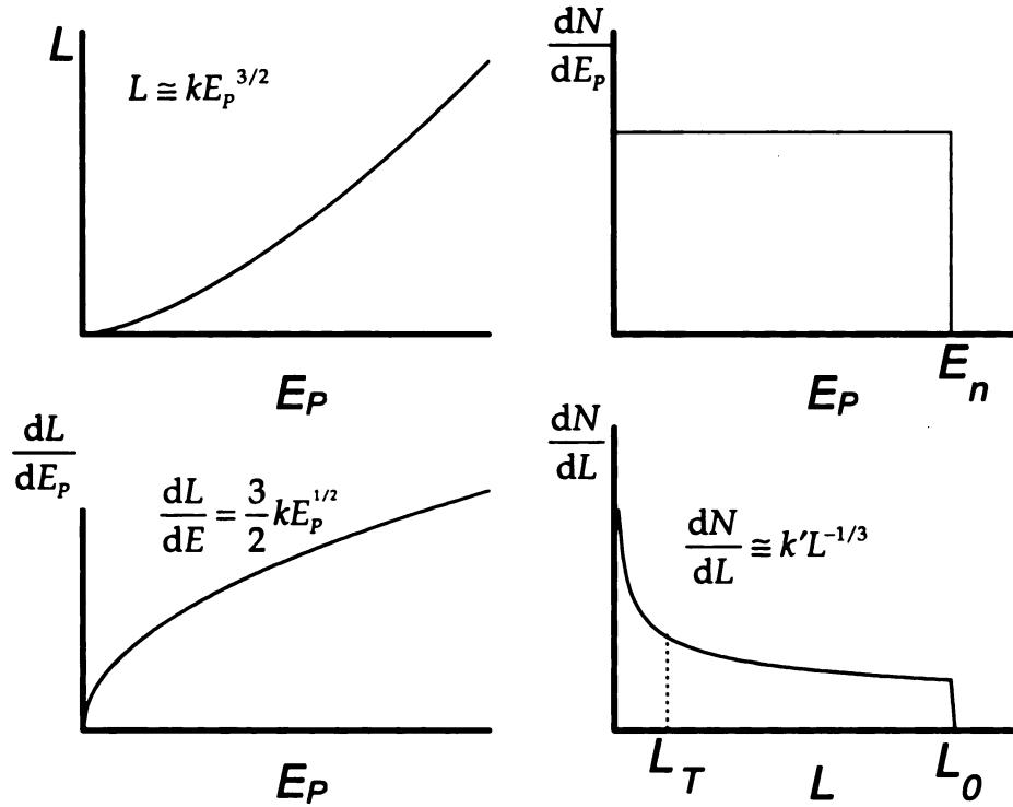
Figure 27 - The two basic contributions to the light output distribution for a monoenergetic neutron beam incident on a detector (from Knoll, ref. 27).
