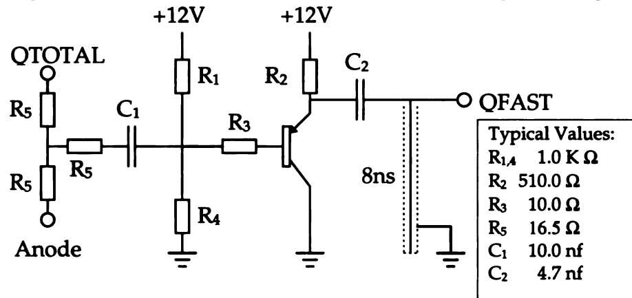
Figure 46 - A simple schematic of the method of producing the PSD signal.
