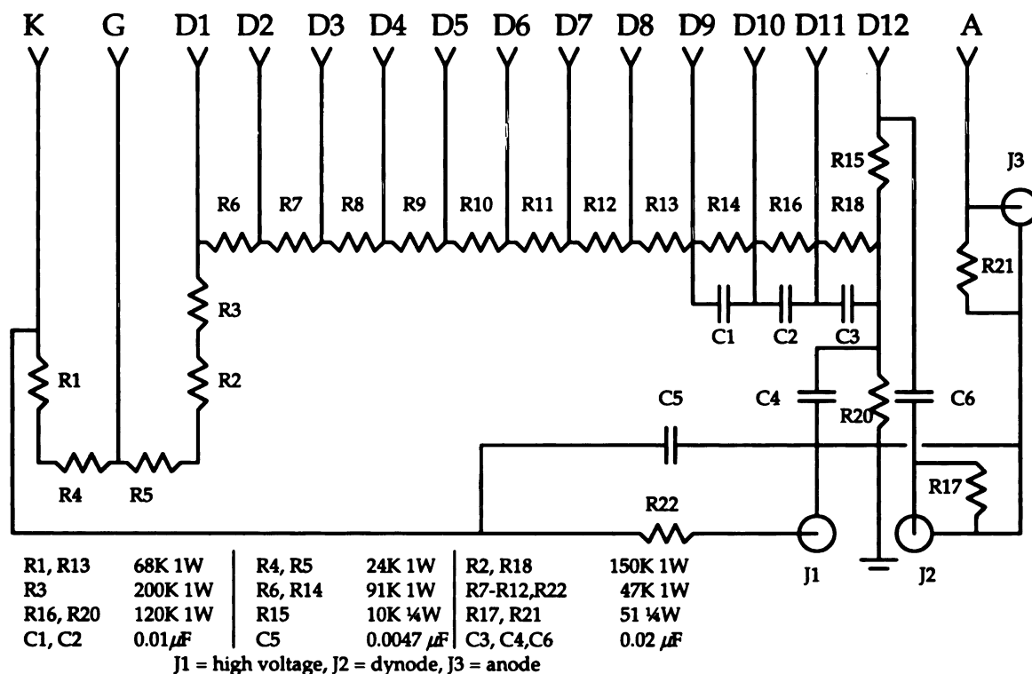
Figure 34 - Schematic drawing of the passive voltage divider used on the XP4312/04 PMT.
