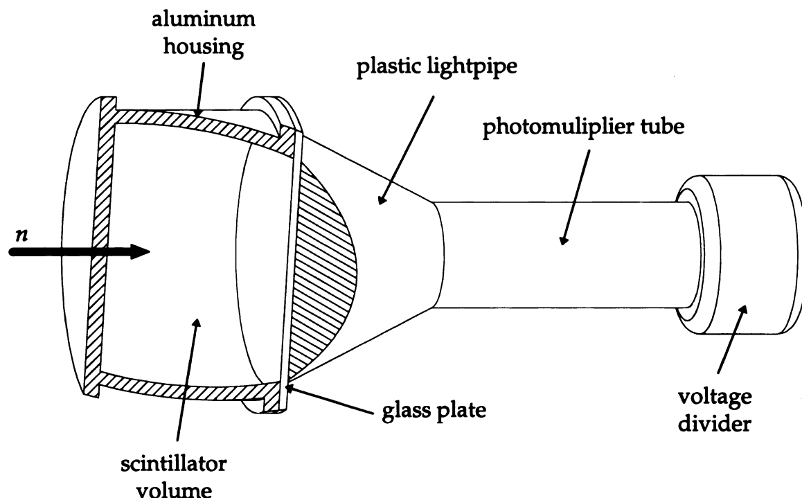
Figure 26 - A cutaway diagram of a neutron detector used by Sackett et al. Neutrons are incident from the left. The scintillator is 5 inches in diameter and 3 inches in depth for a volume of 59 in 3 (0.97 liters).
