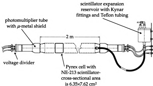
Figure 32 - A drawing of an individual detector cell from the Neutron Wall Array .
