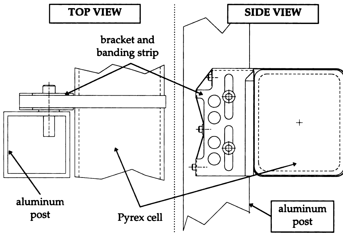
Figure 37 - Top and side view of the cell-mounting bracket.
