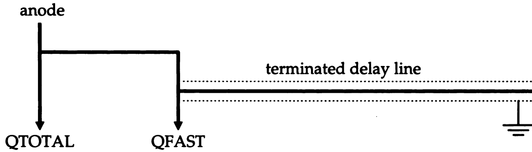
Figure 46 - A simple schematic of the method of producing the PSD signal.
