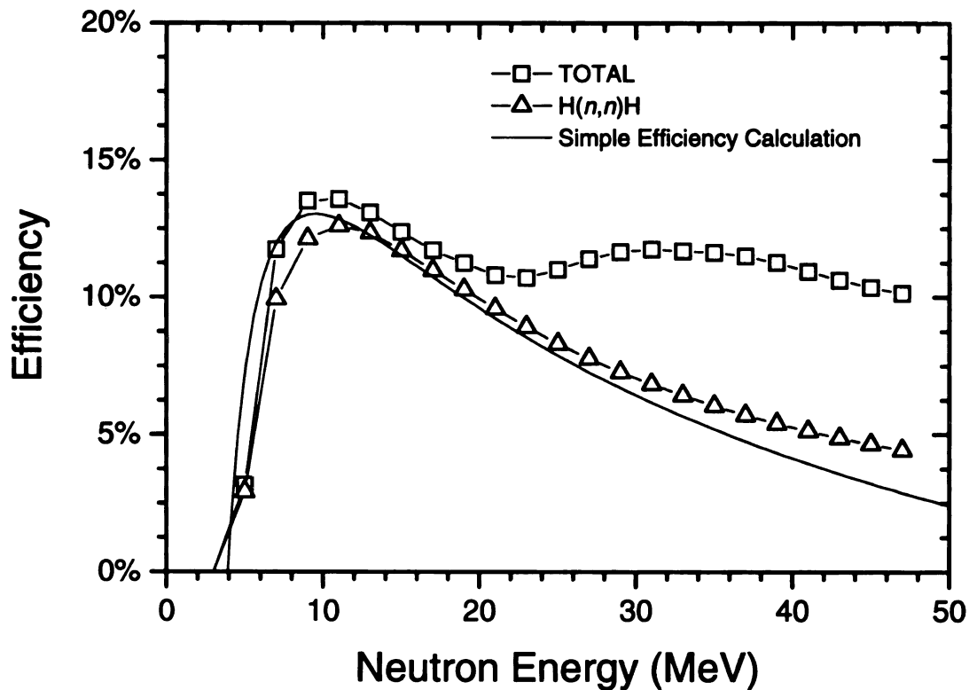
Figure 28 - Neutron detection efficiencies. The solid curve represents a simple estimate of the efficiency based on equations 12 and 15. The points represent the results of the simulation code TOTEFF. The triangle data points represent the efficiency from (n,p) scattering, and the square data points represent the total efficiency for the same detector.
