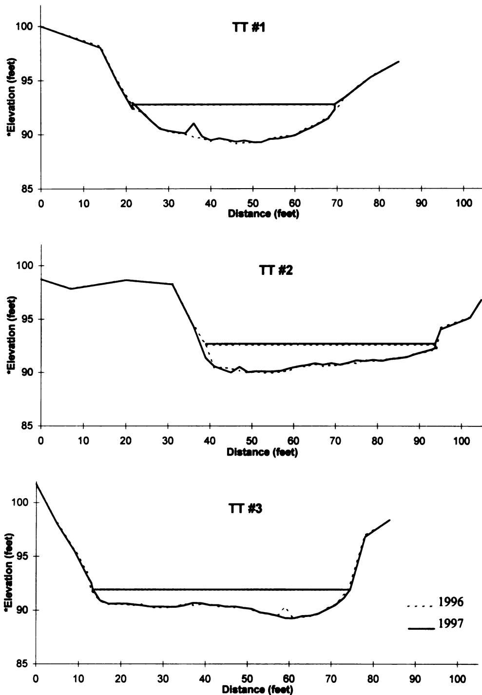
Figure 7. Streambed profiles of the Tip of the Tit (TT) series for 1996 and 1997. These transects are located approximately 6.3 km upstream from Stronach Dam, within the non-impacted zone. *Assumed elevations where USGS datum not available.
