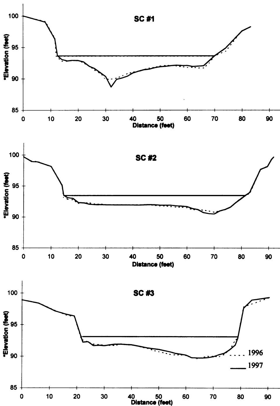
Figure 10. Streambed profiles of the Schofield (SC) series for 1996 and 1997. These transects are located approximately 2.4 km upstream from Stronach Dam, within the impacted zone. *Assumed elevations where USGS datum not available.
