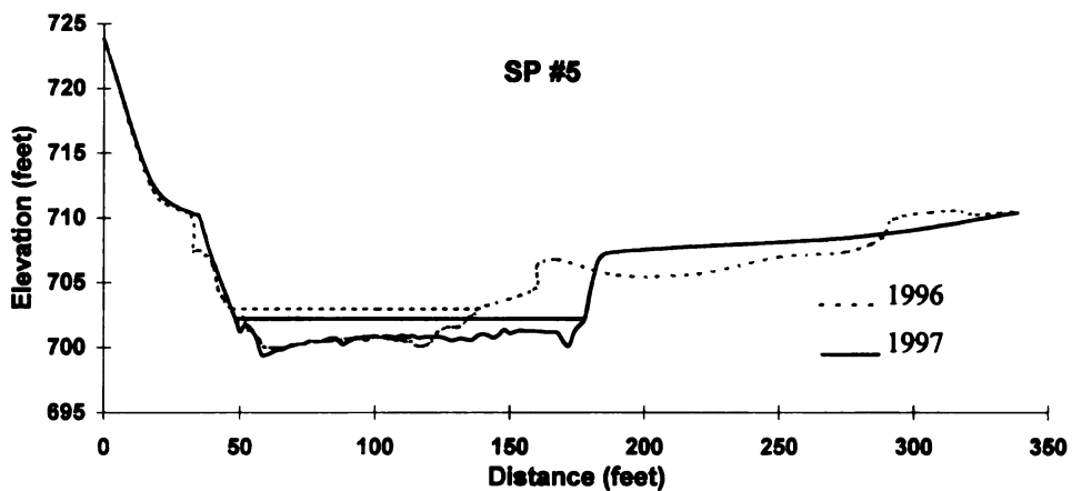
Figure 13 (cont'd.). Streambed profiles of the Stronach Pond (SP) series for 1996 and 1997. These transects are located within approximately 0.6 km of, and upstream from, Stronach Dam, within the impacted zone. (Actual elevations from USGS.)
