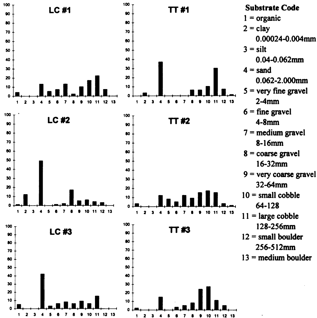
Figure 15. 1997 substrate particle size distributions at LC and TT transects located 7.0 km and 6.3 km upstream from Stronach Dam, respectively, within the non-impacted zone.
