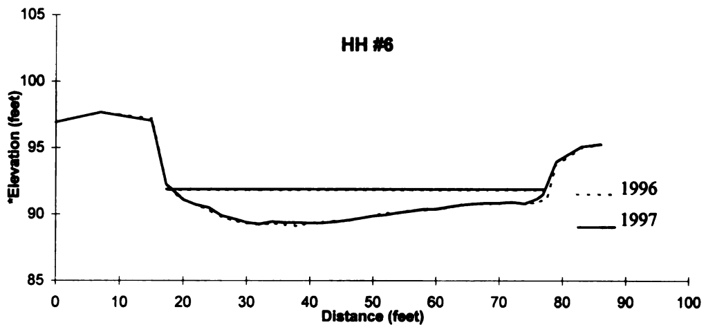
Figure 8 (cont'd.). Streambed profiles of the Harley Hill (HH) series for 1996 and 1997. These transects are located approximately 5.3 km upstream from Stronach Dam, within the non-impacted zone. *Assumed elevations where USGS datum not available.
