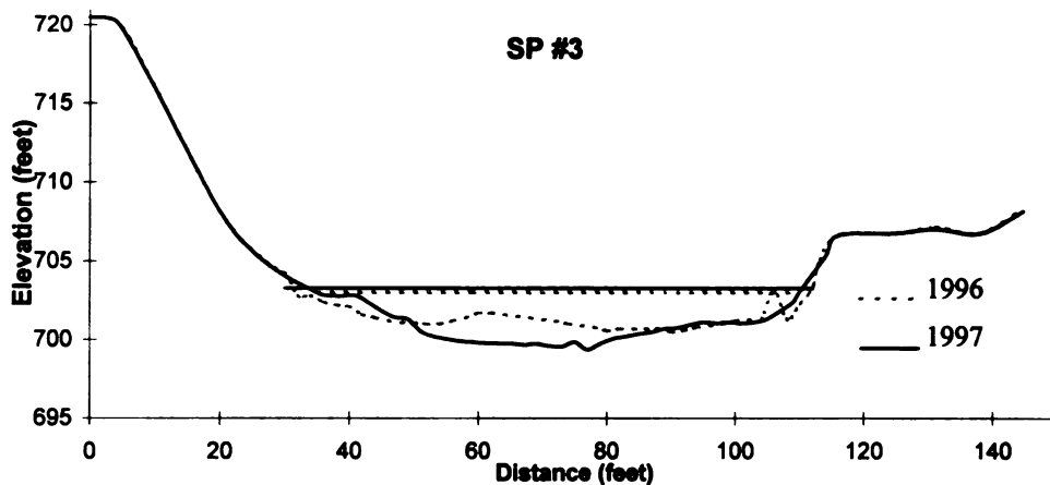
Figure 13. Streambed profiles of the Stronach Pond (SP) series for 1996 and 1997. These transects are located within approximately 0.6 km of, and upstream from, Stronach Dam, within the impacted zone. (Actual elevations from USGS.)
