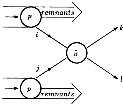
Figure 2.3: Factorization of the p\bar{p} matrix element.
