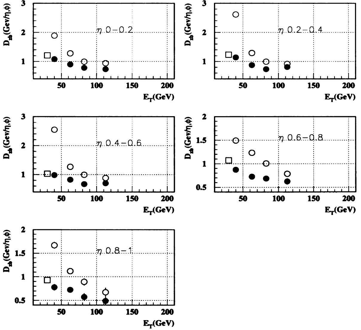
Figure B.3: The smeared (open circles) and unsmeared (full circles) D_{zb} offset for 0.7 cone jets. Both sets of points differ only by the weight assigned to the generated jets. The open box shows for reference the result from the JES D0Note.
