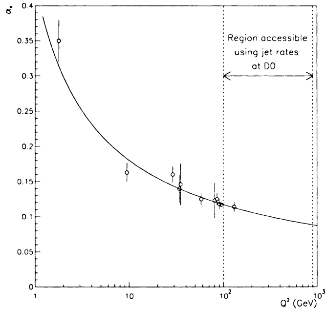
Figure 2.5: Graphical representation of the data from Table 2.5. The curve corresponds to the next-to-leading order running of \alpha_s(Q^2) setting \alpha_s(M_Z) = 0.119 . The region accessible using jet rates at DØ is also shown.
