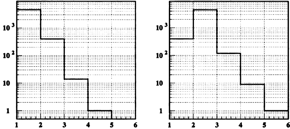
Figure 7.3: Ranking of overlaid k_{\perp} jets compared to non-overlaid jets. Corresponding z5 k_{\perp} jet matched to the leading ( left ) and second leading ( right ) xx k_{\perp} jet. Jets are numbered in decreasing order according to their E_T .
