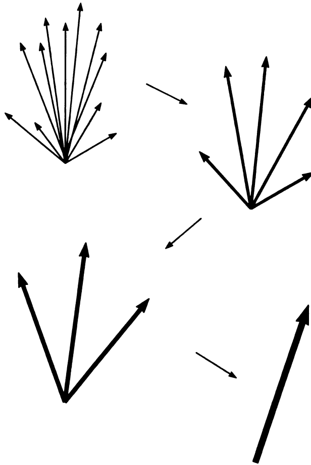
Figure 5.3: k_{\perp} jet clustering.
