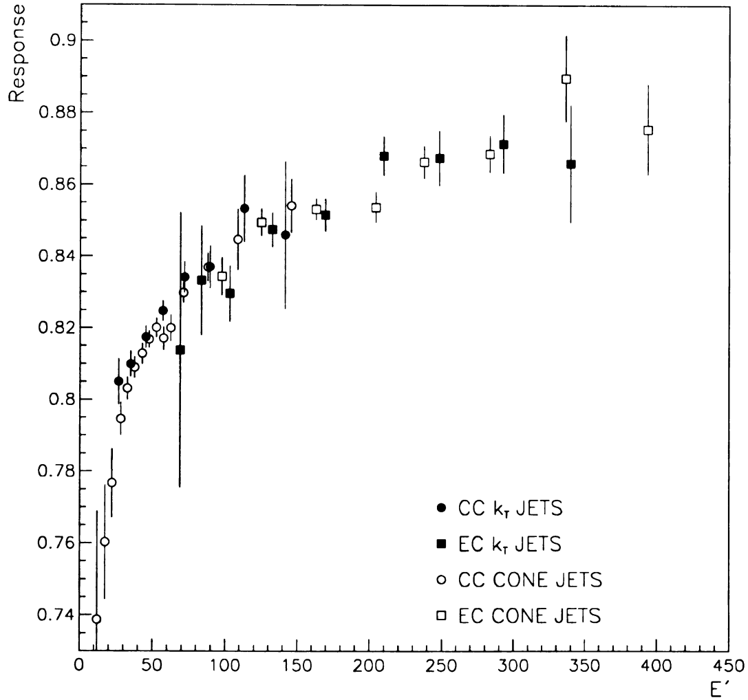
Figure 8.1: Response versus E' . Open symbols are from the full \gamma -jet data sample and solid symbols are from the smaller sample reconstructed with k_{\perp} jets. The additional DØFIX cryostat corrections were removed from k_{\perp} jets.
