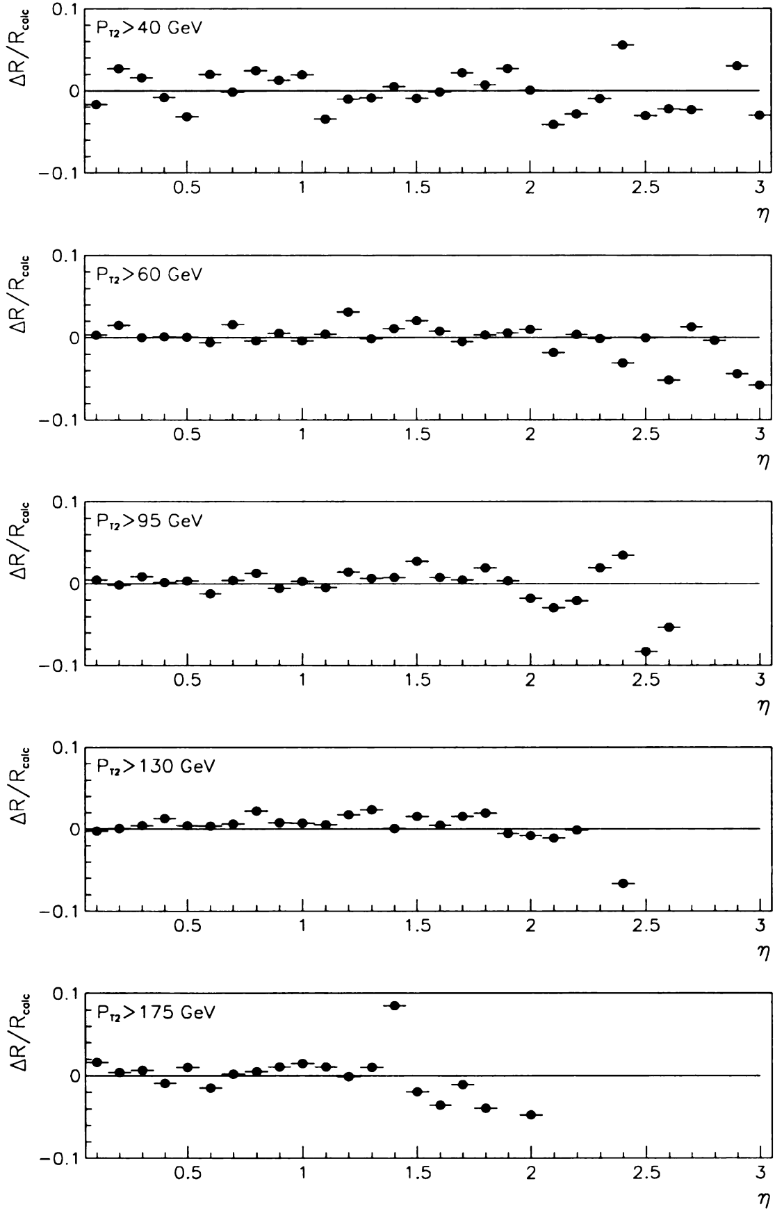
Figure 8.15: The fractional difference between R_{\text{meas}} and R_{\text{calc}} for partially corrected jets. \Delta R = (R_{\text{meas}} - R_{\text{calc}}) / R_{\text{calc}} .
