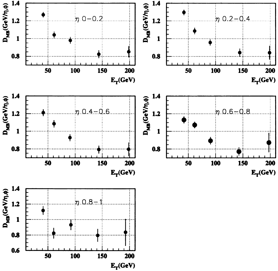
Figure B.6: Dependence of m0-xx on E_T for cone jets
