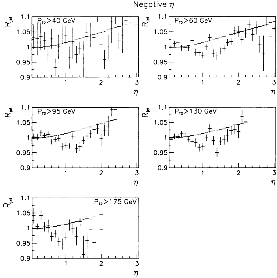
Figure 8.6: Response versus \eta < 0.0 for jet-jet data.
