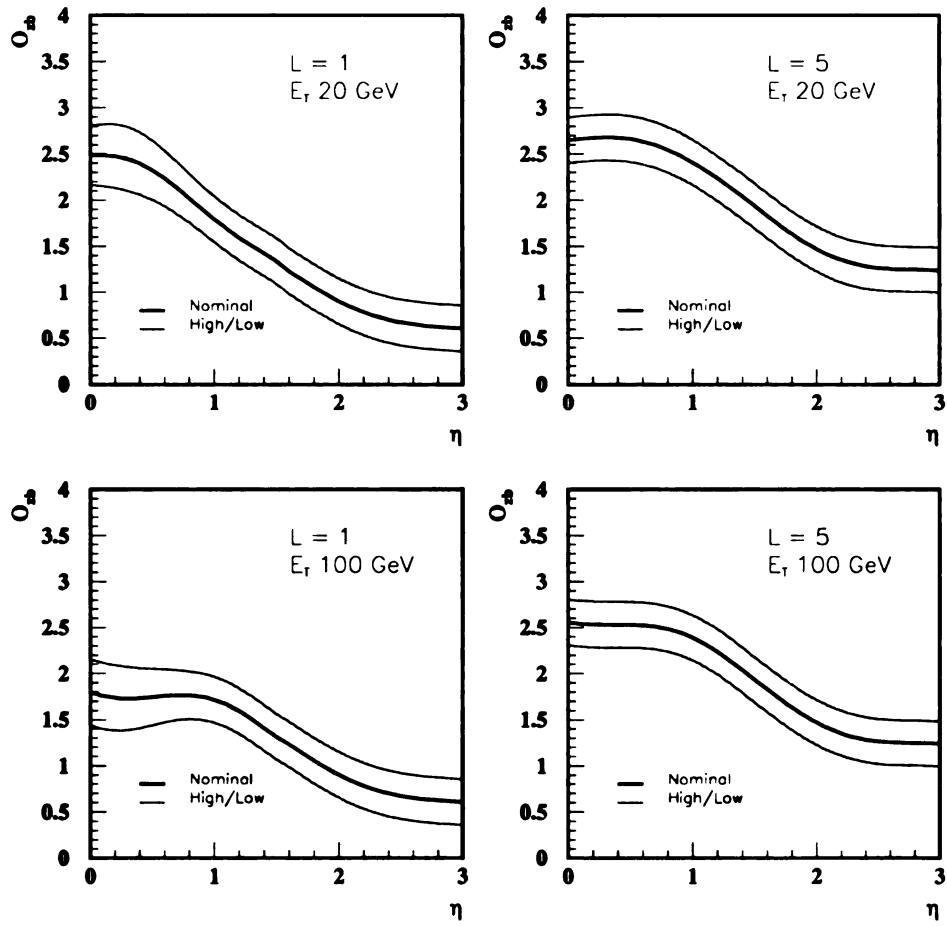
Figure 7.13: O_{zb} \eta dependence and errors for k_{\perp} jets with jet E_T equalling 20 and 100 GeV at \mathcal{L}=1 and \mathcal{L}=5 .
