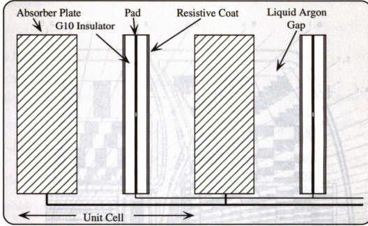
Figure 4.5: Schematic view of a liquid argon readout cell.
