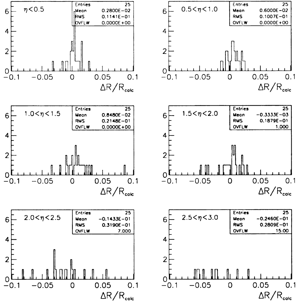
Figure 8.16: The distributions of fractional differences between R_{\text{meas}} and R_{\text{calc}} .
