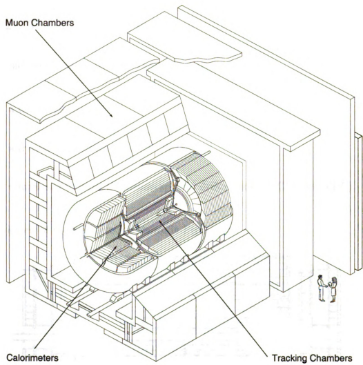
Figure 4.2: Cutaway view of the DØ detector.
