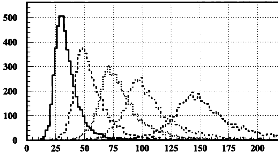
Figure 7.4: Distribution of reconstructed E_T for k_\perp jets without noise overlay. The different line types correspond to samples generated with parton E_T thresholds of 30, 50, 75, 100 and 150 GeV.
