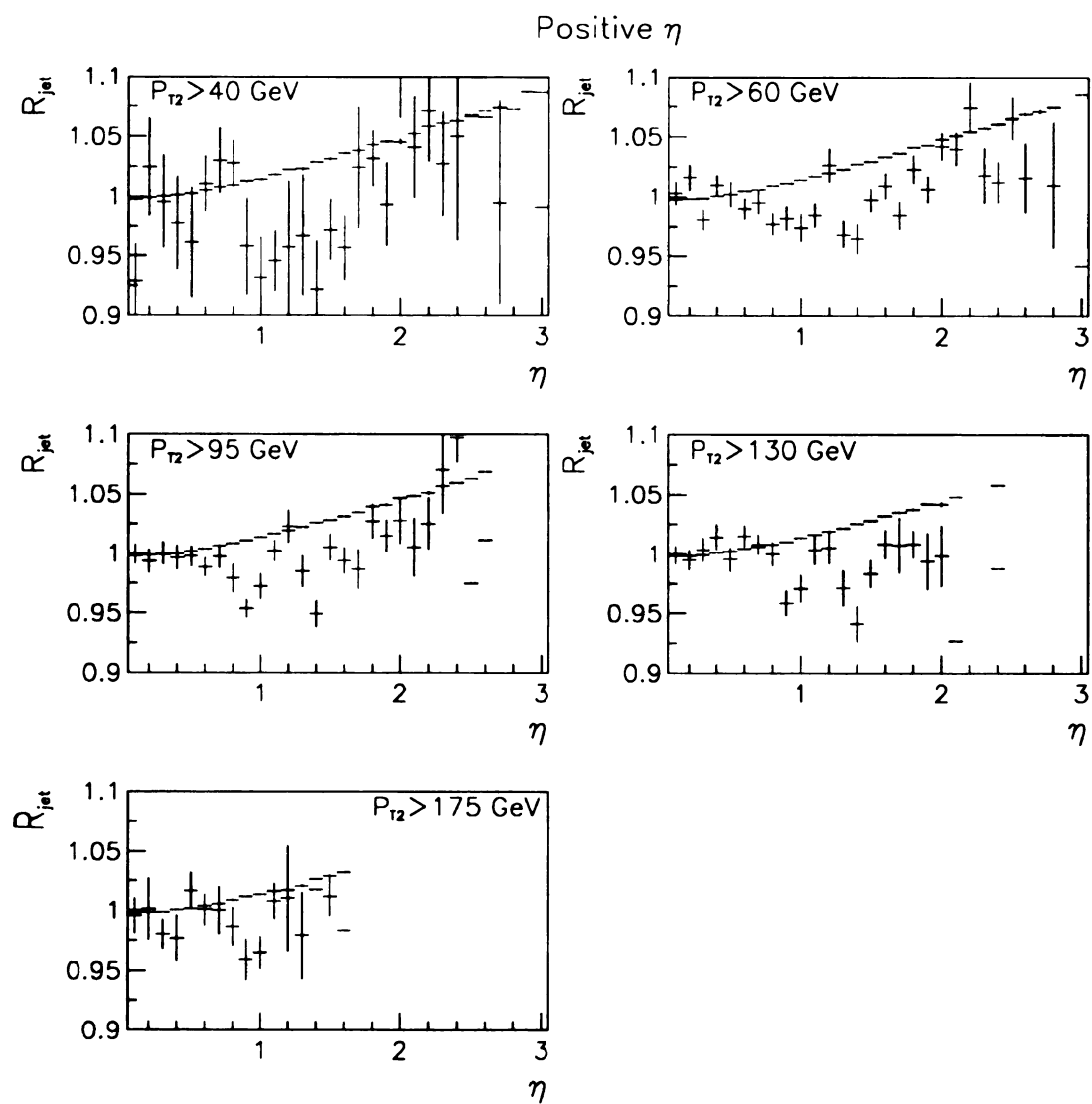
Figure 8.5: Response versus \eta > 0.0 for jet-jet data.
