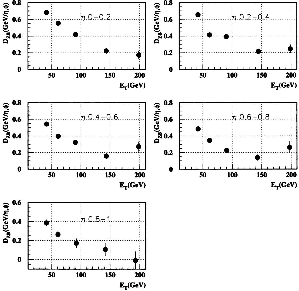
Figure B.7: Dependence of zb-xx on E_T for cone jets. The dependence is the same as in the previous figure, and cancels when getting D_{ue} by taking the difference
