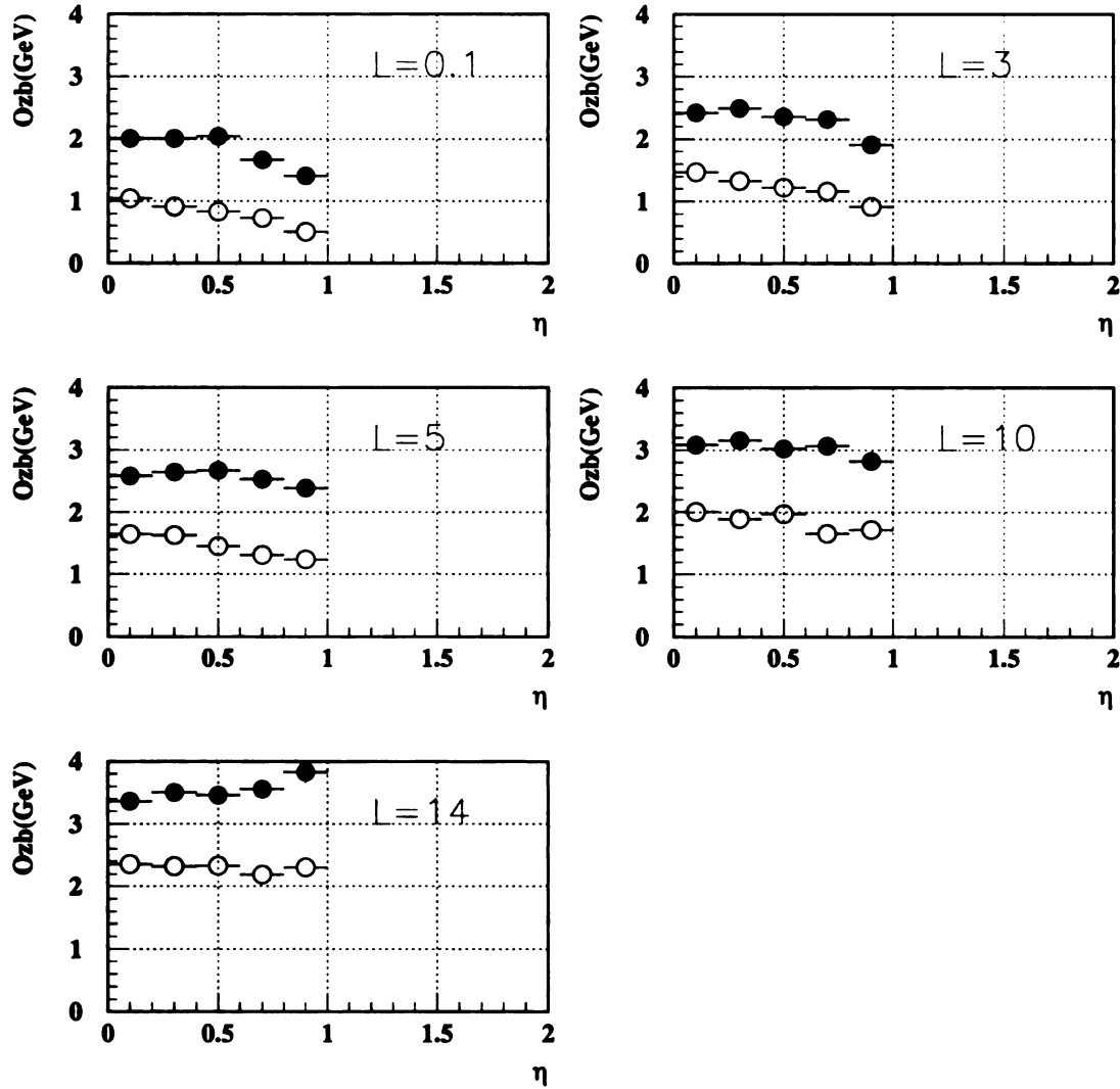
Figure 7.9: O_{zb} offset vs \eta for k_{\perp} jets with 30 < E_T < 50 GeV. The result for cones (open circles) is shown for comparison.
