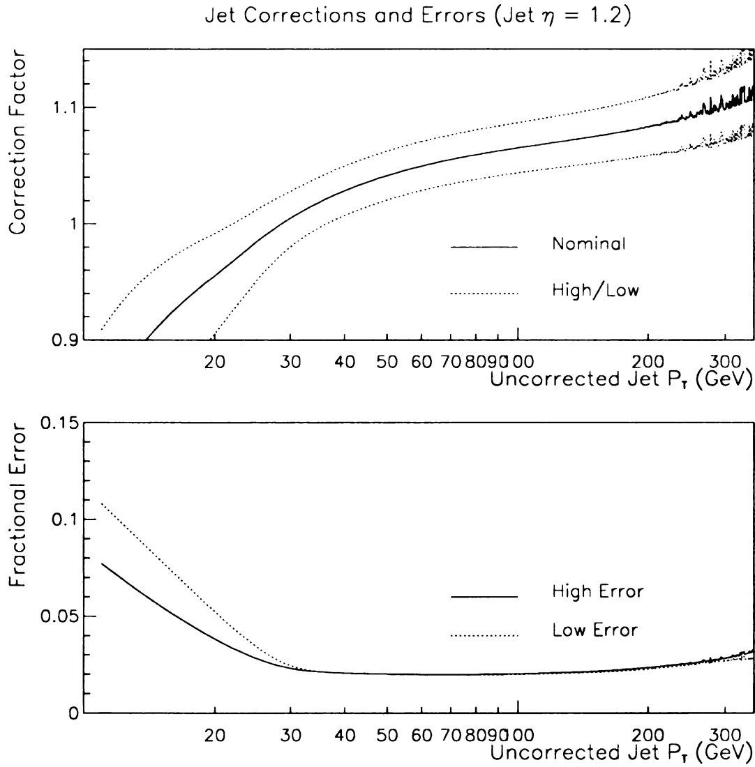
Figure 10.2: Corrections and Errors for \eta_{Ktjet} = 1.2 . Top: Nominal, high, and low correction factors. Bottom: high and low fractional errors.
