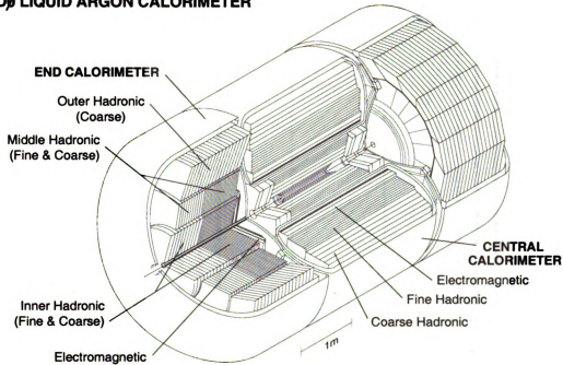
Figure 4.4: Cutaway view of the DØ calorimeter detector.
