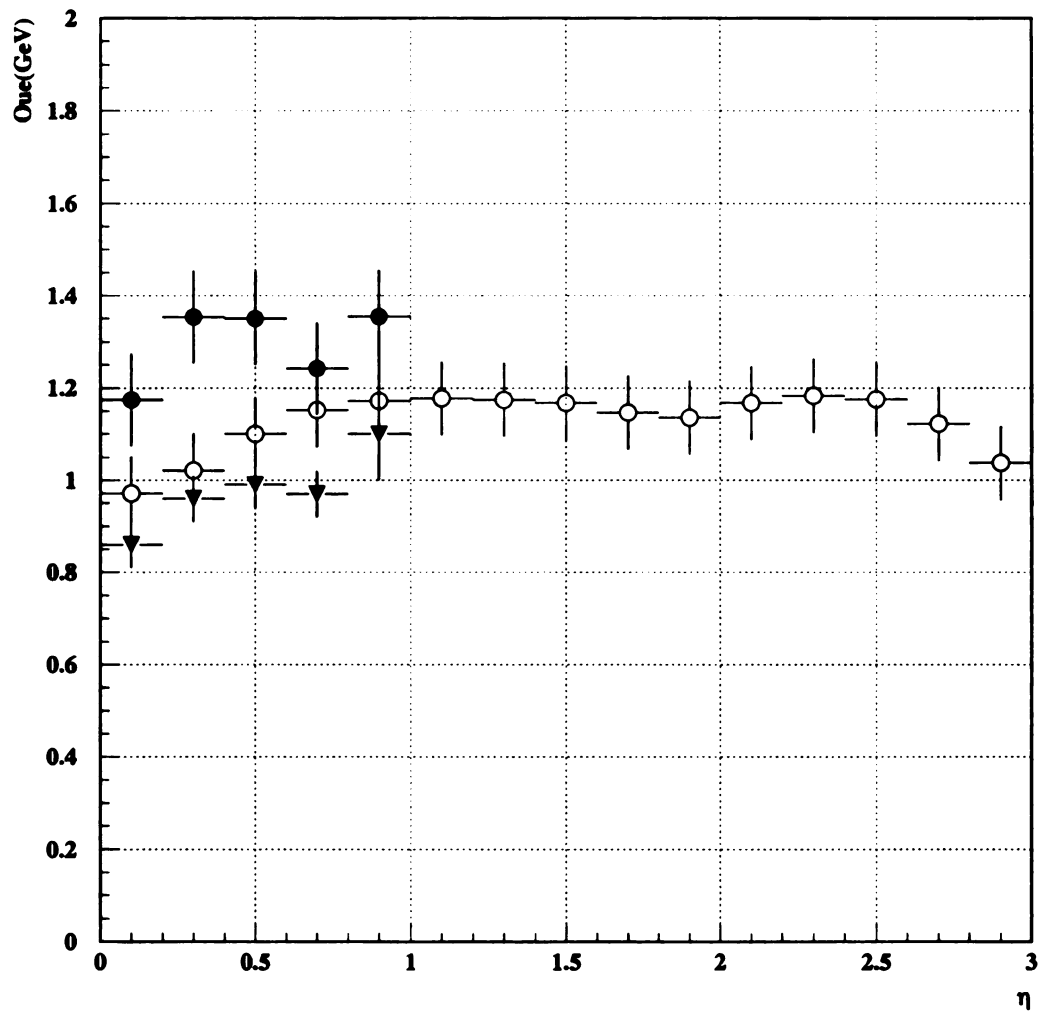
Figure 7.15: Measured O_{ue} vs k_{\perp} jet \eta (solid circles) and cone jets \eta (triangles), together with the results from the CAFIX5.1 (open circles).
