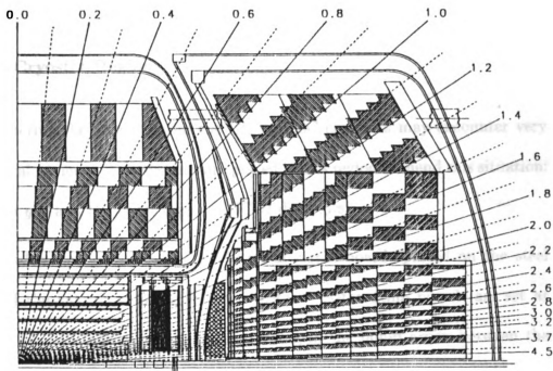
Figure 4.6: One quadrant of the DØ calorimeter.
