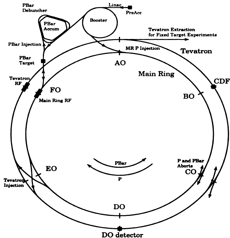
Figure 4.1: Overview of the Fermilab Tevatron.
