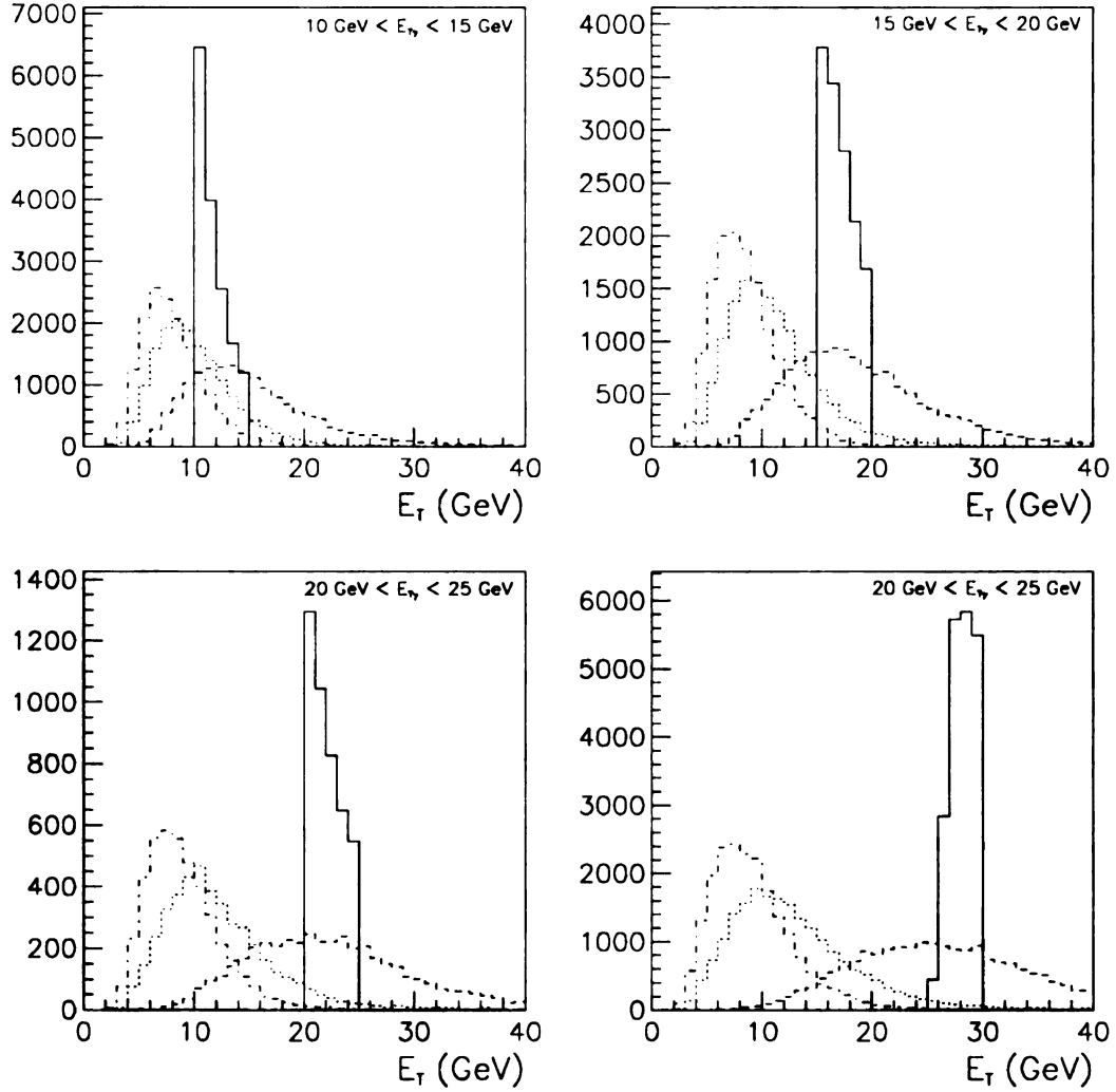
Figure 8.12: E_T distribution of k_\perp jets. Solid lines show E_{T\gamma} distributions and dotted and dashed lines show E_T distributions of the 1st, 2nd and 3rd jets.
