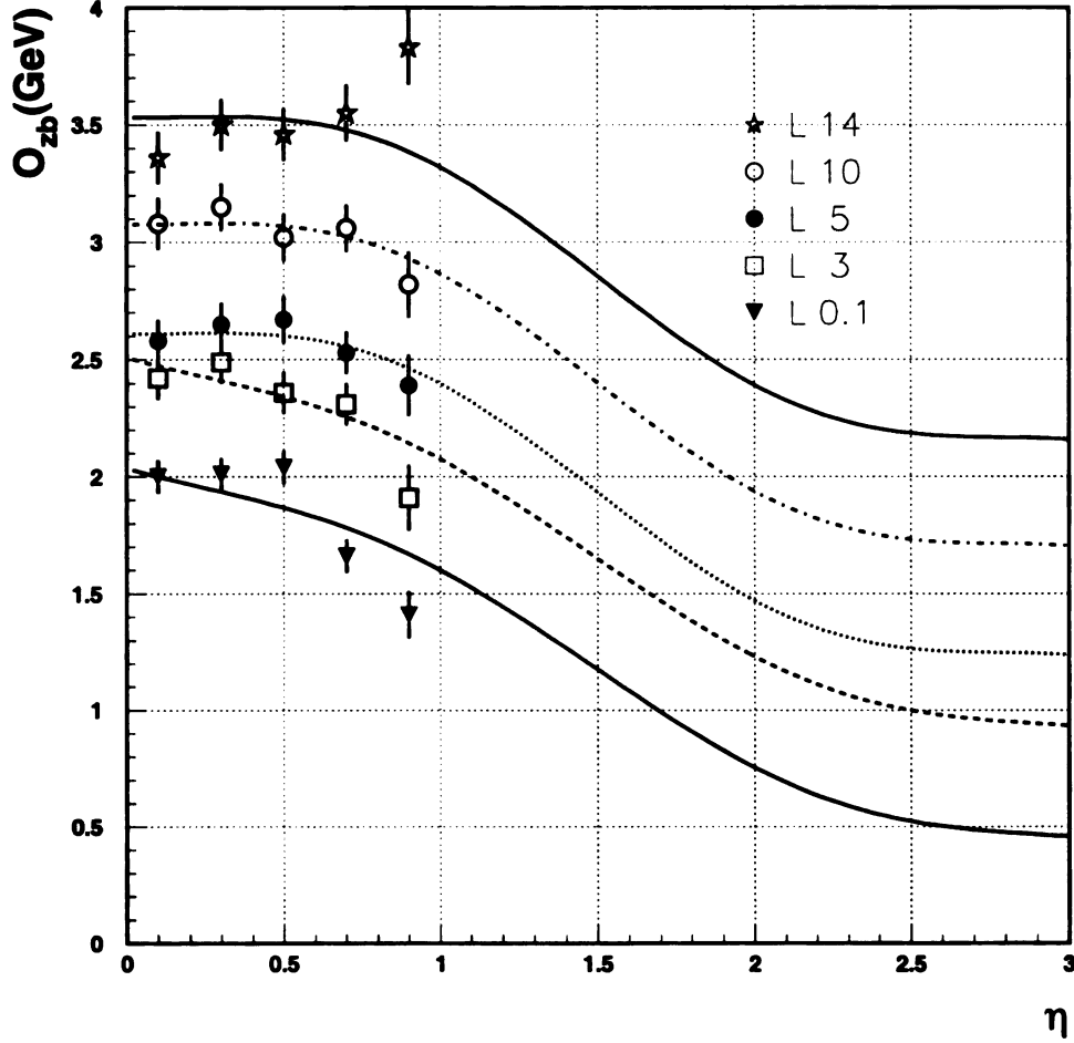
Figure 7.11: Parametrization of O_{zb} vs. k_{\perp} jet \eta for jets with 30 < E_T < 50 GeV, for various luminosities.
