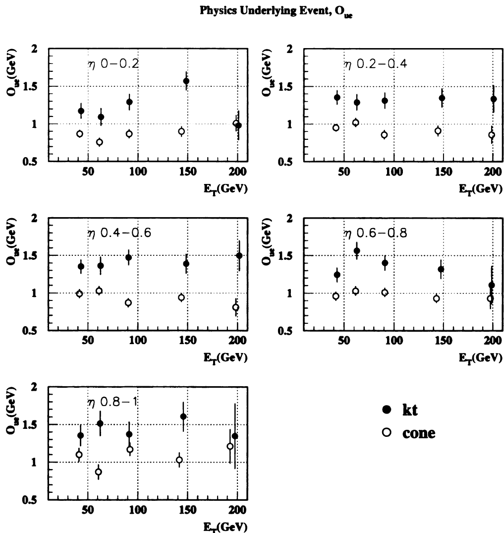
Figure 7.14: Measured O_{ue} vs E_T for k_\perp jets. The result for cones is shown for comparison.
