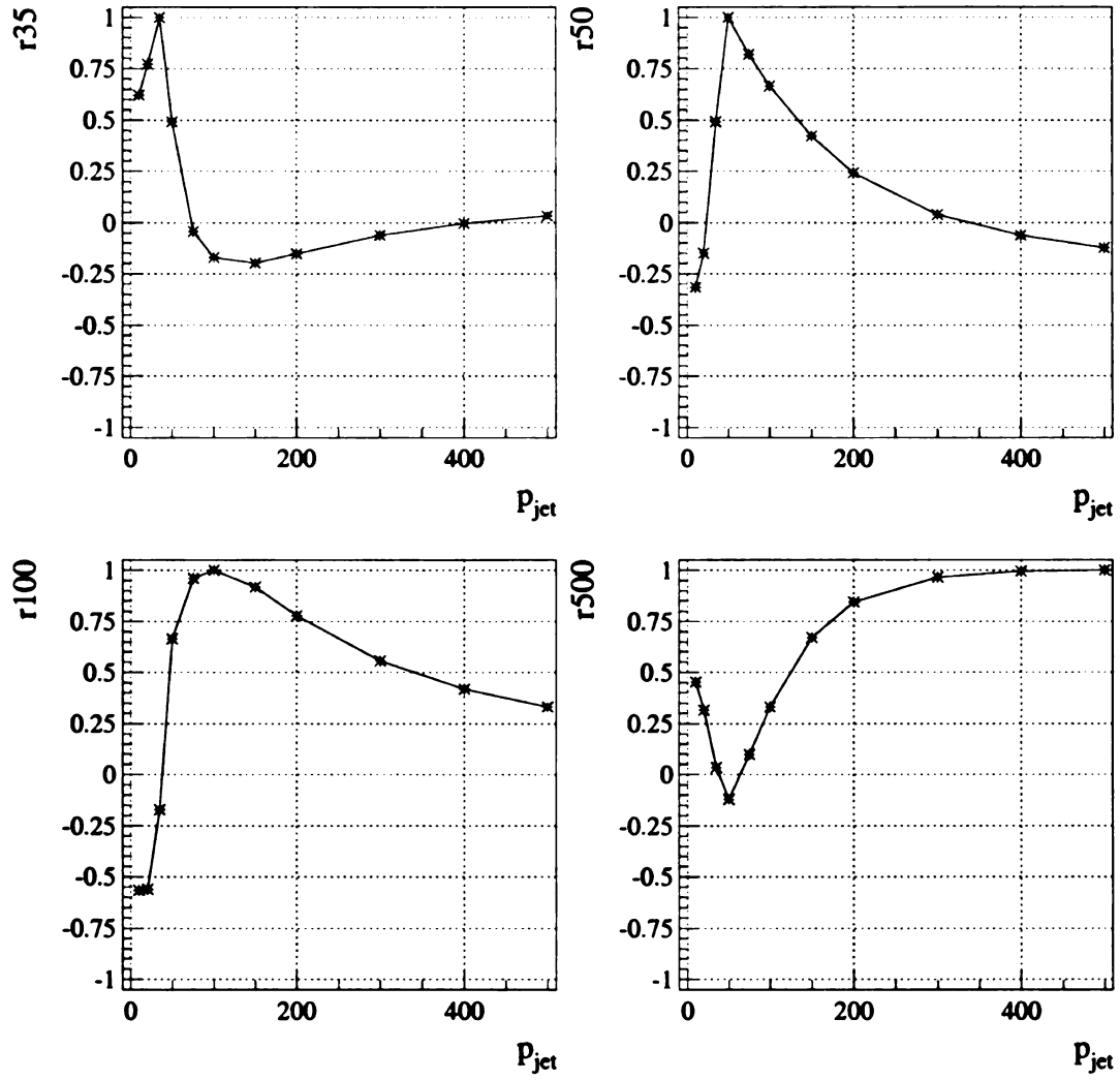
Figure 8.14: Error correlations for k_{\perp} jet response fit. Error correlations are shown in four slices from the full correlation matrix. The four curves show the point-to-point correlation of fit errors relative to momentum values of 35, 50, 100, and 500 GeV respectively.
