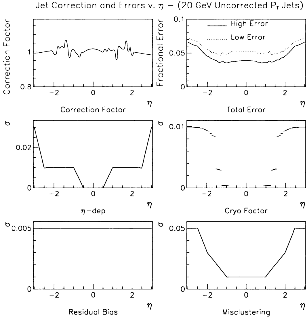
Figure 10.4: Corrections and Errors versus \eta_{Ktjet} , k_{\perp} Jet P_T = 20 GeV. The total correction and error are both shown as well as the eta dependence of several individual components of the jet scale error.
