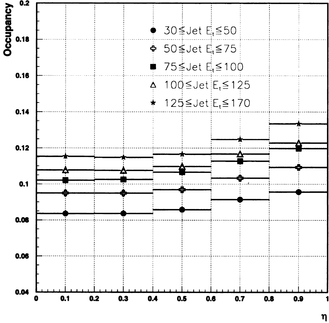
Figure B.5: Jet energy dependence of occupancy for zero bias luminosity 5 and R = 0.7 cone jets.
