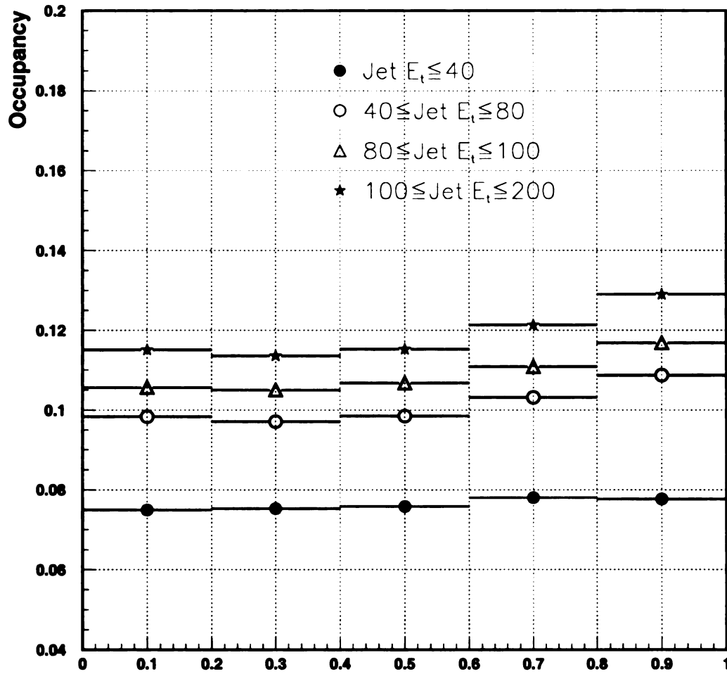
Figure 7.6: 0.7 cone jet occupancy vs. jet \eta for jets found in Monte Carlo with minimum bias overlay data.
