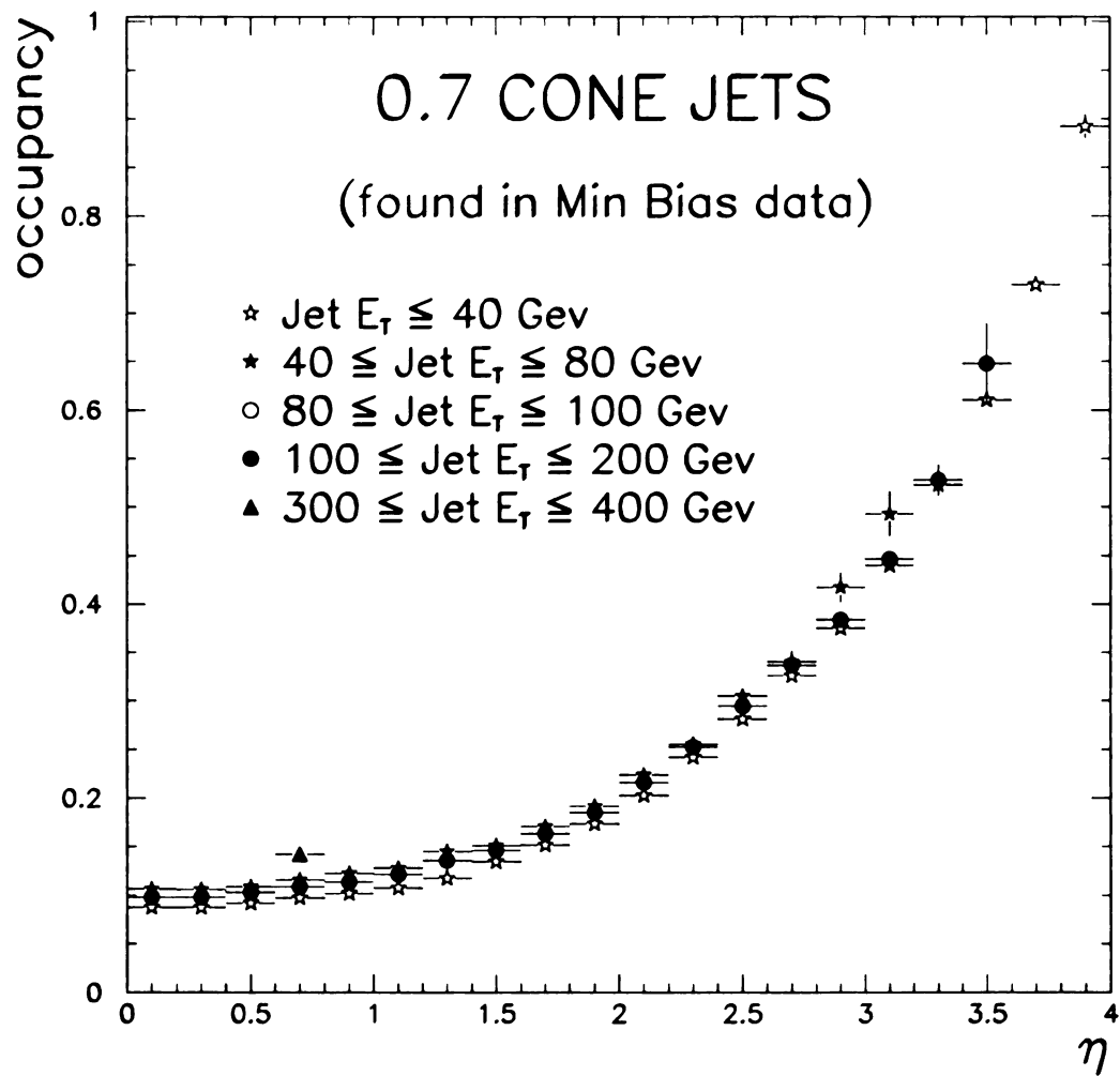
Figure 7.5: 0.7 cone jet occupancy vs. jet \eta for jets found in minimum bias data.
