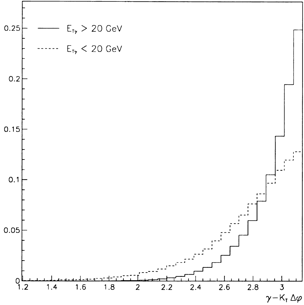
Figure 8.11: \Delta\phi_{\gamma \text{ jet}} normalized distribution for k_{\perp} jets ( \Delta\phi_{\gamma \text{ jet}} = |\phi_{\gamma}| - |\phi_{\text{jet}}| ).
