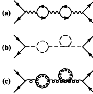
Figure 2.2: Feynman loop diagrams. (a) Fermion loops in the photon propagator. (b) W and Z loops in the Z propagator. (c) gluon loops in the gluon propagator.
