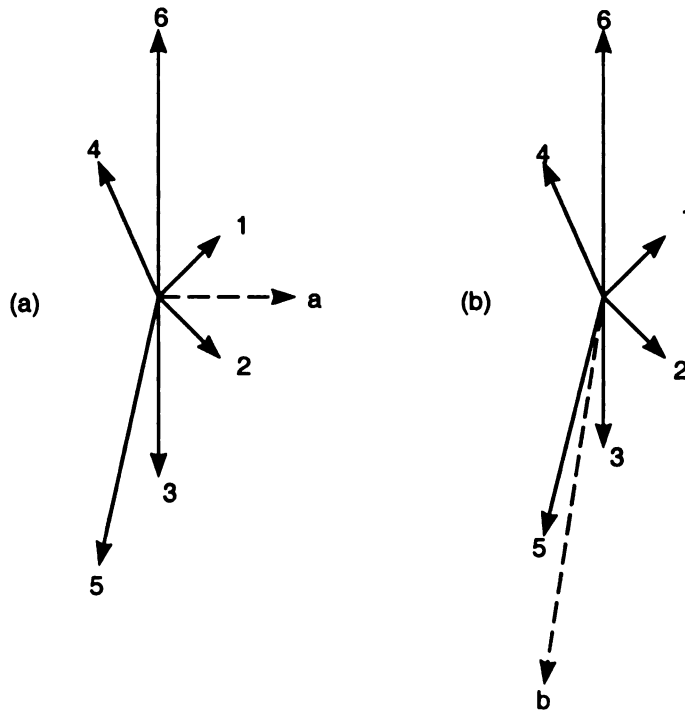
Figure 5.4: Jet Clustering in e^+e^- Collisions. (a) The JADE algorithm. (b) The k_{\perp} (or Durham) algorithm.
