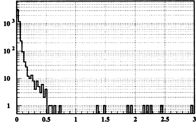
Figure 7.1: Distance in \eta - \phi space from the leading xx k_{\perp} jet to the closest z5 k_{\perp} jet.
