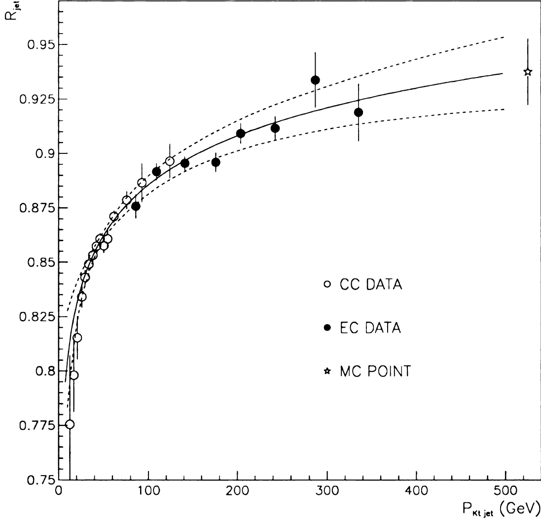
Figure 8.3: R_{jet} versus P_{kt} . The outer band shows limits on the measured jet response for high momentum jets based on the region in parameter space defined by the \chi^2 = \chi^2_{min} + 3.5 surface. This region corresponds to the 68% confidence region of parameter fluctuations from the nominal values.
