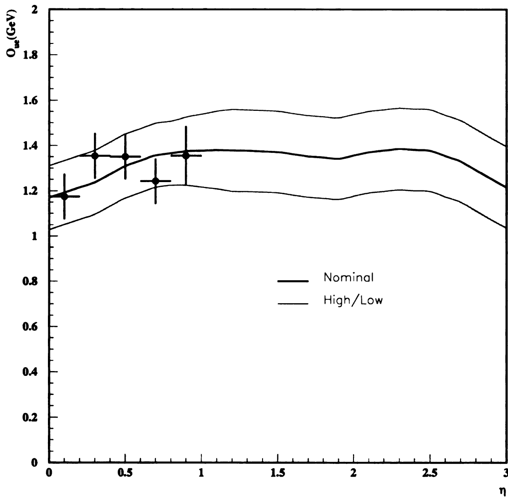
Figure 7.16: O_{ue} correction vs k_{\perp} jet \eta . The points show the measured offset for k_{\perp} jets.
