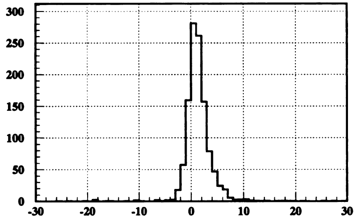
Figure 7.2: Distribution of E_T differences between corresponding k_{\perp} jets in the z5 and xx samples
