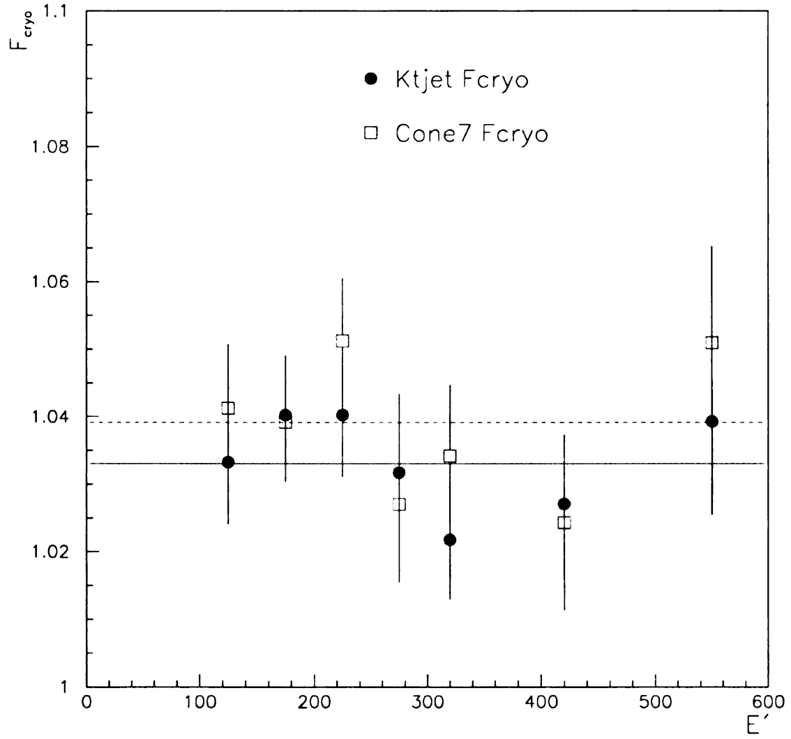
Figure 9.1: Monte Carlo Cryostat Factor. Circles are for k_{\perp} jets and squares are for cone jets. Solid line is a fit to constant for the k_{\perp} jet points; dashed line is a fit to constant for the cone jet points. Errors are statistical only.
