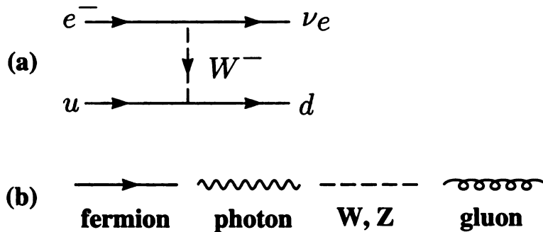
Figure 2.1: (a) Feynman diagram for e^- u \rightarrow \nu_e d by W exchange. Time flows from left to right. (b) Fermions are depicted by a solid line with an arrow pointing in the forward direction of time (an arrow in the reverse direction denotes an antiparticle). Photons are represented by a wavy line, W and Z bosons by a dashed line, and gluons by a helix.
