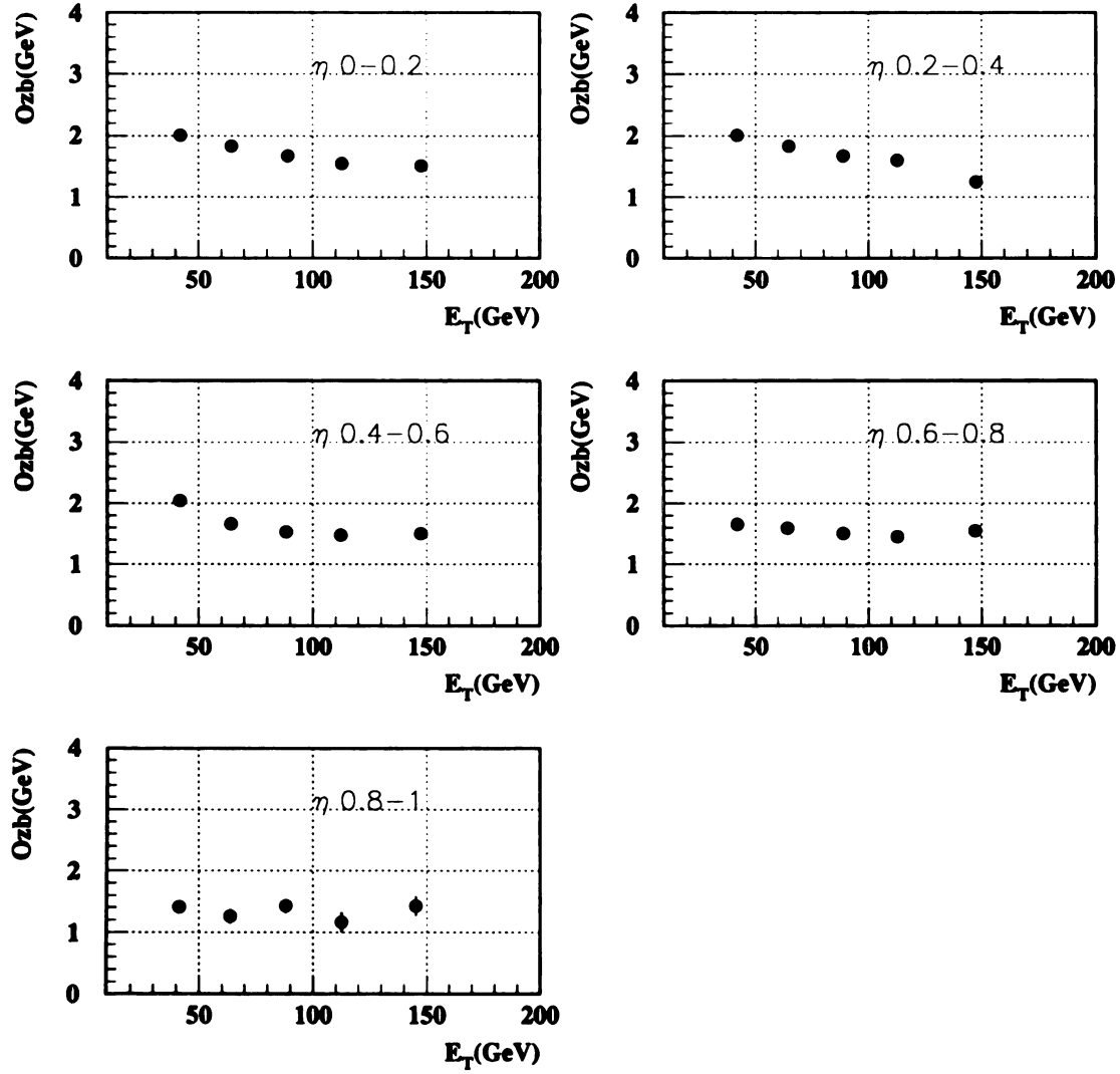
Figure 7.7: Measured O_{zb} vs. k_{\perp} jet E_T at \mathcal{L}=0.1 \times 10^{30} \text{cm}^{-2} \text{sec}^{-1} .
