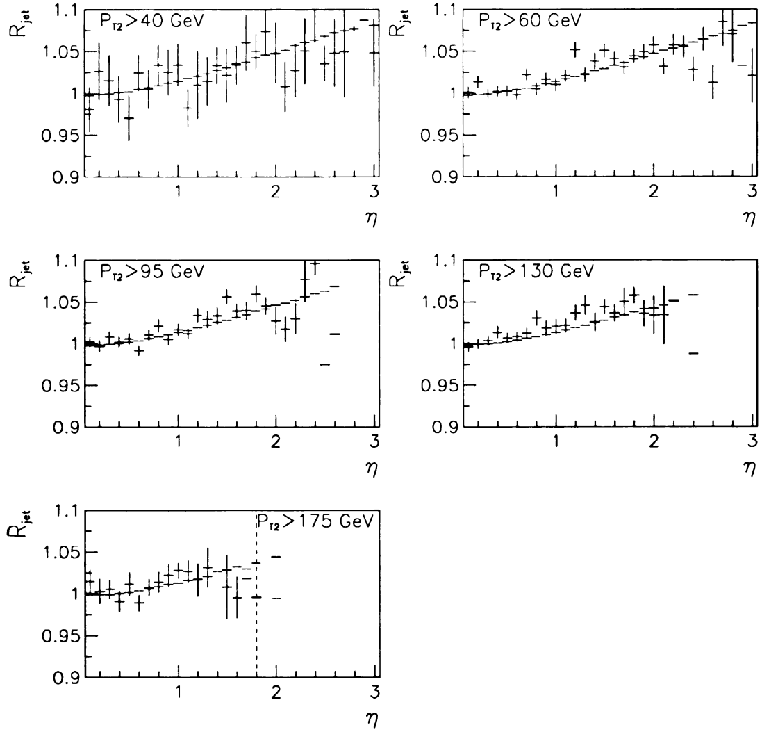
Figure 8.9: Response versus \eta after \eta dependent corrections.
