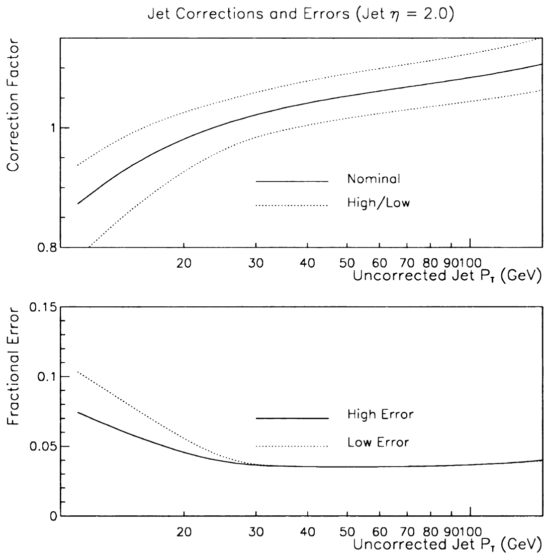
Figure 10.3: Corrections and Errors for \eta_{Ktjet} = 2.0 . Top: Nominal, high, and low correction factors. Bottom: high and low fractional errors.
