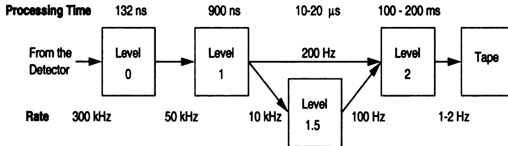
Figure 4.7: Block diagram of the DØ trigger system.
