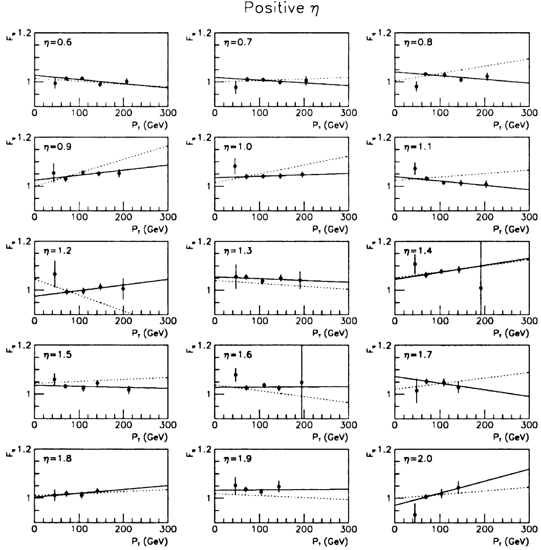
Figure 8.7: Correction factor F_\eta as a function of central jet P_T for positive \eta . The solid straight line is a fit to the data. The dotted line is the CAFIX5.1 correction for 0.7 cone jets.
