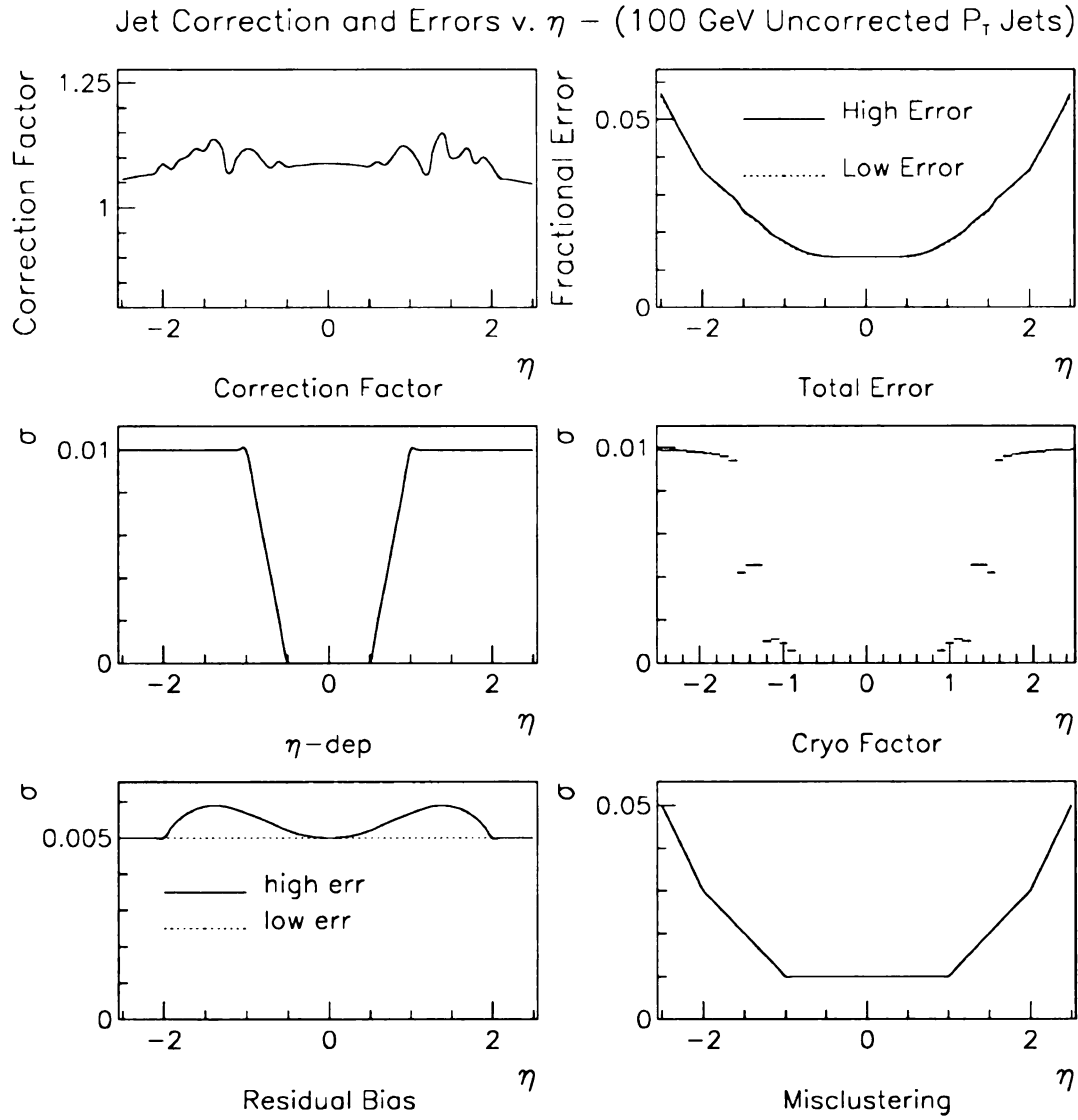
Figure 10.5: Corrections and Errors versus \eta_{Ktjet} , k_{\perp} Jet P_T = 100 GeV. The total correction and error are both shown as well as the eta dependence of several individual components of the jet scale error.
