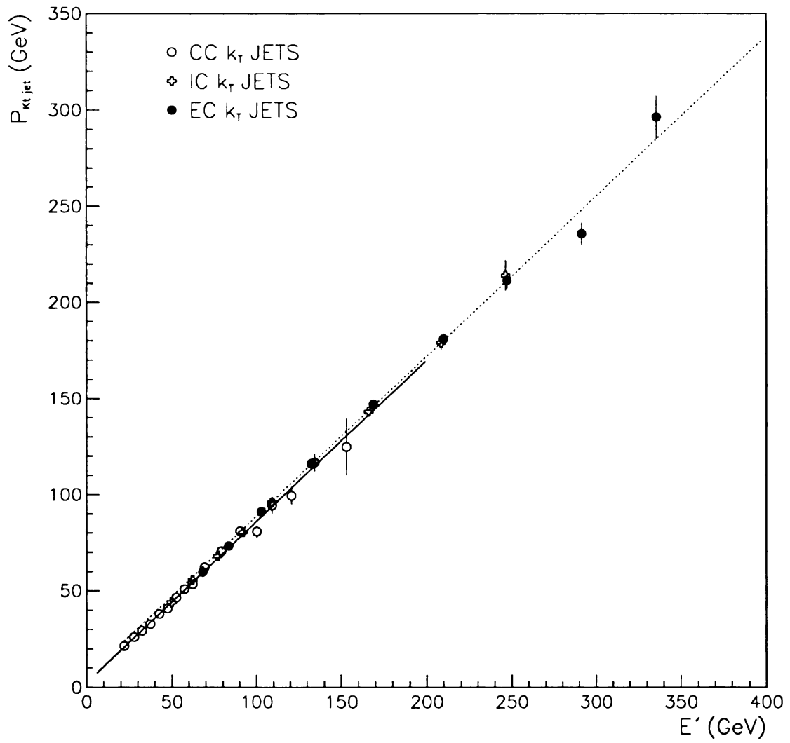
Figure 8.2: k_{\perp} jet P versus E' . Straight lines were fit to the CC and EC separately.
