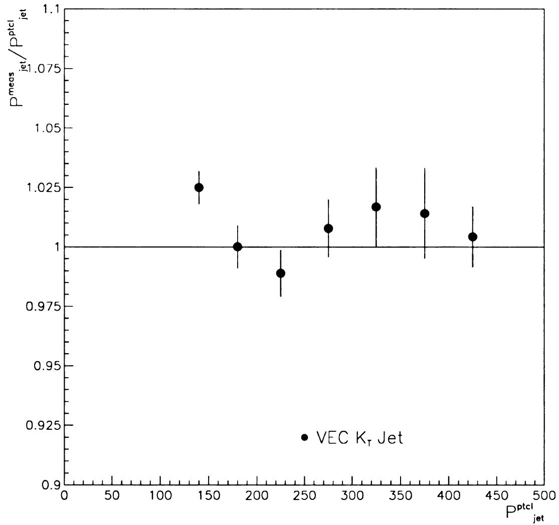
Figure 9.5: Monte Carlo Closure in EC. The ratio of the corrected calorimeter jet energy to the corresponding particle jet energy in the far forward region, VEC, defined by 2.5 < |\eta_{meas}| < 3.5 .
