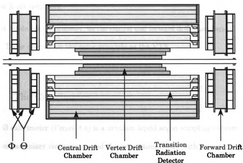
Figure 4.3: The four detectors which comprise the tracking system.
