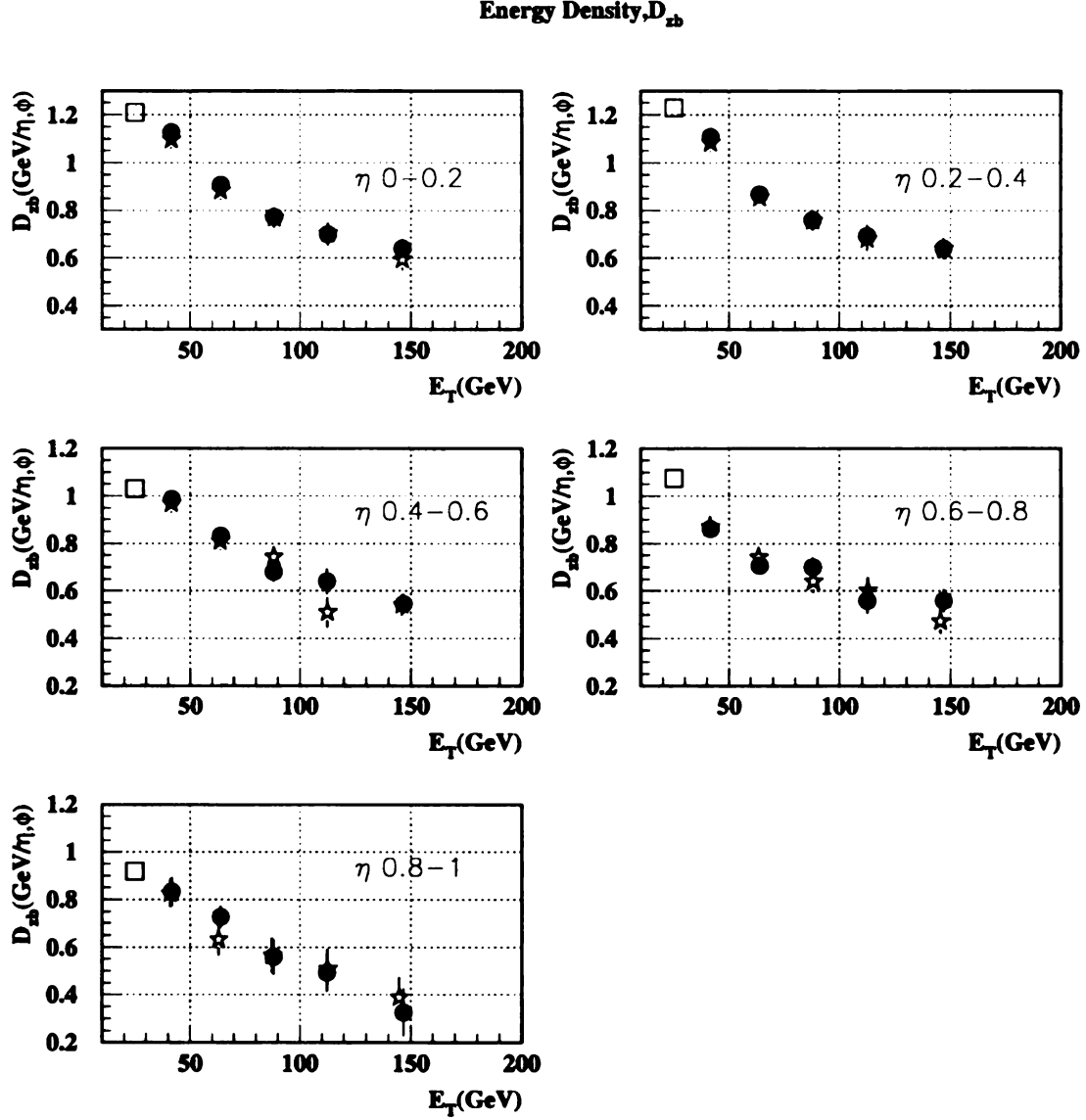
Figure B.2: Unsmeared D_{zb} offset vs. E_T in five \eta ranges for 0.7 cone jets. The cut in E_T is applied either to the raw xx jets (stars), or to z5 jets (full circles) weighed to a flat distribution in E_T . The result from CAFIX5.1 (open box) is shown for comparison on the left, but no E_T is associated with it.
