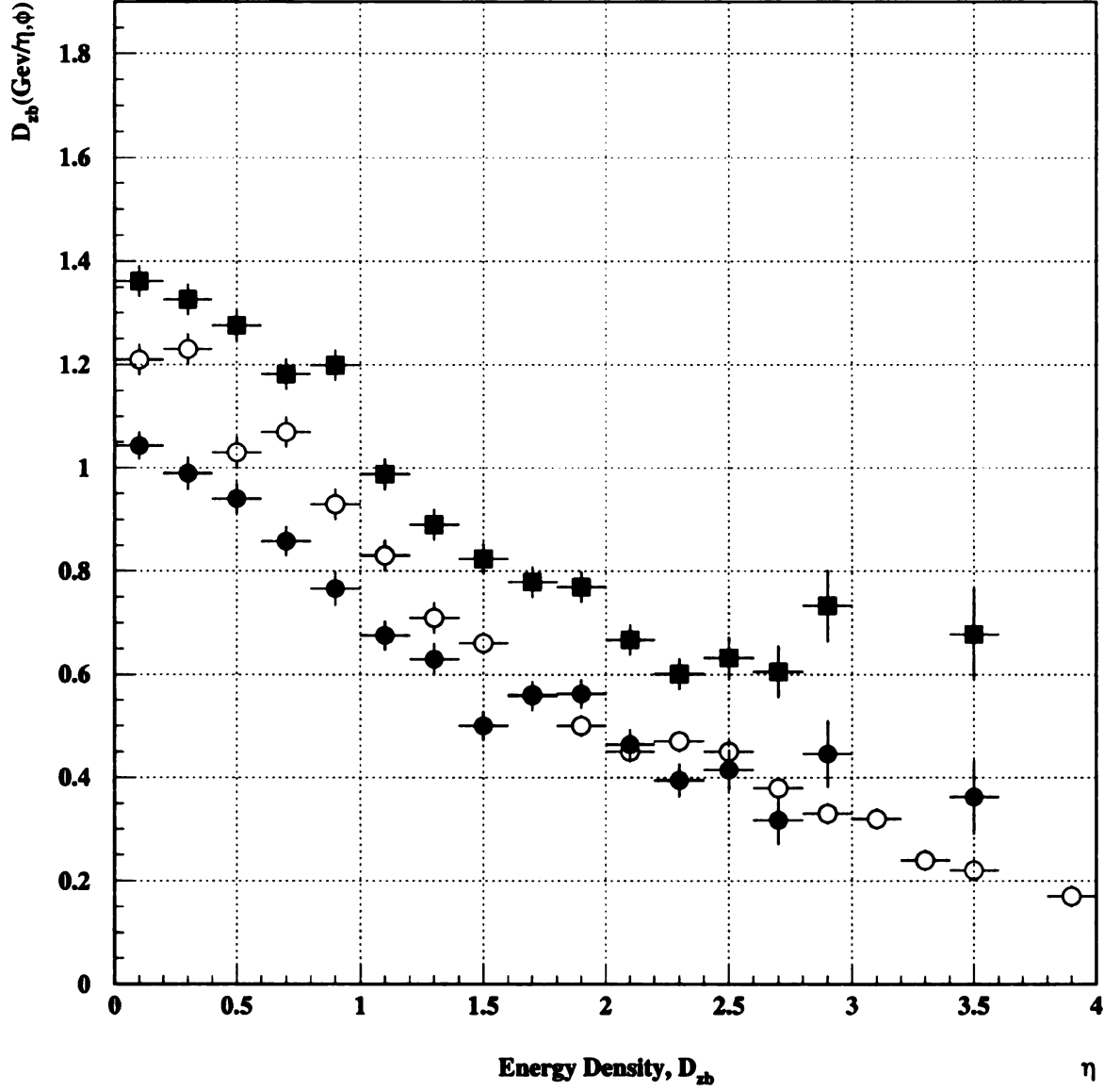
Figure B.1: The 0.7 cone jet offset density, D_{zb} , as obtained by selecting the leading jets either in the z5 (full boxes) or in the xx sample (full circles). The open circles are from CAFIX 5.1.
