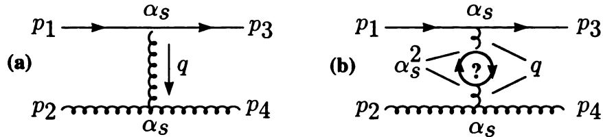
Figure 2.4: Feynman diagrams for qg \rightarrow qg via gluon exchange. (a) Lowest order ( \mathcal{O}(\alpha_s^2) ) diagram. (b) 1 Loop ( \mathcal{O}(\alpha_s^4) ) diagram
