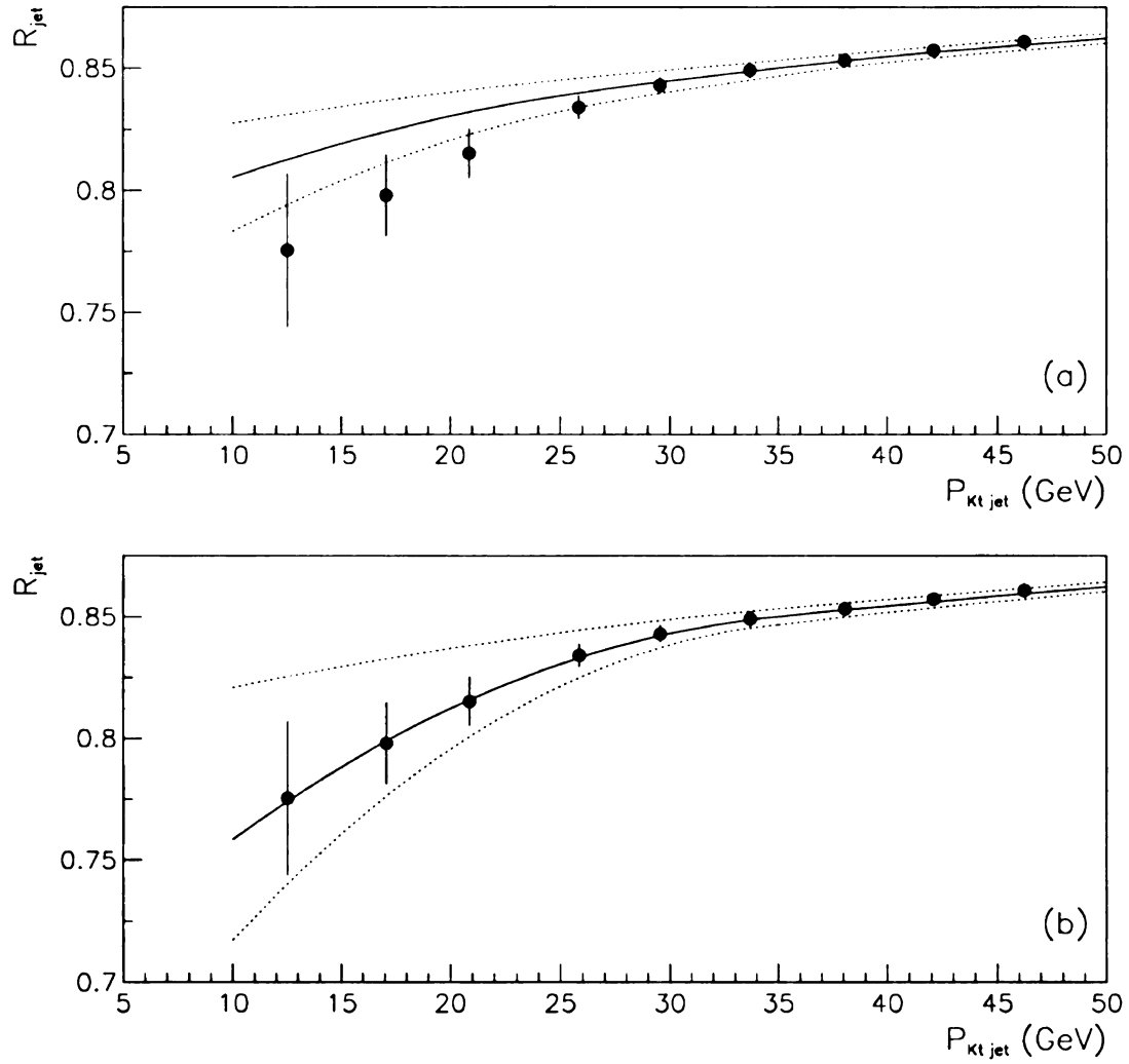
Figure 8.13: Low momentum jet response vs. P_{kt} . (a) The solid line is the extrapolated fit. Dotted lines depict errors on the fit. (b) The solid line is the jet response used to correct jets. The dashed lines show the errors (as a function of P_T ).
