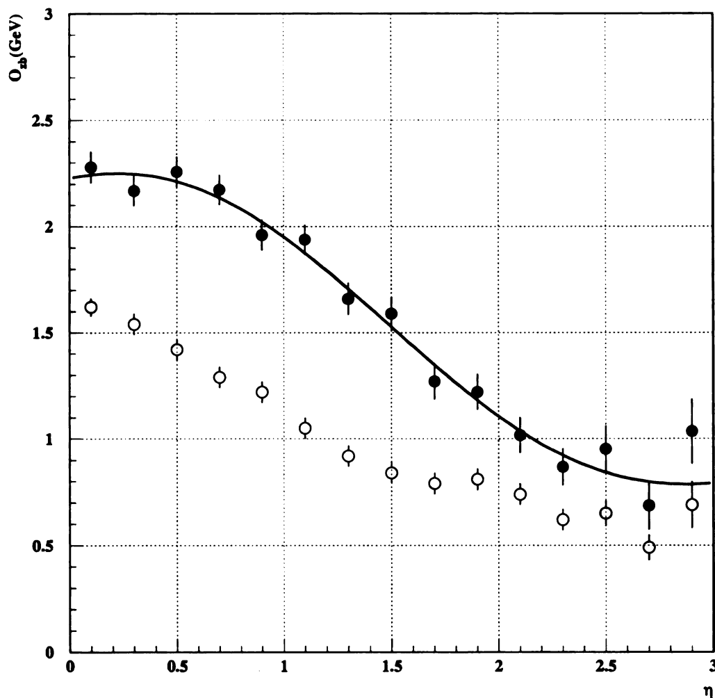
Figure 7.10: Measured O_{zb} vs. \eta for k_{\perp} jets at \mathcal{L}=5 and 30 < E_T < 50 GeV (solid symbols). The result for cones is shown for comparison (open symbols).
