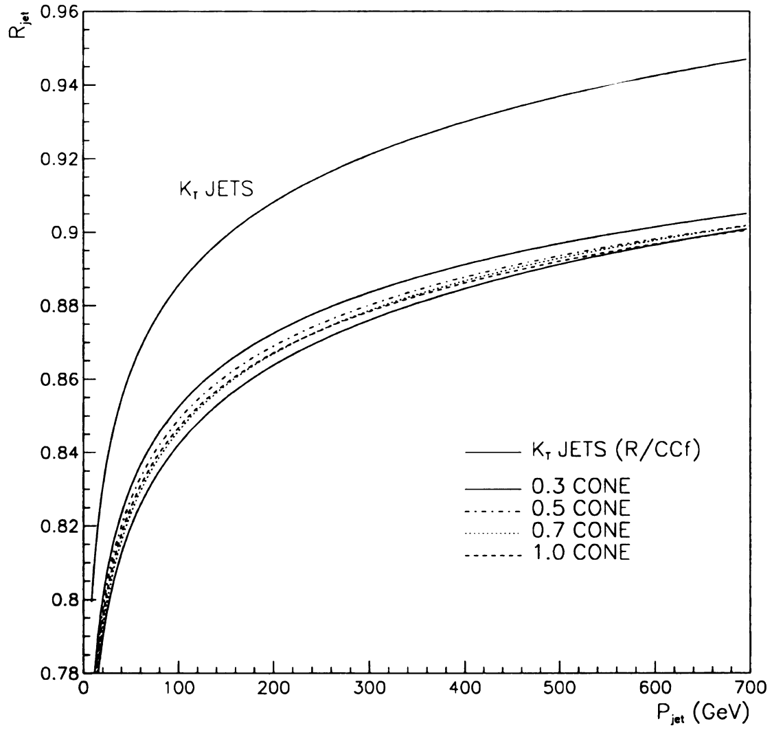
Figure 8.4: Response fit versus jet P_{kt} . R_{jet}(P_{kt}) = a + b \cdot \ln(P_{kt}) + c \cdot \ln(P)^2 .
