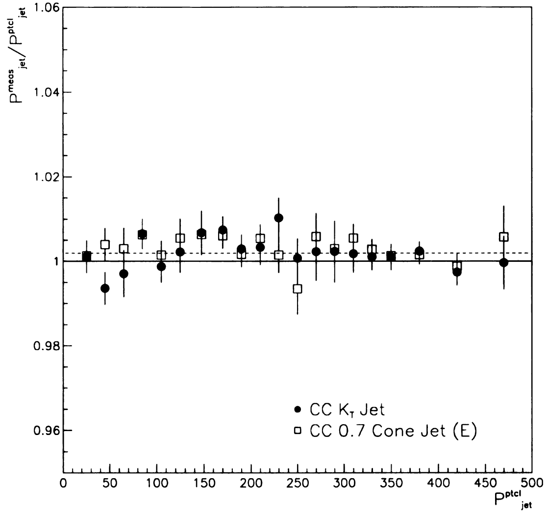
Figure 9.3: Monte Carlo Closure in CC. The ratio of the corrected calorimeter jet momentum to the corresponding particle jet momentum in the central region. Circles are for k_{\perp} jets and squares are for cone jets. Energy is compared for cone jets. The dashed line is a constant fit to the k_{\perp} jet closure.
