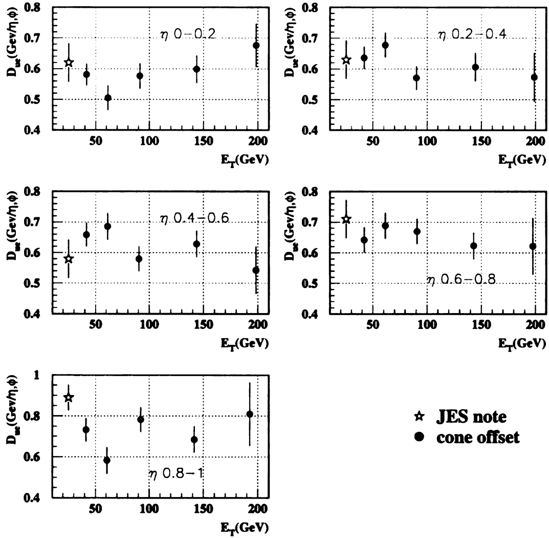
Figure B.4: Dependence of D_{ue} on E_T for cone jets. The result from CAFIX5.1 is shown for reference
