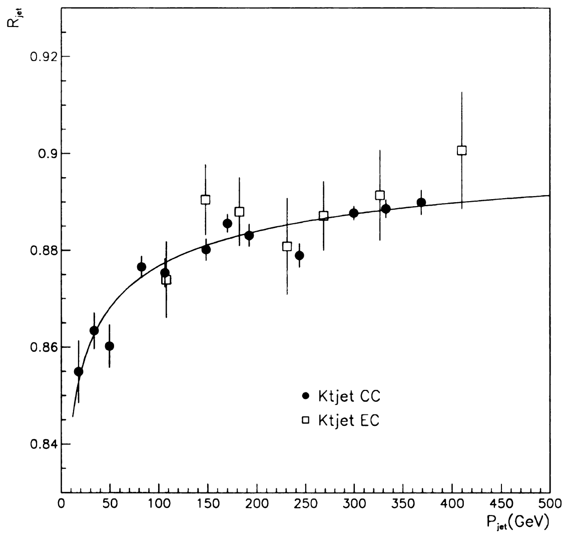
Figure 9.2: R_{jet} vs. P_{kt} in Monte Carlo data. Circles represent CC jets and squares represent EC jets.
