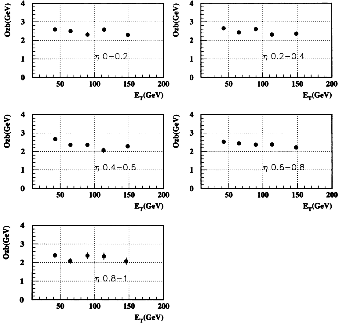
Figure 7.8: Measured O_{zb} vs. k_{\perp} jet E_T at \mathcal{L}=5\times 10^{30}\text{cm}^{-2}\text{sec}^{-1} .
