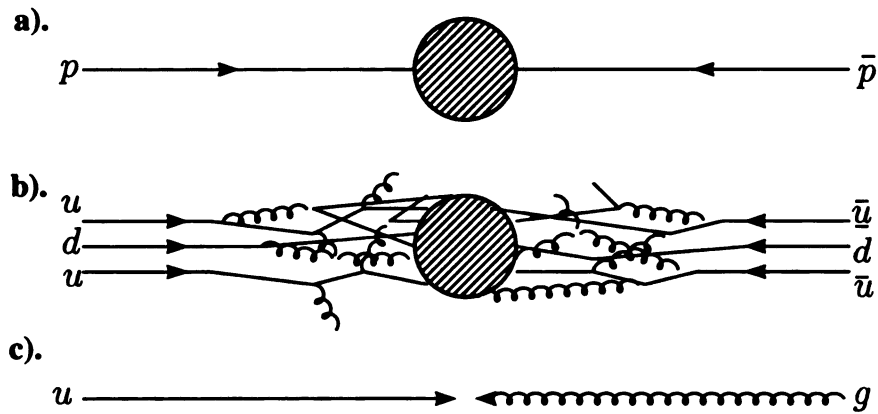
Figure 3.2: A quark from a proton interacts with a gluon from an antiproton (before). (a) At the hadron level, a proton collides with an antiproton. (b) At the parton shower level, a sea of quarks and gluons interact. (c) At the 2 \rightarrow 2 parton level, a quark interacts with a gluon.
