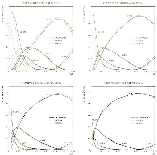
Figure 5.5: k_{\perp} Jet Rates as a function of f_{cut} in Herwig v5.8 Monte Carlo Data.
