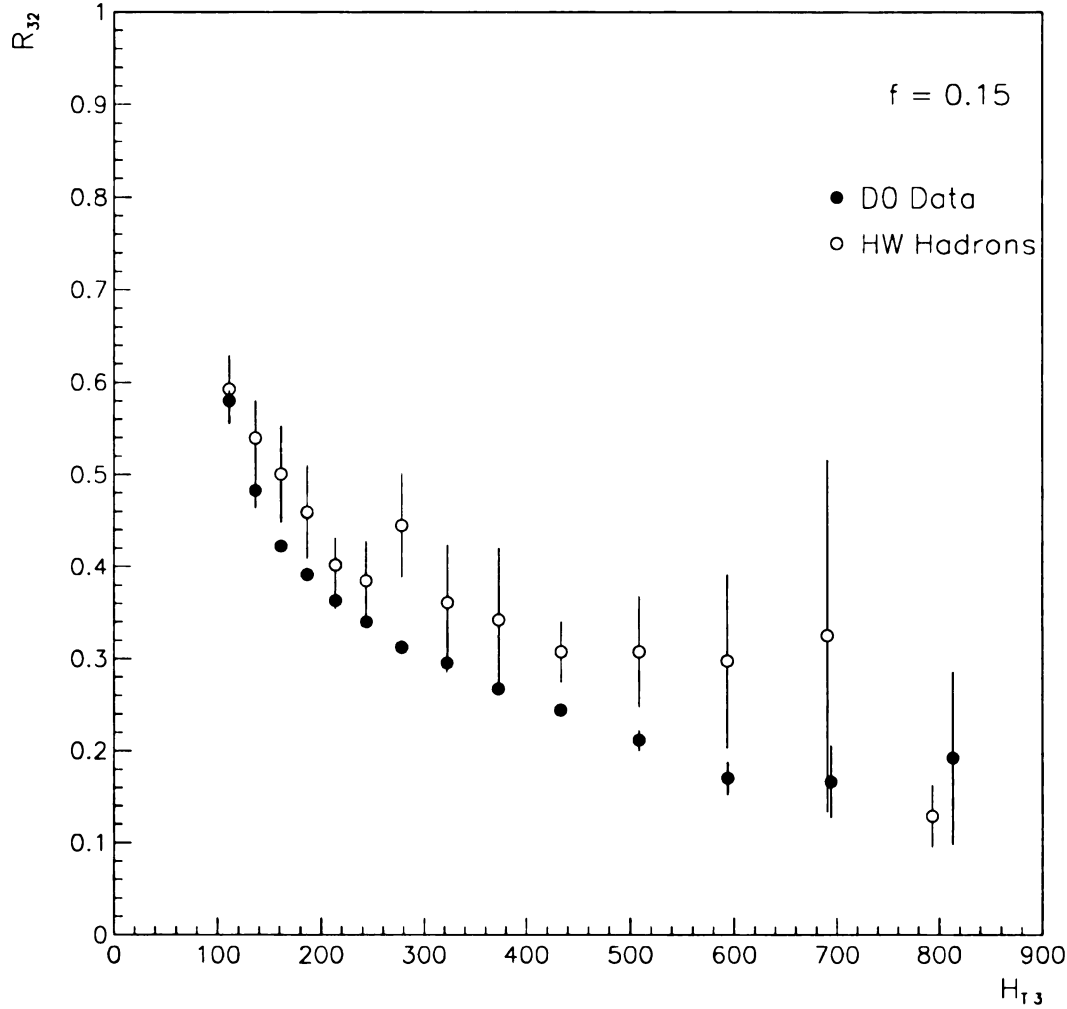
Figure 11.1: R_{32} , vs. H_{T3} . Errors are statistical only. Errors in Monte Carlo Data are the weighted statistical errors.
