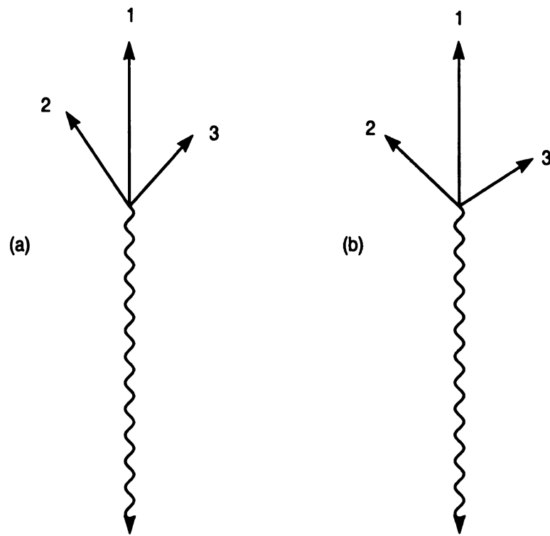
Figure C.1: Showering effects in the MPF method. (a) A photon is balanced by three particles, 1, 2, and 3, in the transverse plane. E_1 > E_2, E_3 and R_1 > R_2, R_3 . (b) The 2nd and 3rd particles are deflected away from the jet axis in the calorimeter.
