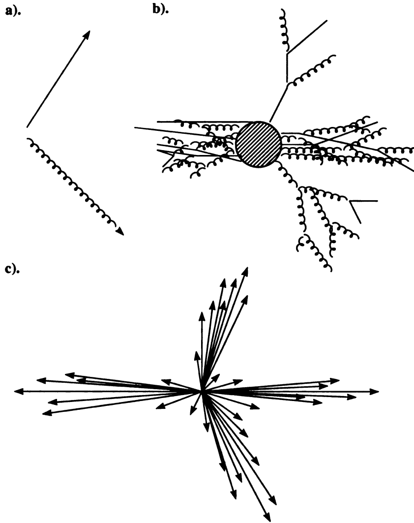
Figure 3.3: A quark from a proton interacts with a gluon from an antiproton (after). (a) At the 2 \rightarrow 2 parton level, a quark and a gluon emerge. (b) At the parton shower level, jets of quarks and gluons emerge. (c) At the hadron level, jets of hadrons emerge.
