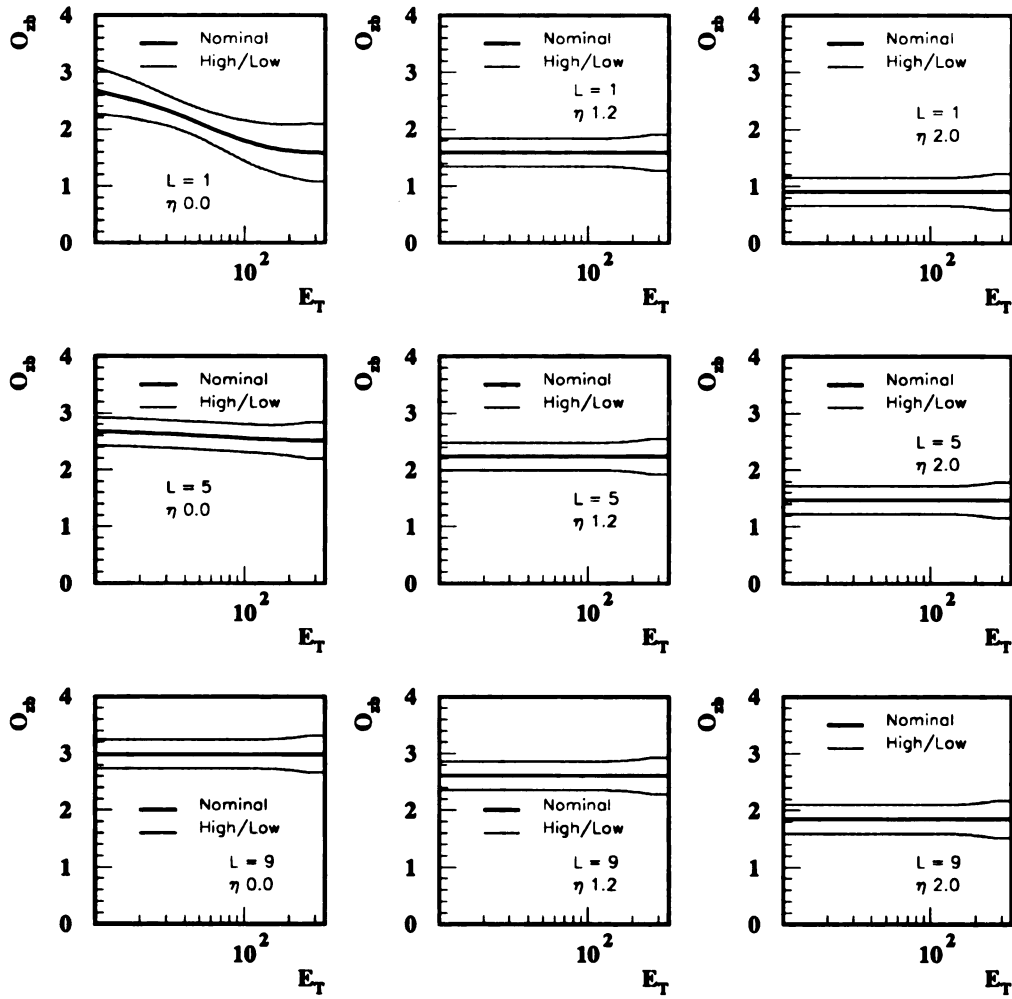
Figure 7.12: O_{zb} E_T dependence and errors, for k_{\perp} jets at \mathcal{L}=1, 5 and 9 and \eta=0.0, 1.2 , and 2.0 .
