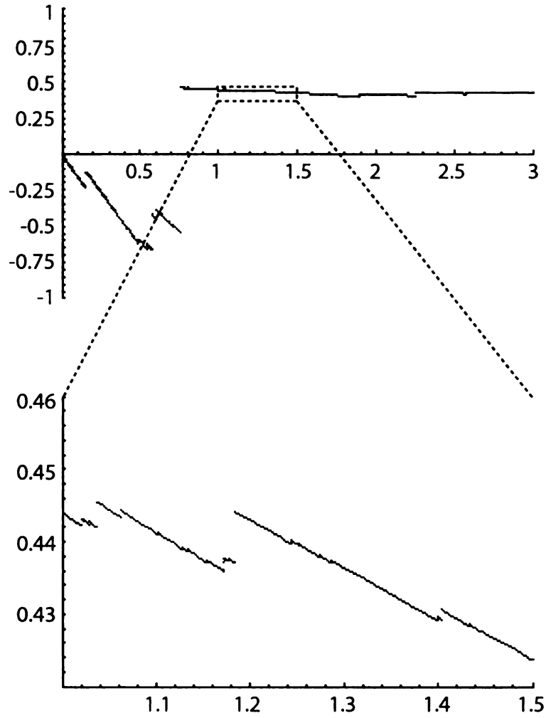
Figure 1.1: Simulated sample path of a martingale with accumulation of jumps everywhere (2 different resolutions).
