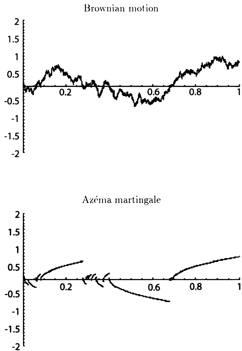
Figure 4.1: Simulated sample paths of Brownian motion and the associated Azéma martingale.
