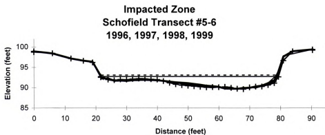
Figure 1.6. Pine River cross-sections illustrating examples where no changes in streambed elevation have been detected between 1996 and 1999.
