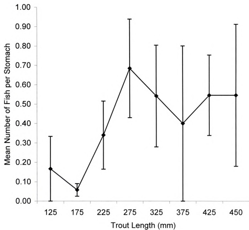
Figure 2.8. The mean number, \pm or -1 standard error, of fish per stomach by varying length classes of trout sampled on the Pine River in 1999.
