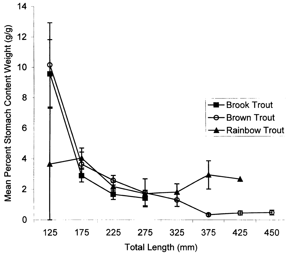
Figure 2.4. Mean percent stomach content weight (g/g), + or - 1 standard error, for all lengths (mm) of brook trout, brown trout, and rainbow trout sampled on the Pine River in 1999.
