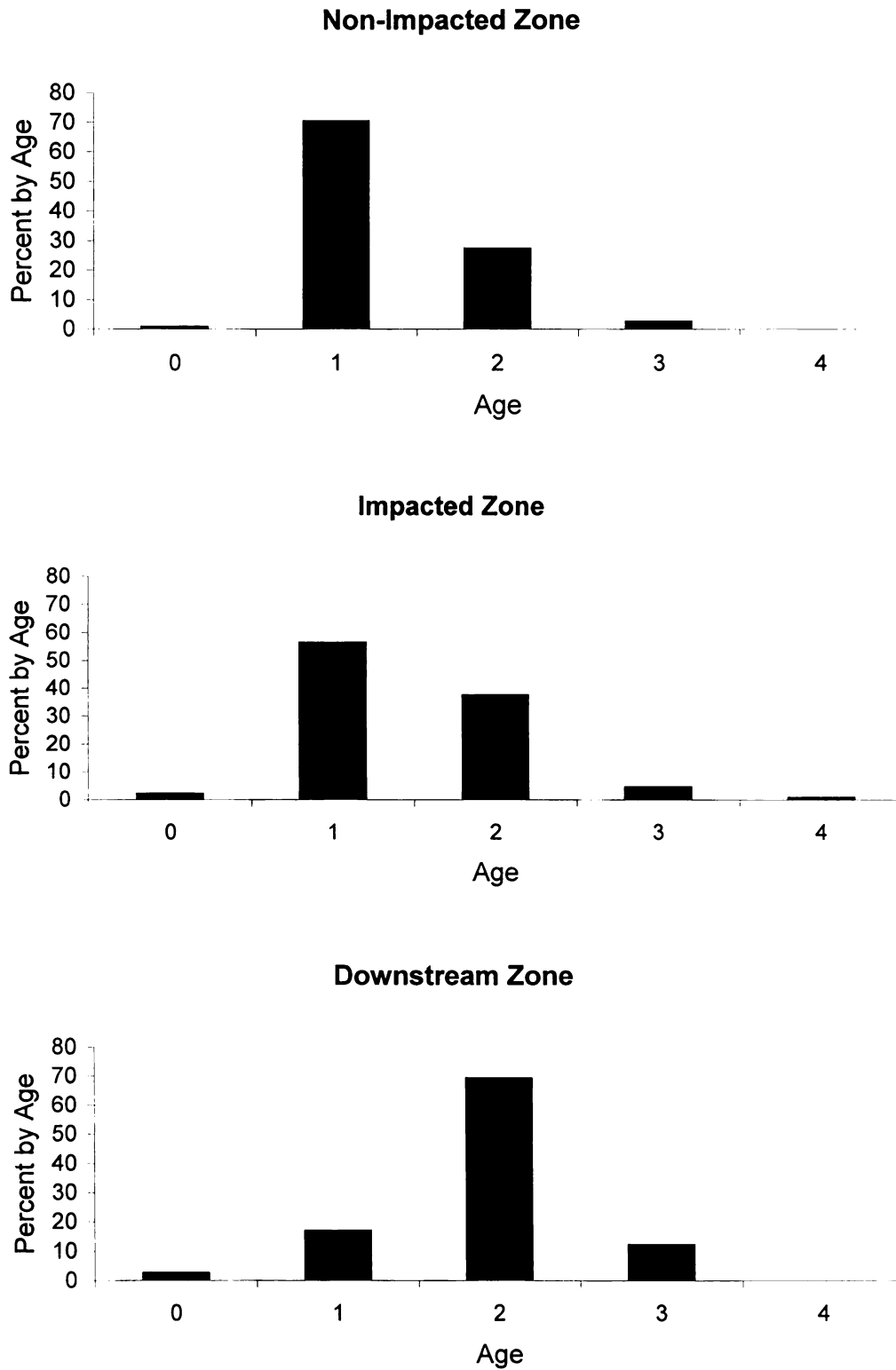
Figure 1.17. Rainbow trout age structure within each zone on the Pine River between 1996 and 1999.
