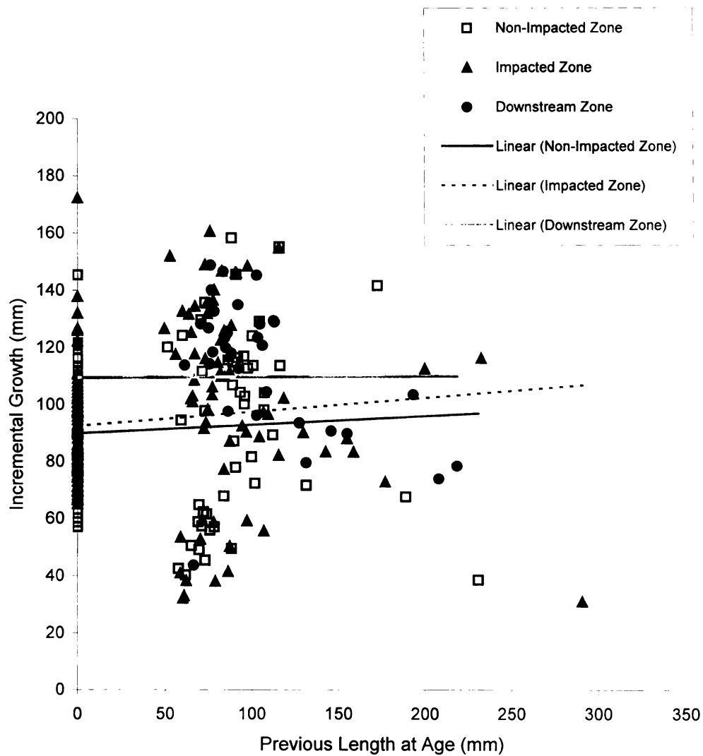
Figure 1.21. Incremental growth regressed on length at previous age by zone for rainbow trout sampled on the Pine River between 1996 and 1999.
