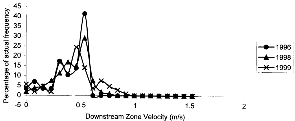
Figure 1.11. Pine River velocity percentage frequency by zone in 1996, 1998, and 1999. Data from 1997 were unavailable.
