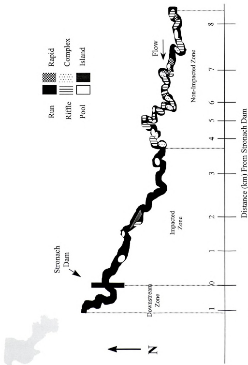
Figure 2.2. Pine River study region delineated into zones by distribution of habitat types.
