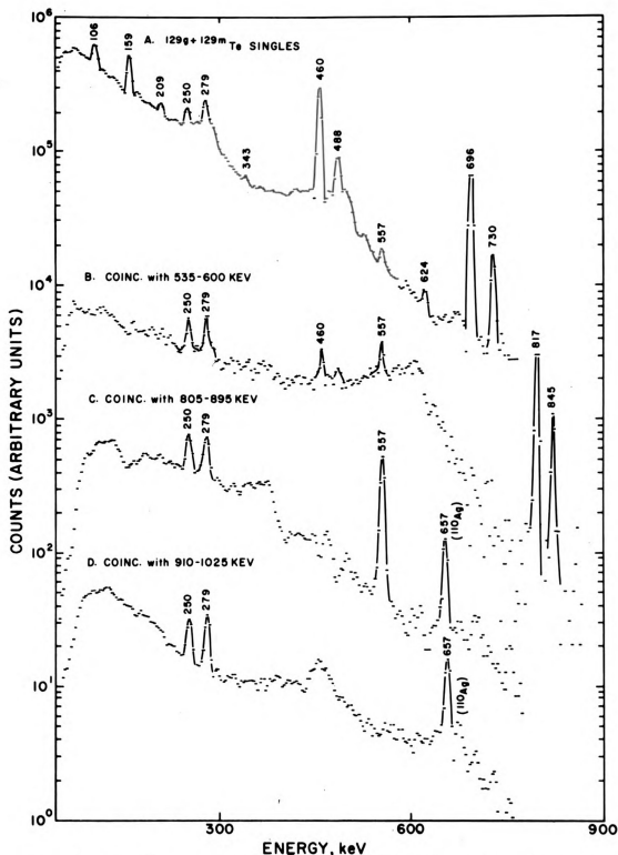
Fig. 9 Ge(Li) spectra of ^{129m+g}\text{Te} in coincidence with three regions of the spectrum seen by a 7.6 \times 7.6 cm NaI(Tl) detector. A 1 \text{ cm}^3 Ge(Li) detector was used. A singles spectrum is shown for reference. The coincident spectra have been gain shifted by the computer to allow an easier comparison.
