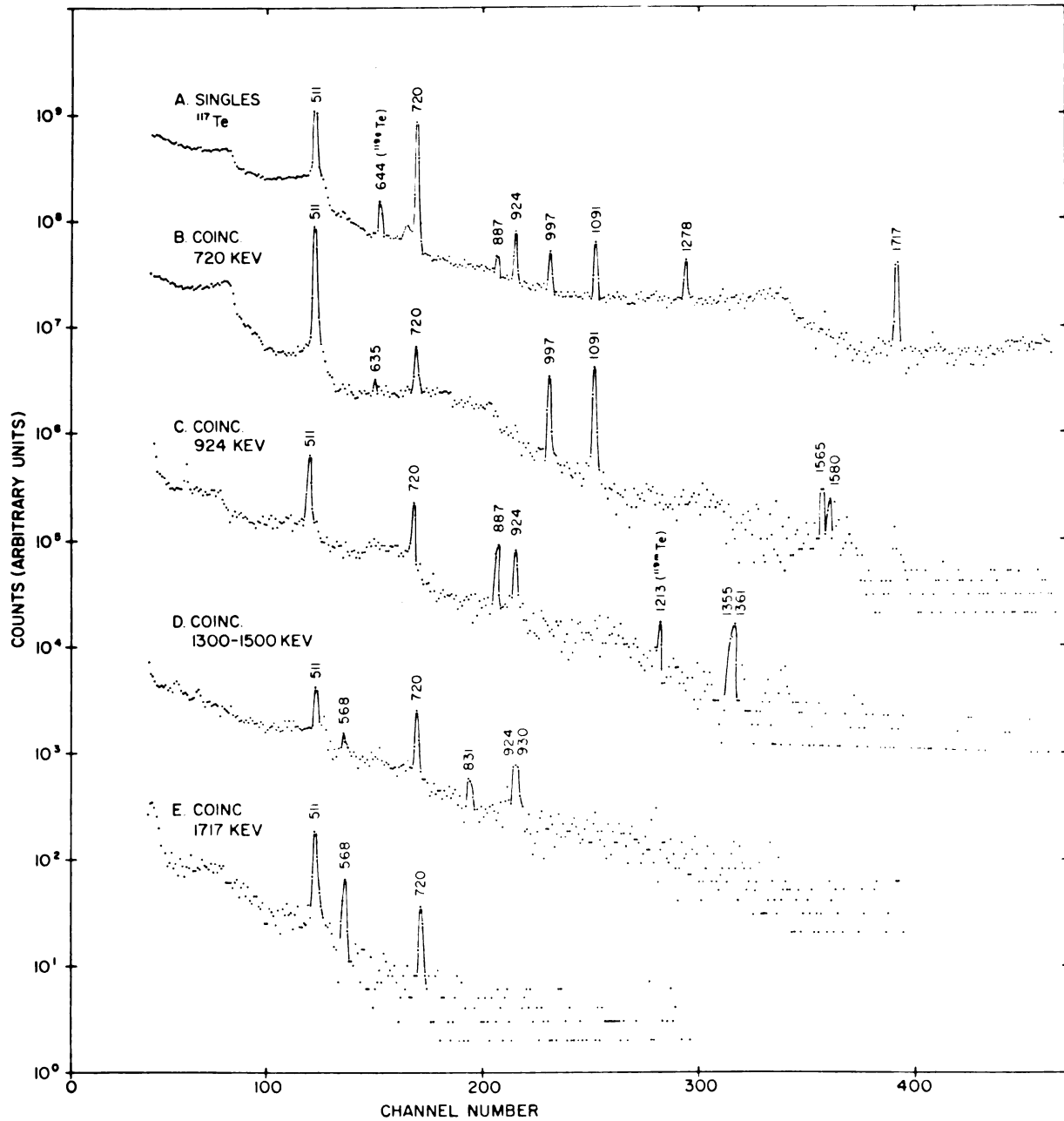
Fig. 26 Coincidence spectra of ^{117}\text{Te} obtained with a 7\text{ cm}^3 Ge(Li) counter and a 7.6 \times 7.6\text{ cm} NaI(Tl) crystal.
