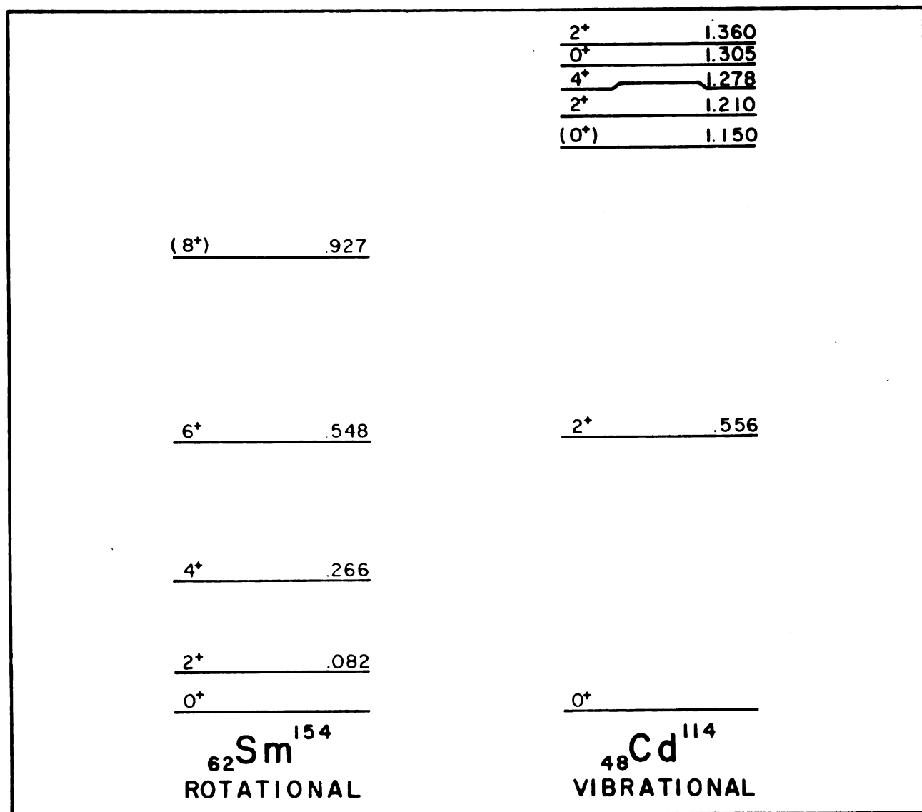
Fig. 1 Examples of rotational and vibrational energy levels which are characteristic of even-even nuclei in the deformed and the spherical regions, respectively, of the periodic table.
