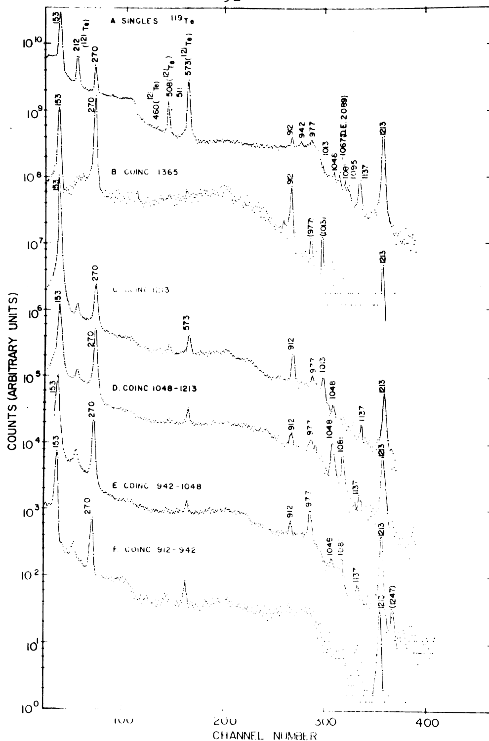
Fig. 16 Gamma ray spectra of ^{119m}\text{Te} in coincidence with various segments of the 900-1400 keV region. These spectra were taken with a 3 cm 3 Ge(Li) detector and a 7.6 cm x 7.6 cm NaI(Tl) crystal. A singles spectrum is given for reference. The spectra have been arbitrarily displaced vertically for ease of presentation. The energy scales have been adjusted to be equal with the MSU CDC3600 computer.
