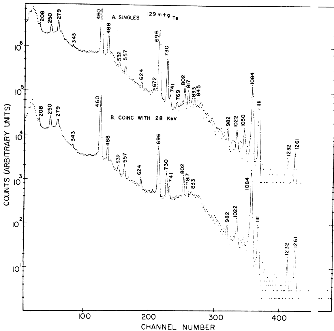
Fig. 11 A spectrum of ^{129m+g}\text{Te} in coincidence with the 28 keV gamma ray. Because only about 5% of the counts in the gate (corresponding to the 28 keV gamma ray and to x-rays) are in coincidence with other transitions, a large contribution to the spectrum arises from chance coincidences. The coincidence peaks can be identified by comparing their relative heights in the coincidence and singles spectra. A 7\text{ cm}^3\text{ Ge(Li)} detector and a 2.5 \times 3.8\text{ cm NaI(Tl)} crystal with a thin Be window were used.
