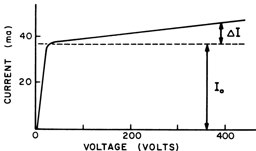
Fig. 34 A typical room temperature diode characteristics of a Ge(Li) detector.
