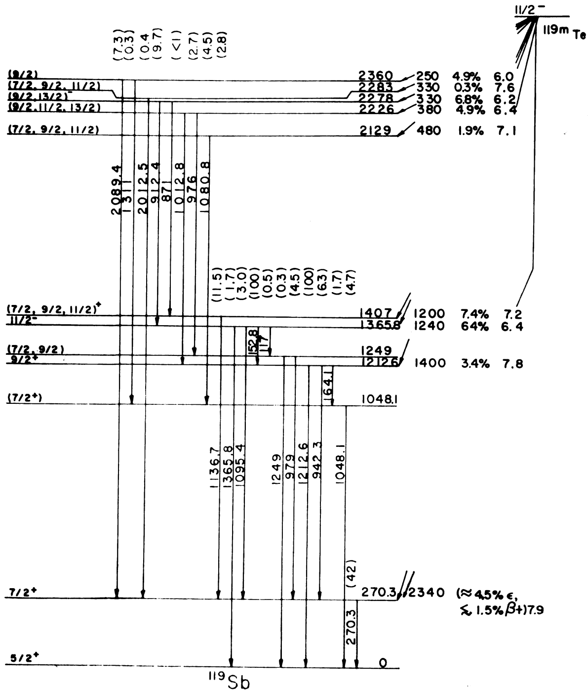
Fig. 20 Proposed decay scheme of ^{119m}\text{Te} .
