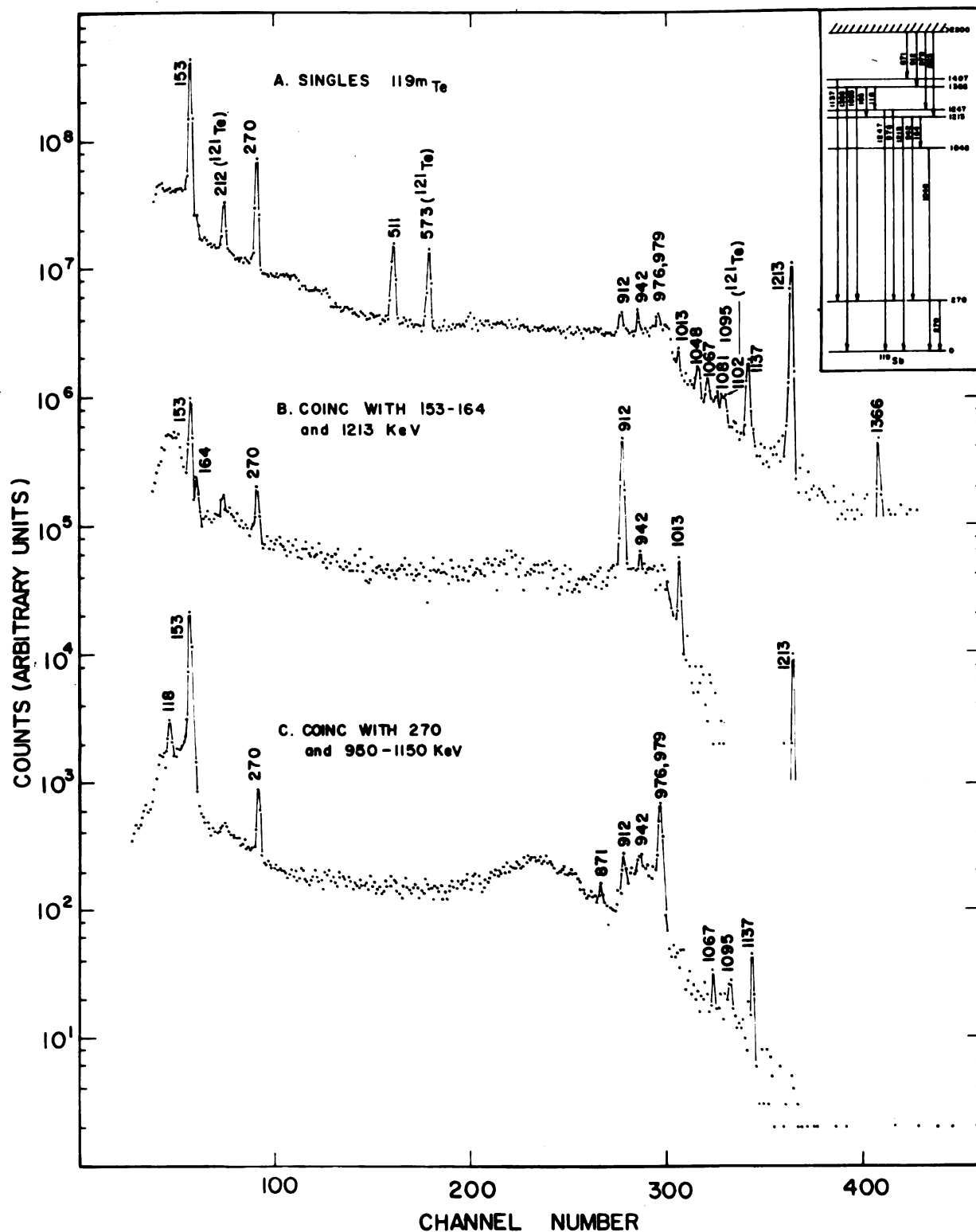
Fig. 5 Results of a triple coincidence experiment with the NaI(Tl) annulus and a 7 cm 3 Ge(Li) detector. The pertinent part of the decay scheme being investigated is shown in the upper right-hand corner of the figure. A singles spectrum is shown for easier identification of coincident photopeaks. Note the absence of the Compton distribution of the 912 keV gamma ray in spectrum B.
