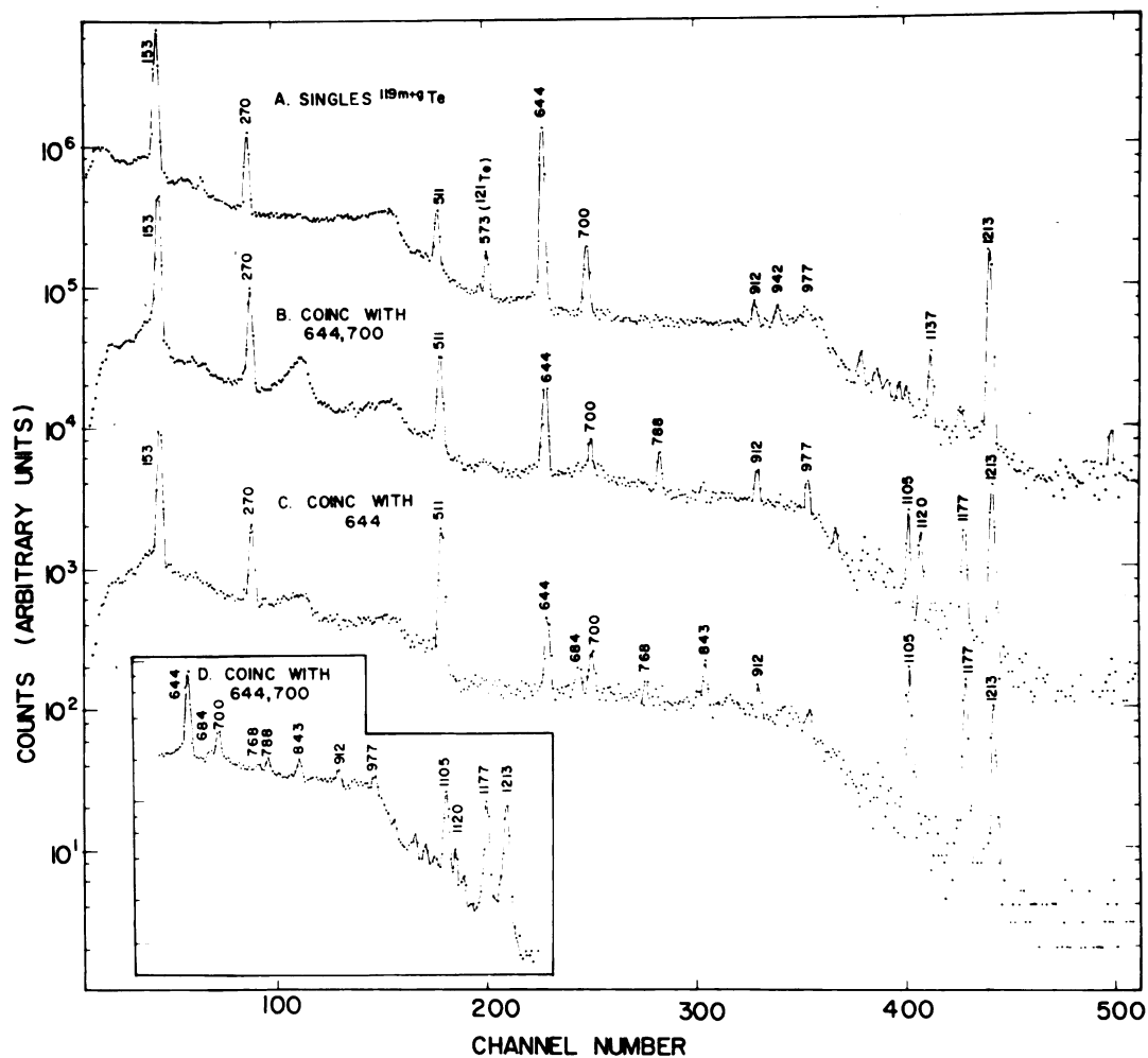
Fig. 18 Gamma ray spectra in coincidence with the 644-700 keV region in ^{119m}\text{Te} . The 7\text{cm}^3 Ge(Li) detector and one half of a 20.3\text{ cm} \times 20.3\text{ cm} NaI(Tl) split annulus crystal were used to record these spectra. Spectra B and C were recorded with the NaI(Tl) detector gated on the high and low sides of the 644-700 keV doublet, respectively. Spectrum D was obtained from an earlier source and shows a segment of the spectrum in coincidence with the 600-750 keV region.
