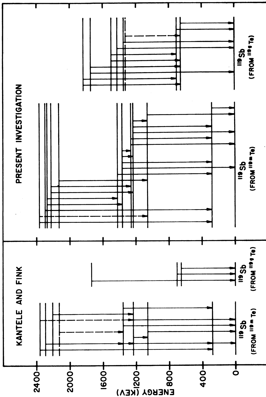
Fig. 6 Decay schemes of ^{119}\text{Te} isomers which were constructed from scintillation and conversion electron studies, compared to those constructed from high resolution gamma ray spectral studies.
