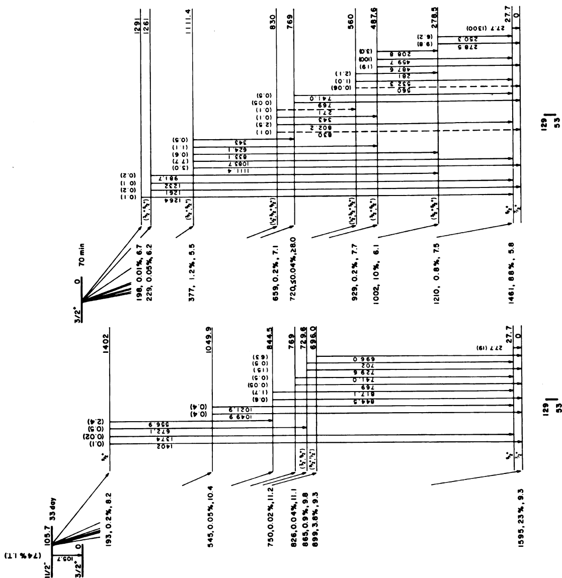
Fig. 12 Proposed decay schemes of ^{129m}\text{Te} and ^{129g}\text{Te} . The dashed lines represent transitions which were observed at MIT (refs. 50 and 51) but could not be reliably identified in our investigation. They are included because of a joint MSU-MIT publication.
