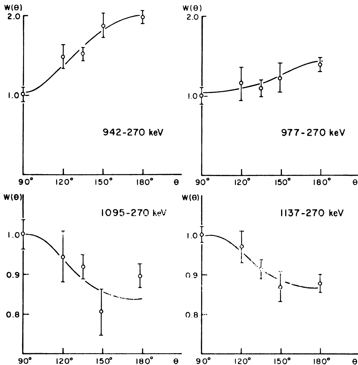
Fig. 22 Same as fig. 21 for four additional cascades. The differences in the magnitudes of the error bars for points in a given set arise from the fact that the results from several runs with different angular increments have been combined.
