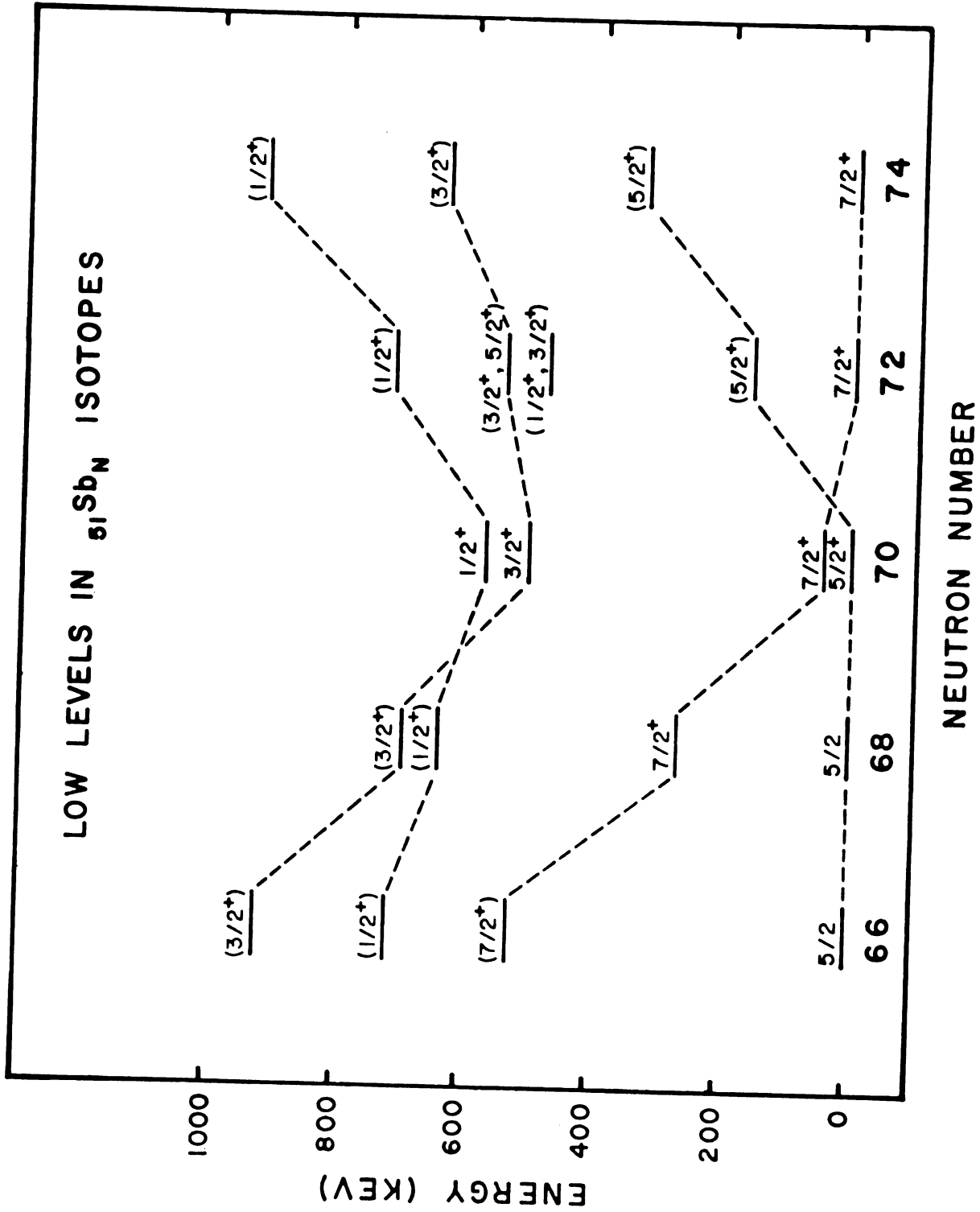
Fig. 29 Low lying levels in ^{51}\text{Sb}_N isotopes as observed in 8-\gamma decay (9,45) and (^3\text{He},d) and (d,d') experiments (54-56).
