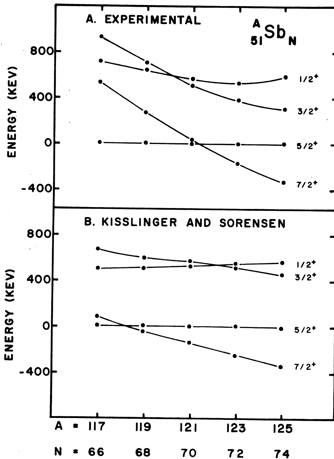
Fig. 33 A comparison of the observed low lying energy levels in the odd mass antimony isotopes with the values calculated by Kisslinger and Sorensen (6).
