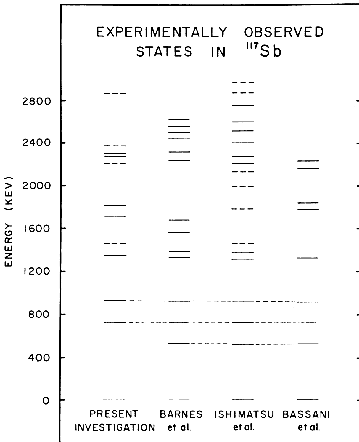
Fig. 31 Comparison of ^{117}\text{Sb} levels populated by beta decay to those observed in (^3\text{He}, d) reactions (54-56). The \beta - \gamma set is less complete than that for ^{119}\text{Sb} because of the absence of an identifiable isomeric decay ^{117m}\text{Te} .
