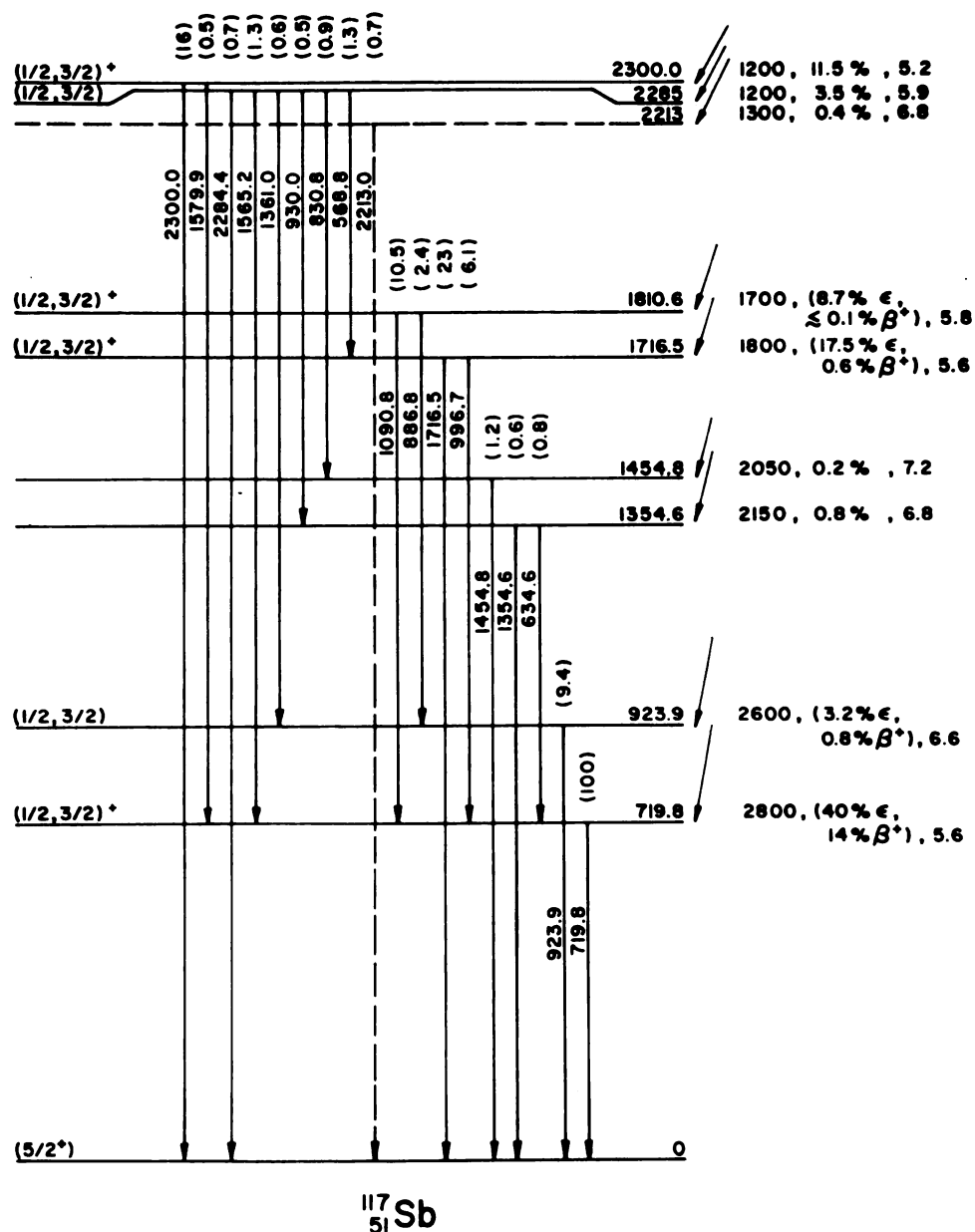
Fig. 27 The proposed decay scheme of ^{117}\text{Te} . Weak transitions of 2380 and 2885 keV, which could not be definitely assigned to the decay of ^{117}\text{Te} , have been omitted.
