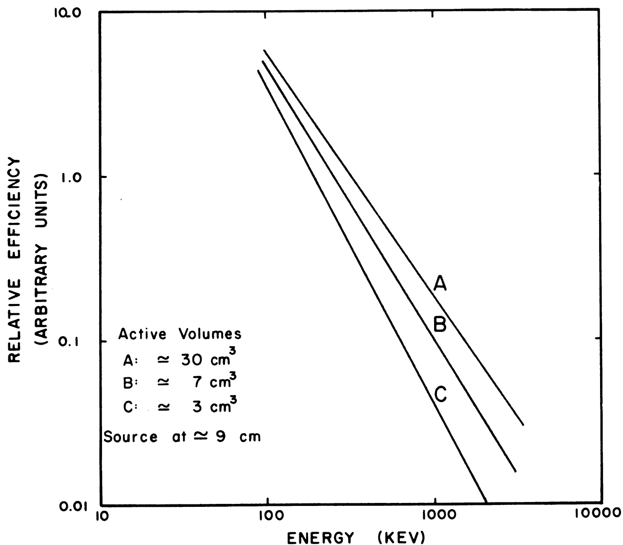
Fig. 2 Relative photopeak efficiency curves for three Ge(Li) detectors. Data for curves A and B were recorded with sources approximately 9 cm from the nearest face of the detector. Data for curve C were recorded at a different time, and the reference point for this curve has been adjusted so that the results approximately correspond to the counting conditions for curves A and B.
