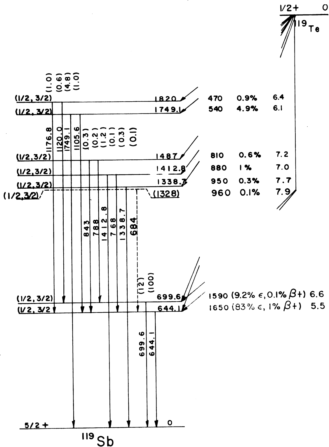
Fig. 19 Proposed decay scheme of ^{119}\text{gTe} .
