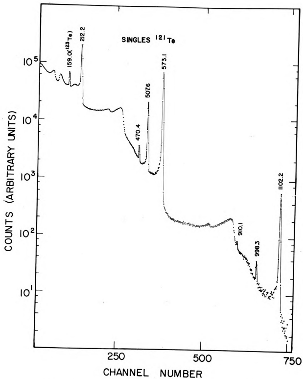
Fig. 15 Singles spectrum of ^{121}\text{Te} , recorded with a 3 cm 3 Ge(Li) detector after the ^{119m}\text{Te} had decayed away.
