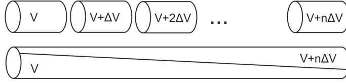
Figure 3.2: A comparison between using fine segmentation and using a diagonal crosscut to create a drag potential in a beam cooler.
