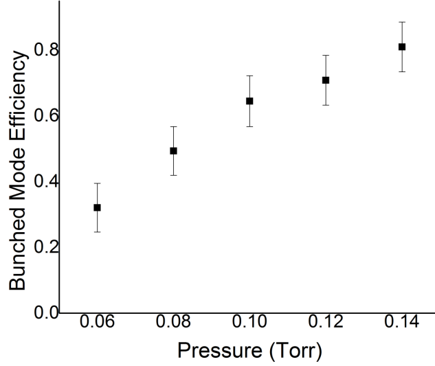
Figure 6.14: Measured bunched mode efficiency as a function of buffer gas pressure in the cooler.
