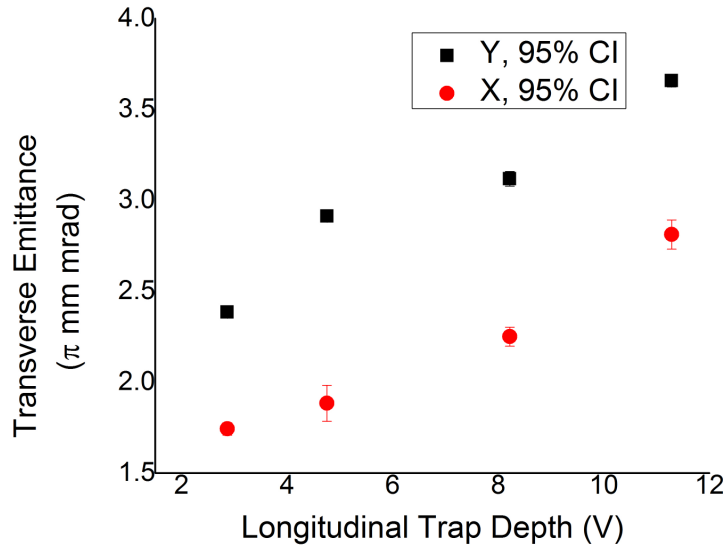
Figure 6.35: Measured transverse emittances versus static trap potential depth.
