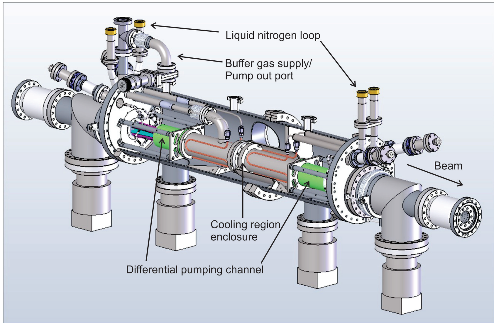
Figure 6.4: Design image of BECOLA beam cooler and buncher. The vacuum chamber interior view shows the exterior of differential pumping channel and cooling region.
