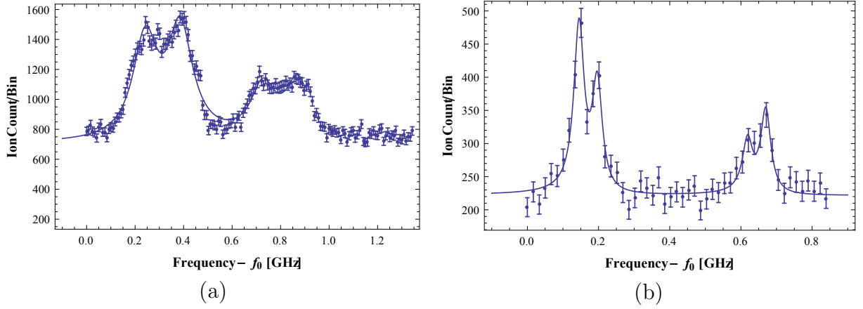
Figure 6.20: Hyperfine spectrum of D1 transition of ^{39}\text{K} for two different RF settings. Left (a): Spectrum was taken using 5.3 MHz frequency and 900 V pp amplitude. Right (b): Spectrum was taken using 1.2 MHz RF frequency and 110 V pp amplitude.
