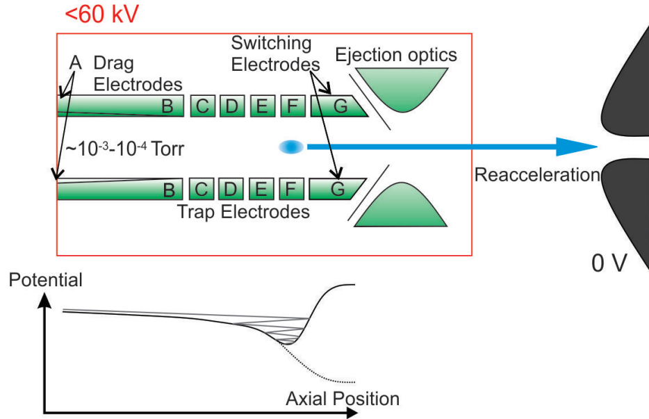
Figure 4.11: Sketch of the buncher and extraction portion of the BECOLA beam cooler and buncher.
