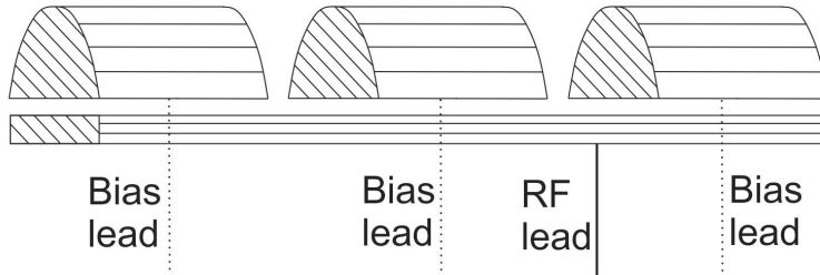
Figure 3.3: An illustration of the RF backbone coupling scheme.
