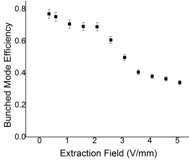
Figure 6.18: Results of efficiency measurements as a function of the extraction field at the potential minimum.
