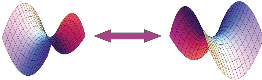
Figure 2.3: An oscillating or rotating saddle-point potential, such as that produced by a radiofrequency quadrupole.
