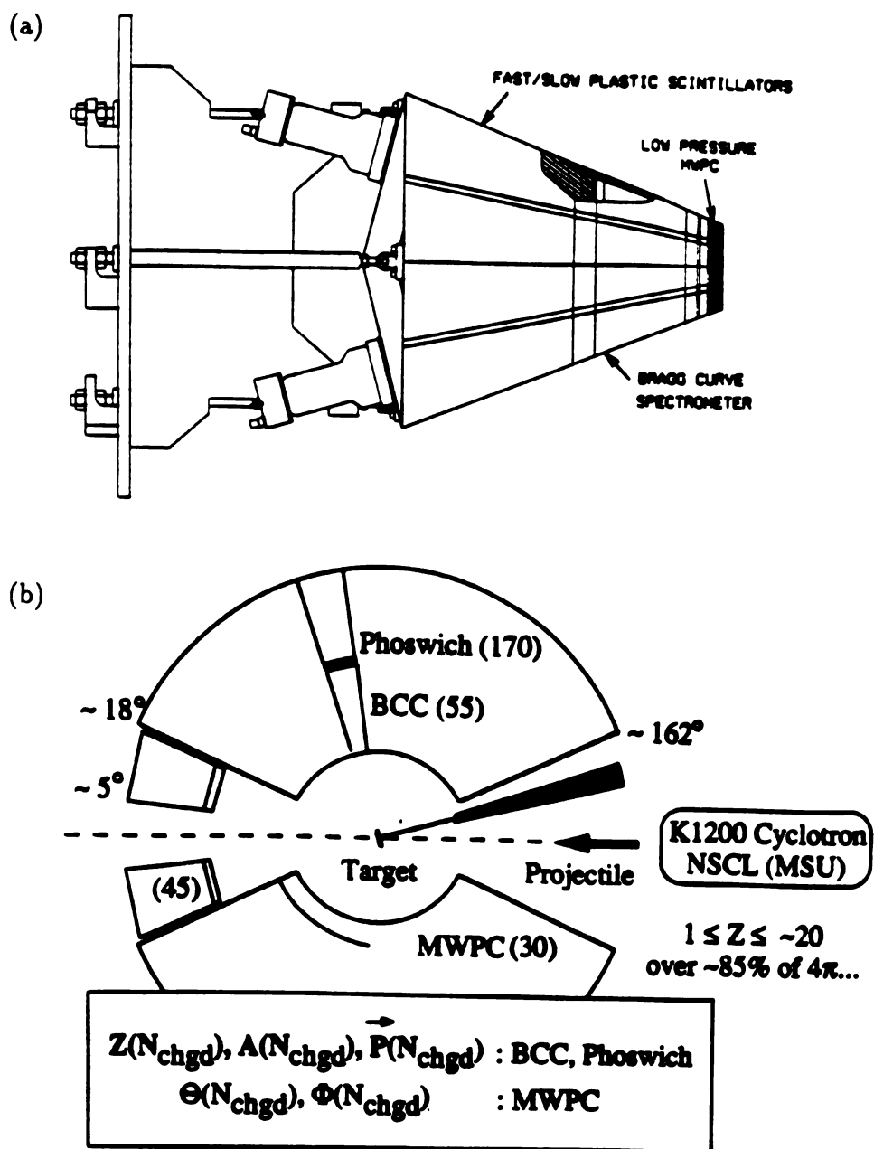
Figure 2.1: (a) A single module that consists of MSU 4\pi Array. (b) Side view of MSU 4\pi Array, that shows the arrangement of each component.
