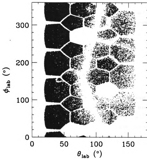
Figure 2.7: Angular distribution of MWPC events.
