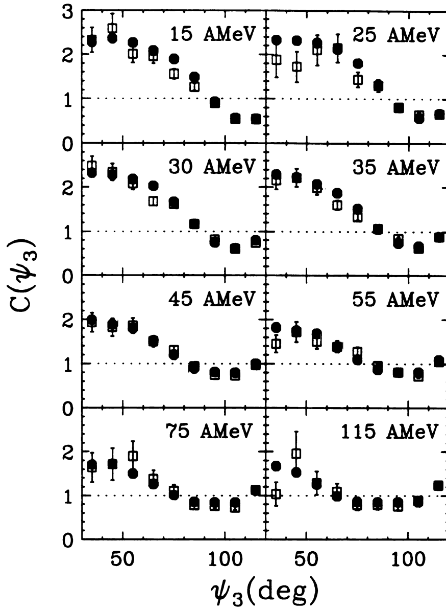
Figure 4.6: Azimuthal correlation function distributions for the reaction ^{40}\text{Ar} + ^{232}\text{Th} at E_{beam} = 15 - 115 A MeV. Only central collisions are considered. Open squares ( \square ) are experimental data. Closed circles ( \bullet ) are from simulation.
