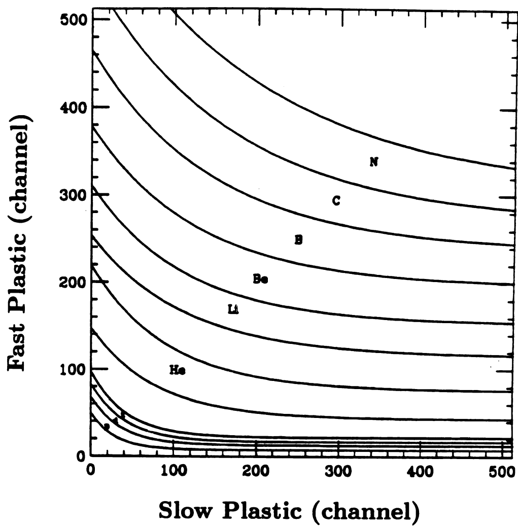
Figure 2.15: Particle identification template that assigns charge, mass and energy values to a particle projected onto a certain point.
