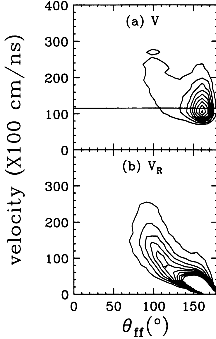
Figure 2.8: (a) Velocity spectra of the particles detected in MWPC. The line is from the Viola's empirical formular. See text for details. (b) Recoil velocity of the compound nucleus. Data are from the reaction ^{40}\text{Ar} + ^{232}\text{Th} at E_{beam} = 35 A MeV
