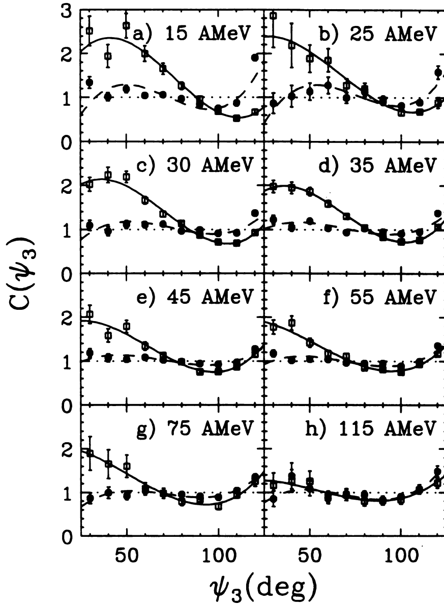
Figure 4.4: Azimuthal correlation function ( C(\psi_3) ) vs. \psi_3 . Open squares ( \square ) are for central collisions, and closed circles ( \bullet ) are for peripheral collisions. C(\psi_3) = 1 means no correlation. \psi_3 < 30^\circ region is not plotted because of the lack of statistics. Such a case does not have different meaning from C(\psi_3) \simeq 50^\circ so that dropping that region does not affect the argument. Data are from the reaction ^{40}\text{Ar} + ^{232}\text{Th} at E_{\text{beam}} = 15 - 115 A MeV.
