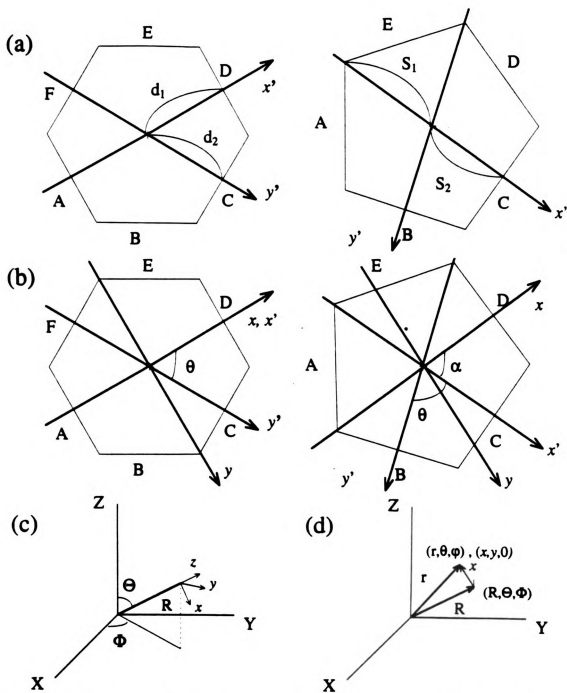
Figure 2.6: (a) Cathode coordinate system (x', y') . (b) Module coordinate system (x, y, z) . (c) The orientation of the unit vectors of module coordinate system in lab. frame. (d) r = R + x
