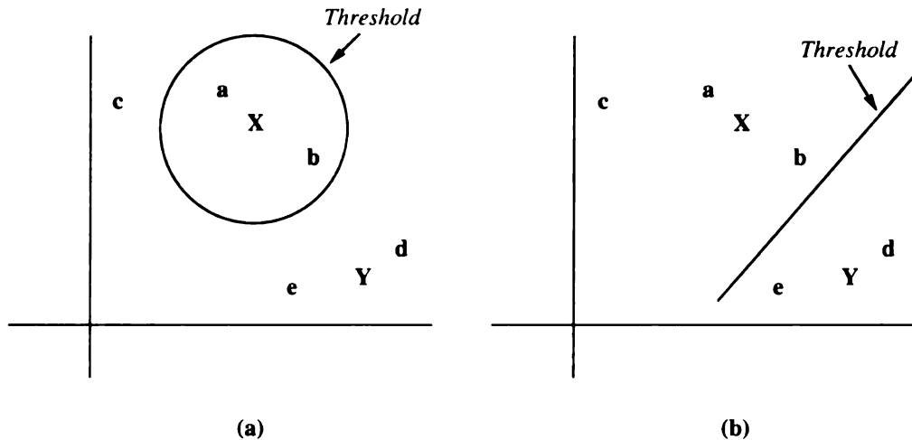
Figure 4.4: Similarity and difference features. (a) Similarity features: while training patterns a and b are grouped based on their similarity, to template X , examples c and d , although very different from each other, will be grouped together; (b) Difference features: training patterns on each side of the decision threshold (difference between template X and template Y ) are more similar to each other than to patterns on the other side.
