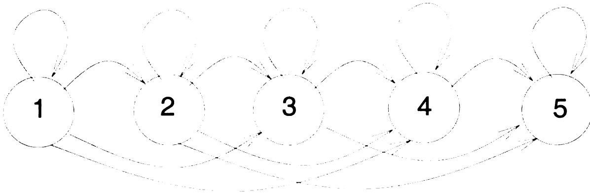
Figure 5.1: The topology of our hidden Markov models. Note that only single or double state skipping transitions are allowed.
