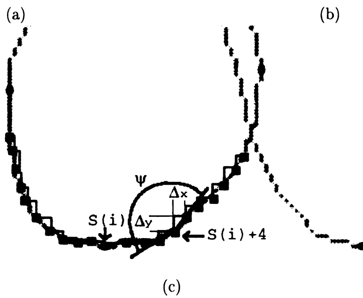
Figure 6.1: An example of Critical Point features: (a) calculation of structural features \theta , and \phi , (b) y (in relation to baseline shown), and critical point (\Delta x, \Delta y) , (c) calculation of local neighborhood features \Delta x , \Delta y , and \psi .
