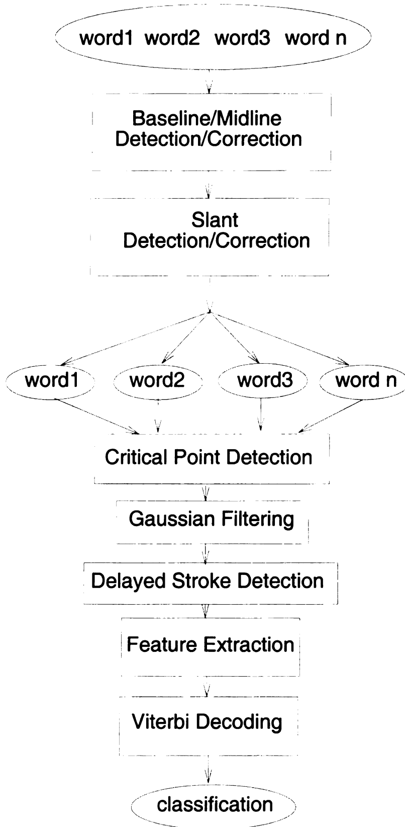
Figure 7.1: Word recognition system.
