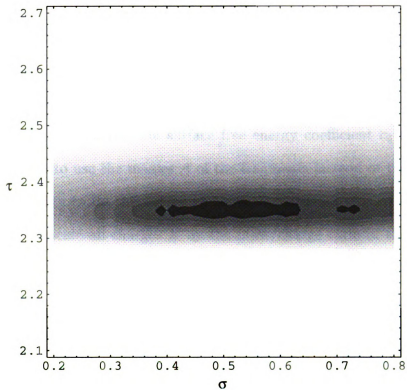
Figure 3.11: Density plot of \chi^2 as a function of \sigma and \tau for the experimental data (with filter- and sequential decay correction). The 4 innermost contours represent [\chi^2/(\text{degrees of freedom})] -values of 3.3, 3.7, 4.1 and 4.6, respectively. A critical temperature of 8.3 MeV has been used in this plot.
