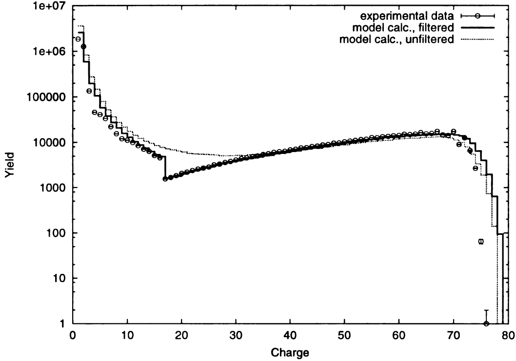
Figure 3.2: Inclusive charge yield spectrum. The experimental data (corrected by the “17-20” events, see Section 3.2.3) is given by the circles, the filtered and unfiltered model data by the solid and dotted lines, respectively. The charge is given, as in all following diagrams, in multiples of the charge of a proton.
