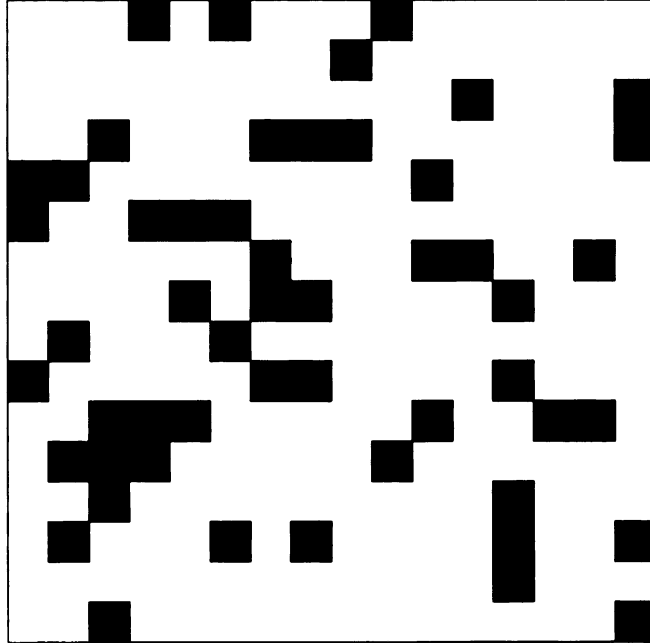
Figure 2.1: Example of a typical site percolation configuration with a density of p=0.2
