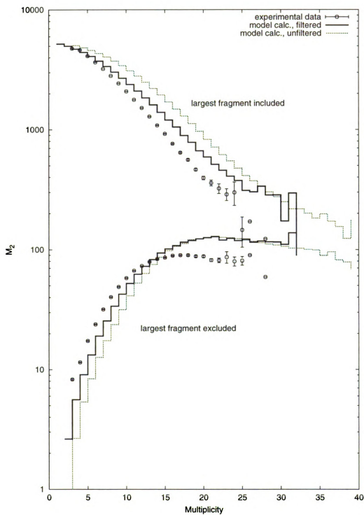
Figure 3.6: Second moment ( M_2 ) versus multiplicity. In the upper branch, the second moments have been calculated including the largest fragment, in the lower branch the largest fragment has been excluded.
