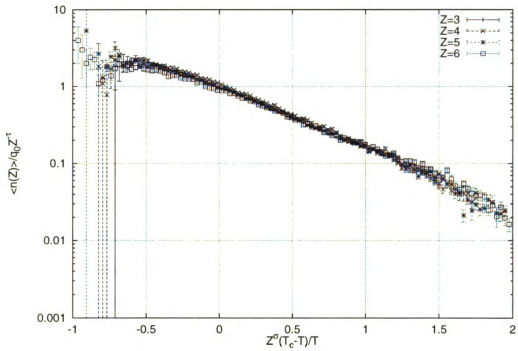
Figure 3.12: Plot of the scaled fragment distribution as a function of the scaled control parameter (multiplied by T_c ) for the experimental data (with filter- and sequential decay corrections) Values of \sigma = 0.5 , \tau = 2.35 and T_c = 8.3 MeV have been used.
