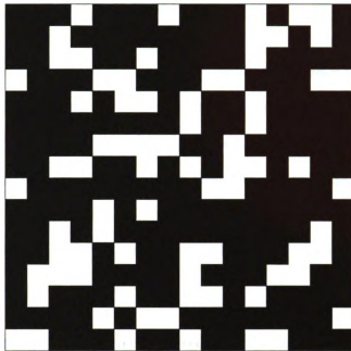
Figure 2.2: Example of a typical site percolation configuration with a density of p=0.7
