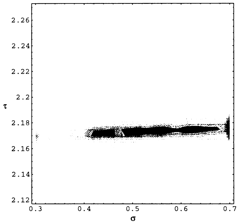
Figure 3.8: Density plot of \chi^2 as a function of \sigma and \tau for the unfiltered percolation events. The 4 innermost contours represent [\chi^2/(\text{degrees of freedom})] -values of 3.2, 3.5, 3.8 and 4.1, respectively. A critical breaking probability of 0.65 has been used in this plot.
