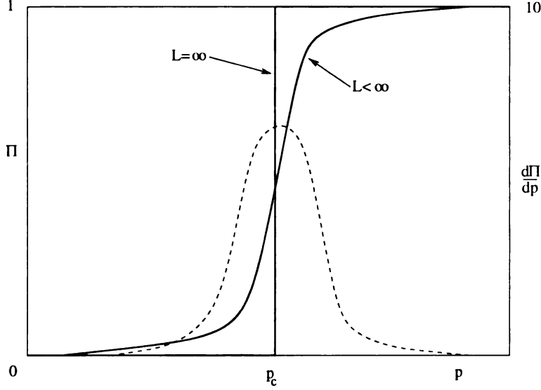
Figure 2.3: Variation of the probability \Pi (solid lines) that a cluster is spanning the whole system for medium and large system sizes. The dashed line gives \frac{d\Pi}{dp} , proportional to the probability that at concentration p a spanning cluster starts to appear. The width of the transition region or peak should vary according to L^{1/\nu} .
