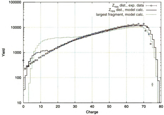
Figure 3.4: Distribution of Z_{\text{residue}} (experimental data and filtered model data, circles and solid lines) and of the largest fragment (unfiltered model data, dotted lines).
