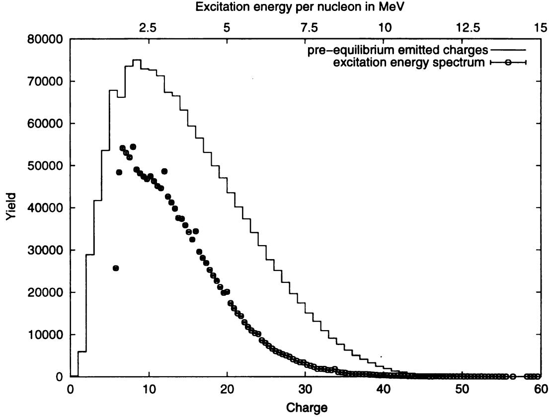
Figure 3.1: Spectrum of excitation energy per nucleon and frequency of pre-equilibrium emitted charges in experimental data.
