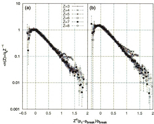
Figure 3.7: Plot of the scaled fragment distribution as a function of the scaled control parameter (multiplied by p_c ) for fragments of charge Z . (a) shows the filtered data, (b) the unfiltered model data. In this plot, a critical percolation probability p_c = 0.7 , \sigma = 0.45 and \tau=2.18 have been chosen.
