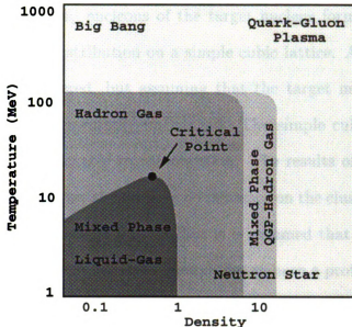
Figure 2.4: The Nuclear Phase Diagram (schematic)
