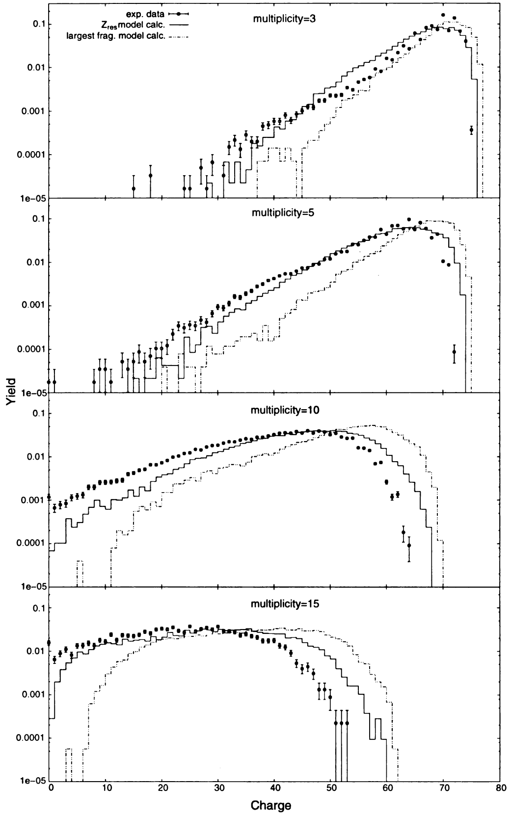
Figure 3.5: Z_{res} distribution for different multiplicities. In the case of the unfiltered data the distribution of the largest fragment is plotted instead.
