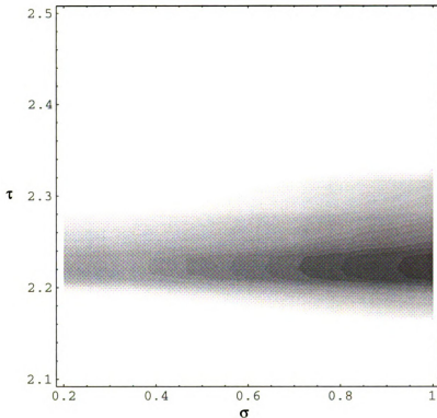
Figure 3.9: Density plot of \chi^2 as a function of \sigma and \tau for the experimental data (uncorrected). The innermost contour corresponds to a [\chi^2/(\text{degrees of freedom})] -value of \approx 12 .
