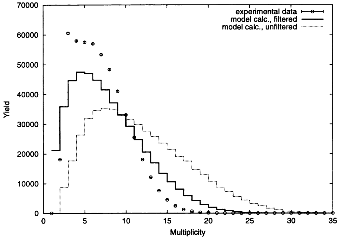
Figure 3.3: Multiplicity distribution. The experimental data are given by the circles, the filtered and unfiltered model data by the solid and dotted line, respectively.
