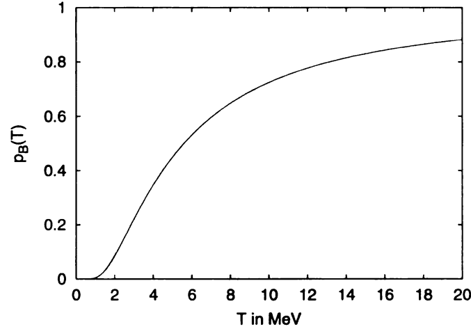
Figure 2.6: Relation between p_B and the temperature of the fragmenting nucleus as given by Equation 2.38 ( B=6.6\text{MeV} )
