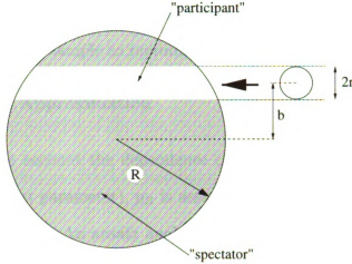
Figure 2.5: The fireball geometry: the lattice sites in the cylindrical channel with radius r at impact parameter b are left unoccupied.
