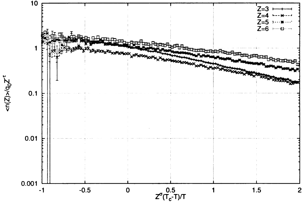
Figure 3.10: Plot of the scaled fragment distribution as a function of the scaled control parameter (multiplied by T_c ) for the experimental data (uncorrected). Values of \sigma = 0.99 , \tau = 2.13 and T_c = 9.5 MeV have been used.
