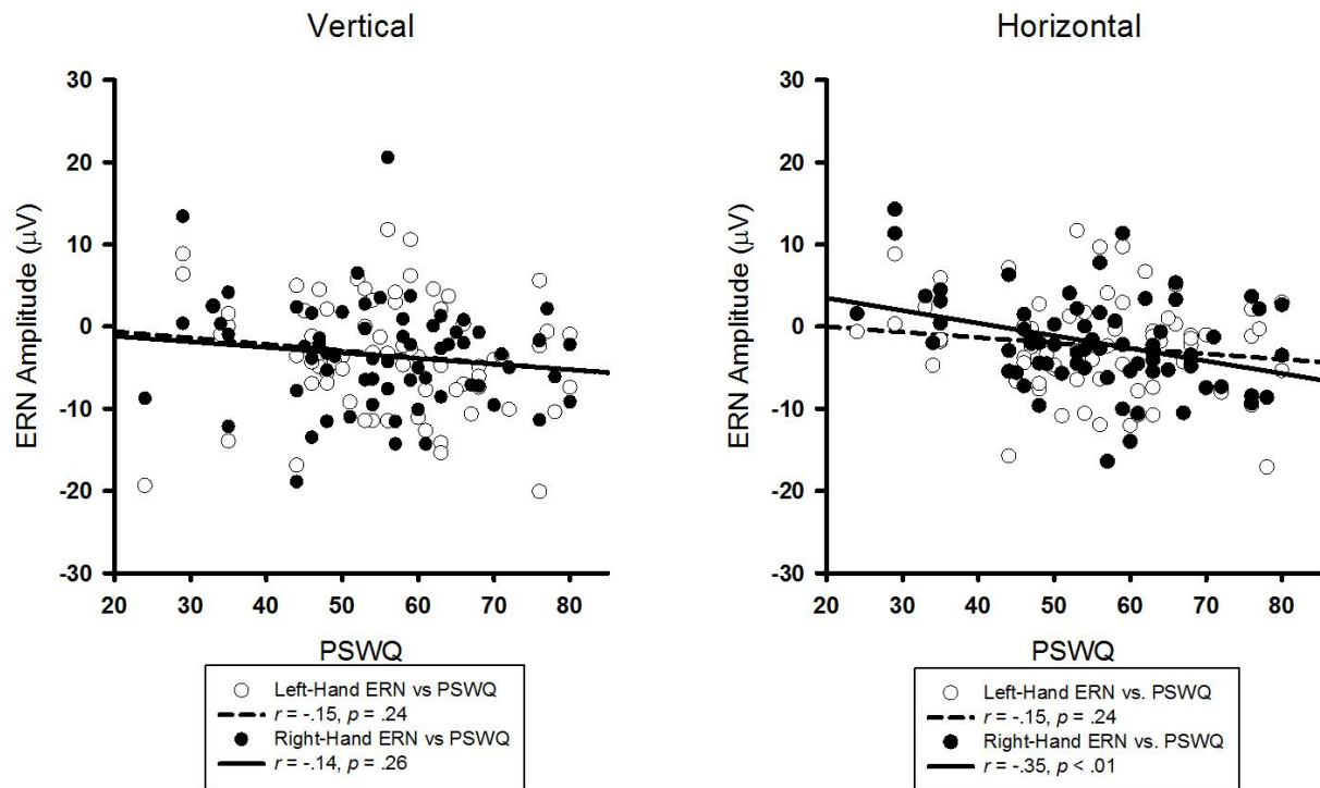
Figure 4. Experiment 2 Scatter Plot.
