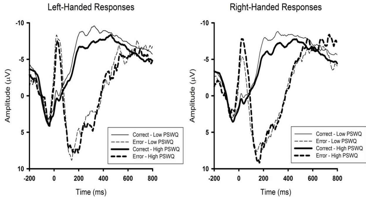
Figure 1. Experiment 1 Response Locked ERPs.
