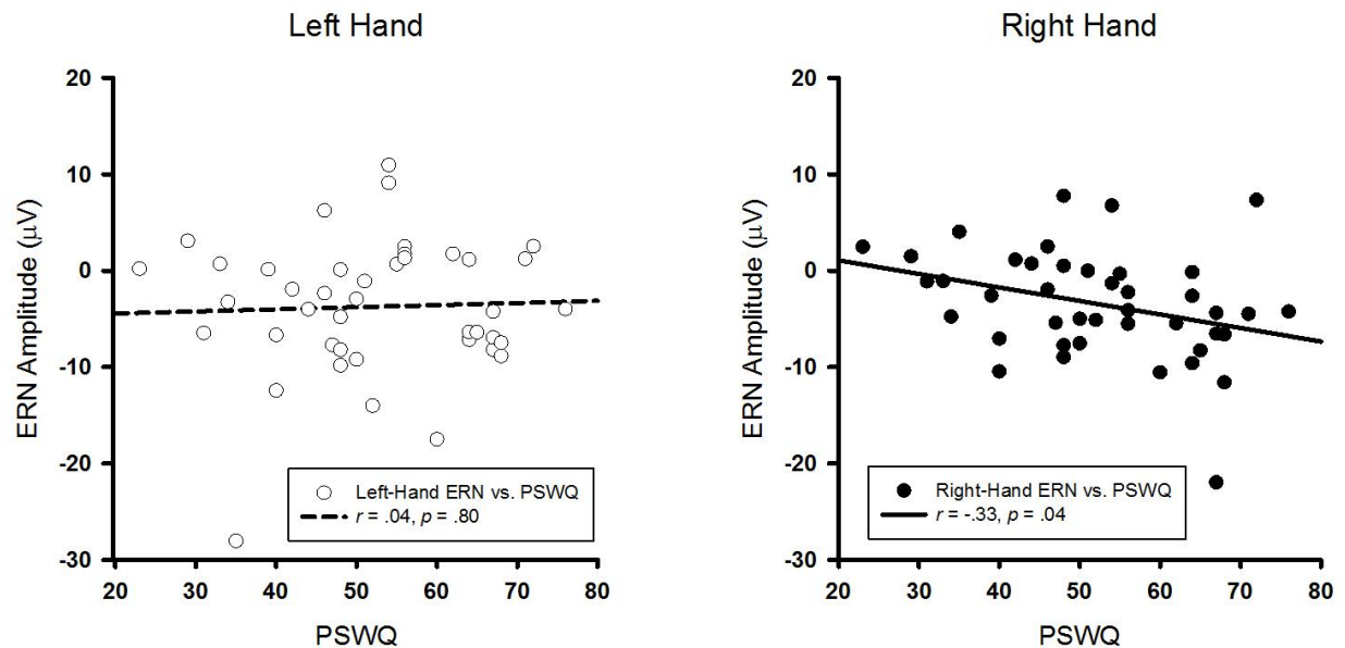
Figure 2. Experiment 1 Scatter Plot.
