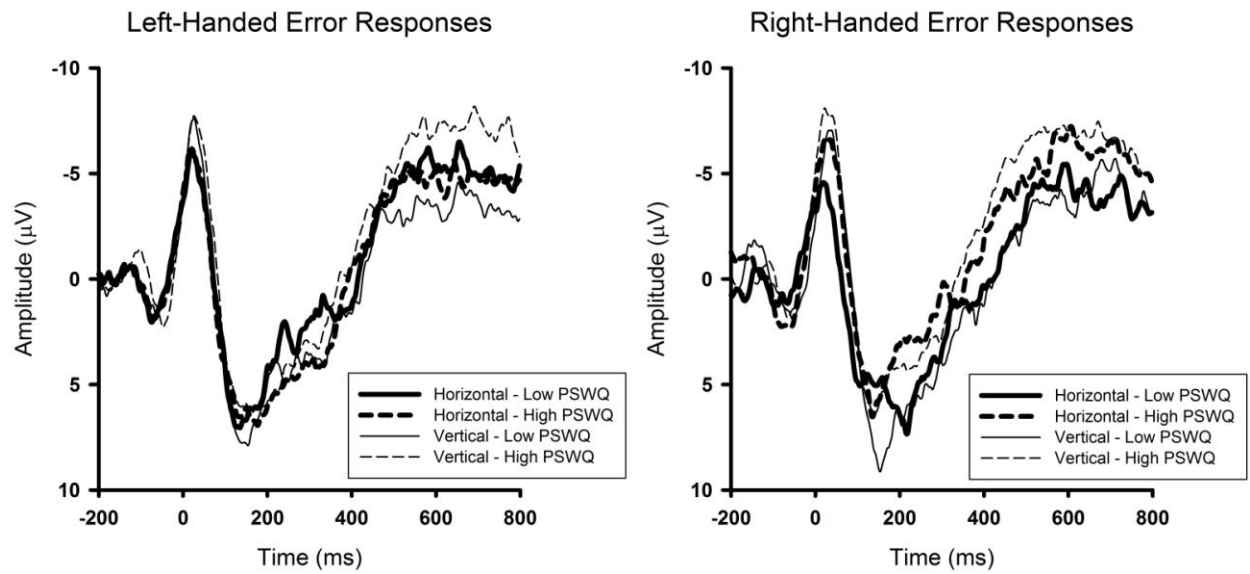
Figure 3. Experiment 2 Response Locked ERPs.
