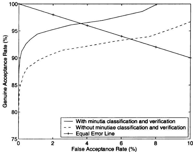
Figure 7.7: ROC for fingerprint verification when both minutiae classification and verification are used.
