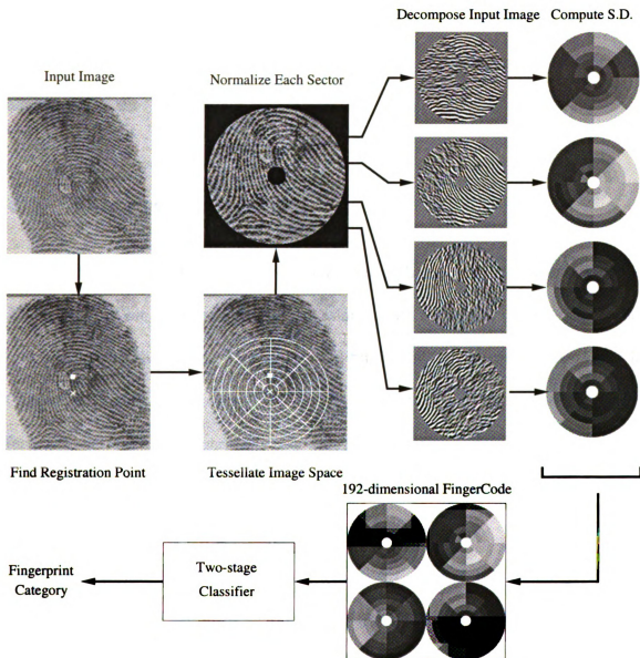
Figure 4.2: Flow diagram of our fingerprint classification algorithm.
