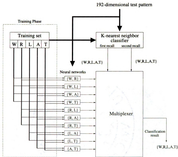
Figure 4.7: Two-stage classification scheme using K-NN and neural network classifiers.
