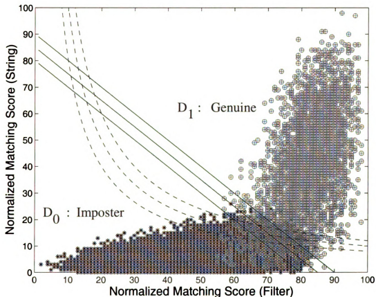
Figure 6.4: Plot of joint scores from matchers String and Filter . The solid lines denote the three sum rule decision boundaries corresponding to three different thresholds. The dotted lines denote the three product rule decision boundaries corresponding to three different thresholds.
