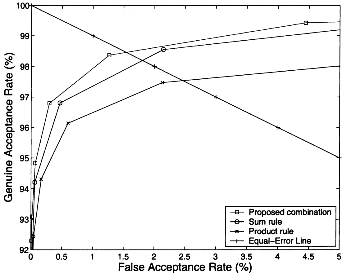
Figure 6.7: Comparison of the proposed combination scheme with the sum and the product rules for the String + Filter combination.
