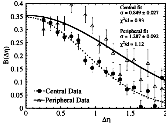
Figure 7.29: Pion pair balance function ( \Delta\eta ) for central (circles) and peripheral (open triangles) events, analyzed with the new, \eta -dependent normalization. Gaussian fits are applied omitting the first two bins.
