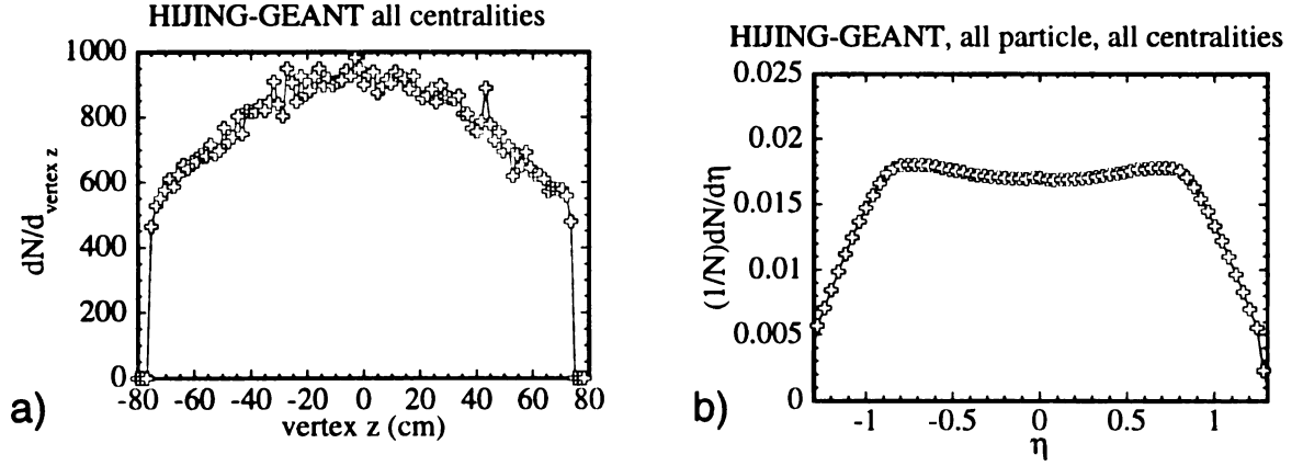
Figure 4.10: HIJING-GEANT a) non-normalized vertex distribution and b) normalized \eta distribution, both for charged particles.
