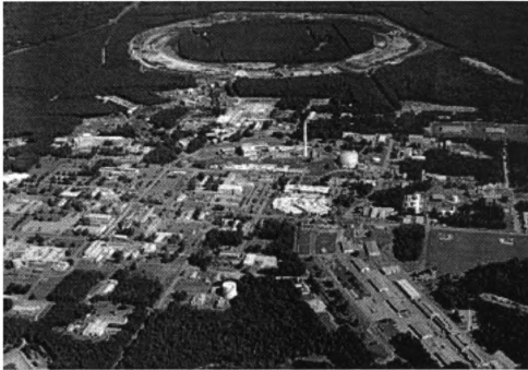
Figure 1.2: View of Brookhaven lab from the air showing the RHIC ring (largest circle) [27].
