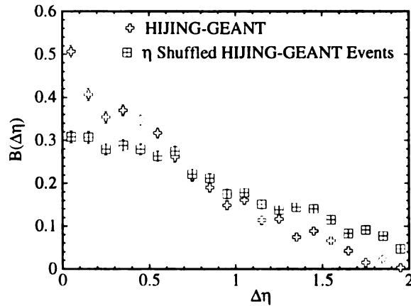
Figure 7.8: Charged particle balance function. HIJING-GEANT events are plusses, shuffled \eta events are represented by squares with + 's.
