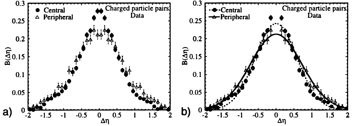
Figure 5.28: Charged particle pair balance function for central (circles), and peripheral (triangles) events of the complete data set. Measurements are shown both a) with all bins and b) omitting two middle bins with the dashed line showing the central Gaussian fit, and the solid line showing the peripheral Gaussian fit.
