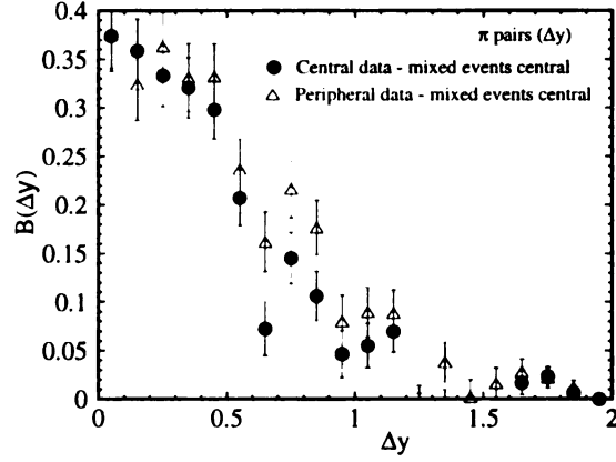
Figure 7.3: Pion pair mixed event balance function subtracted from the pion pair balance function. Central data are dots, peripheral events are triangles.
