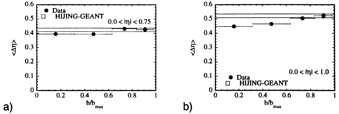
Figure 7.13: Charged particle balance function widths. Data (circles), and HIJING-GEANT (shaded bar) events are analyzed for particles with a) |\eta| < 0.75 , and b) |\eta| < 1.0 .
