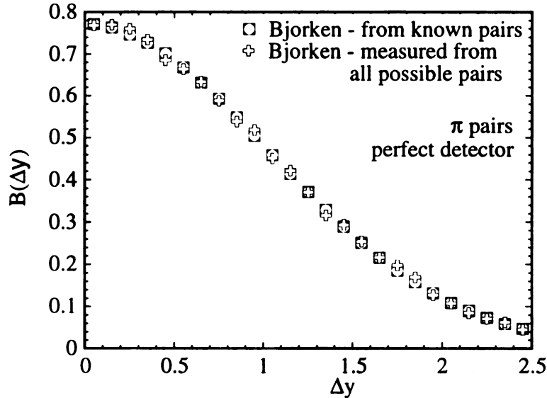
Figure 3.2: The shape of the balance function plotted for a perfect detector. Plusses are from the statistical measure, whereas squares with circles are from known balancing pairs.
