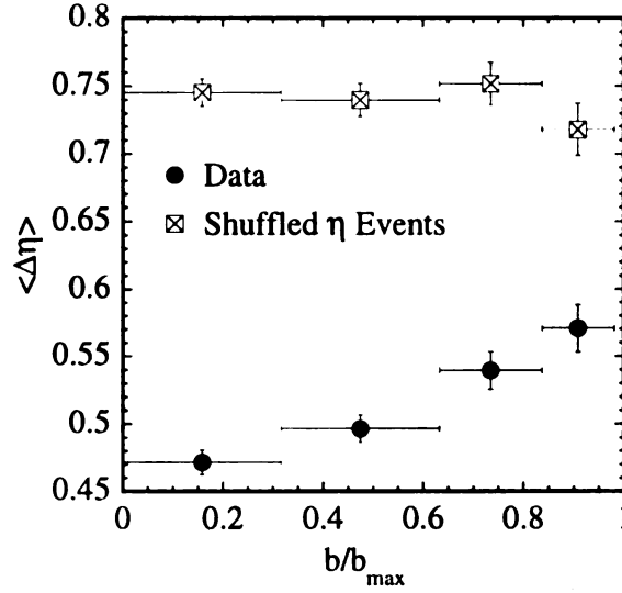
Figure 7.7: Charged particle balance function widths. Unmixed data are dots, shuffled \eta events are represented by squares with x's.
