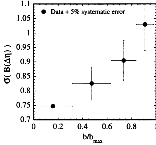
Figure 7.31: Charged particle pair balance function Gaussian fit widths for data (circles), analyzed with the new, \eta -dependent normalization. Width error bars have an additional 5% systematic error.
