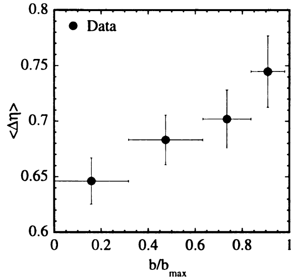
Figure 5.11: Summary of widths of the pion pair balance functions ( \Delta\eta ) for the four centrality bins of the data, plotted with respect to impact parameter. The first two bins were removed from the data for the width calculation.
