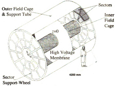
Figure 2.2: Schematic of the STAR Time Projection Chamber [28].
