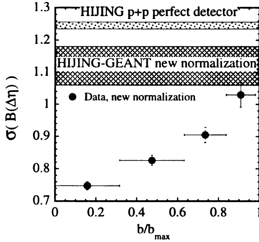
Figure 7.33: Charged particle pair balance function Gaussian fit widths for data (circles), analyzed with the new, \eta -dependent normalization. The top shaded bar shows old normalization HIJING p+p events Gaussian width. The lower shaded bar shows the Gaussian width for HIJING-GEANT events analyzed with the new normalization.
