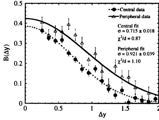
Figure 7.27: Pion pair balance function for central (circles) and peripheral (open triangles) events, analyzed with the new, \eta -dependent normalization. Gaussian fits are applied omitting the first two bins.
