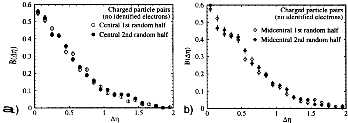
Figure 7.40: Charged particle balance function for a) central 1st (open circles) and 2nd (closed circles), and b) midcentral 1st (open diamonds) and 2nd (closed diamonds) half of the data set.
