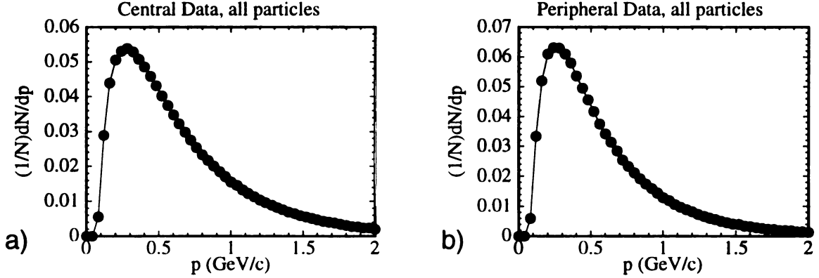
Figure 4.3: All charged particles normalized momentum distribution for a) central and b) peripheral events.
