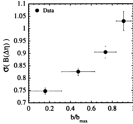
Figure 7.26: Charged particle pair balance function Gaussian fit widths for data (circles), analyzed with the new, \eta -dependent normalization.
