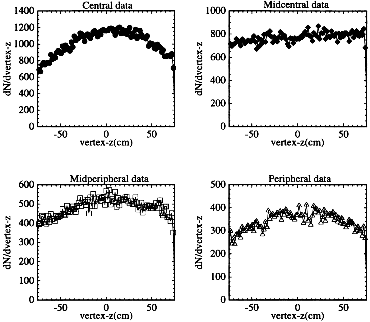
Figure 2.8: Vertex distribution for year 2000 events used in the analysis, all four centralities are shown.
