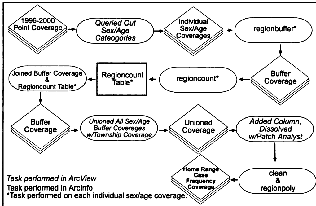
Figure 6. Data Flow Diagram of Home Range Case frequency Coverage
