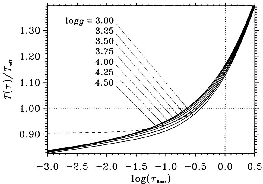
Fig. 19. The change of the T - \tau relation with gravity, for fixed, solar T_{\text{eff}} = 5777 K. The horizontal dotted line indicates the effective temperature, and the vertical dotted line, optical depth unity. The dashed line shows the grey atmosphere.
