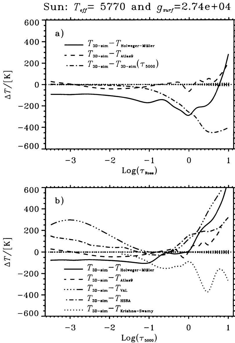
Fig. 15. Comparison of the T - \tau relation from the simulation, with some often used solar T - \tau relations. a) The difference in Rosseland T - \tau relations between the simulation and an Atlas9 atmosphere model (Kurucz 1993; Castelli et al. 1997). b) Differences, on a \tau_{5000} -scale, between the simulation and an Atlas9 model, and four semi-empirical atmosphere models: The model by Holweger & Müller (1974), the classical fit by Krishna Swamy (1966a; 1966b), the HSRA model (Gingerich et al. 1971) and the VAL model (Vernezze et al. 1981).
