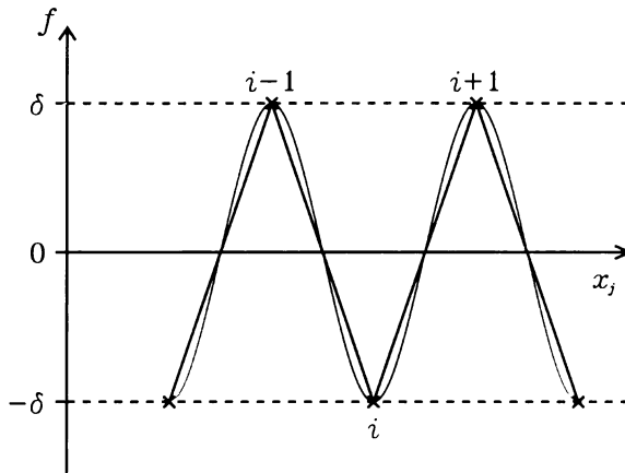
Fig. 1. Schematic of a pure two-zone oscillation. The thin curve is an example of a smooth interpolating function, illustrating the zero derivatives at the grid-points, which are marked with \times .
