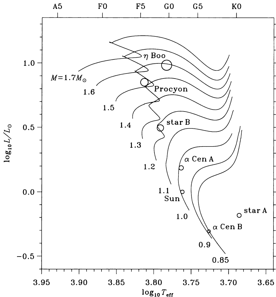
Fig. 21. The position of the seven simulations in the HR-diagram. The size of the symbols, reflects the diameter of the star. I have also plotted evolutionary tracks, with masses as indicated, to put the simulations in context.
