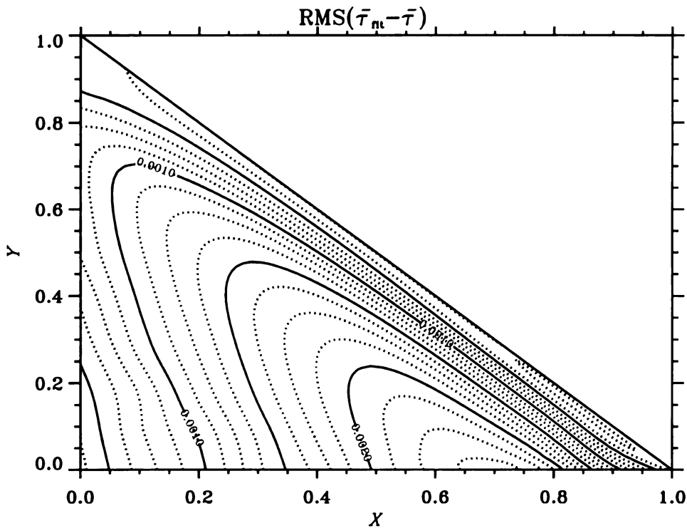
Fig. 8. The RMS-deviations of the \bar{\tau} evaluated from the fifth-order binomial fits, from the exact expression, Eq. (81). The dotted contours are spaced 0.0125% apart and solid contours are 0.05% apart.
