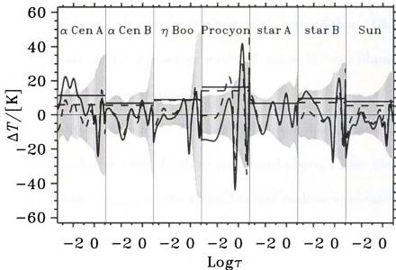
Fig. 16. Plot of the differences between the actual T - \tau relations and the global fit (solid line) and the individual fits (dashed line). The horizontal solid and dashed lines are the corresponding RMS deviations from the fits. The shaded areas show the RMS of the temporal variation of the temperature.
