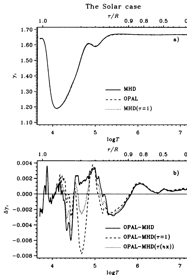
Fig. 20.— \gamma_1 for the solar track and the H-He mixture. a) the absolute value, b) the difference (OPAL minus MHD).
