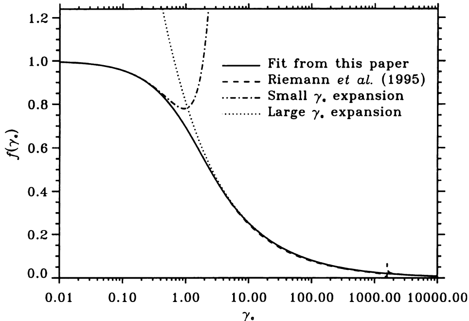
Fig. 7. The quantum diffraction term, as evaluated from Eq. (65) and (66), compared with the Padé-formula given by Riemann et al. (1995) and with analytical expansions for small and large \gamma .
