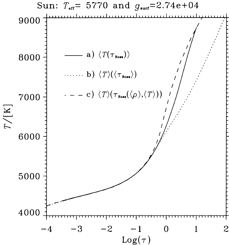
Fig. 14. The effect of various averaging techniques applied to a solar simulation (see text for details). Notice how cases a) and b) follow closely in the atmosphere down to \langle T \rangle = T_{\text{eff}} , at \log_{10} \tau \simeq -0.2 .
