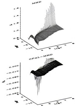
Fig. 2.— The logarithmic pressure derivative with respect to density \chi_e = (\partial \ln P / \partial \ln \varrho)_T for pure hydrogen in the upper panel, and its difference (OPAL minus MHD) in the lower panel.
