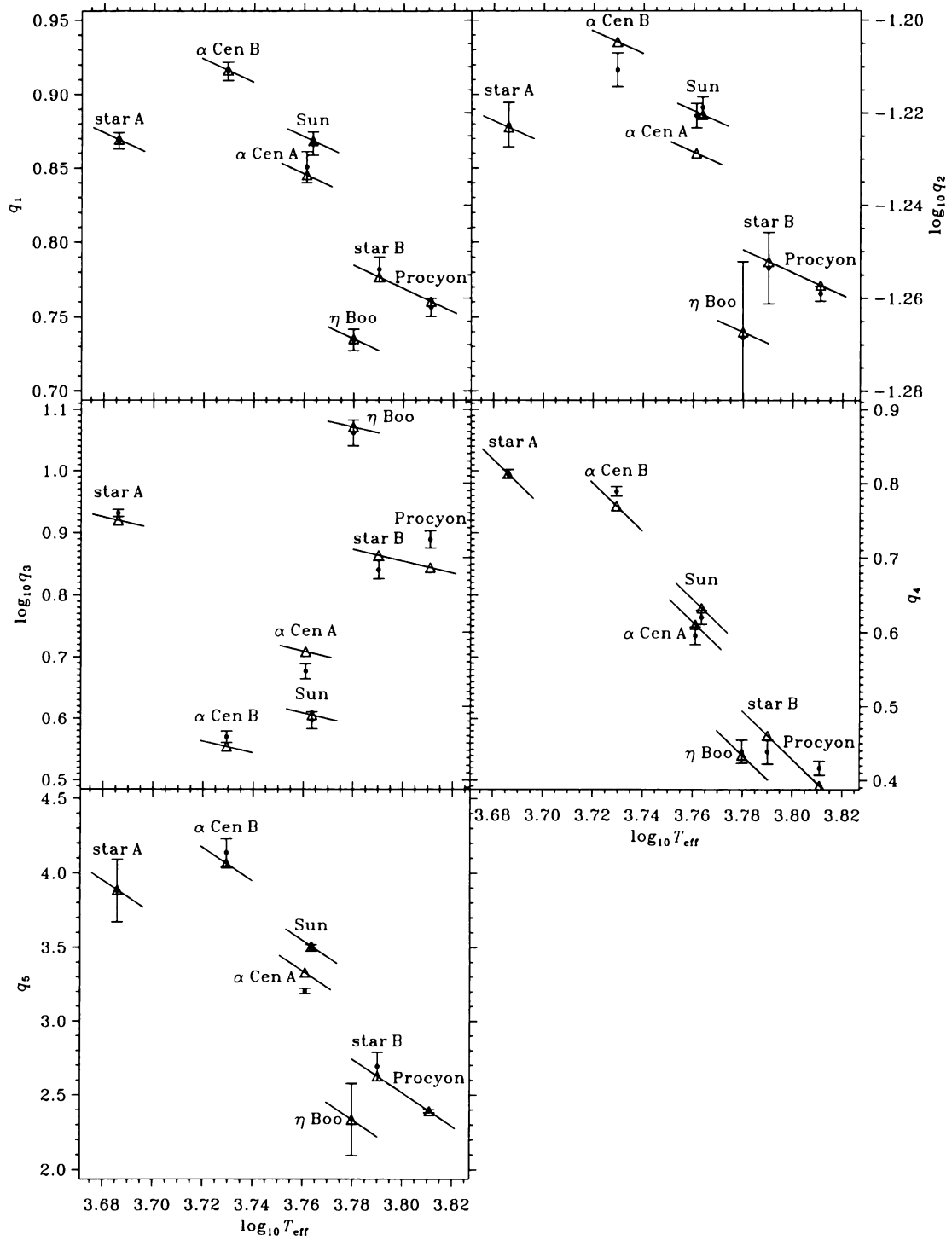
Fig. 17. Plot comparing the global (triangles) and individually (filled circles with error-bars) fit parameters for the T - \tau relation-fits. The line segments show the \log_{10} T gradient of the global fits. The error bars are the RMS-scatter from T - \tau relation fits to single time-steps of the simulations.
