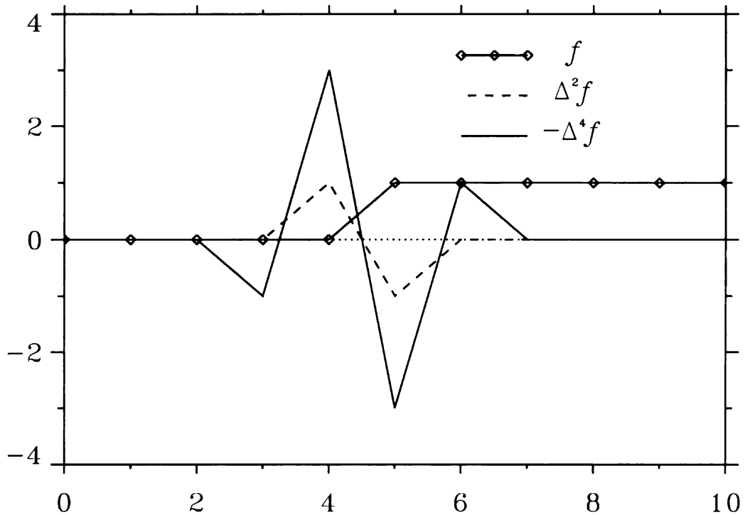
Fig. 2. Schematic of the response to a step function (solid line with diamonds). The dashed lined shows the corresponding linear second-order difference, and the solid line is the linear fourth-order difference.
