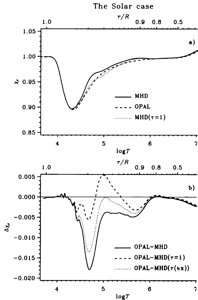
Fig. 14.— The logarithmic pressure derivative with respect to density, \chi_{\rho} , along the solar \rho , T -track for pure hydrogen. a) the absolute value, b) the difference (OPAL minus MHD).
