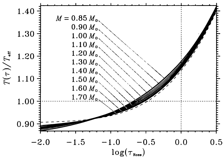
Fig. 18. The change of the T - \tau relation with stellar mass, on the zero-age main-sequence. The horizontal dotted line indicates the effective temperature, and the vertical dotted line, optical depth unity. The dashed line shows the grey atmosphere.
