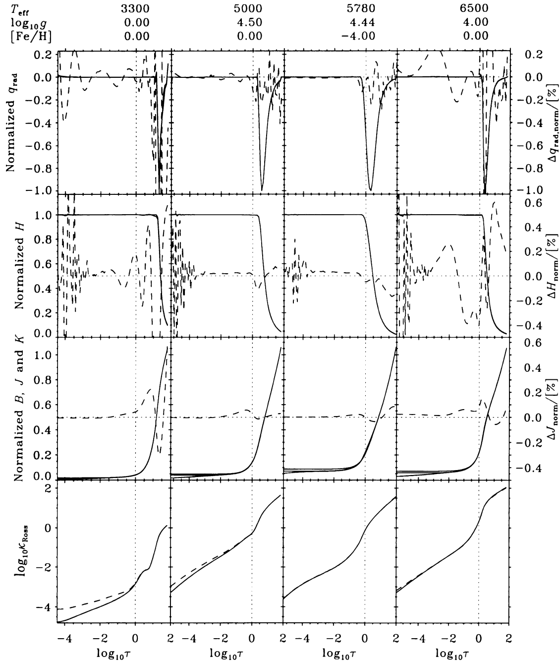
Fig. 12. Heating q , flux H , J , B , 3K and Rosseland opacity for four of the test cases (horizontally). In the three upper panels, the dashed lines (right axis) are the differences in the sense (SOS – monochromatic). In the lower panel the dashed line is the Rosseland opacity from my method. The horizontal dotted lines are the zero-points for the differences, and the vertical ones show the location of \tau = 1 . From left to right, the columns represent a red giant, a cool solar-type star, a metal-poor “Sun” and Procyon—a sub-giant.
