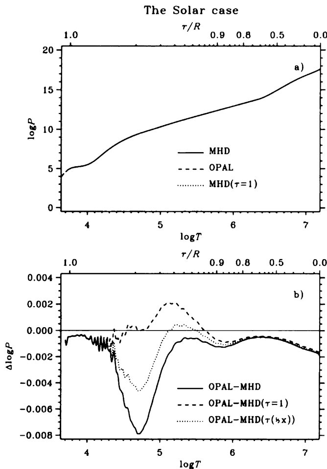
Fig. 13.— The logarithmic pressure along a solar \rho , T -track for pure hydrogen. The upper panel shows the absolute values of the MHD (solid line) and the OPAL (dashed line) pressure. We also plot the MHD pressure, using \tau = 1 to show the effect of omitting this correction ( cf. Sect. 2.2.2). These three pressures are indistinguishable unless we look at the lower plot, showing the difference OPAL minus MHD. Here we show, apart from the normal MHD, also the version with \tau = 1 , which seems closer to OPAL, and a version where we have halved the argument of \tau .
