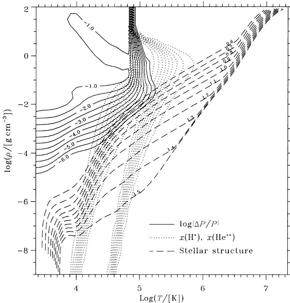
Fig. 4. This figure shows contours of the difference in pressure between including and ignoring the \Psi -term, in the sense \log_{10}|\Delta P/P| . The dashed lines going from lower left to upper right are tracks of stellar structure for stars in the mass range 0.6 - 1.5M_{\odot} , as indicated above each track. The dotted contour lines mark the hydrogen and second helium ionization zones respectively, with contour lines in steps of 10%.
