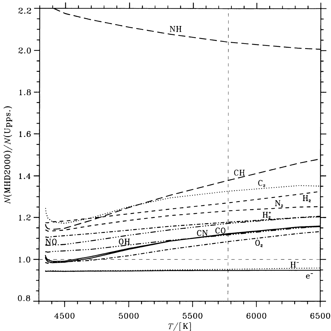
Fig. 11. Ratios of molecular number-densities between the present EOS and those obtained with the EOS in the Uppsala-package, which is part of the MARCS stellar atmosphere-models. The thin, horizontal, dashed line marks a ratio of one.
