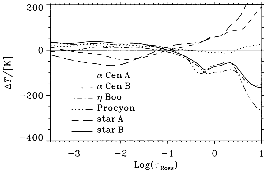
Fig. 20. Scaled T - \tau relations for the seven simulations, relative to the solar simulation in the sense: T_{\star} \times (T_{\text{eff},\odot}/T_{\text{eff},\star}) - T_{\odot} . The more vigorous the convection, the flatter the T - \tau relation.
