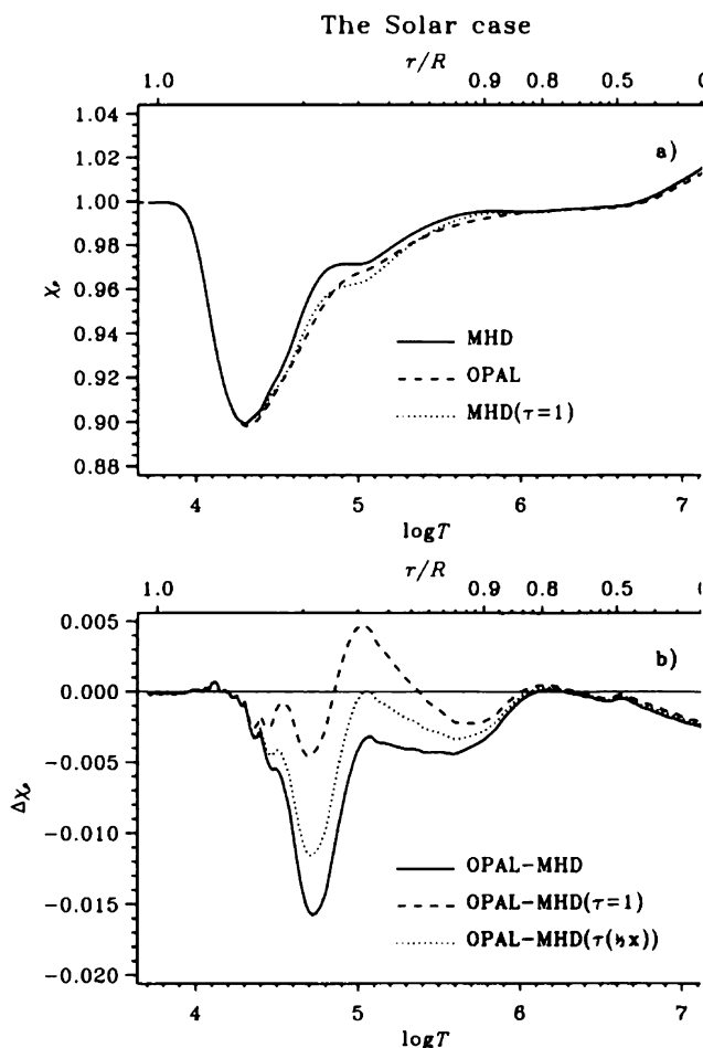
Fig. 18.— \chi_e for the H-He-mixture along the solar track. a) the absolute value, b) the difference (OPAL minus MHD).
