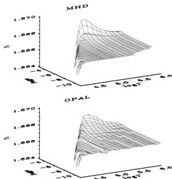
Fig. 25.— This is a zoom-in on the fully ionized, perfect gas region of a pure hydrogen plasma (cf. Fig. 4), where \gamma_1 = 5/3 . The upper panel shows the results for the MHD EOS which uses analytical expressions for all first- and second-order derivatives. The lower panel shows the same for the OPAL EOS, where derivatives are calculated numerically on a grid that are much denser in g and T though, than in the tables published.
