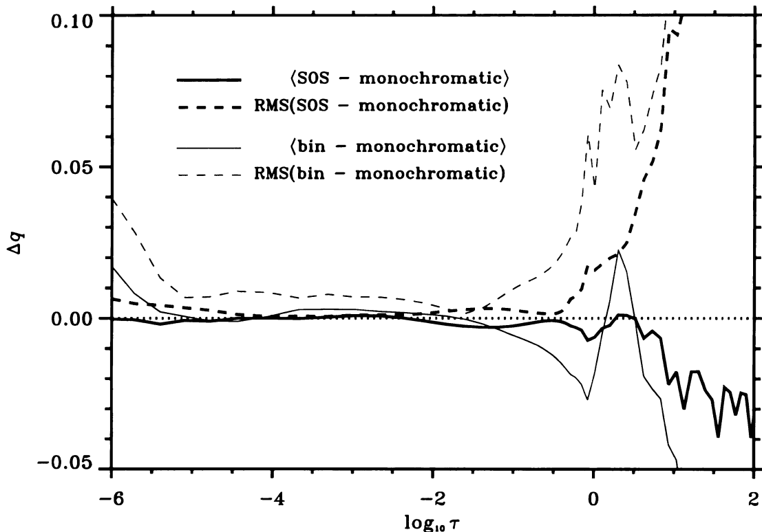
Fig. 13. Comparison of the heating from the opacity binning (bin, thin lines) and my new method (SOS, thick lines), with the “monochromatic” case (see text). A \langle . . . \rangle denotes horizontal averages over a 1.5 \times 6 Mm, 82 \times 200 point vertical slice from a solar simulation (solid). RMS denotes the corresponding horizontal root-mean-square averages (dashed lines).
