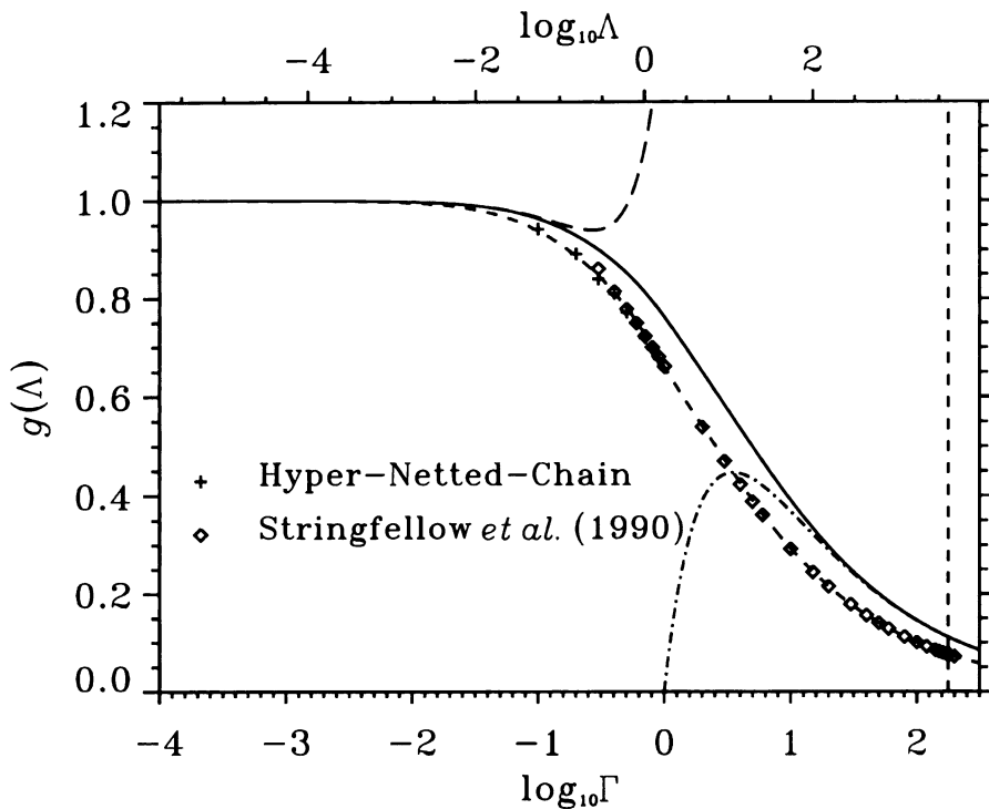
Fig. 10. The effect of higher order correlations on the free energy. The solid line is my fit to g = F/F_{\text{DH}} , Eq. (105) and the dashed line is the corresponding g_U = U/U_{\text{DH}} . The long-dashed line diverging at -0.5, is the Abe cluster expansion (Abe 1959), and the dot-dashed line is the fit to the fluid-phase free-energy presented in Stringfellow et al. (1990). The vertical dashed line shows the location of the transition to the crystalline phase.
