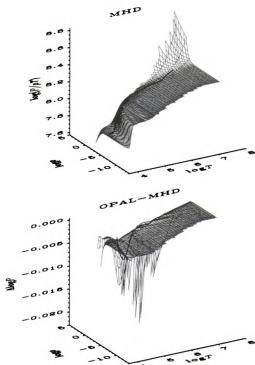
Fig. 5.— The reduced pressure, P/(gT) , for the H-He mixture in the upper panel, and its differences (OPAL minus MHD) in the lower panel.
