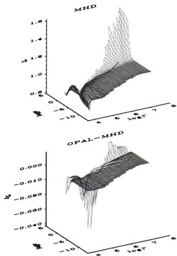
Fig. 10.— \chi_g , the logarithmic pressure derivative at constant temperature, for the full mixture in the upper panel, and its differences (OPAL minus MHD) in the lower panel.
