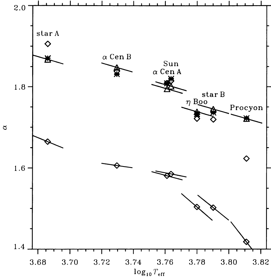
Fig. 22. A plot of the \alpha 's found from the matching procedure (stars), compared with the linear fit from Eqs. (183) and (184) (triangles). The (lower) diamonds show the 2D calibration by Ludwig et al. (1999), which I have also multiplied by 1.14 to agree with my result for the Sun (upper diamonds). The line-segments show the local \text{Log}T -derivative of the fitting expressions.
