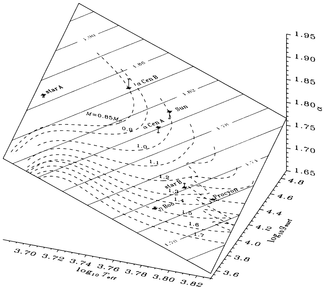
Fig. 23. This figure shows \alpha 's behavior with T_{\text{eff}} and g_{\text{surf}} . The surface is the fit given in Eq. (183). The dashed lines shows evolutionary tracks for stellar masses as indicated. The stars show the \alpha 's as listed in Tab. 10 and the little circles, connected by lines, show the projection onto the fitting-plane.
