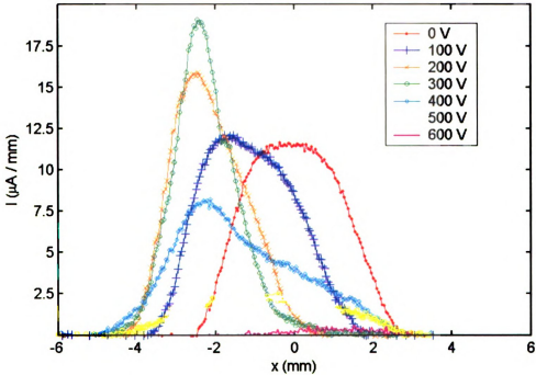
Figure 17: Transverse beam profiles measured with the first horizontal scanning wire for different voltages in the chopper. When the plates are biased to more than \pm 600\text{V} , the beam is deflected and is not injected.
