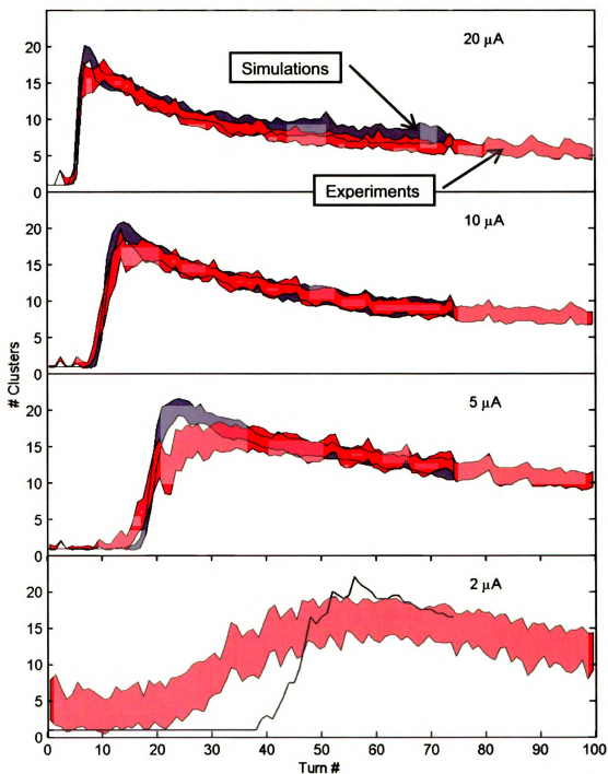
Figure 91: Comparison in the evolution of the average number of clusters between simulations (characteristics of the bunches listed in Table 9) and experiments (characteristics listed in Table 21).
