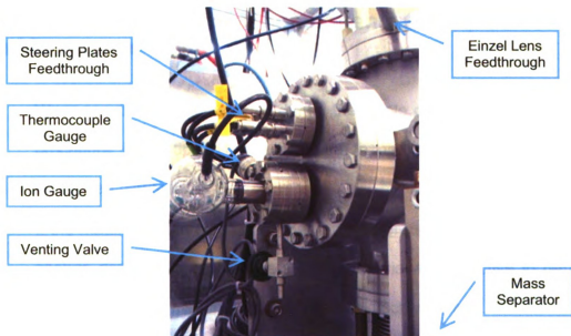
Figure 106: Picture of the venting valve and one of the thermocouple gauges used in the injection line of SIR.
