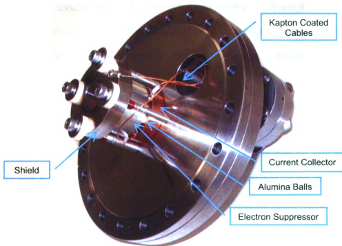
Figure 22: Picture of the Faraday cup at the end of the injection line of SIR.
