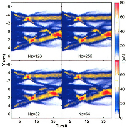
Figure 62: Evolution of the longitudinal profile of a bunch with characteristics listed in Table 7 for different values of N_z (Number of grid points in the FFT algorithm used to calculate the space charge electric field in the z direction (perpendicular to the medium plane of the ring)).
