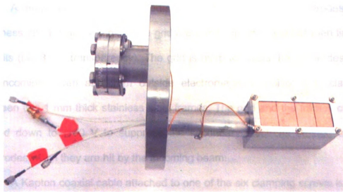
Figure 27: Picture of the sector fast Faraday cup used to measure beam longitudinal profiles when they are extracted from the ring.
