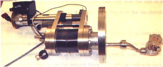
Figure 31: Picture of the movable fast Faraday cup used to measure longitudinal beam profiles.
