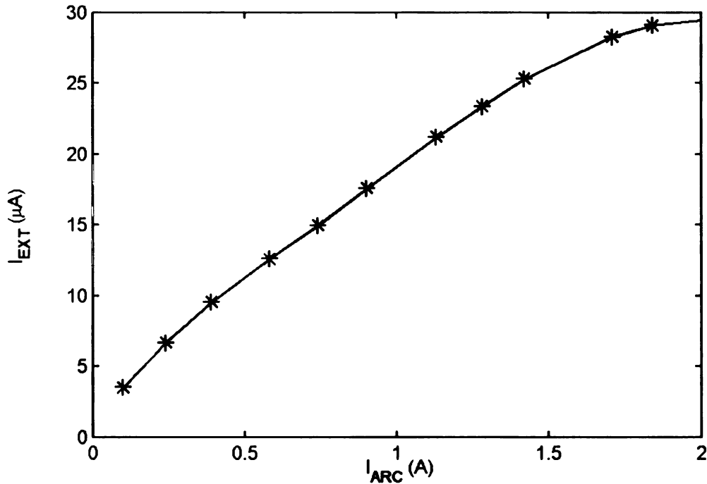
Figure 51: Relationship between arc current and the extraction current of \text{H}_2^+ ions when the filament power is changed as shown in Figure 52. The value of the arc voltage, extraction voltage and pressure are kept constant. (Values are listed in Table 5.)
