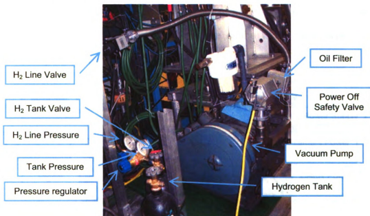
Figure 95: Picture of the hydrogen tank and regulator.
