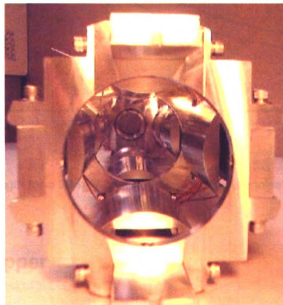
Figure 14: Picture of the triplet of electrostatic quadrupoles used in the injection line of SIR.
