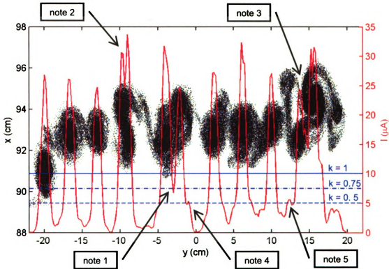
Figure 59: Top view (in black) and longitudinal profile (in red) of a H_2^+ bunch 60 turns after being injected. The energy when it was injected was 20 keV, the peak current 10 \mu A, the length 300 ns and the emittance 30 \pi mm mrad.
