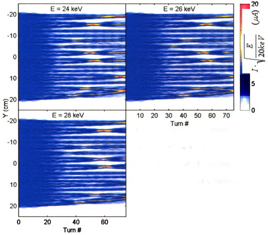
Figure 76: Waterfall diagrams representing the evolution of the longitudinal bunch profile for energies ranging from 24 keV to 28 keV. The other parameters that characterize the bunch are listed in Table 12.
