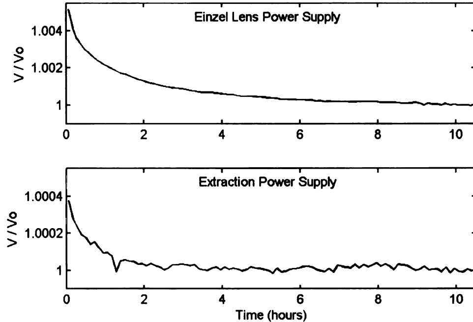
Figure 47: Long term variability of the extraction and Einzel lens power supplies. V_o for the Einzel lens power supply is 16.5 kV and for the extraction power supply is 20 kV. The variability of these voltages was monitored over a period of 10 hours.
