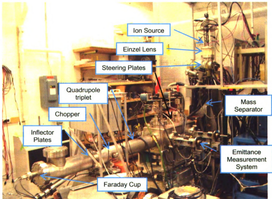
Figure 4: Picture of the injection line of SIR.
