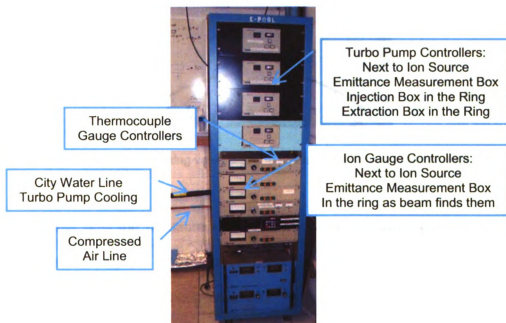
Figure 105: Picture of the vacuum system control area.
