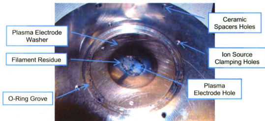
Figure 102: Picture of the flange that holds the ion source and the plasma electrode washer.
