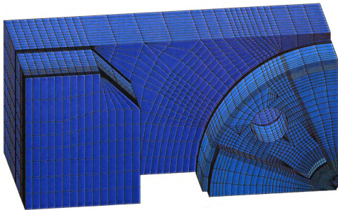
Figure 2.5: This figure shows a three dimensional model of the magnet steel shape used in TOSCA to calculate the fields of the ion source test stand magnet. Due to the symmetry, only \frac{1}{8} of the magnet needed to be modeled.
