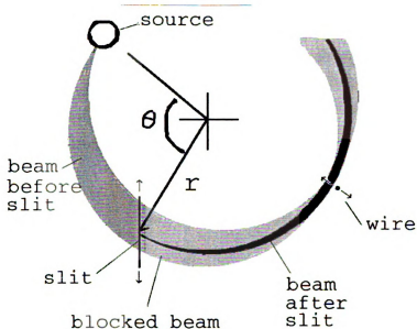
Figure 1.9: Simplified schematic of slit and wire probes for measuring radial emittance. Shown are the relative location of the source, slit and wire. (The diagram does not include focusing effects of the electric field between the source and the puller.)
