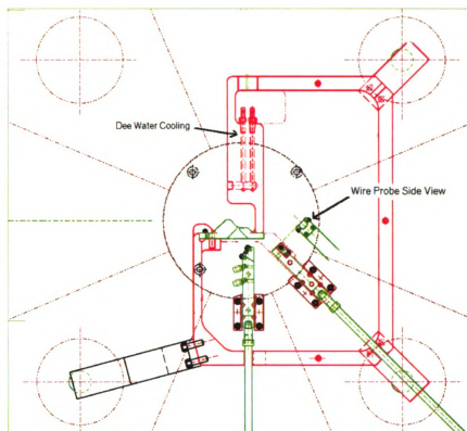
Figure 2.11: Drawing of High Voltage Dee.
