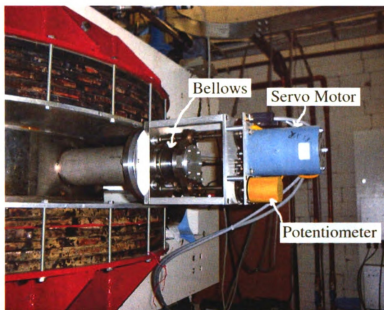
Figure 2.14: Probe Control Servo.
