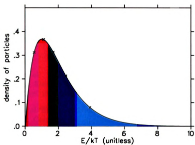
Figure B.1: Maxwell-Boltzmann Distribution of Particle Energies
