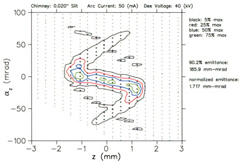
(b) 0.020" Chimney Axial Emittance
