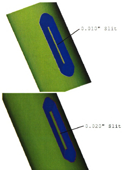
Figure 3.7: The two slit chimneys that were used are shown. One chimney has a 0.010" (0.254 mm) slit. The other has a 0.020" (0.508 mm) slit. Both have a 10° chamfer.
