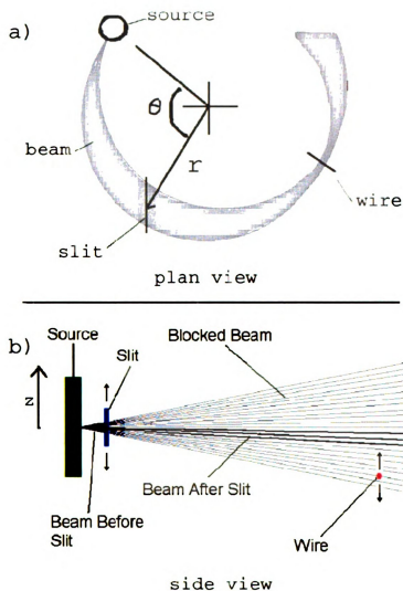
Figure 1.8: Simplified schematic of slit and wire probes for measuring axial emittance. The plan view (a) shows the relative location of the source, slit and wire. The side view (b) shows the motion of the slit and wire with respect to the beam. The diagram does not show the effect of the electric field between the source and the puller on the beam.
