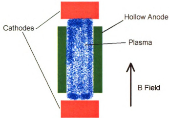
Figure 1.1: Geometry of a Penning Discharge as Used in Internal Ion Sources. (Images in this dissertation are presented in color.)
