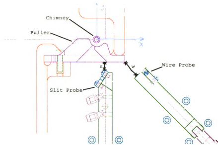
Figure 2.12: A CAD drawing of the central part of the ion source test stand. Visible are the chimney, puller and the slit and wire probes. Parameters s and w are recorded along with the current on the slit probe and the current on the wire for each data point. Parameter s is defined as the distance from the back edge of the puller to the front tip of the slit probe. Parameter w is defined as the distance from the corner of the puller to the front edge of the wire probe.
