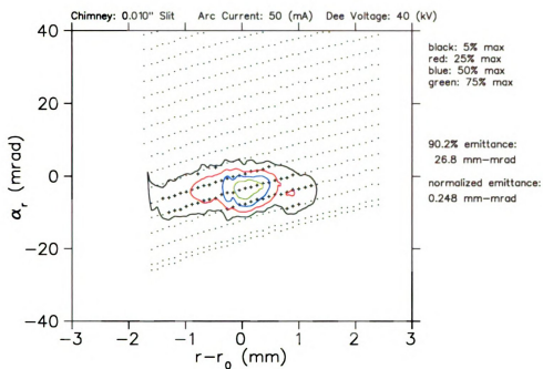
(a) 0.010" Slit Chimney Radial Emittance
