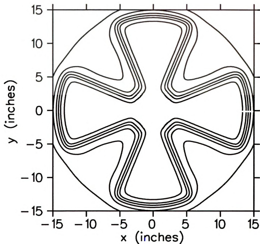
Figure 2.4: Shown is a measured magnetic field of the “High Intensity Test Cyclotron” version of the magnet i.e. before the “Ion Source Test Stand” modifications were made. The coil current for this measurement was 101 A. Magnetic field contours 3, 5, 7, 9, 11 and 13 kG from the outside working in; the maximum field being 13.6 kG.
