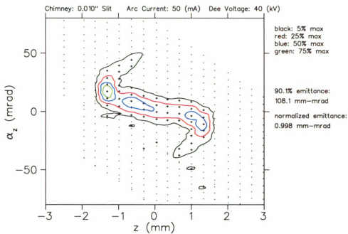
(a) 0.010" Chimney Axial Emittance
