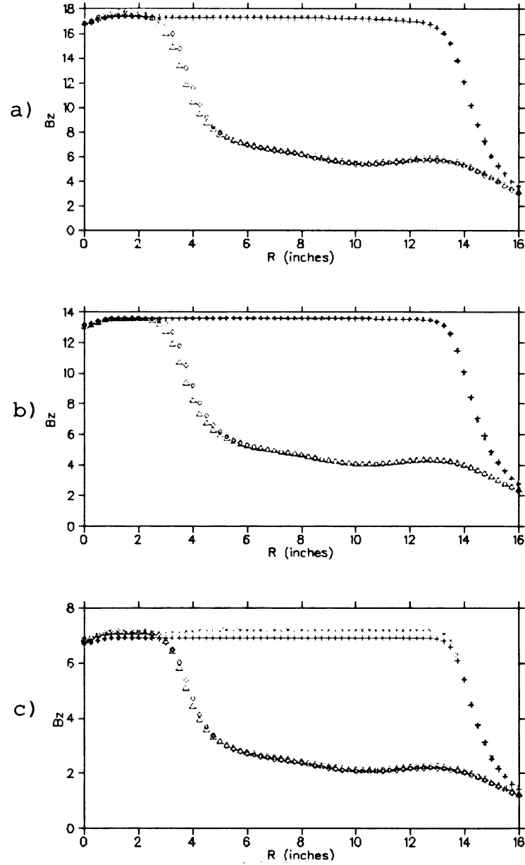
Figure 2.6: The measured magnetic field ( \times ) of the High Intensity Test Cyclotron magnet, and the calculated magnetic field (+) from TOSCA along two azimuths, one along a hill and another along a valley, for coil currents of (a) 152 amps, (b) 101 amps, and (c) 51 amps.
