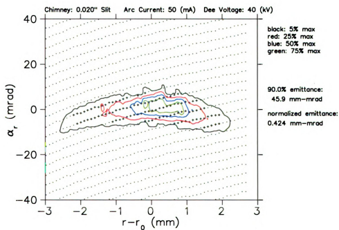
(b) 0.020" Slit Chimney Radial Emittance
