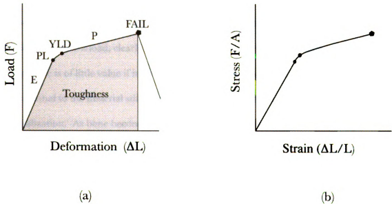
Figure 2-5. Structural and material properties. (a) Load-Deformation curve. E=elastic region of the curve, the slope of this region represents the rigidity of the structure; P=plastic region of the curve; PL=proportional limit; YLD=yield point; FAIL=failure point (=ultimate or failure strength of the structure); the shaded area under the curve represents the energy absorbed to failure (toughness). (b) Stress-Strain curve.
