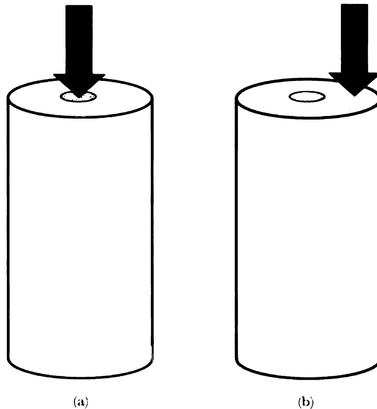
Figure 2-3. Axial loading. (a) Centric loading. (b) Eccentric loading.
