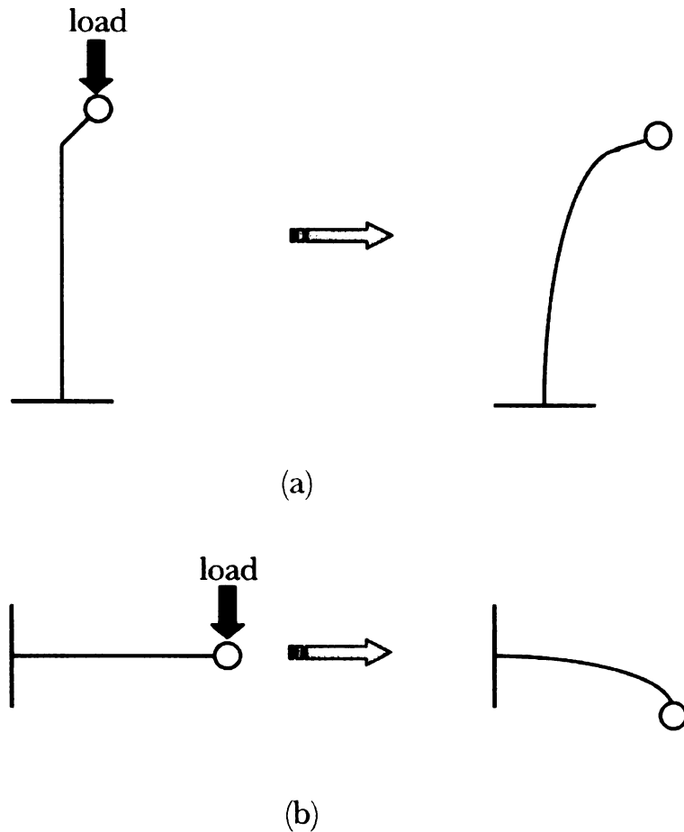
Figure 2-4. Loads that produce bending of long bones. (a) Eccentric column loading. (b) Cantilever beam loading.
