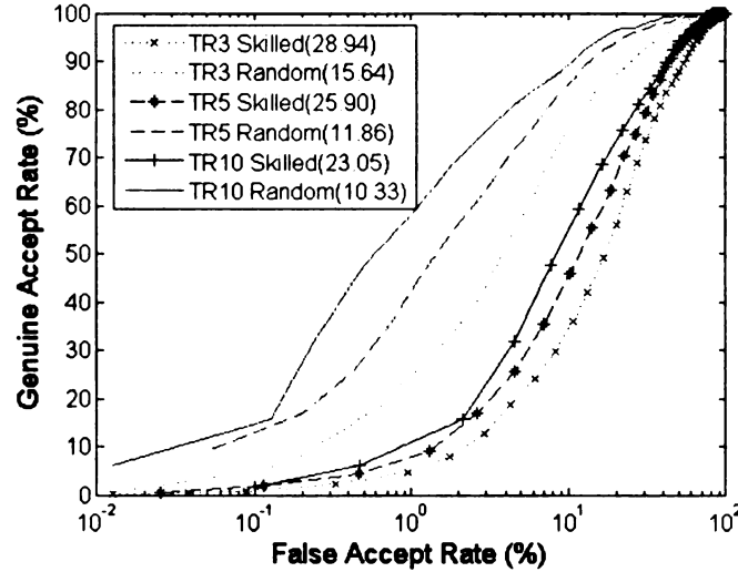
Figure 2.17: Average ROC Curves for the new signature verification algorithm using global features on the SVC database. Tests were run on both skilled and random forgeries and the results are presented separately. TR3, TR5, and TR10 are examples of testing with 3, 5, and 10 training samples, respectively. The equal error rate of each curve is shown in the parenthesis of the label.
