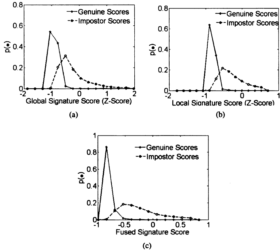
Figure A.2: Distribution of genuine and impostor signature scores from one trial of testing on the multimodal database after performing z-score normalization and sum rule fusion using weights of 0.1 and 0.9 for the global and local systems respectively; (a) Global (distance score), (b) Local (distance score) and (c) Fused scores using the sum rule.
