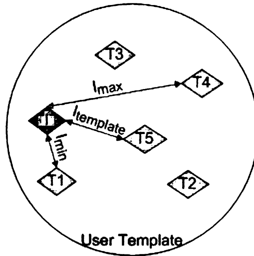
Figure 2.11: User-dependent normalization. I is the input signature and T_i , i = \{1, \dots, 5\} are the 5 stored templates for the claimed identity. The distances I_{min} , I_{max} , and I_{template} are used to construct the three-dimensional score vector. T_5 is selected as the template because it has the smallest average distance to all the other samples.
