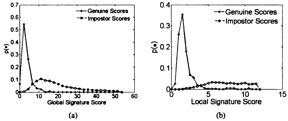
Figure A.1: Distribution of genuine and impostor signature scores from one trial of testing on the multimodal database; (a) Global (distance score) and (b) Local (distance score).
