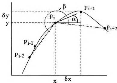
Figure 2.4: Features calculated for point p_i with respect to the shape of the signature [15].
