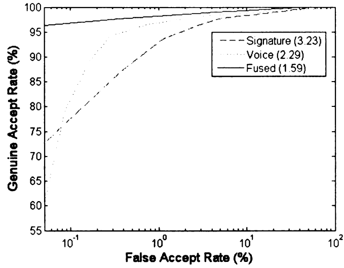
Figure 4.5: Receiver operating characteristic curves for the signature, voice, and fused system scores using min-max normalization. The equal error rate of each system is displayed in parenthesis in the legend.
