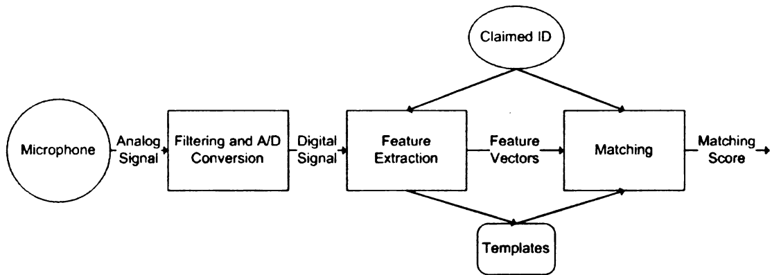
Figure 3.1: Design of a generic speaker verification system.
