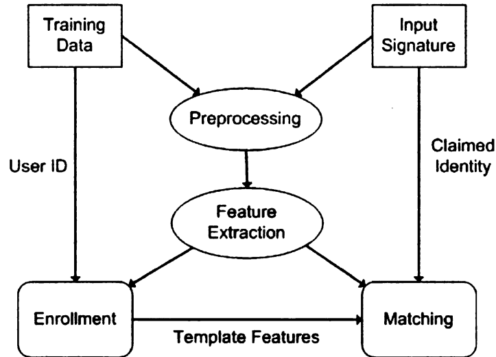
Figure 2.2: A typical signature verification system.
