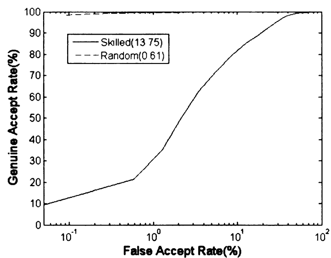
Figure 2.19: Average ROC Curves for the fused local and global scores on the SVC database. Tests were run on both skilled and random forgeries and the results are presented separately. Five training signatures are used for testing. The scores are normalized using the z-score normalization and the weighted sum rule was applied with weight of 0.95 and 0.05 for the local and global systems, respectively. The equal error rates of each curve is shown in the parenthesis of the label.
