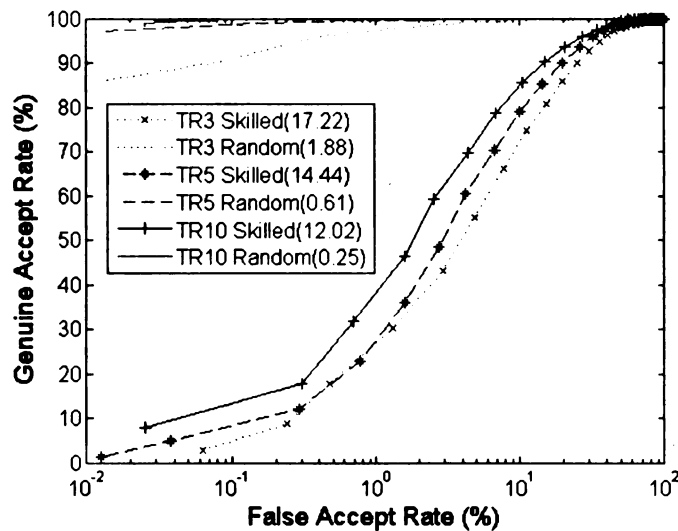
Figure 2.16: Average ROC Curves for the proposed signature verification algorithm on the SVC database using PCA dimensionality reduction. Tests were run on both skilled and random forgeries and the results are presented separately. TR3, TR5, and TR10 are examples of testing with 3, 5, and 10 training samples, respectively. The equal error rate of each curve is shown in the parenthesis of the label.
