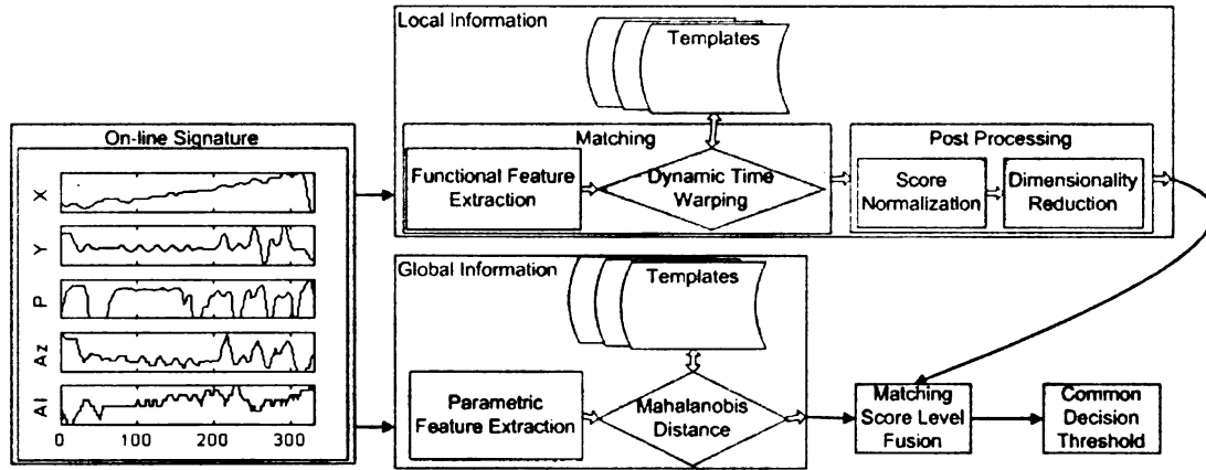
Figure 2.6: Block diagram of the signature verification system.
