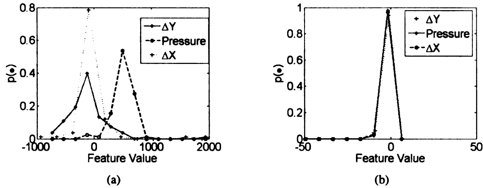
Figure 2.9: Feature normalization; (a) and (b) display the feature values before and after normalization, respectively.
