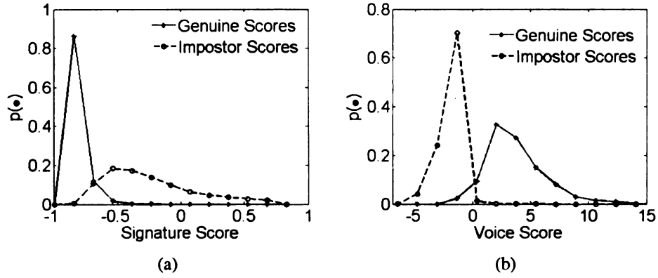
Figure 4.1: Distribution of genuine and impostor signature scores; (a) Signature (distance score) and (b) Voice (similarity score). Signature scores are based on the combination of local and global features.
