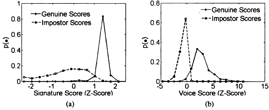
Figure 4.3: Distribution of genuine and impostor signature scores after z-score normalization; (a) Signature and (b) Voice.
