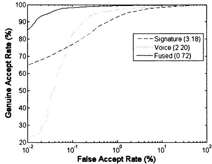
Figure 4.6: Receiver operating characteristic curves for the signature, voice, and fused system scores using z-score normalization. The equal error rate of each system is displayed in parenthesis in the legend.
