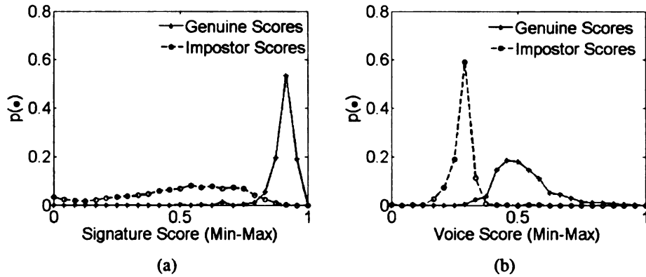
Figure 4.2: Distribution of genuine and impostor signature scores after min-max normalization; (a) Signature and (b) Voice.
