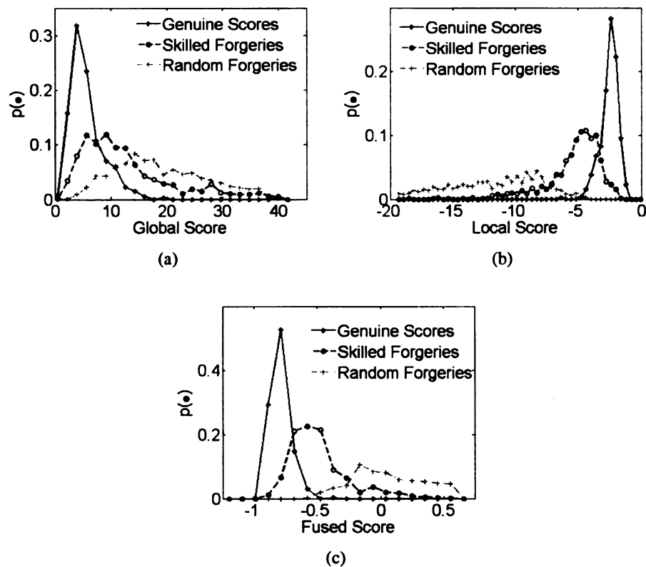
Figure 2.18: Distribution of genuine and impostor scores from one trial of SVC testing; (a) Global (distance score), (b) Local (similarity score), (c) After sum rule fusion (distance score).
