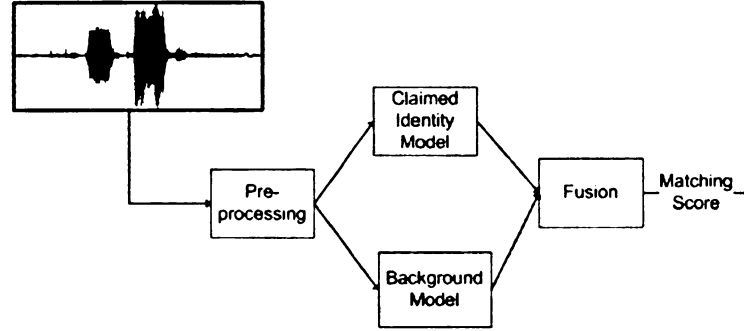
Figure 3.5: Speaker verification using a background model. A likelihood ratio is computed based on the probabilities generated from the claimed identity model and the background model to produce the matching score.
