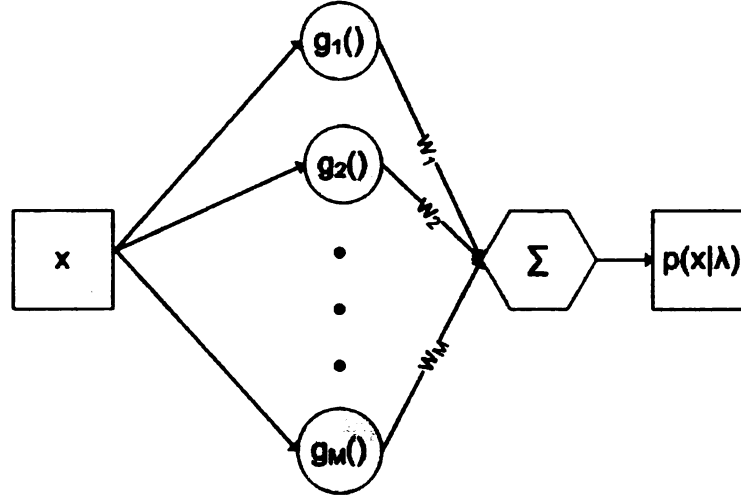
Figure 3.6: Diagram of a Gaussian mixture density representing the model for identity \lambda . g_i is the i^{\text{th}} Gaussian component, and w_i is the associated mixture weight. i ranges from 1 to m , where m is the number of components. Each Gaussian component is represented by a mean \mu_i and covariance matrix \Sigma_i .
