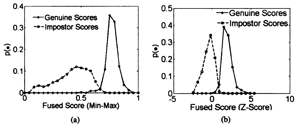
Figure 4.4: Distribution of genuine and impostor signature scores after sum rule fusion; (a) Min-Max normalization and (b) Z-Score normalization. The weights assigned to the signature and voice systems were 0.65 and 0.35, respectively.
