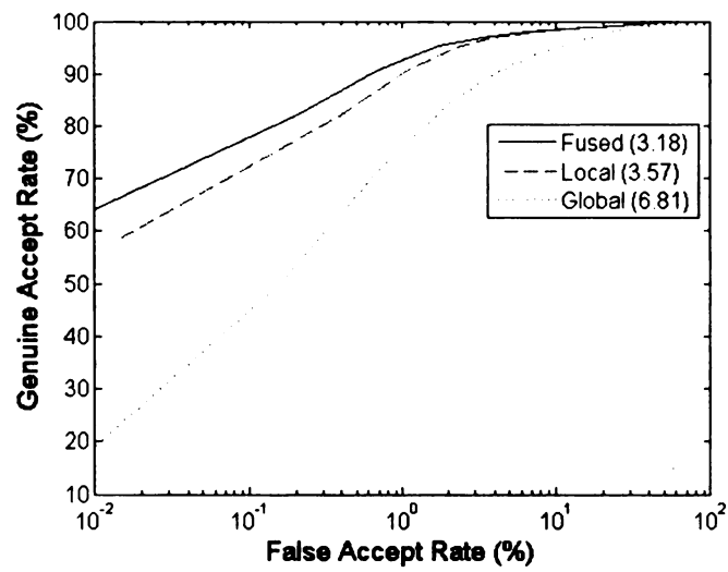
Figure A.3: Receiver operating characteristic curves for the global, local, and fused signature scores. The equal error rate (%) of each system is displayed in parenthesis in the legend.
