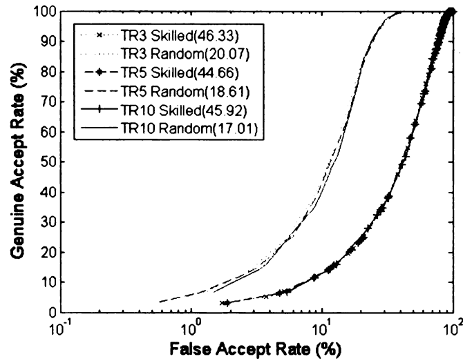
Figure 2.15: Average ROC Curves for the signature verification algorithm described in Section 2.2 on the SVC database. Tests were run on both skilled and random forgeries and the results are presented separately. TR3, TR5, and TR10 are examples of testing with 3, 5, and 10 training samples, respectively. The equal error rate of each curve is shown in the parenthesis of the label.
