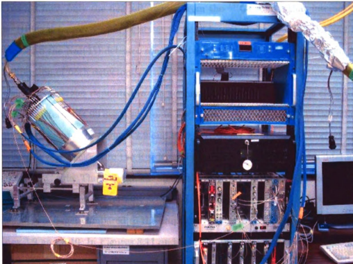
Figure 3.8: Experimental setup of the SeGA scanning stand.
