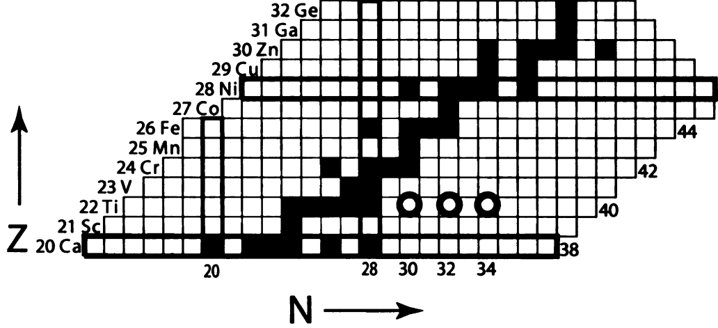
Figure 1.1: A section of the nuclear chart showing the region of interest. The black squares are the \beta -stable nuclei. The three titanium isotopes ( ^{52,54,56}\text{Ti} ) are circled.
