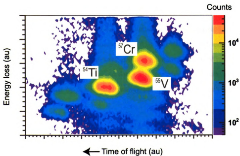
Figure 2.3: Particle identification spectrum for the ^{54}\text{Ti} setting. The number of counts is color coded and log scale.
