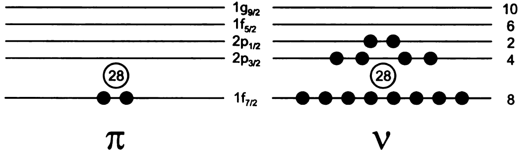
Figure 1.2: Simplistic view of the orbital structure for ^{56}\text{Ti} above the 1f_{7/2} shell
