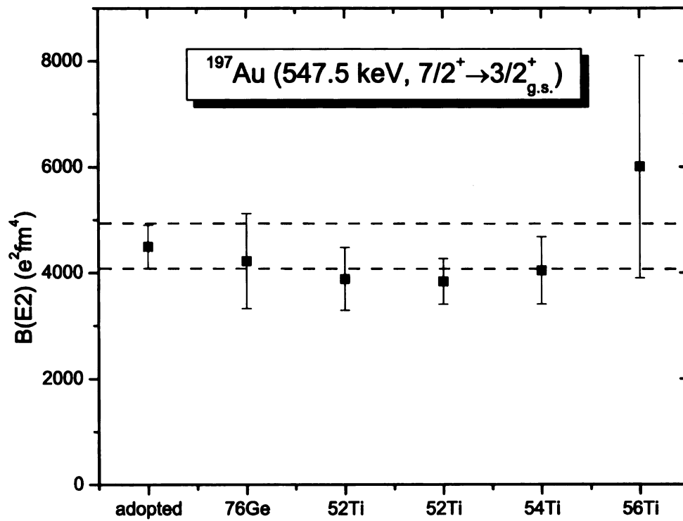
Figure 2.6: Measurement of the reduced transition probability from the ground state to the 7/2^+ state in the Au target for all beams used in this experiment.
