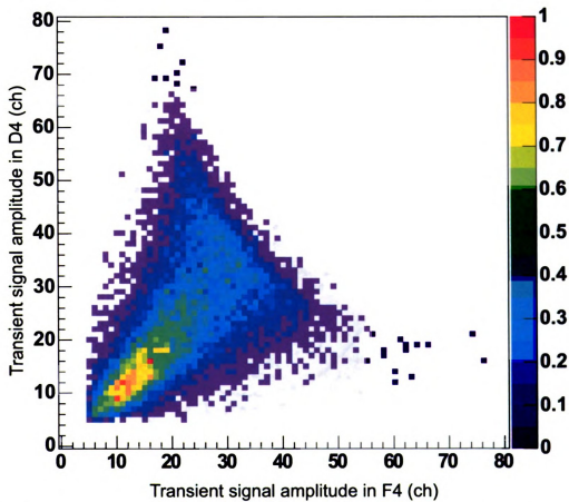
Figure 3.16: Amplitudes of the transient signals for segments F4 (horizontal) and D4 (vertical). The collimator is moved by 2 mm for each graph. Second position.
