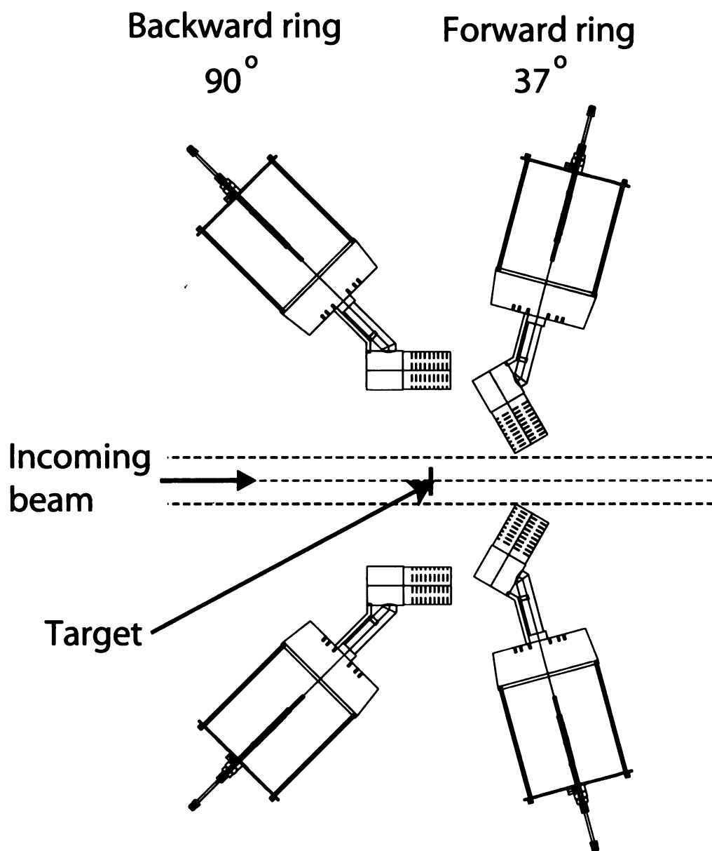
Figure 2.5: The segmented germanium detectors distributed in two rings around the secondary target position.
