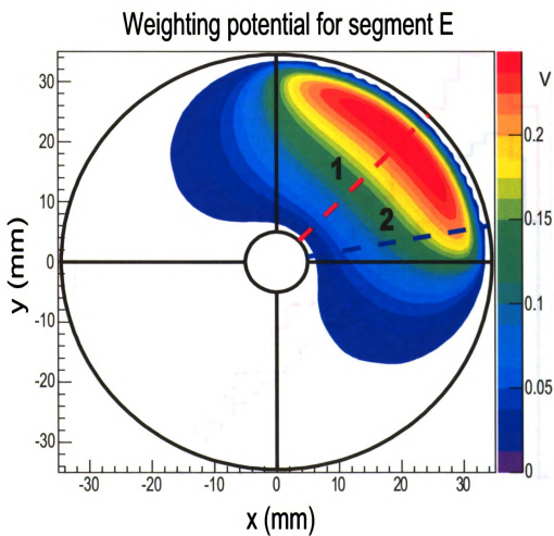
Figure 3.4: Weighting potential for segment E, transversal cut 2 mm above the border between segments E and D.
