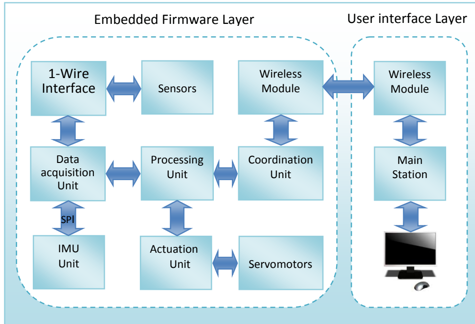
Figure 2.6: The software architecture.
