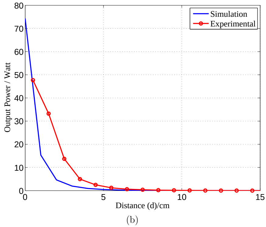
Figure 4.6: Simulation and experimental results: (a) input power vs. separation distance; (b) output power vs. separation distance.
