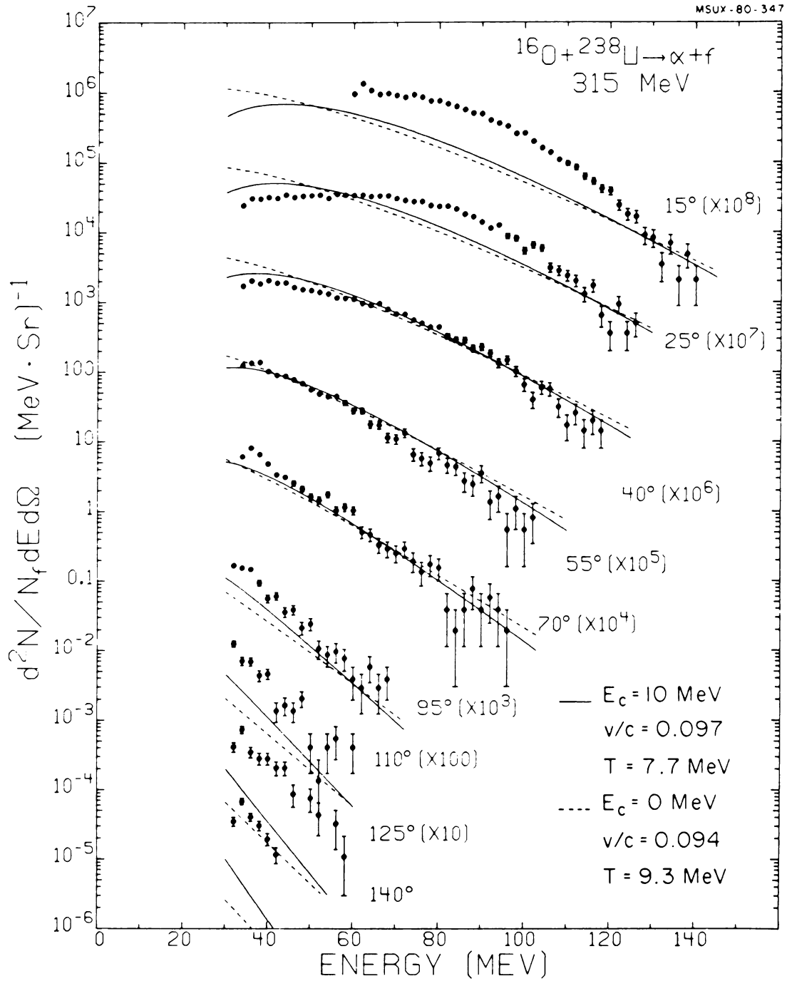
Figure V-29. Energy spectra of alpha-particles detected in the reaction ^{238}\text{U} (^{16}\text{O}, \alpha f) at 315 MeV. The curves have been calculated with the moving source model of Eq. (V-10). The laboratory angles and moving source parameters are indicated.
