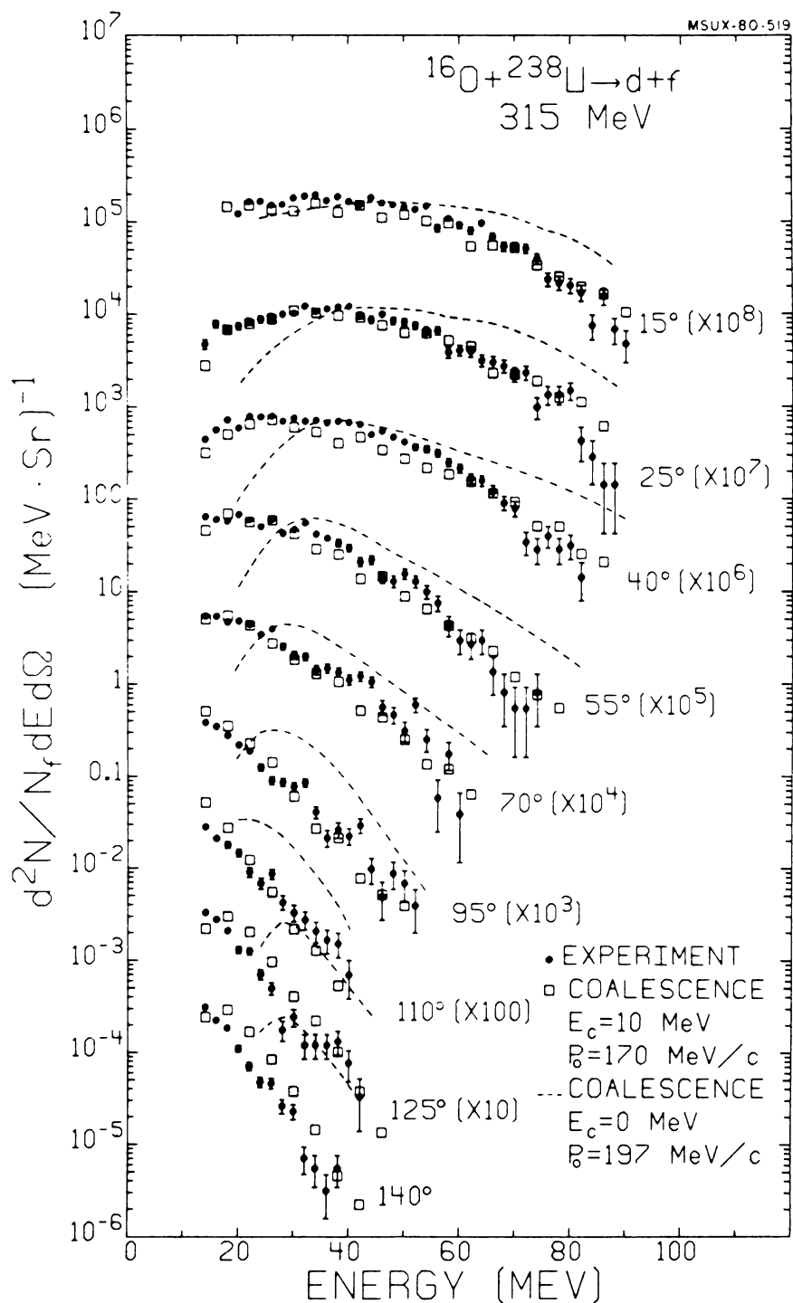
Figure VI-3. Energy spectra of deuterons (solid points) detected in the reaction ^{238}\text{U} ( ^{16}\text{O} , \text{df} ) at 315 MeV. The open squares are spectra predicted by the Coulomb-modified coalescence model; the dashed curves are the predictions of the coalescence model if Coulomb effects are neglected.
