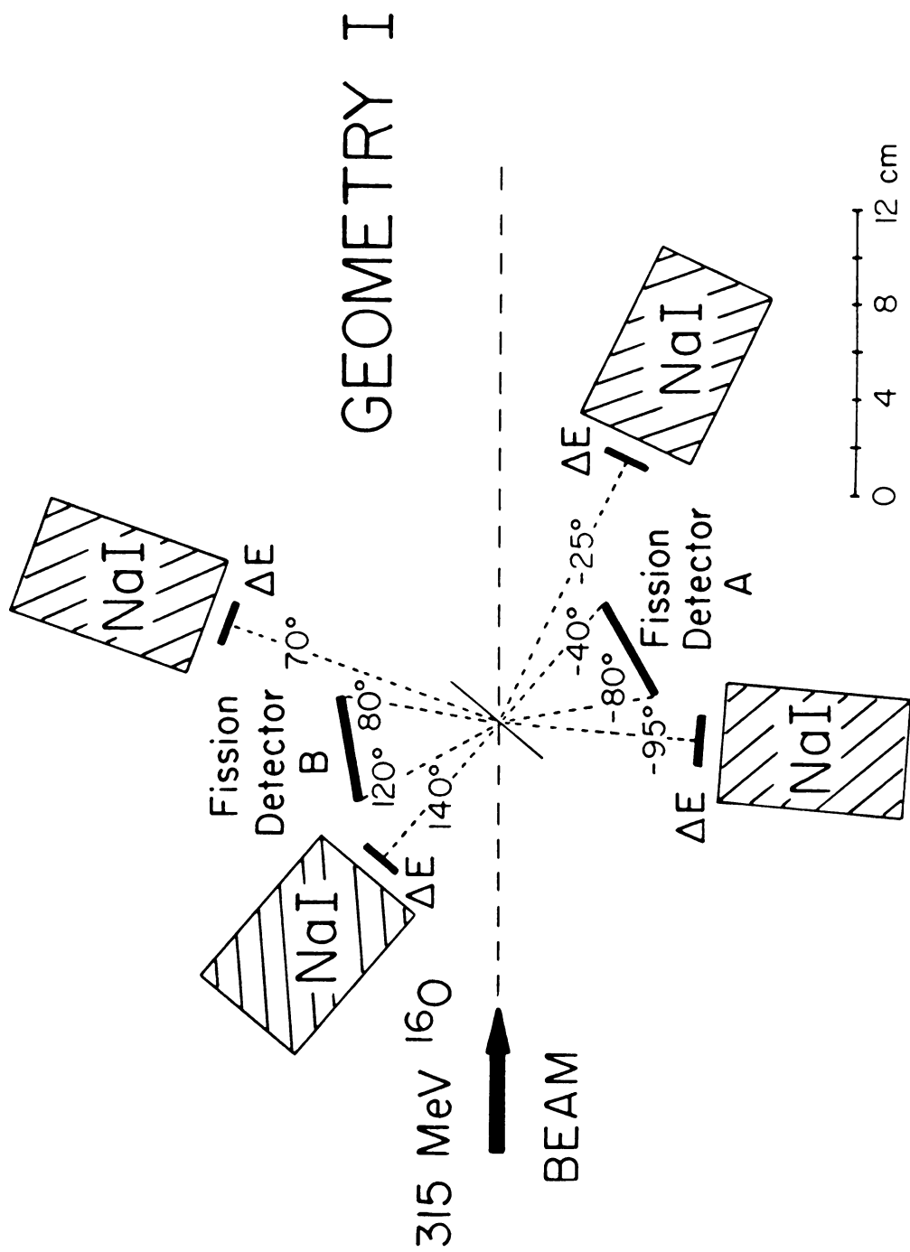
Figure II-2. Experimental geometry used in the experiment in which light particles were measured in coincidence with fission fragments.
