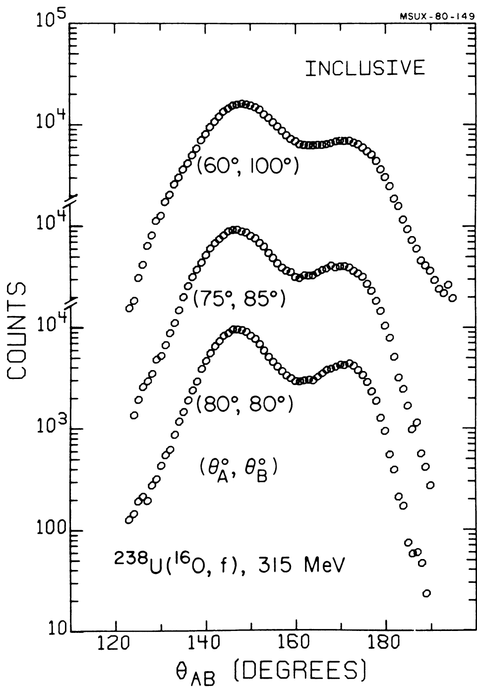
Figure V-1. Folding-angle distributions of fission fragments measured inclusively for the experimental geometries of this study ( \theta_A^\circ = 60^\circ , \theta_B^\circ = 100^\circ ; \theta_A^\circ = 75^\circ , \theta_B^\circ = 85^\circ ; and \theta_A^\circ = \theta_B^\circ = 80^\circ ).
