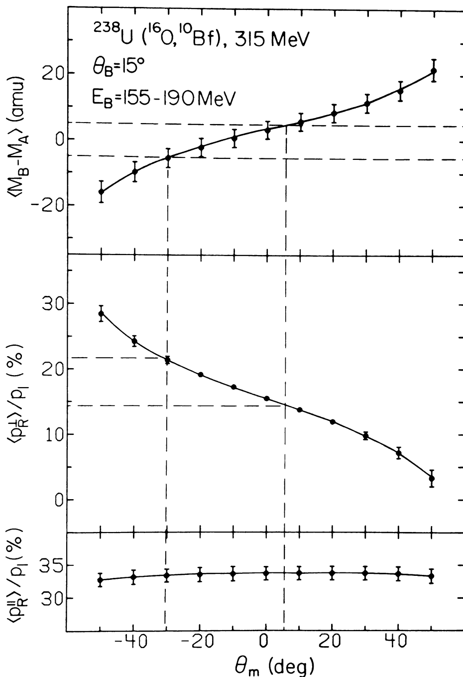
Figure III-4. The average mass difference \langle M_B - M_A \rangle of fission fragments detected in the two fission counters, the average transverse momentum of the recoiling nucleus \langle p_R^\perp \rangle and the average longitudinal recoil momentum \langle p_R^\parallel \rangle are shown as a function of the assumed angle of emission of the missing mass. Note the extreme insensitivity of \langle p_R^\parallel \rangle on \theta_m over the range of \theta_m , where approximate balance of fission fragment masses in the two detectors is achieved.
