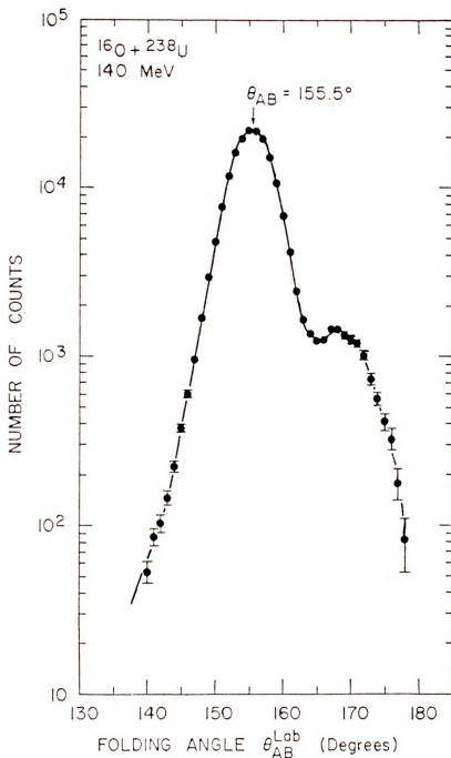
Figure A-2. Inclusive fission fragment folding-angle distribution for 140 MeV ^{16}\text{O} on ^{238}\text{U} . Data have been corrected for systematic errors due to imperfect beam and target positions, as well as the folding-angle dependent detection efficiency.
