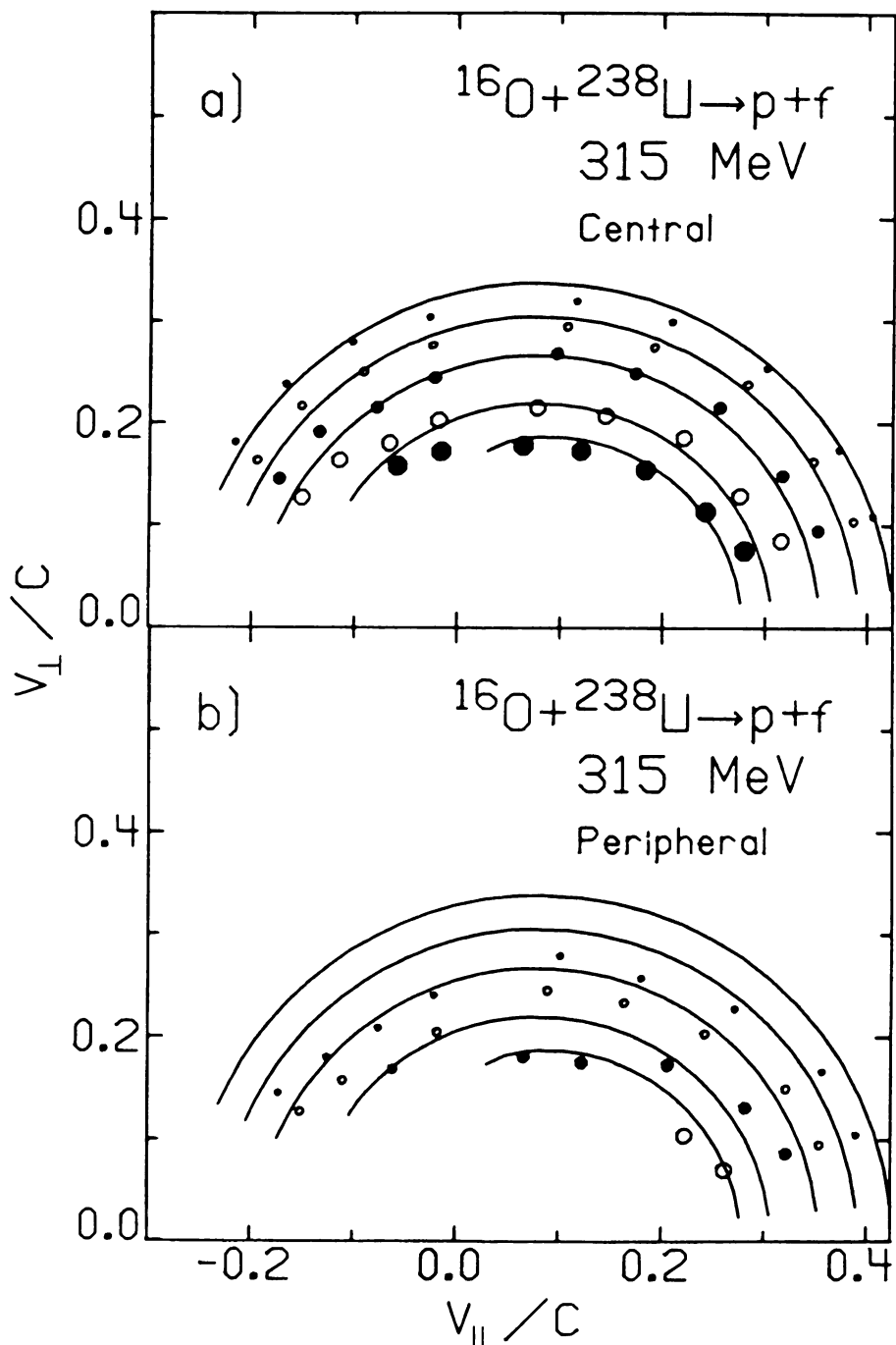
Figure V-24. Contour plot of the Lorentz invariant proton cross section. The contours are in the ratios 1:4:4:4:2. The curves describe the emission from a single thermal source moving with slightly less than half the beam velocity. The cross sections for "central" collisions are shown in part (a), the ones for "peripheral" collisions are shown in part (b).
