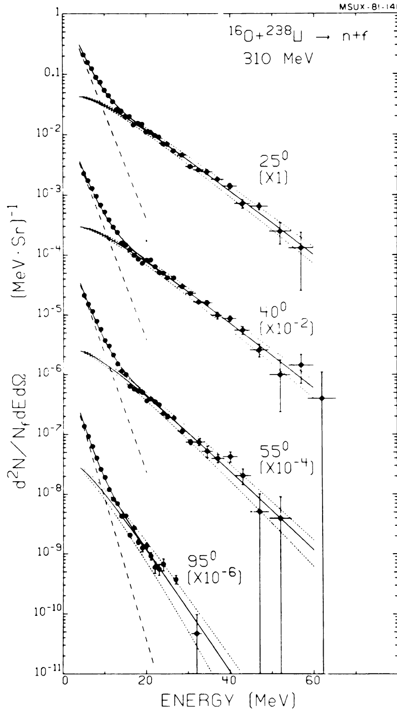
Figure VI-13. Differential neutron multiplicities per fission event measured for the reaction ^{238}\text{U} (^{16}\text{O}, \text{nf}) at 310 MeV. The solid and dashed lines show the decomposition into equilibrium and nonequilibrium components, respectively. The dotted lines indicate the estimated errors within which the high energy regions of the neutron spectra are established. These limits are used for the comparison with the proton spectra in Figure VI-14.
