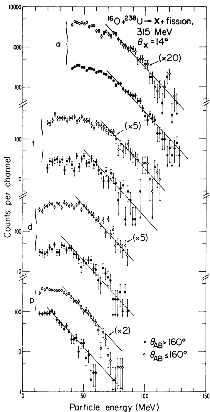
Figure V-8. Laboratory energy spectra of protons, deuterons, tritons, and \alpha -particles detected in the \theta = 14^\circ Si-NaI telescope in coincidence with fission fragments with folding angles \theta_{AB} < 160^\circ (open circles, central collisions) and with folding angles \theta_{AB} > 160^\circ (filled circles, peripheral collisions).
