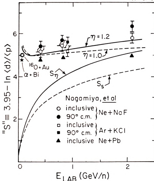
Figure VI-2. The bombing energy dependence of the entropy (taken from Stöcker [St 80]) as calculated for a viscous ( S_\eta ) and an inviscid fluid ( S_s ). Also shown are the "entropy" values, "S" , calculated using the measured d/p-ratios via Eq. (VI-5). The measured values are taken from Nagamiya et. al. [Na 81], Wu et. al. [Wu 79] ( \alpha + Bi at E/A = 25 MeV) and from the present study ( ^{16}O + Au at E/A = 20 MeV). The solid (dashed) lines denoted by \eta = 1.2 ( \eta = 1.0 ) represent the viscous (inviscid) calculation of "S" from the calculated d/p-ratios.
