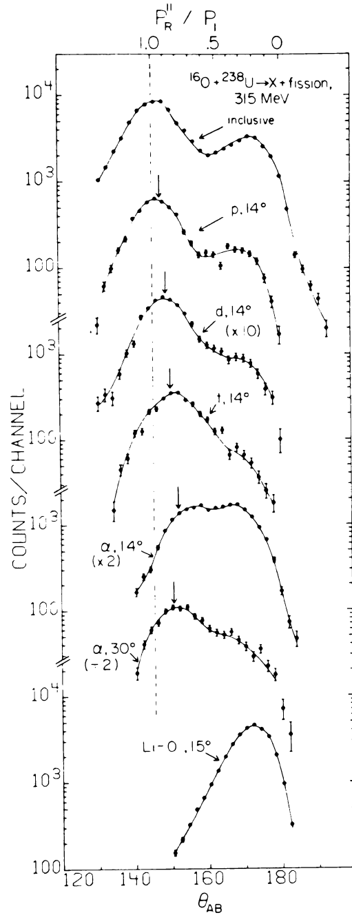
Figure IV-4. Folding-angle distributions of fission fragments measured inclusively (top), in coincidence with protons, deuterons, tritons, and \alpha -particles in the \theta = 14^\circ Si-NaI telescope, in coincidence with \alpha -particles in the \theta = 30^\circ in-plane telescope and in coincidence with heavy projectile residues (Li-O) in the heavy ion telescope at \theta = 15^\circ . The momentum scale at the top of the figure corresponds to the solid curve of Figures III-5 and III-6.
