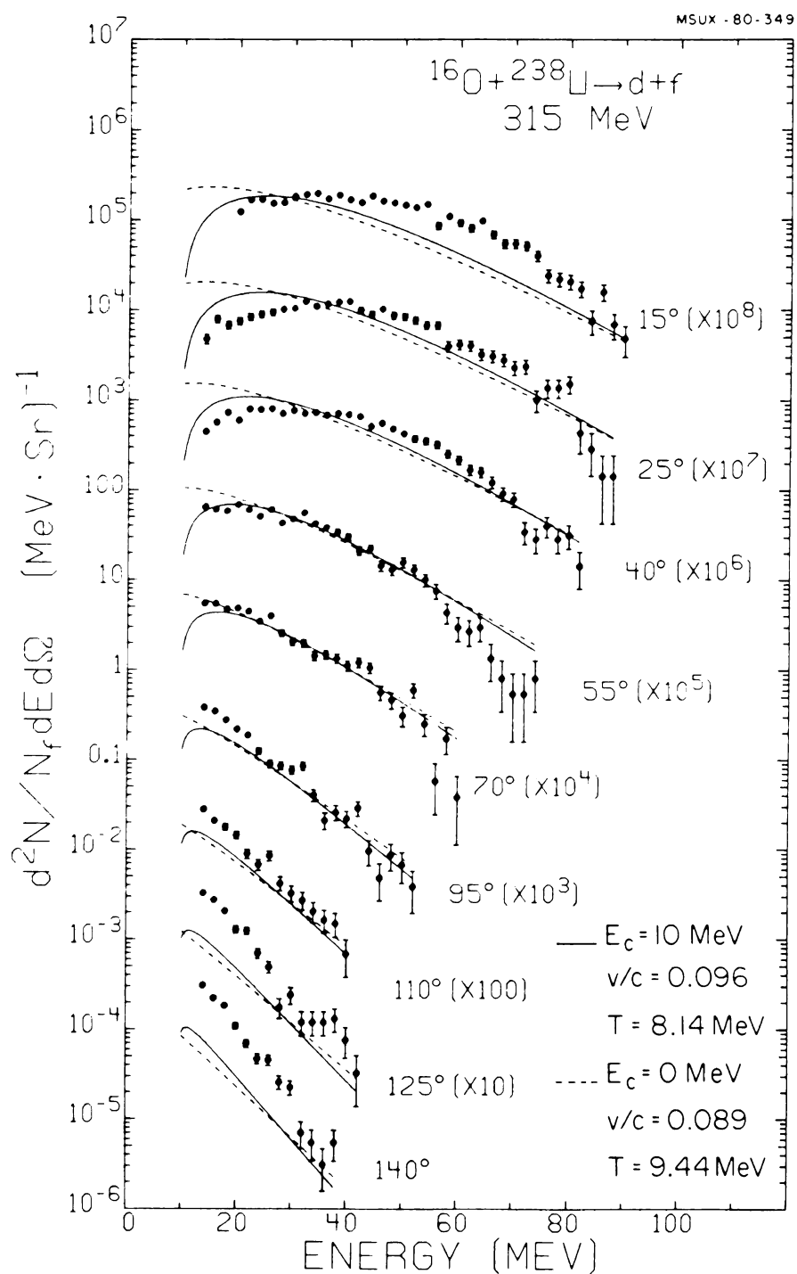
Figure V-27. Energy spectra of deuterons detected in the reaction ^{238}\text{U} (160, \text{df}) at 315 MeV. The curves have been calculated with the moving source model of Eq. (V-10). The laboratory angles and moving source parameters are indicated.
