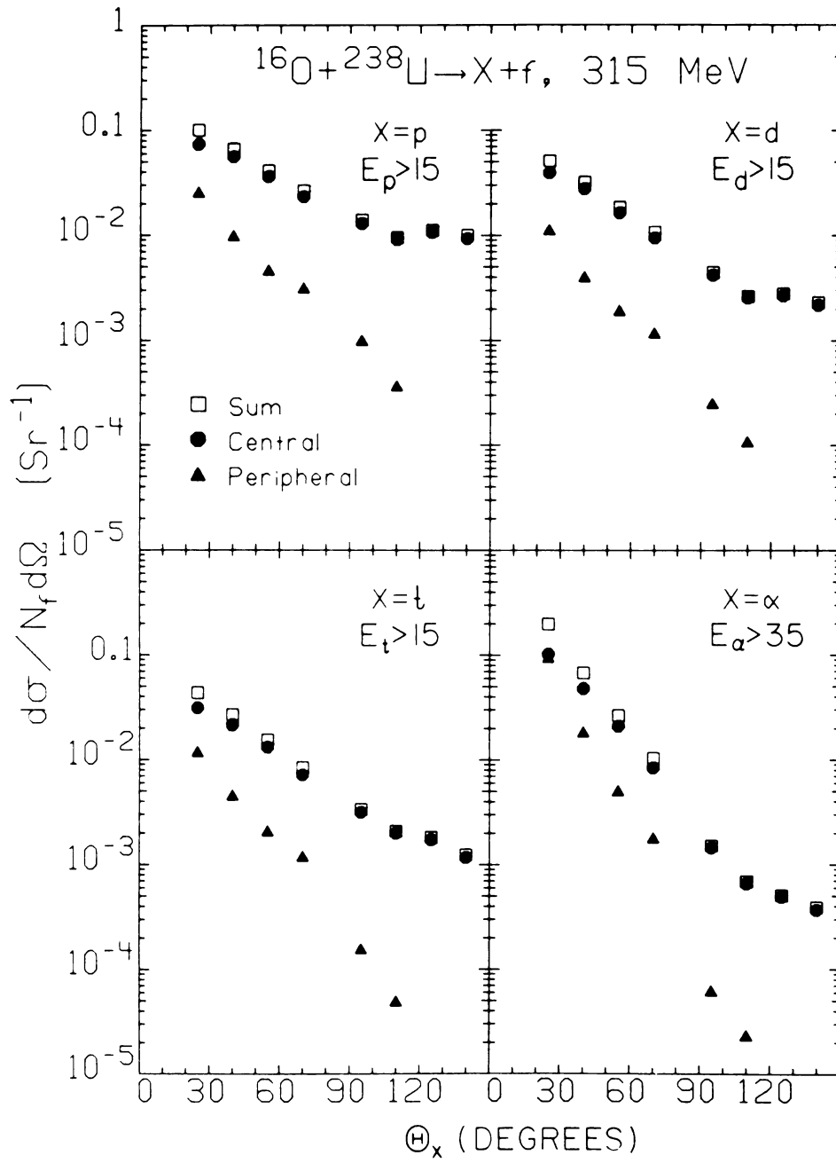
Figure V-7. Angular distributions of light particles, p, d, t, and \alpha , in coincidence with fission fragments produced in central and peripheral collisions. The sum of the two contributions is also shown. The lower energy cutoffs are given in the figure. The cross-sections are normalized to fission singles.
