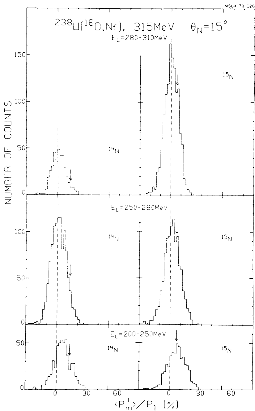
Figure IV-6. Missing momentum distributions for 3 different gates on the laboratory energy of ^{14}\text{N} and ^{15}\text{N} projectile residues. \langle P_m^{\parallel} \rangle is positive in the beam direction.
