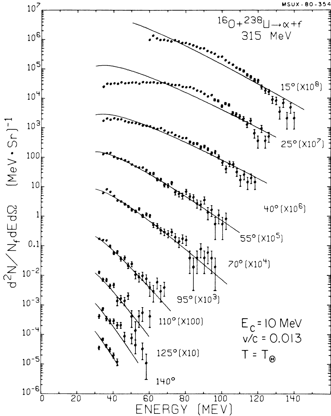
Figure V-20. Energy spectra of alpha-particles detected in the reaction ^{238}\text{U} (^{16}\text{O}, \alpha f) at 315 MeV. The spectra are labeled by the detection angle of the coincident alpha-particles. The cross sections are normalized to fission singles. The data are fit with the rotating hot spot model of Eq. (V-3).
