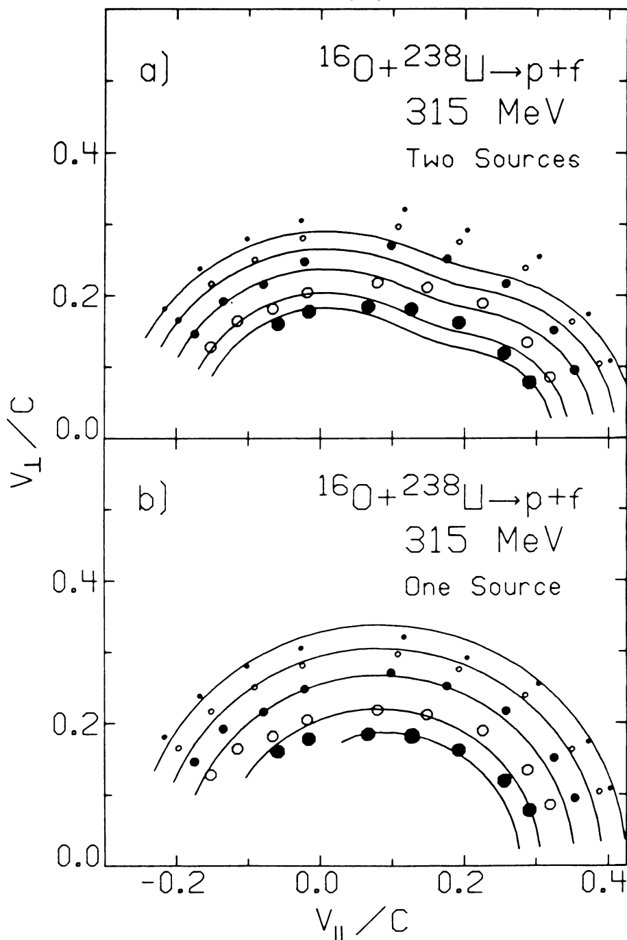
Figure V-23. Contour plot of the Lorentz invariant proton cross section. The contours are in the ratios 1:4:4:4:2. The experimental data are given by circles. The curves in part (a) represent the cross sections calculated for thermal emission from two sources, one moving with the beam velocity and the other moving with the compound nucleus velocity (see also solid curves in Figure V-25). The curves in part (b) describe the emission from a single thermal source moving with slightly less than half the beam velocity (see solid curves in Figure V-26).
